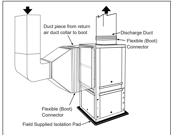
Figure 10: Typical installation using ducted return
