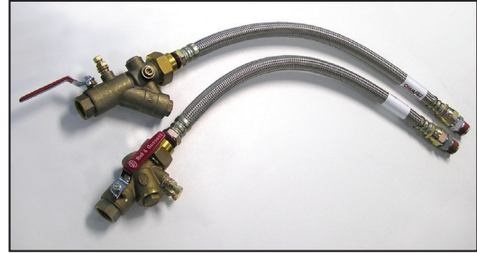
Figure 3: Supply and return hoses
