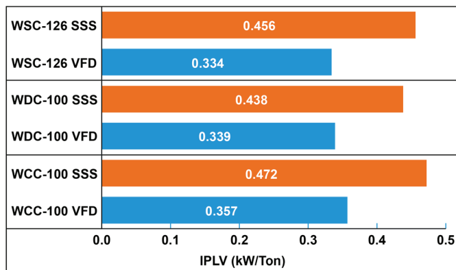
Figure 10: IPLV Comparison by Model
