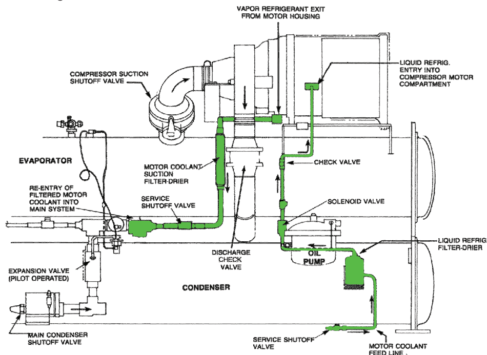
Figure 7: WDC Motor Cooling
