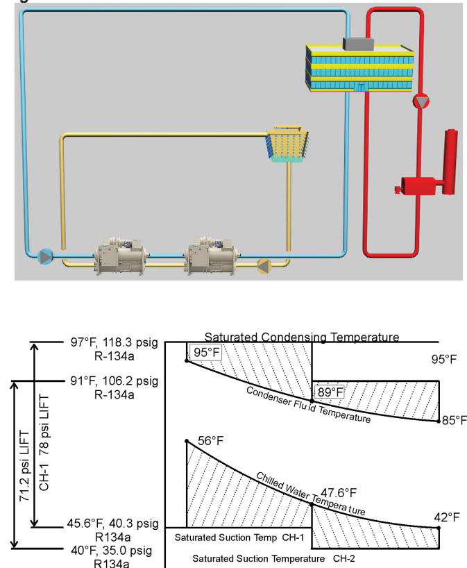
Figure 13: Series Counterflow Flow
