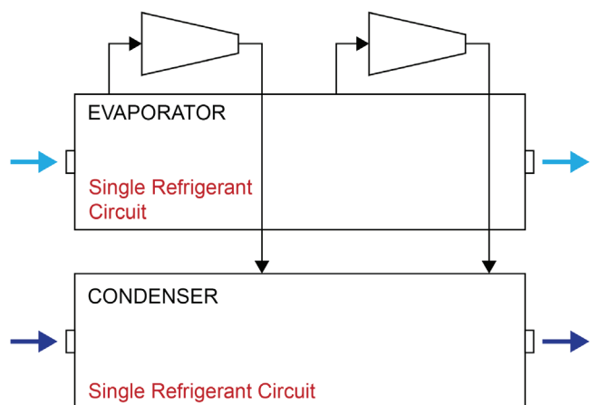
Figure 6: Single Circuit WDC Chillers
