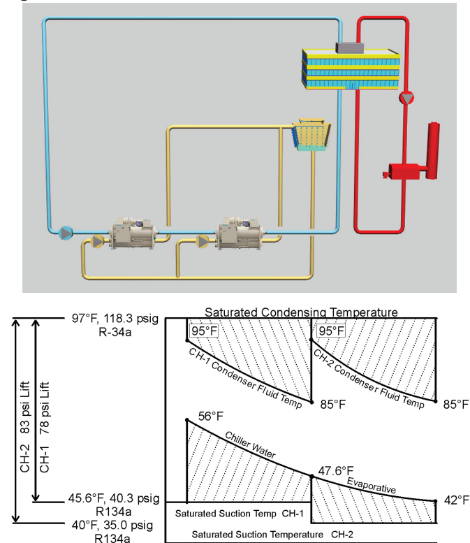
Figure 12: Series Parallel Flow
