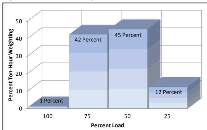
Figure 16: IPLV Defined by AHRI Standard 550/590
