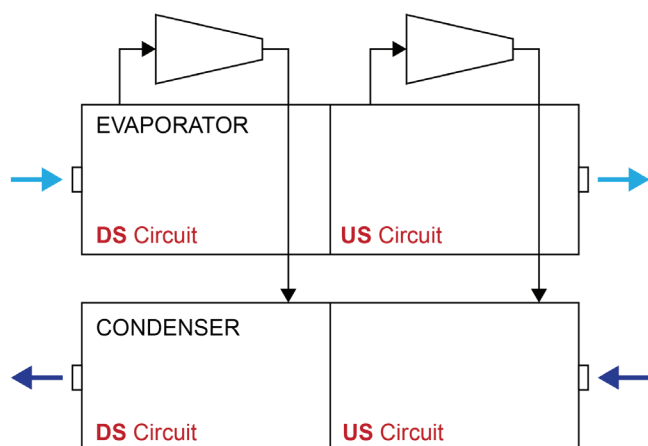
Figure 5: Dual Circuit WCC Counterflow Chillers
