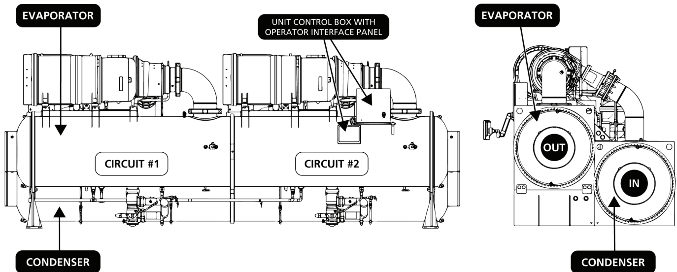
Figure 9: WCC Layout
