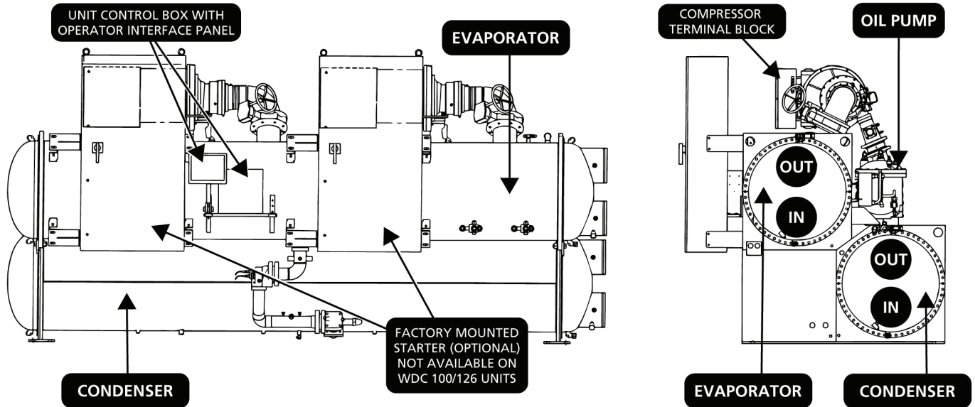
Figure 8: WDC Layout
