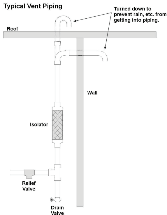
Figure 17: Typical Vent Piping
