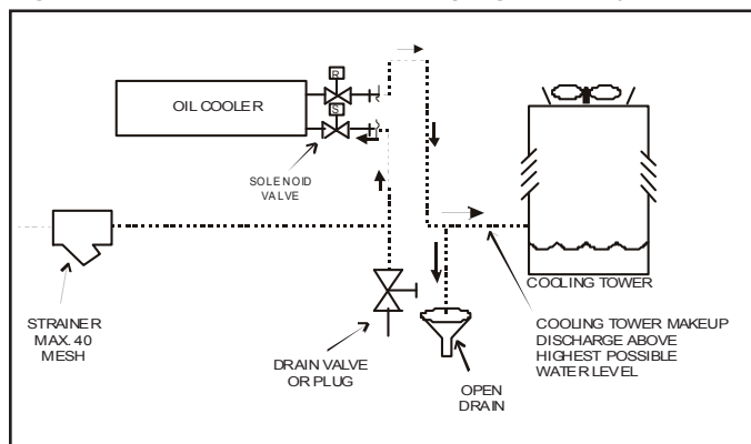
Figure 15: WDC/WCC Oil Cooler Piping With City Water
