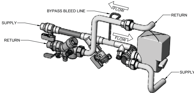
Figure 8: Bypass Bleed Line
