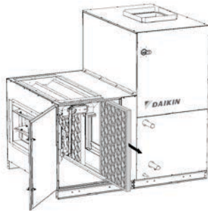
Figure 26: Filter Access Doors
