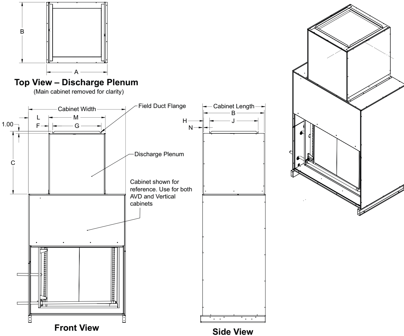
Figure 49: Vertical Discharge Plenum (Sizes 030-050)
