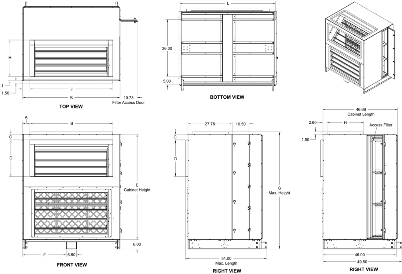
Figure 55: Economizer Dimensions (Sizes 060-100)
