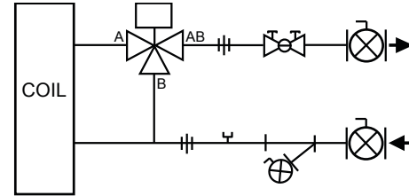
Figure 38: Deluxe 3-Way Valve Package (Manual CS)
