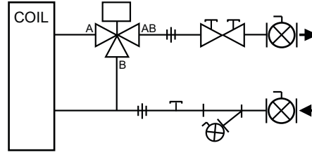
Figure 36: Deluxe 3-Way Valve Package (Auto CS)
