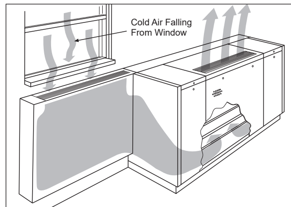
Figure 40: DraftStop Window Downdraft Protection
