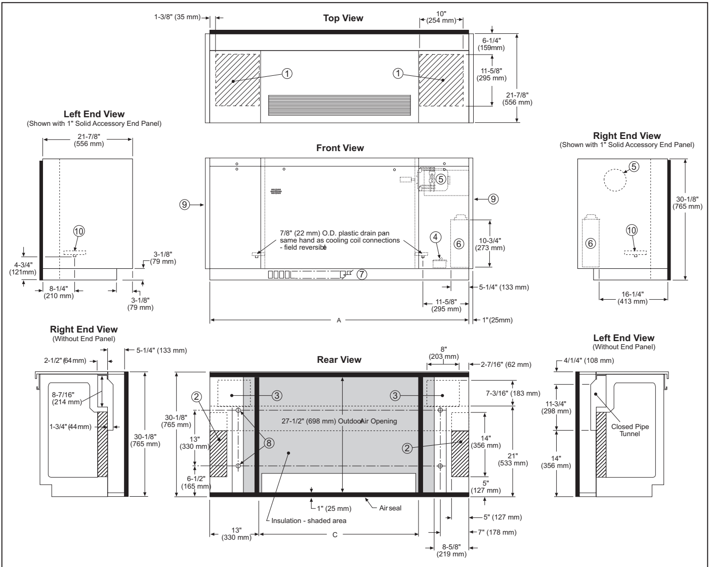
Figure 44: Arrangement AN – Full Adapter Back with Closed Pipe Tunnel, 21-7/8" Deep
