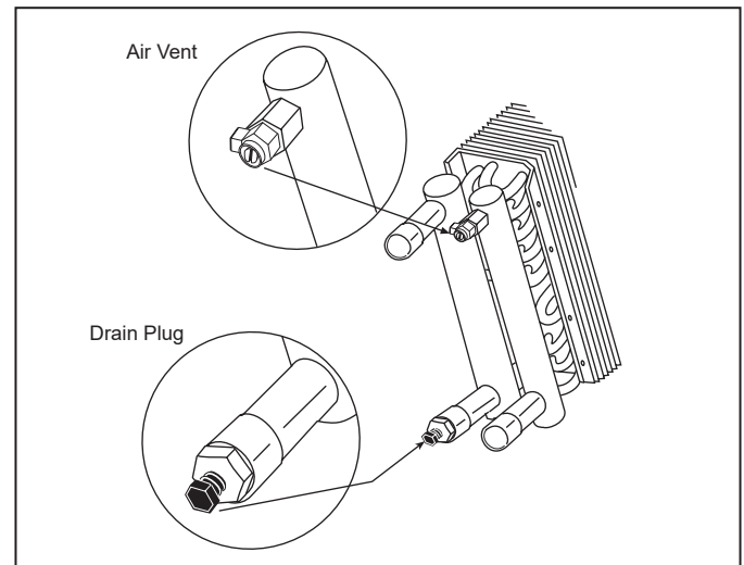
Figure 111: Manual Air Vent and Drain Plug
