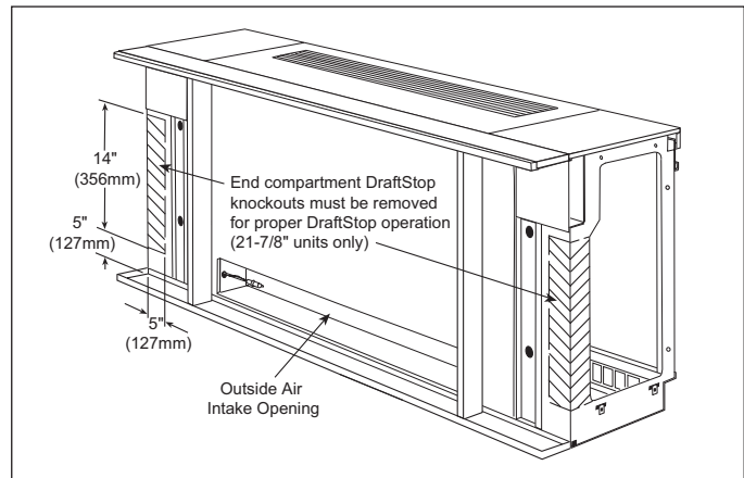
Figure 123: DraftStop Knockouts
