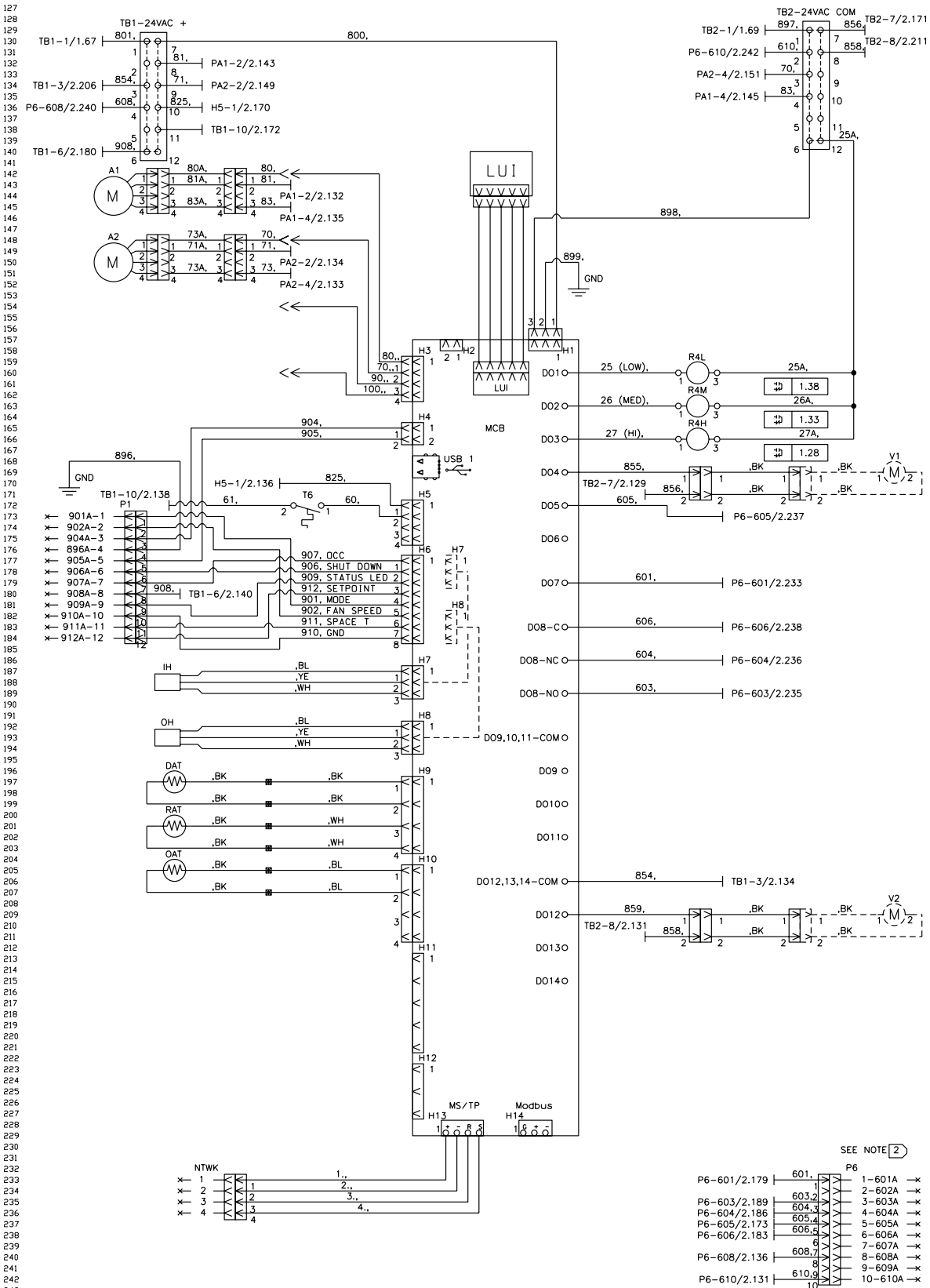
Figure 89: Typical MicroTech Wiring Diagram – 115V / 60Hz / 1Ph
