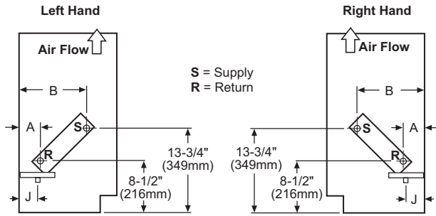
Figure 71: Steam Heating Only Unit (Coils 68, 69, 78, 79)
