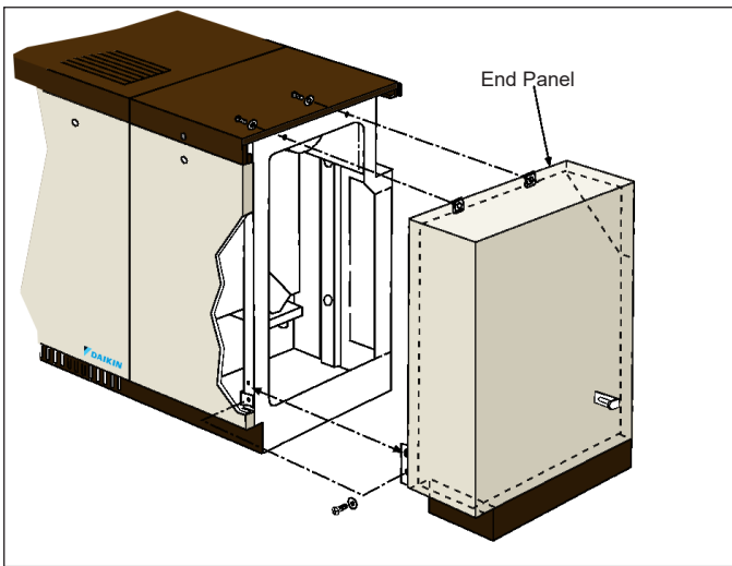
Figure 31: End Panels (6" End Panel Shown)
