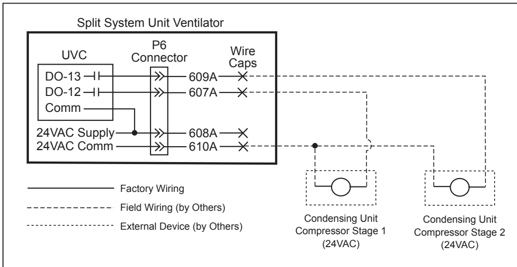
Figure 95: Split-System Condensing Unit Signal Wiring
