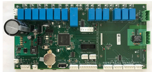
Figure 100: MicroTech Control Board
