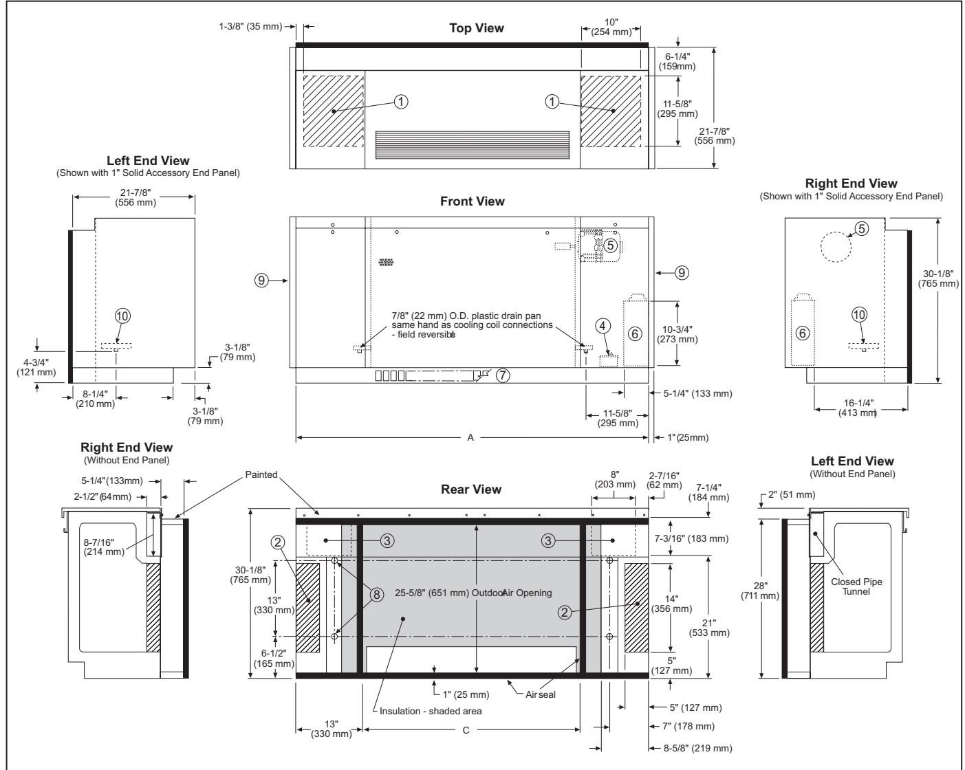
Figure 45: Arrangement AM – Full Adapter Back with 2" Step Down; Closed Pipe Tunnel, 21-7/8" Deep
