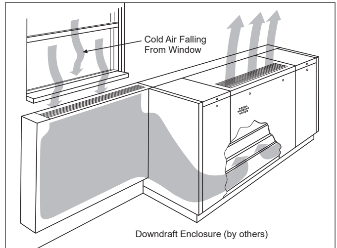
Figure 122: DraftStop Window Downdraft Protection
