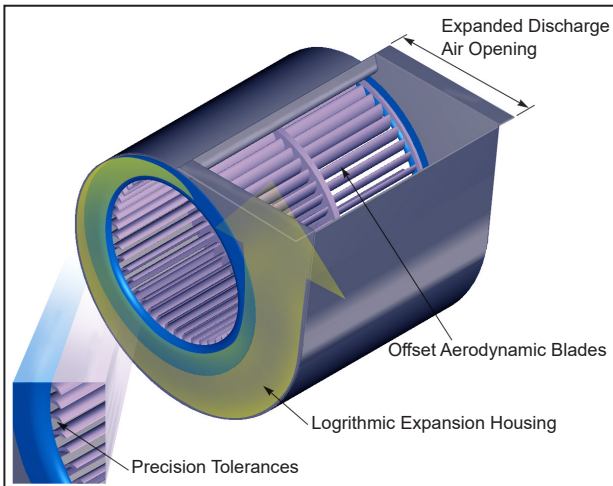
Figure 2: GentleFlo Reduced Turbulence
