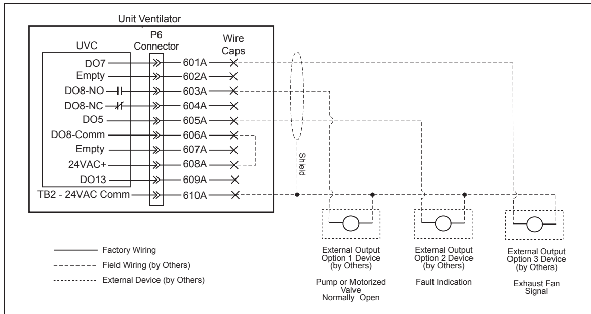
Figure 90: External Output Wiring - Single Unit
