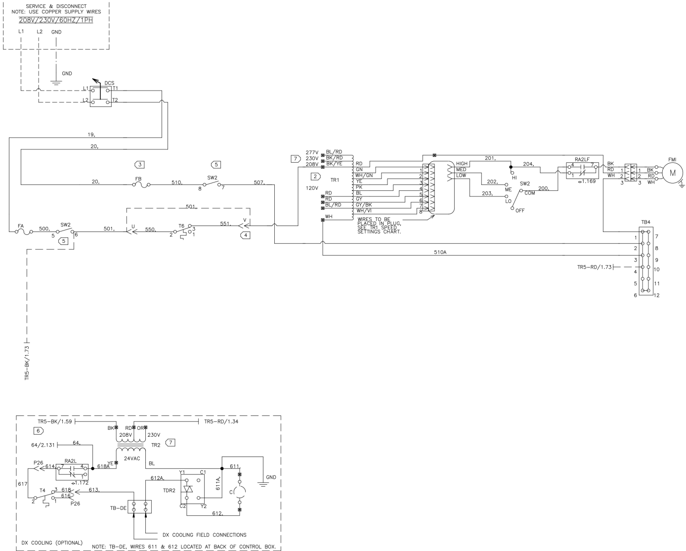
Figure 99: Controls by Others – Field Installed - 208-230 V/60 Hz/1 Ph
