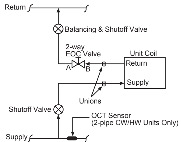
Figure 131: 2-Way Hot Water EOC Valve Piping
