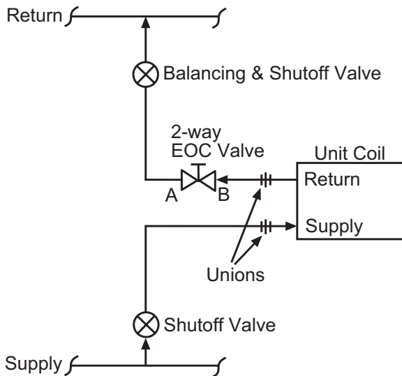
Figure 133: 2-Way Chilled Water EOC Valve Piping
