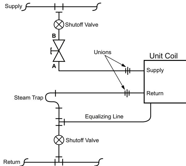
Figure 139: 2-Way Steam End of Cycle Valve Piping
