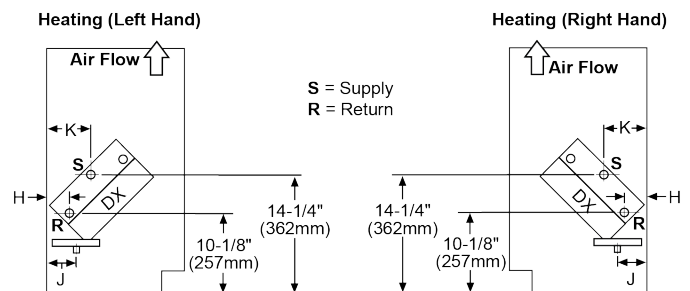
Figure 52: Steam Heating Coils 68, 69, 78, 79
