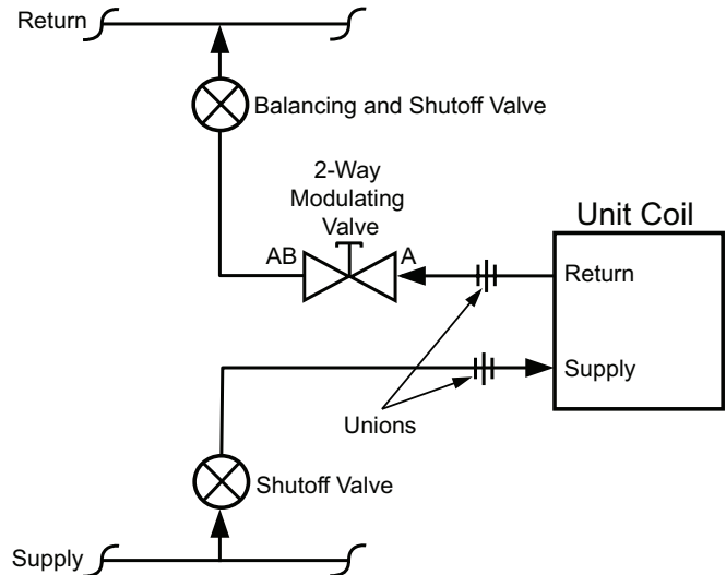
Figure 137: 2-Way Chilled Water Modulating Valve Piping
