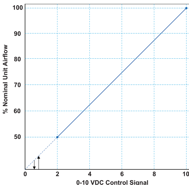
Figure 120: 0-10VDC Motor Operation
