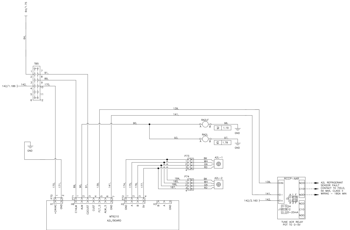
Figure 103: Controls by Others – Field Installed - 265 V/60 Hz/1 Ph
