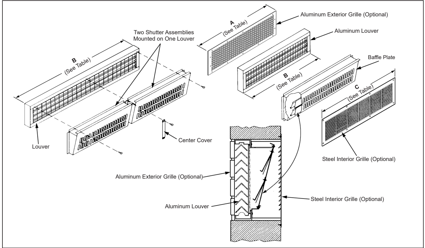
Figure 79: VentiMatic Shutter Assembly with Optional Grille
