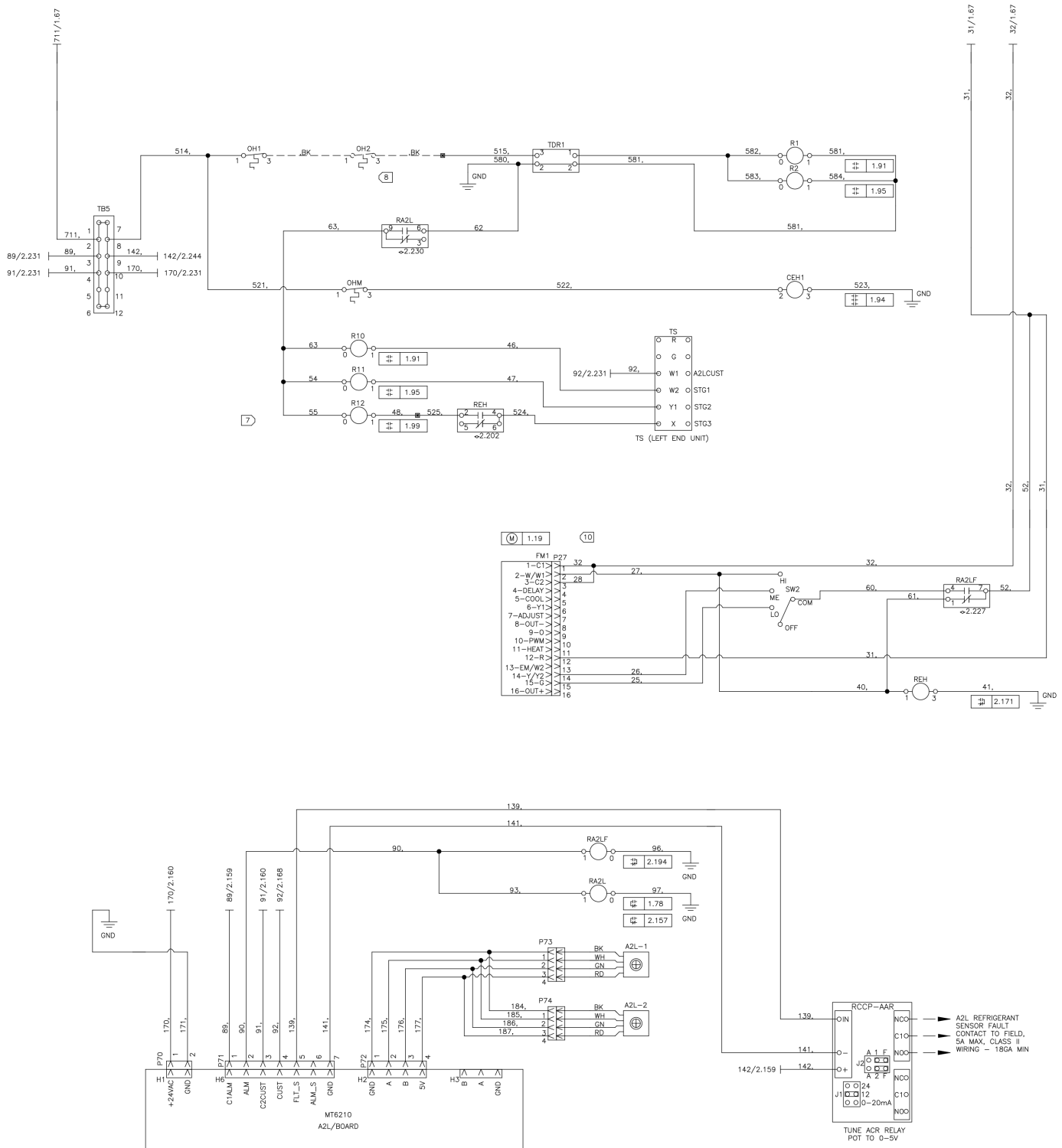
Figure 105: Electric Heat Wiring Diagram – Typical 460 V/60 Hz/3 Ph
