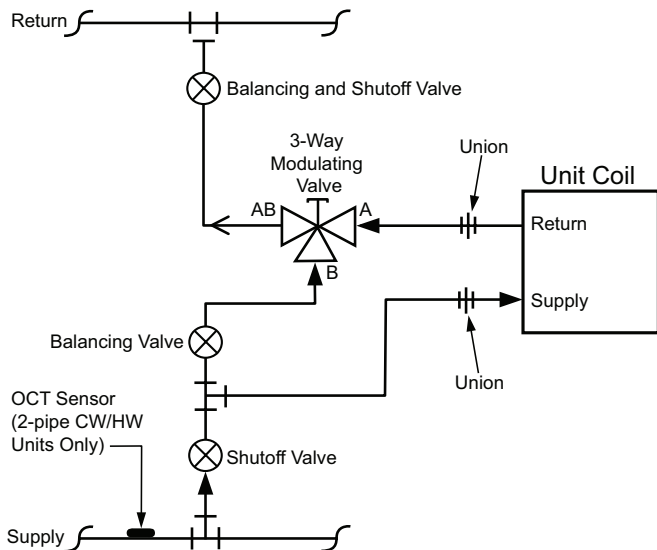
Figure 136: 3-Way Hot Water Modulating Valve Piping
