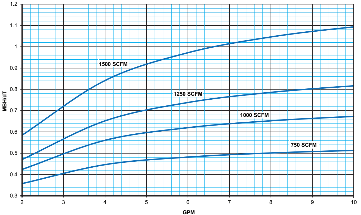
Figure 81: 2-Row Hot Water Coil (Parallel Flow)
