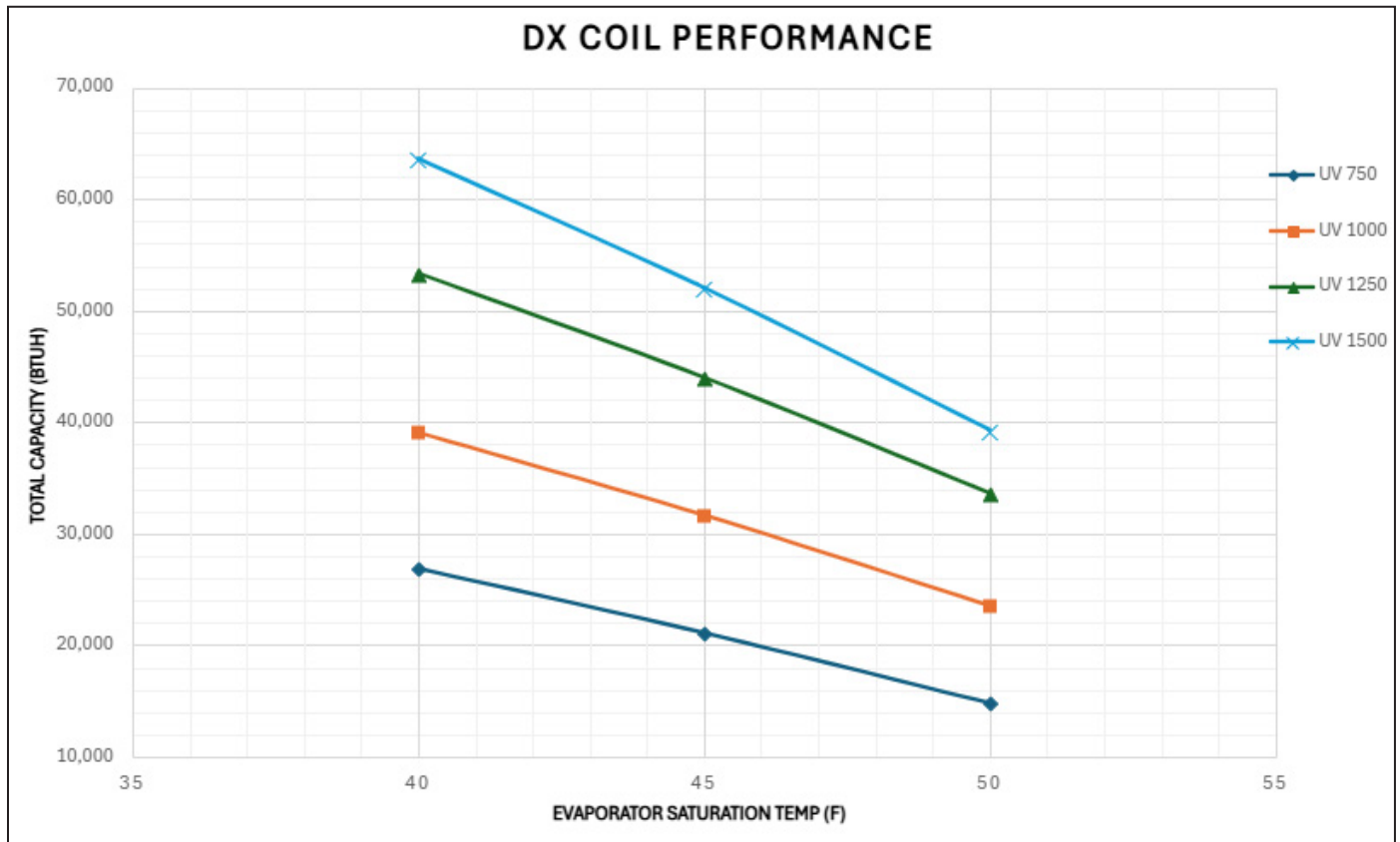
Figure 84: DX Coil Estimated Performance (Mbh at 115°F Liquid Temperature)
