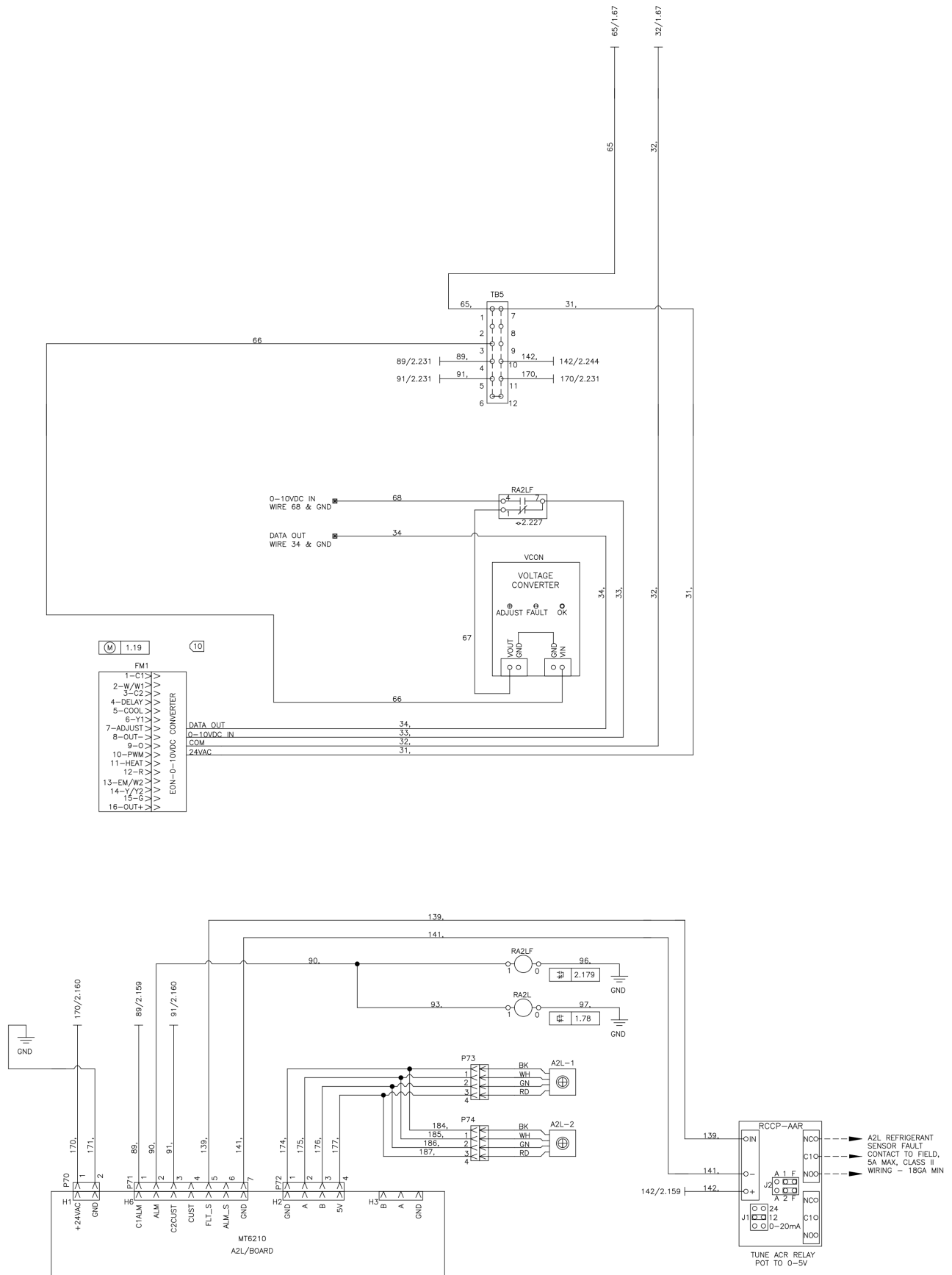
Figure 94: Variable Airflow 208-230V /60 Hz/1 Ph – Motor Switchbox, Non-Electric Heat Units
