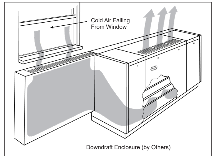
Figure 128: DraftStop Window Downdraft Protection
