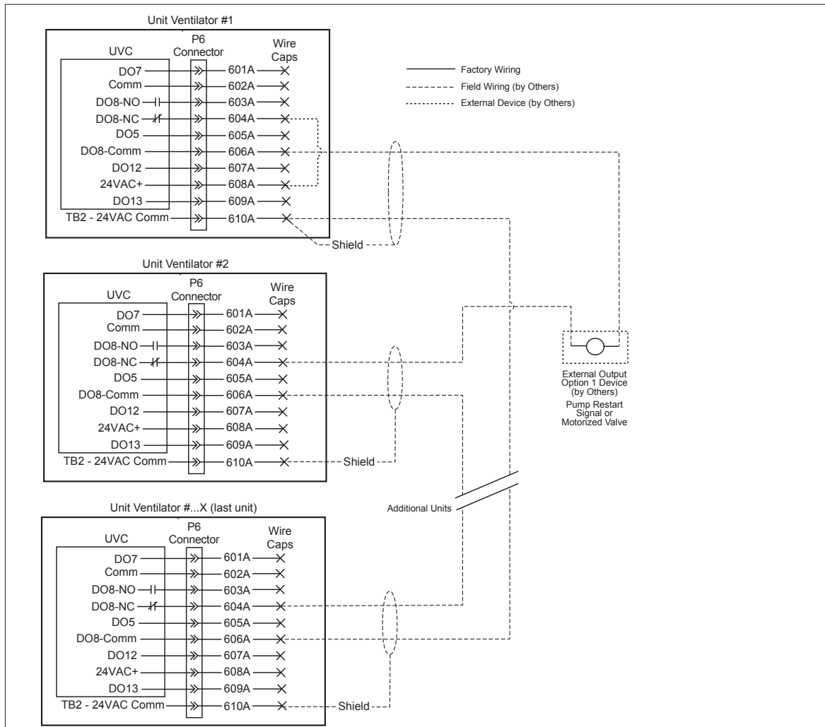
Figure 91: External Output Wiring - Multiple Units Shown
