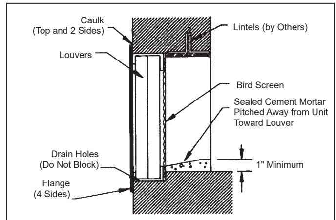
Figure 123: Flanged Wall Louver Installation Detail
