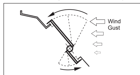
Figure 21: Room Air Damper Auto-Closed by Wind Gusts
