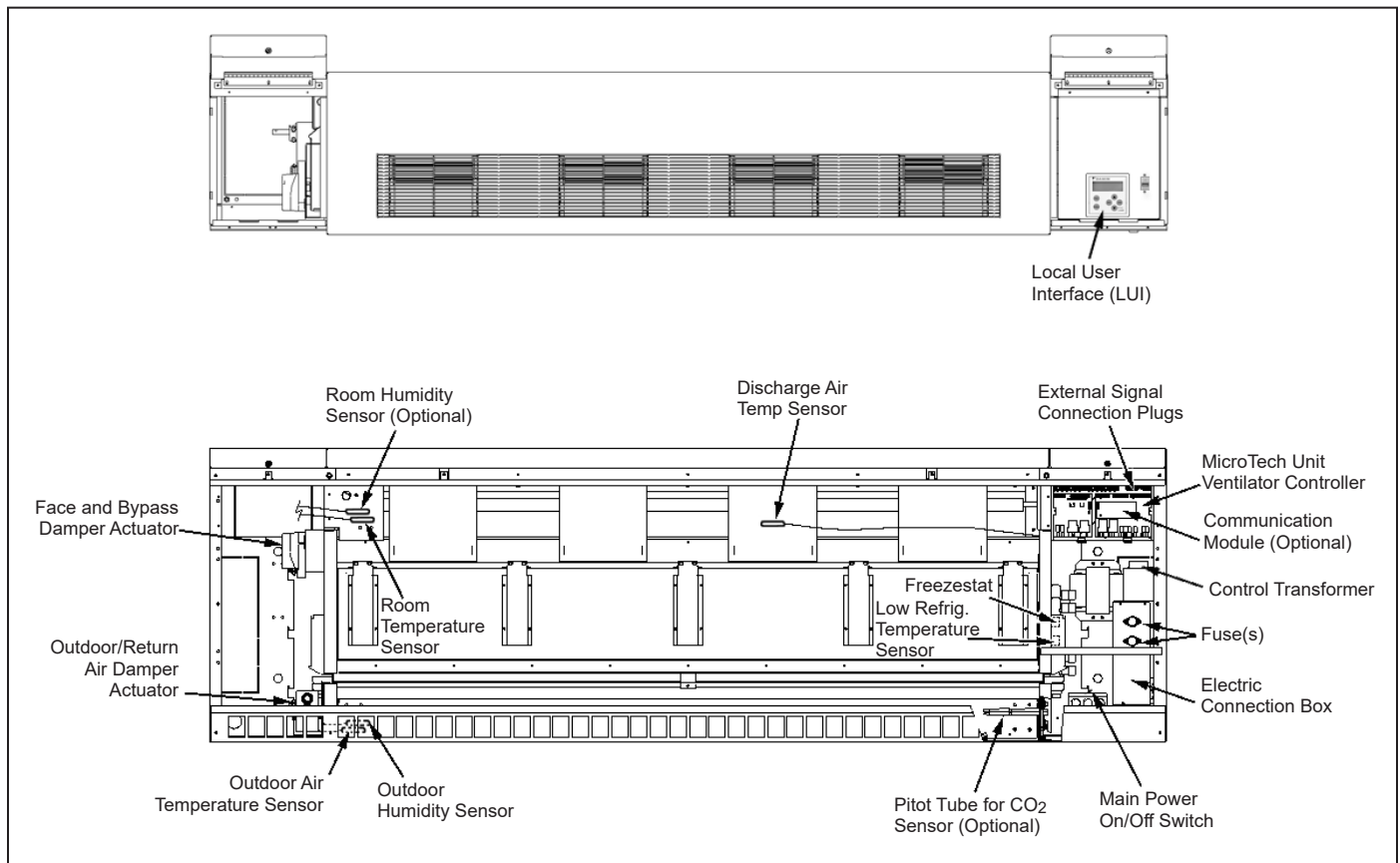
Figure 108: MicroTech Sensor and Component Locations
