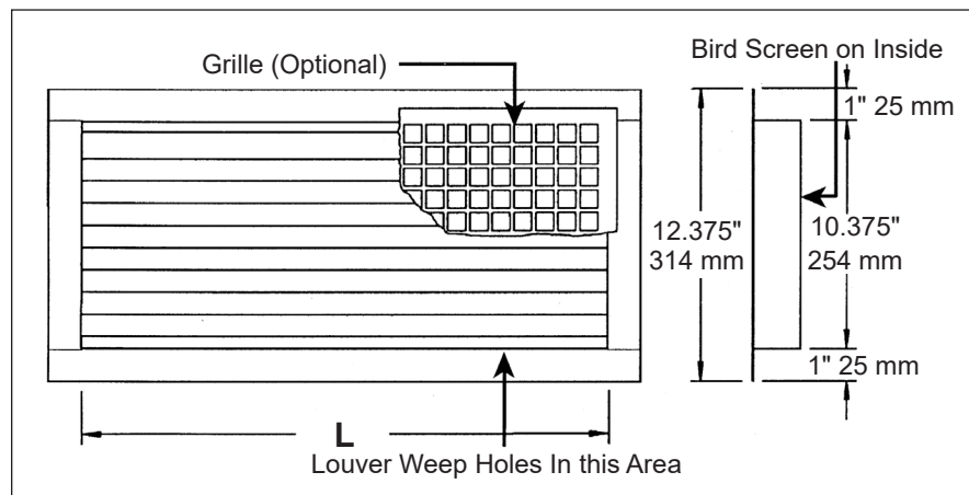
Figure 77: Louver with Flange (Horizontal Blades Shown)
