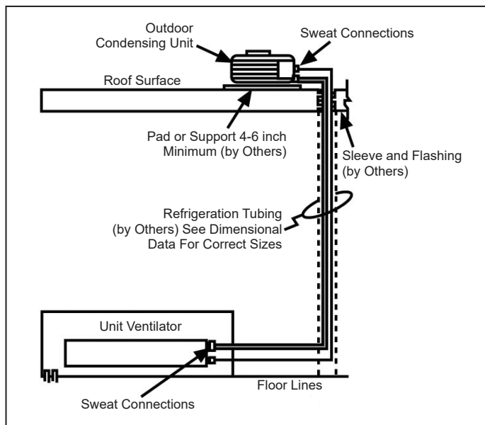
Figure 119: Typical DX System Piping
