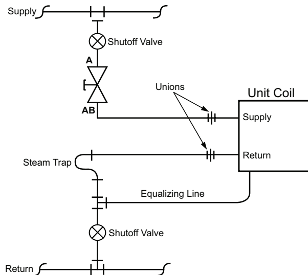
Figure 140: 2-Way Steam Modulating Valve Piping
