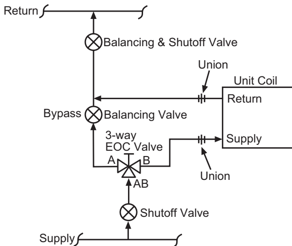
Figure 134: 3-Way Chilled Water EOC Valve Piping
