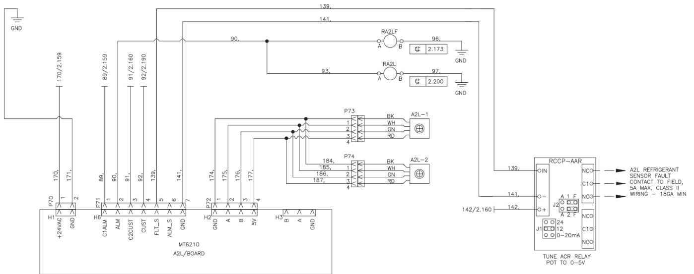
Figure 85: Electromechanical Controls – A2L Leak Mitigation
