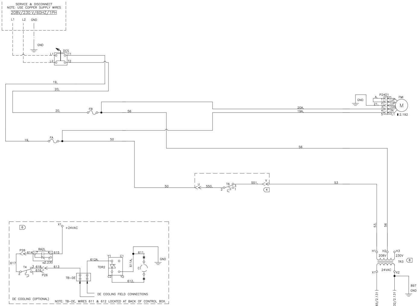
Figure 93: Variable Airflow 208-230V /60 Hz/1 Ph – Motor Switchbox, Non-Electric Heat Units
