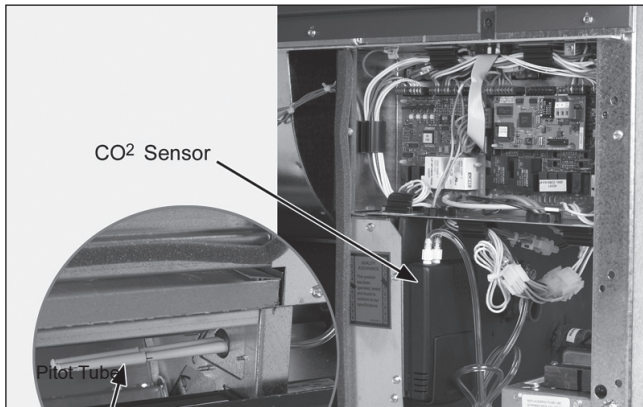
Figure 109: CO 2 Sensor for Demand Control Ventilation
