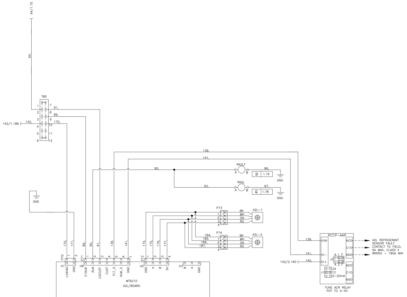
Figure 101: Controls by Others – Field Installed - 115 V/60 Hz/1 Ph
