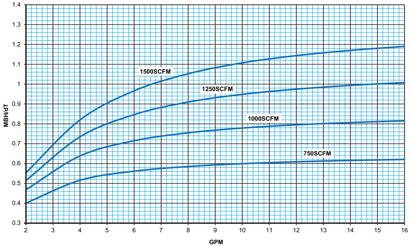
Figure 82: 3-Row Hot Water Coil (Parallel Flow)
