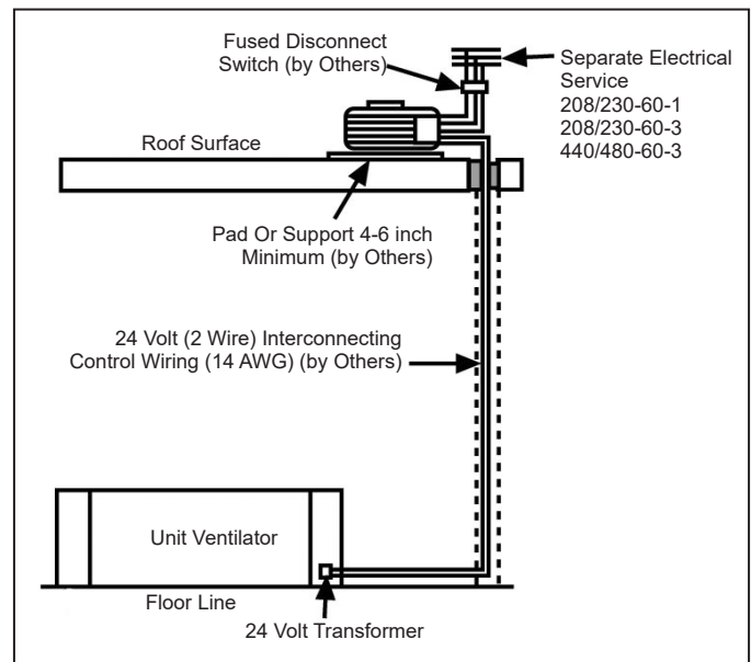
Figure 118: Typical DX System Wiring
