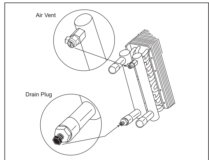
Figure 117: Manual Air Vent and Drain Plug
