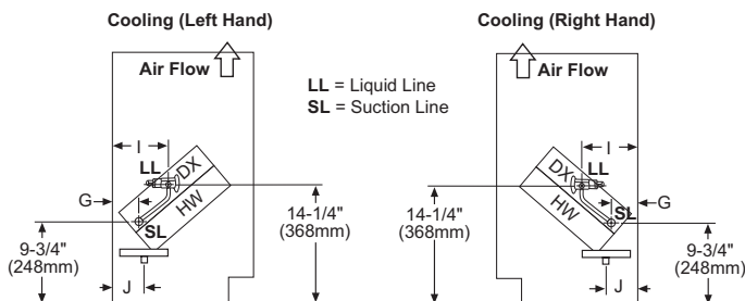
Figure 49: Direct Expansion Cooling Coils G[9], M[0]
