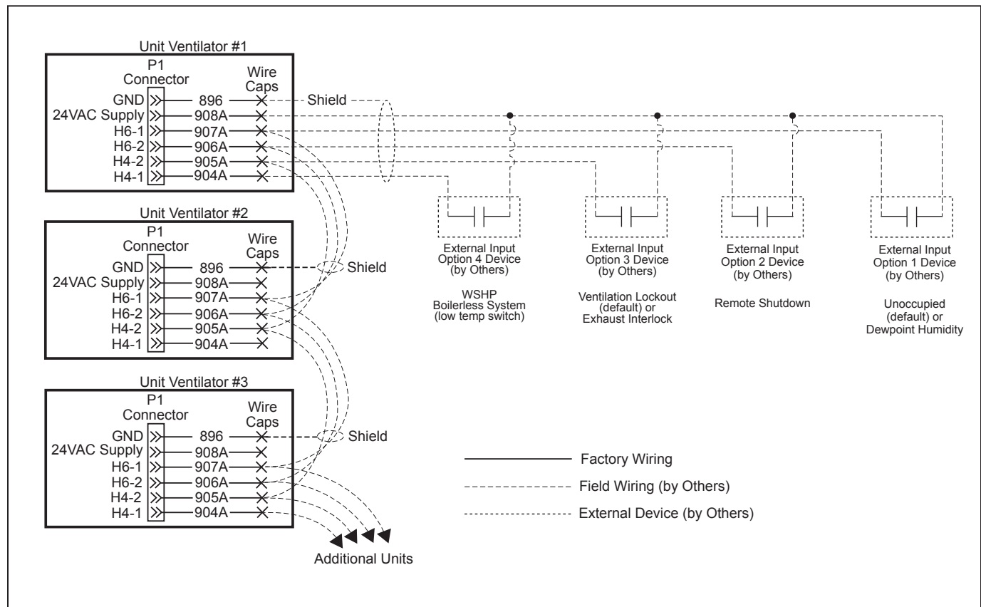
Figure 89: External Input Wiring Examples with or Without Daisy Chaining of Units
