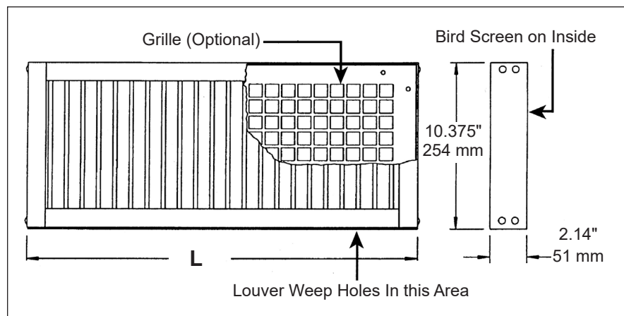
Figure 78: Louver Without Flange (Vertical Blades Shown)
