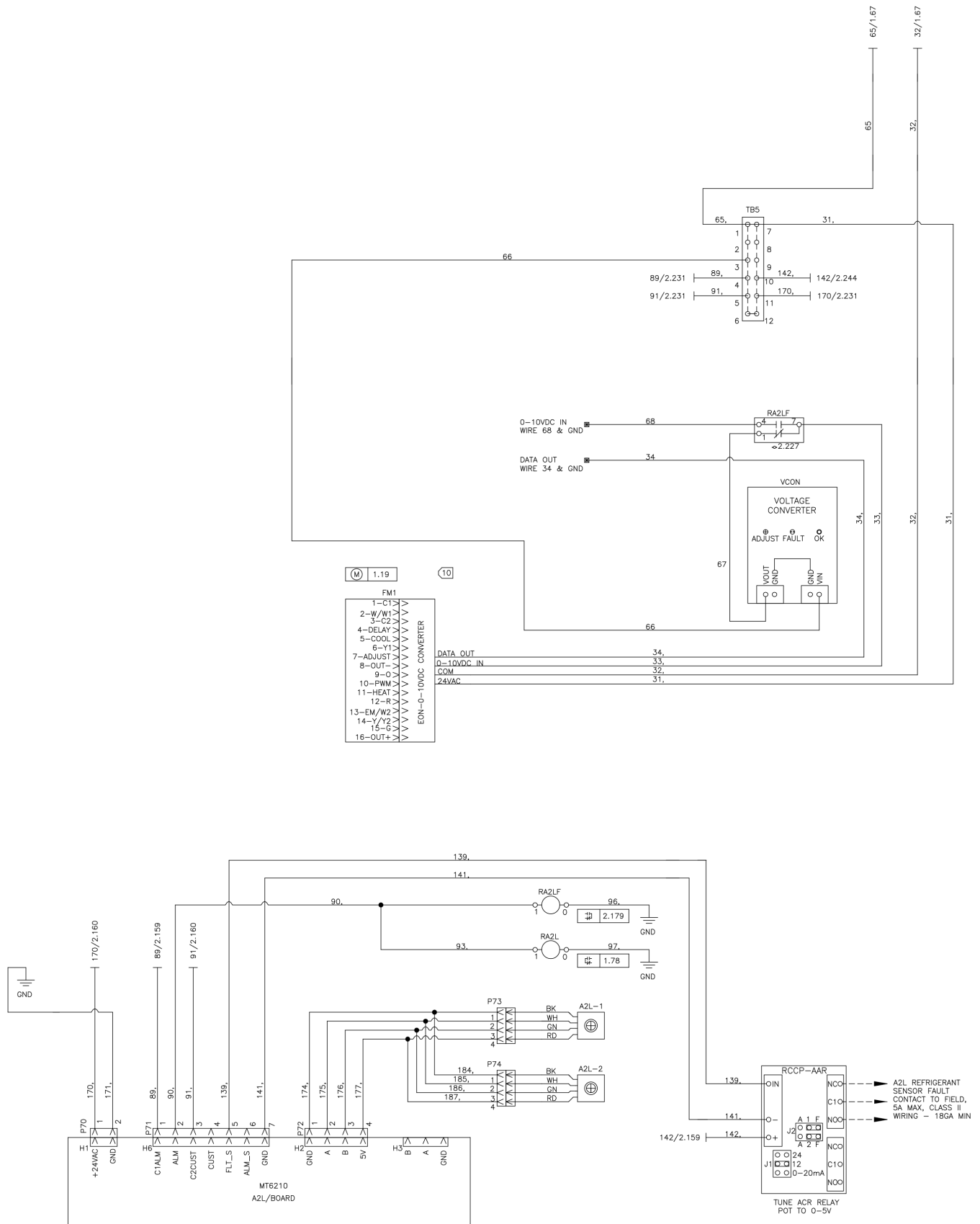
Figure 98: Variable Airflow 265 V/60 Hz/1 Ph – Motor Switchbox, Non-Electric Heat Units
