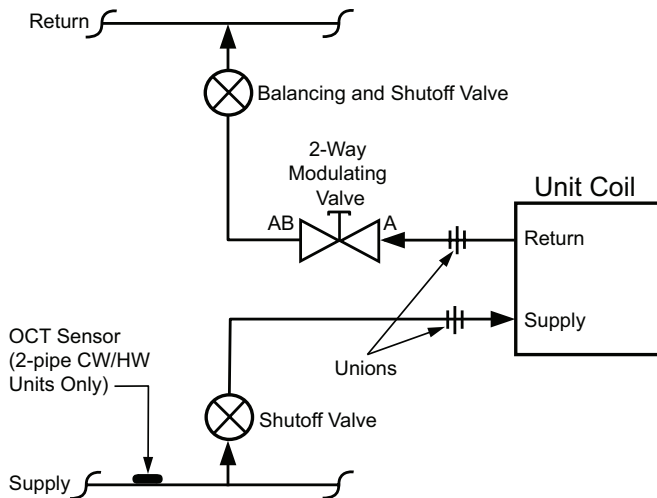
Figure 135: 2-Way Hot Water Modulating Valve Piping
