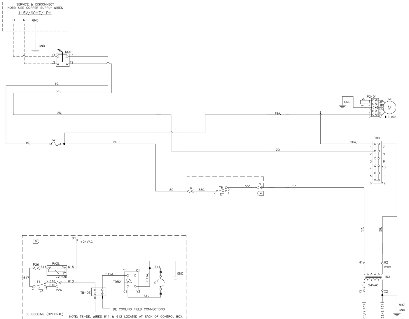
Figure 95: Variable Airflow 115 V/60 Hz/1 Ph – Motor Switchbox, Non-Electric Heat Units
