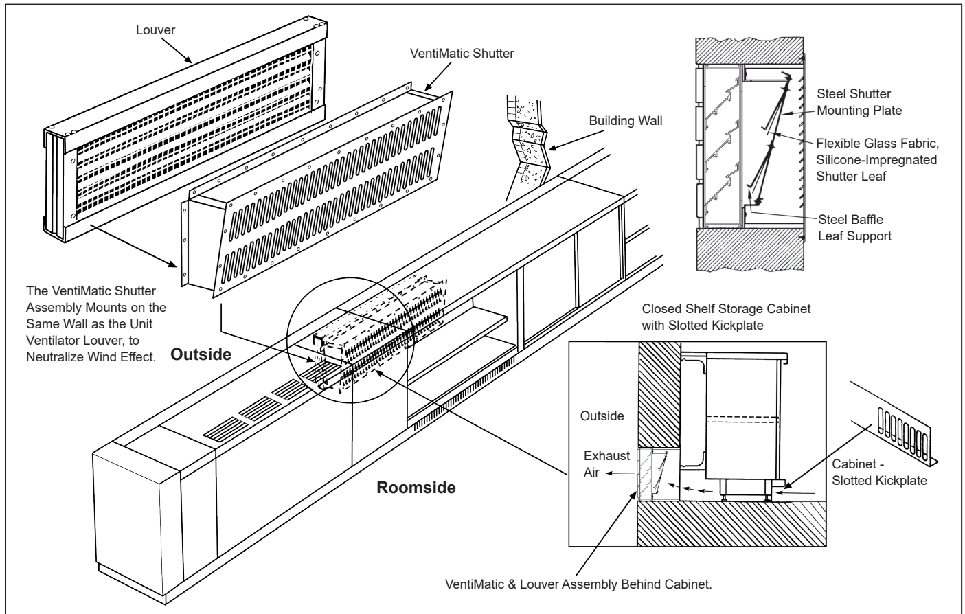
Figure 127: VentiMatic Shutter Installation
