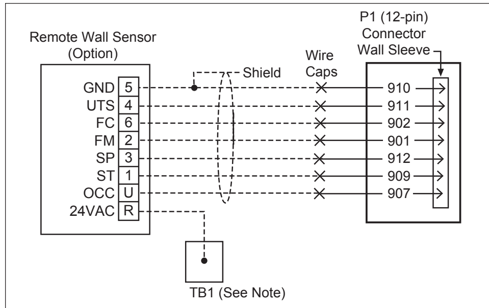
Figure 88: Wall-Mounted Temperature Sensor Wiring
