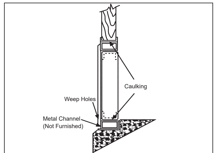
Figure 124: Panel Wall Louver Installation Detail
