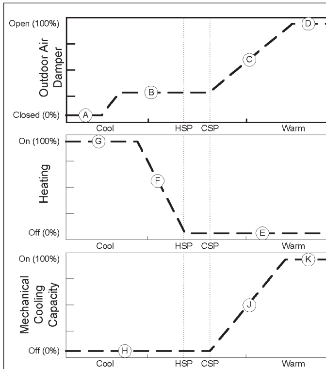
Figure 121: ASHRAE Cycle II Operation
