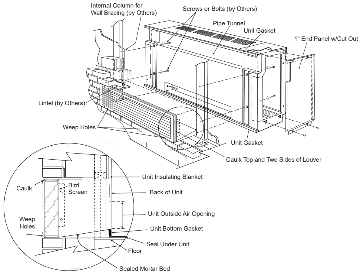
Figure 125: Recessed Wall Louver Installation Detail
