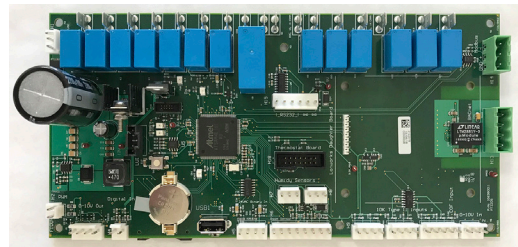
Figure 106: MicroTech Control Board
