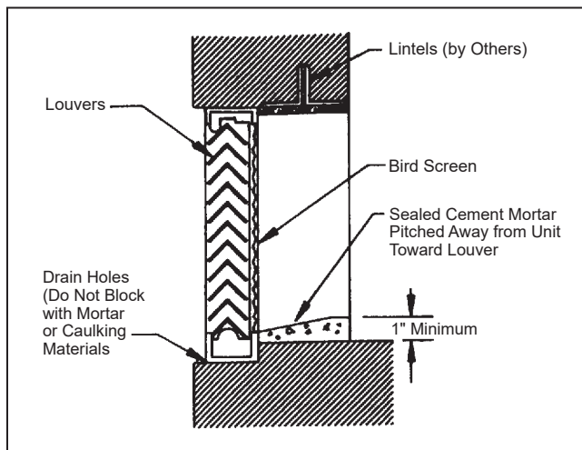
Figure 122: Recessed Wall Louver Installation Detail
