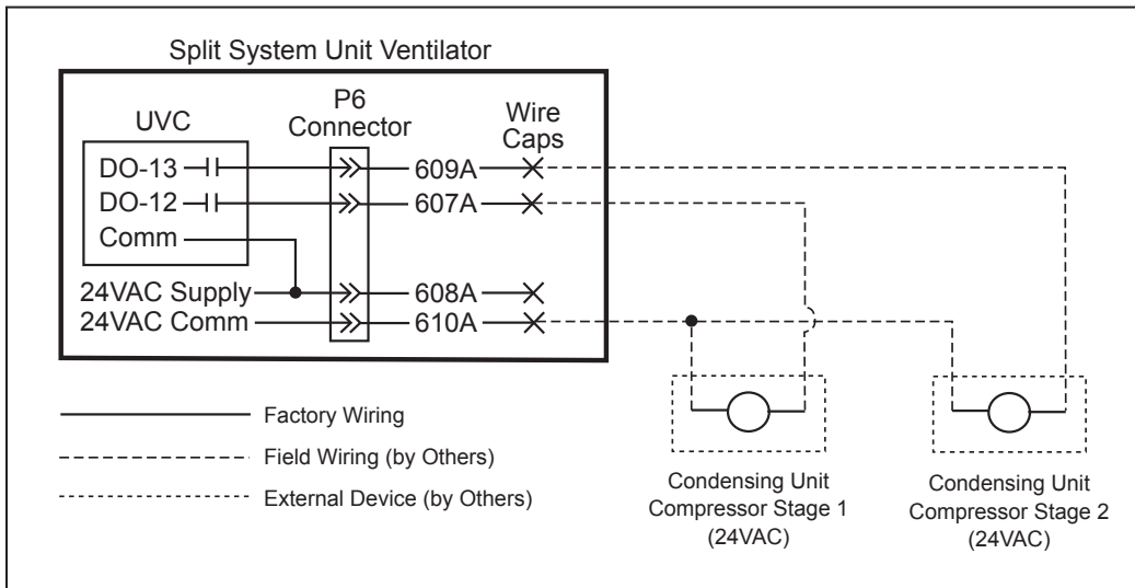
Figure 92: Split-System Condensing Unit Signal Wiring
