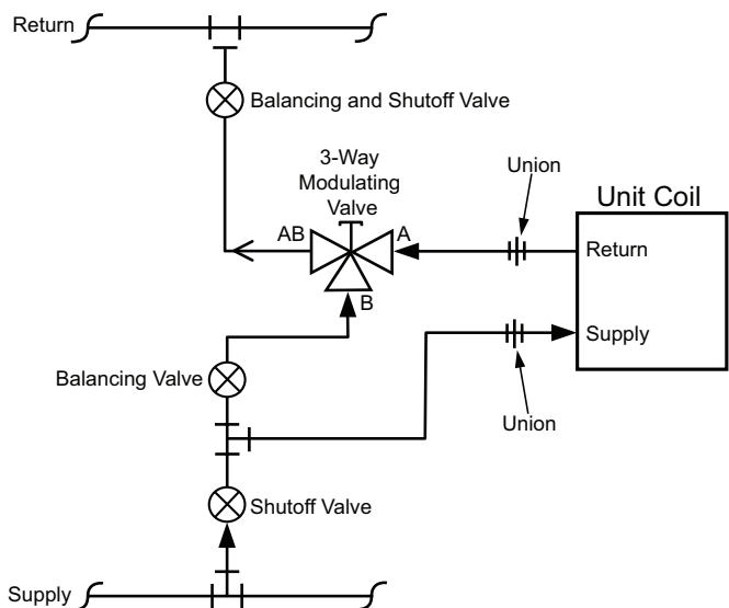
Figure 138: 3-Way Chilled Water Modulating Valve Piping
