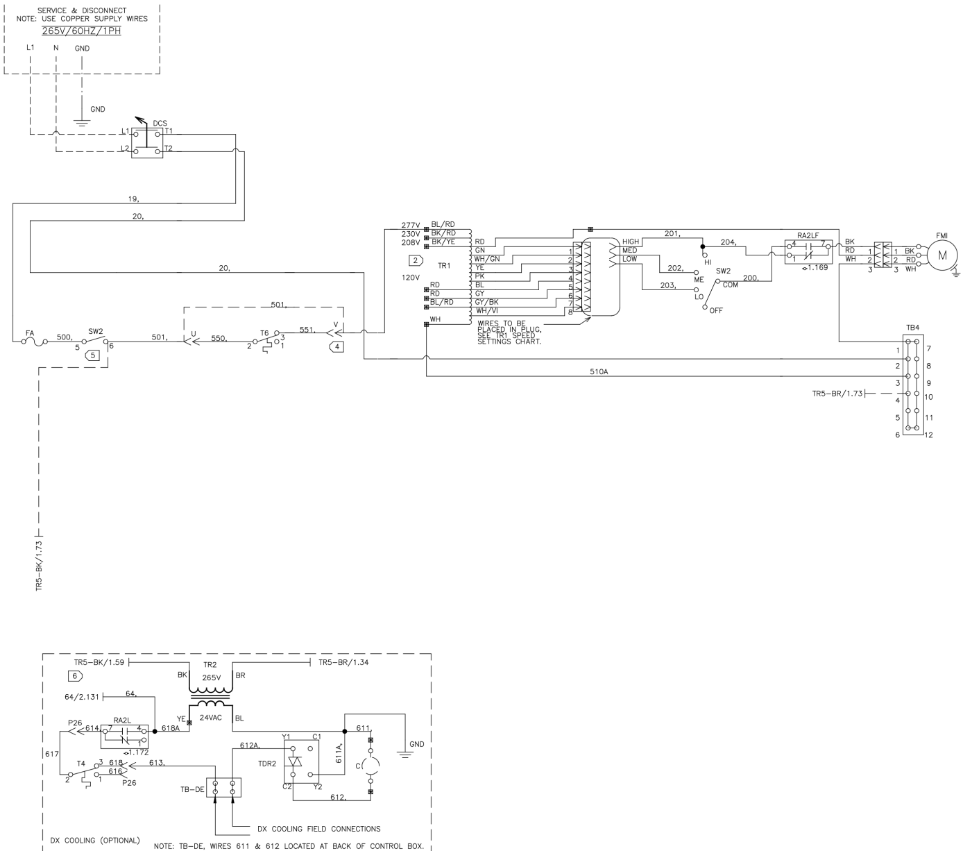
Figure 102: Controls by Others – Field Installed - 265 V/60 Hz/1 Ph
