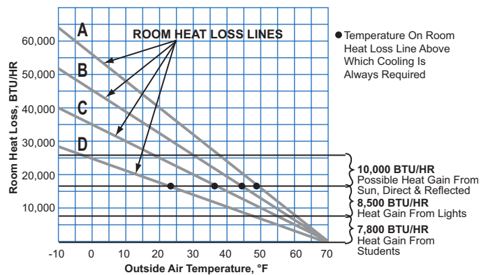
Figure 114: Heat Gain Vs. Heat Loss In Occupied Classrooms
