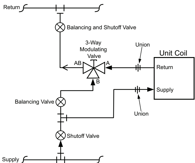
Figure 123: 3-Way Chilled Water Modulating Valve Piping
