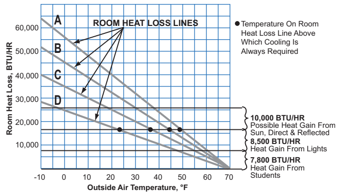
Figure 99: Heat Gain Vs. Heat Loss In Occupied Classrooms
