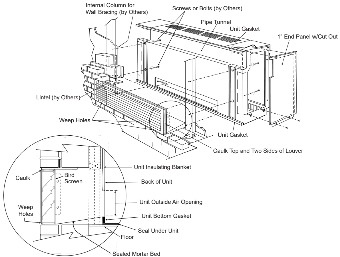
Figure 110: Recessed Wall Louver Installation Detail
