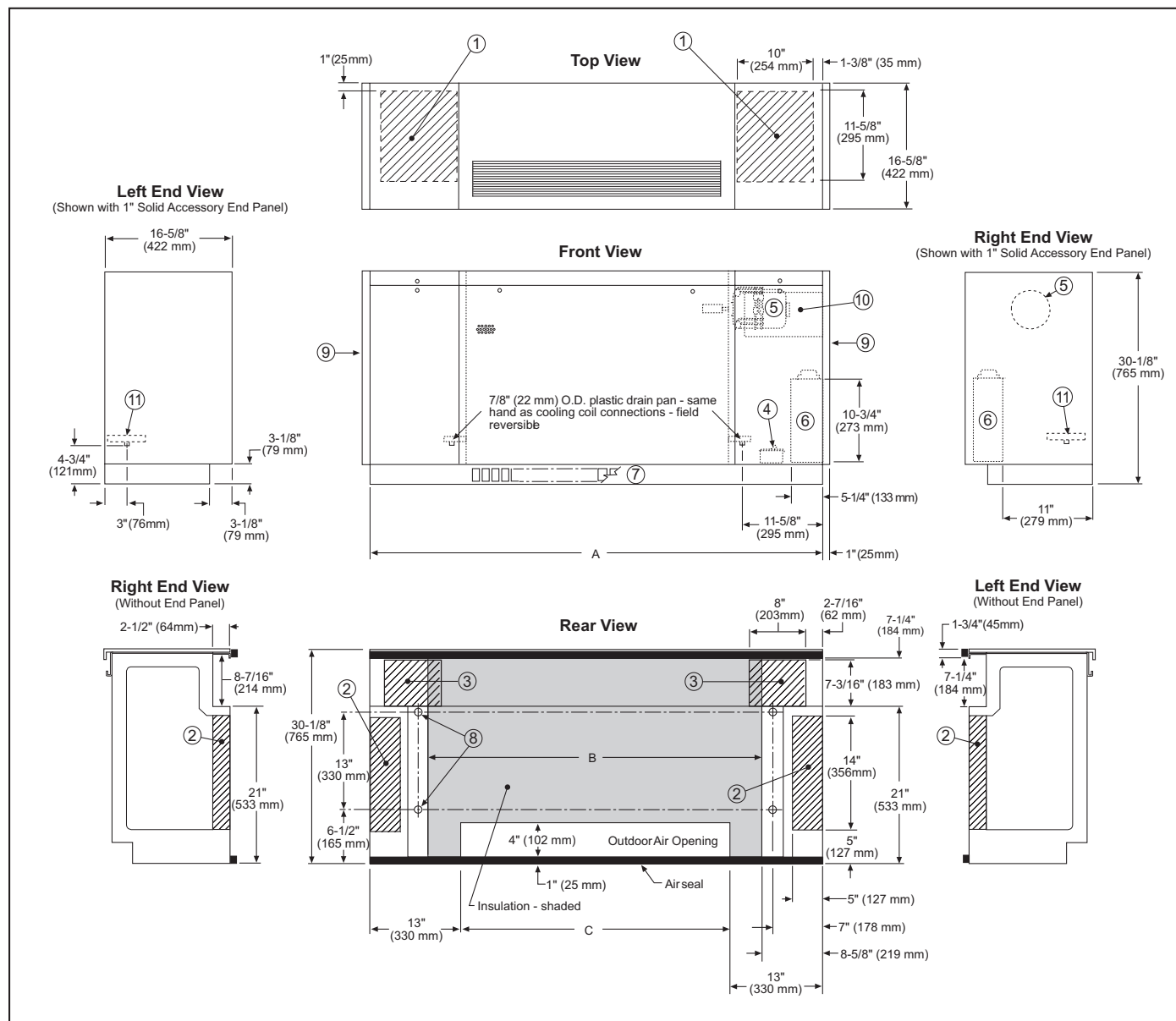
Figure 41: Arrangement AL with Open Pipe Tunnel, 16-5/8" Deep
