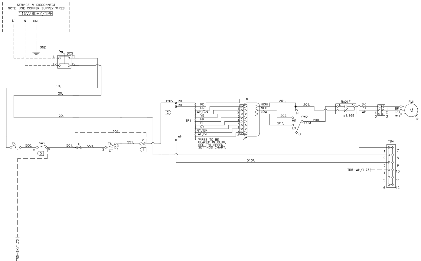
Figure 11: Controls by Others – Field Installed - 115 V/60 Hz/1 Ph
