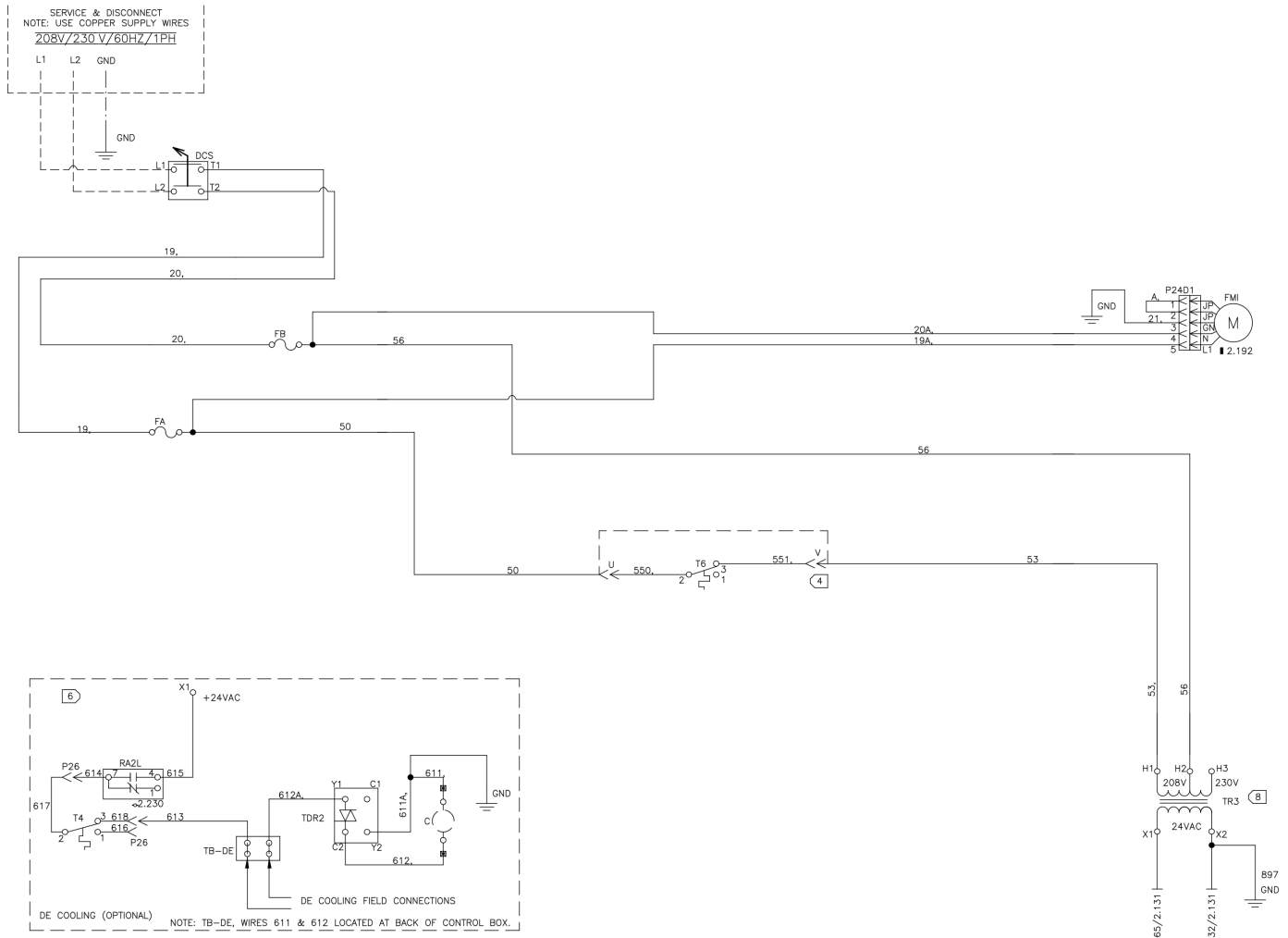
Figure 4: Variable Airflow 208-230V /60 Hz/1 Ph – Motor Switchbox, Non-Electric Heat Units
