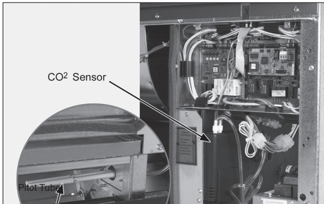
Figure 94: CO 2 Sensor for Demand Control Ventilation
