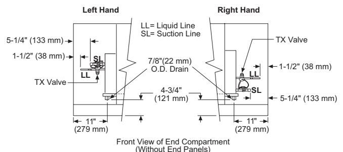
Figure 73: Condensate Drain and DX Coil Connections
