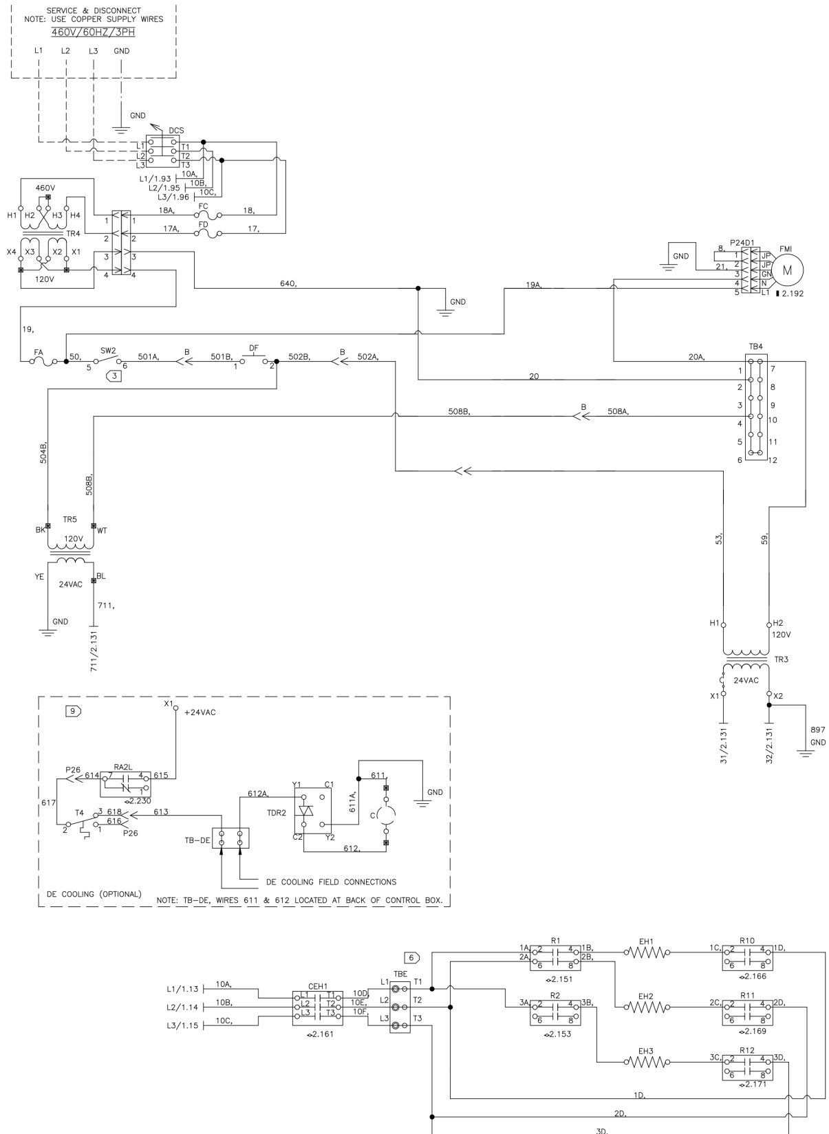
Figure 15: Electric Heat Wiring Diagram – Typical 460 V/60 Hz/3 Ph
