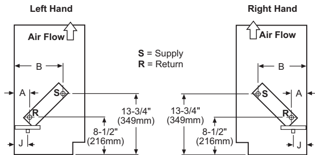
Figure 68: Steam Heating Only Unit (Coils 68, 69, 78, 79)
