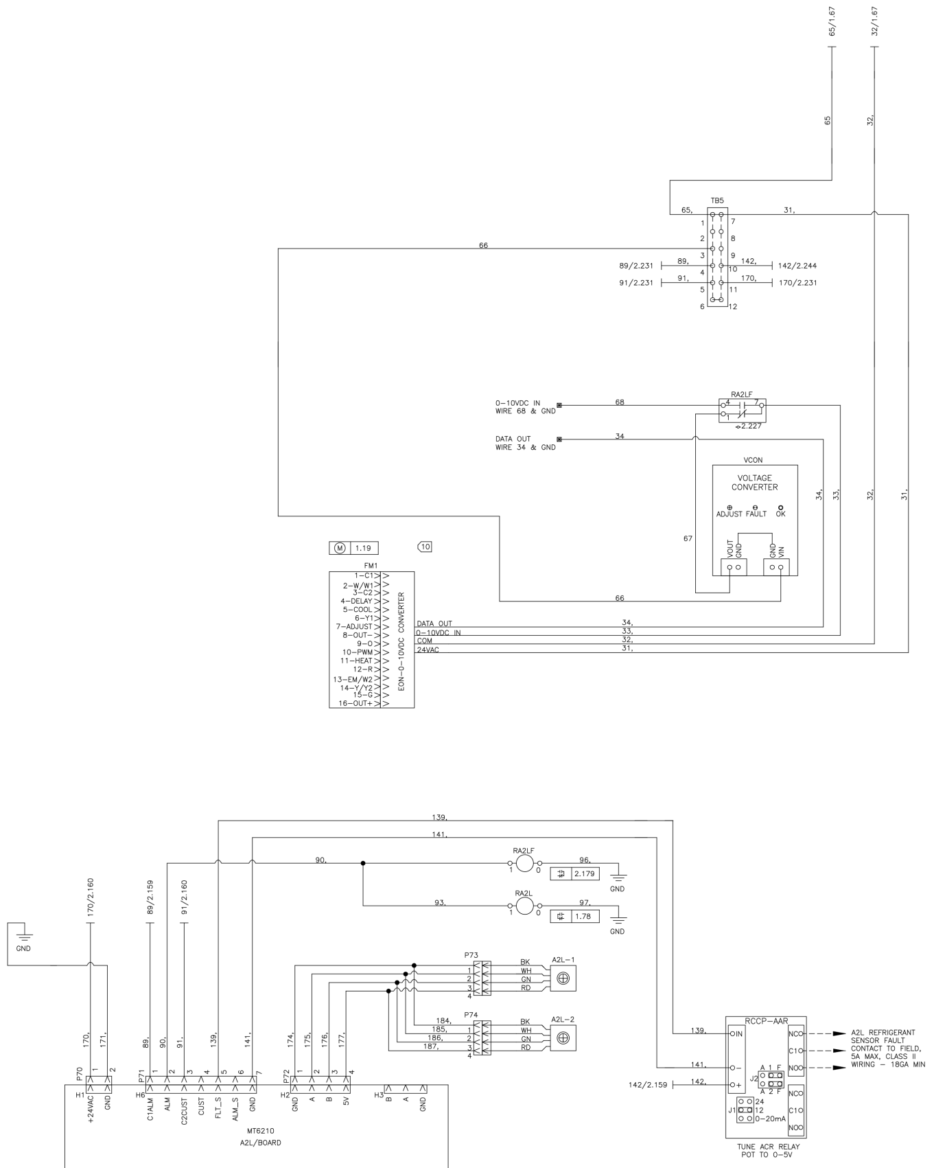
Figure 9: Variable Airflow 265 V/60 Hz/1 Ph – Motor Switchbox, Non-Electric Heat Units
