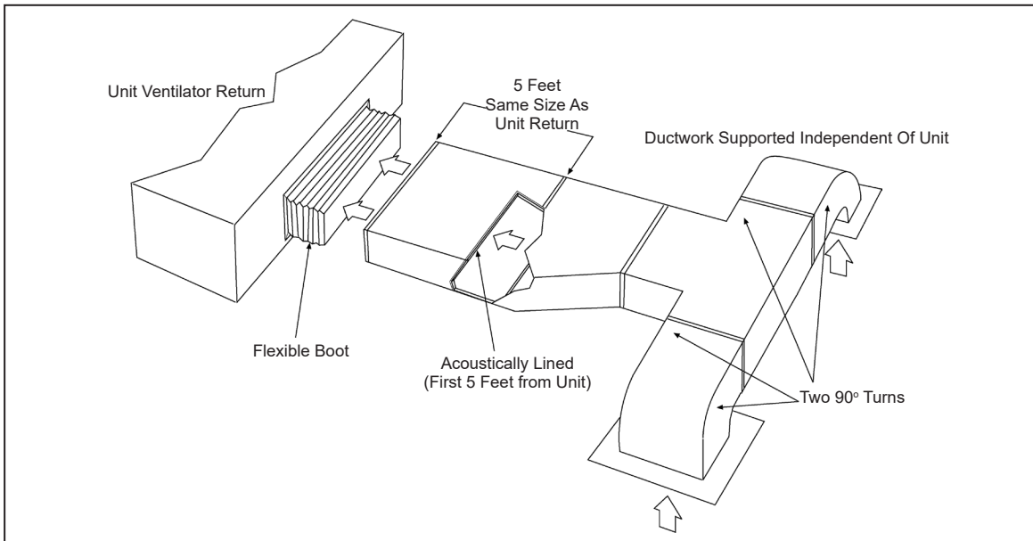
Figure 130: Suggested Return Air Ducting per ASHRAE and SMACNA Publications
