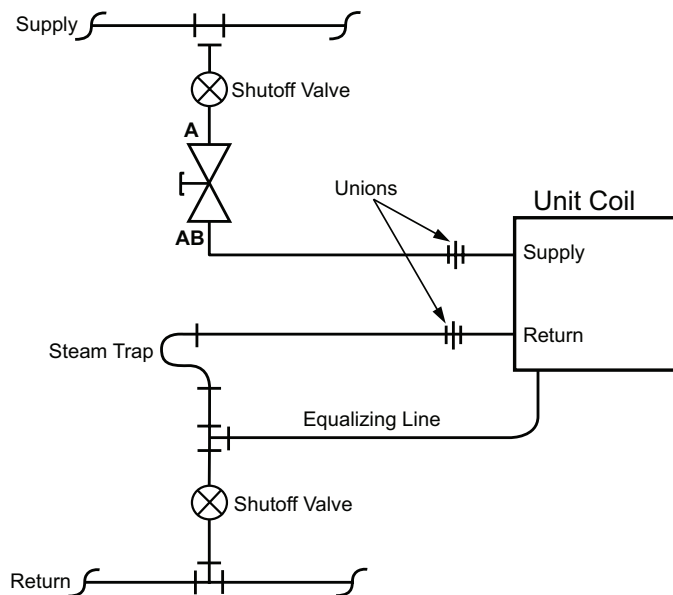
Figure 147: 2-Way Steam Modulating Valve Piping
