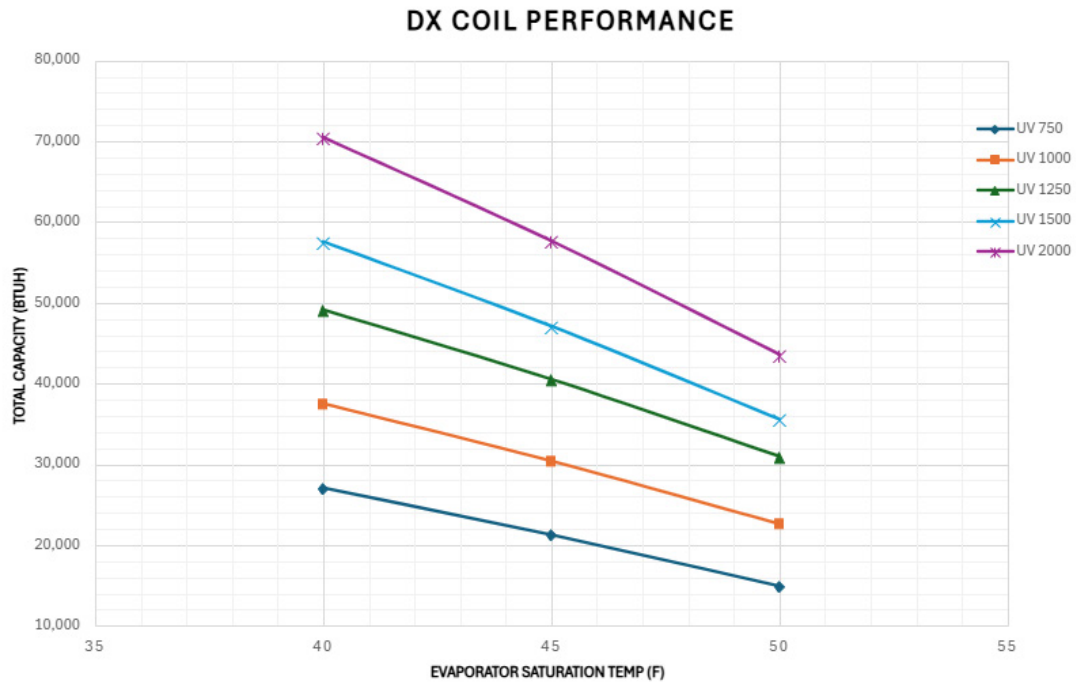
Figure 79: DX Coil Estimated Performance (Mbh at 115°F Liquid Temperature)
