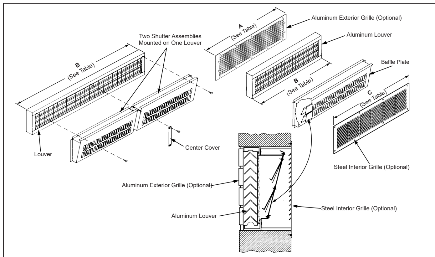
Figure 74: VentiMatic Shutter Assembly with Optional Grille
