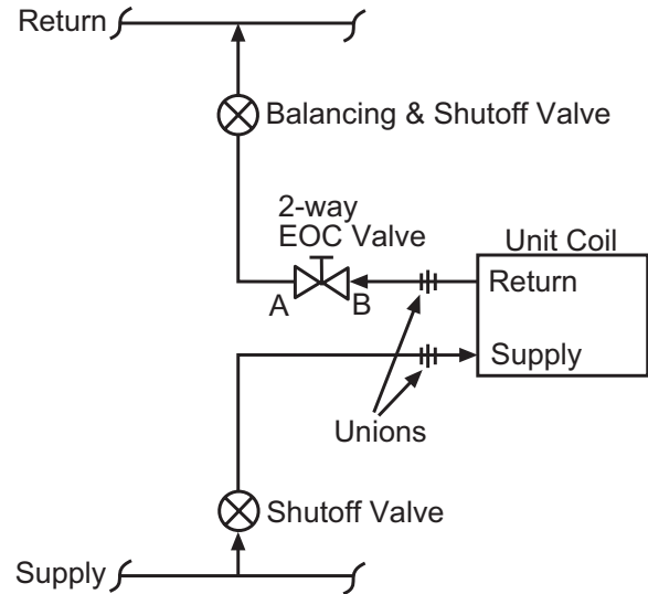
Figure 140: 2-Way Chilled Water EOC Valve Piping
