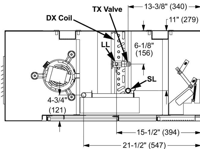
Figure 66: Direct Expansion Cooling Only Unit (Coil G[9], M[0])
