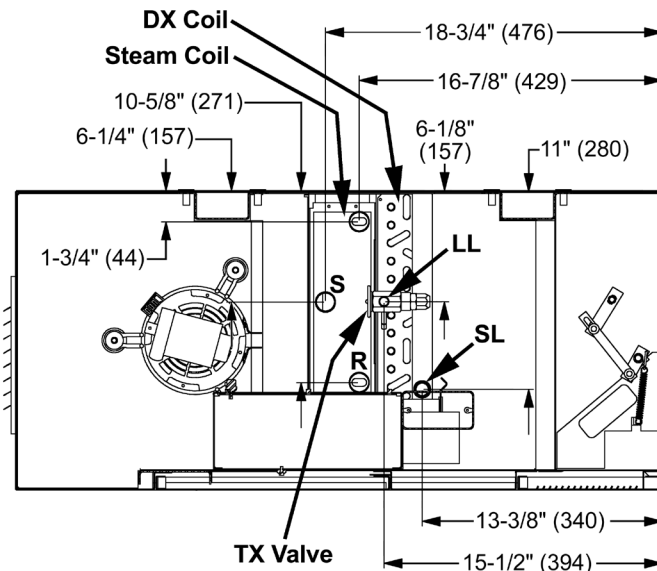
Figure 54: Direct Expansion (1st Position) and Steam Unit (Cooling Coil G[9], M[0], Heating Coils 68, 69)
