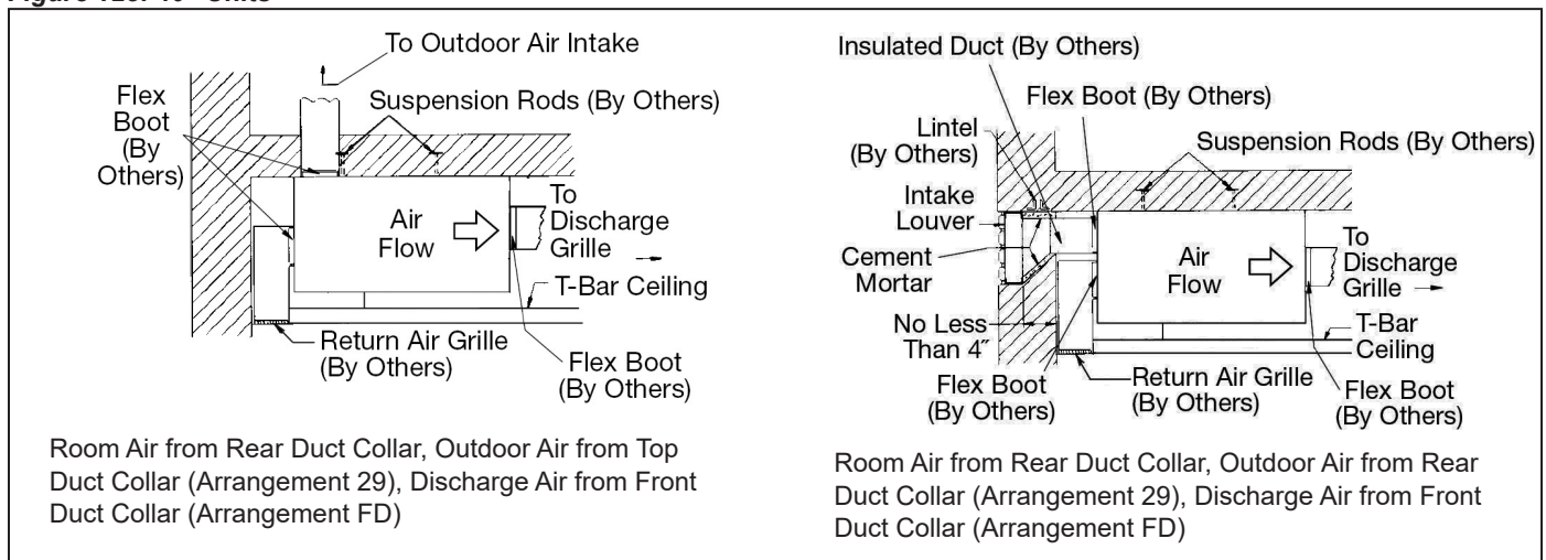
Figure 128: 40" Units
