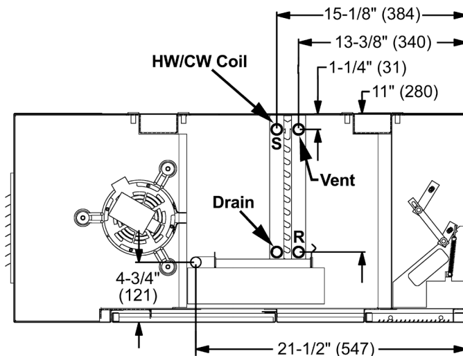
Figure 49: Chilled/Hot Water (2-pipe) Unit (Coils U[1], D[2], E[3], F[4])
