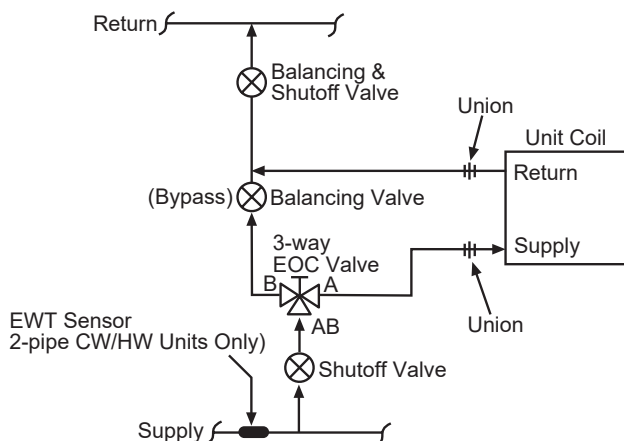
Figure 139: 3-Way Hot Water EOC Valve Piping
