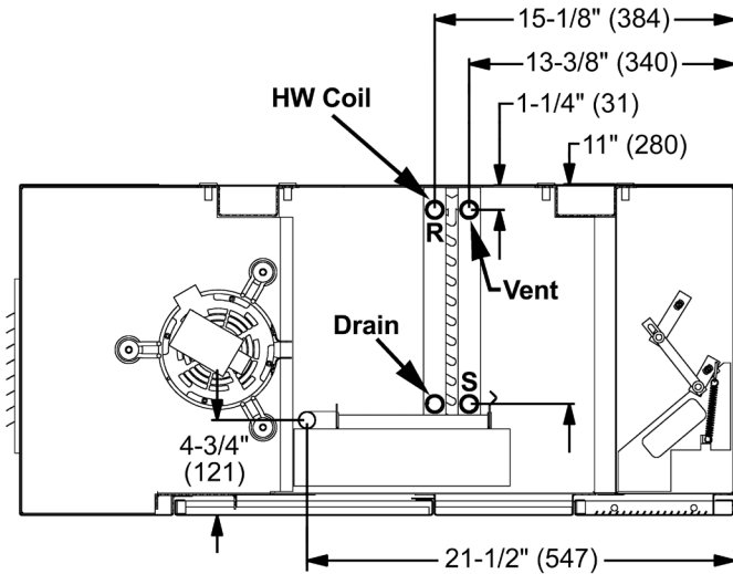
Figure 62: Hot Water Heating Only Unit (Coils 65, 66, 67)
