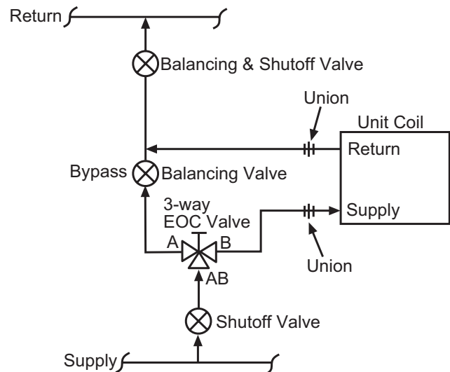
Figure 141: 3-Way Chilled Water EOC Valve Piping
