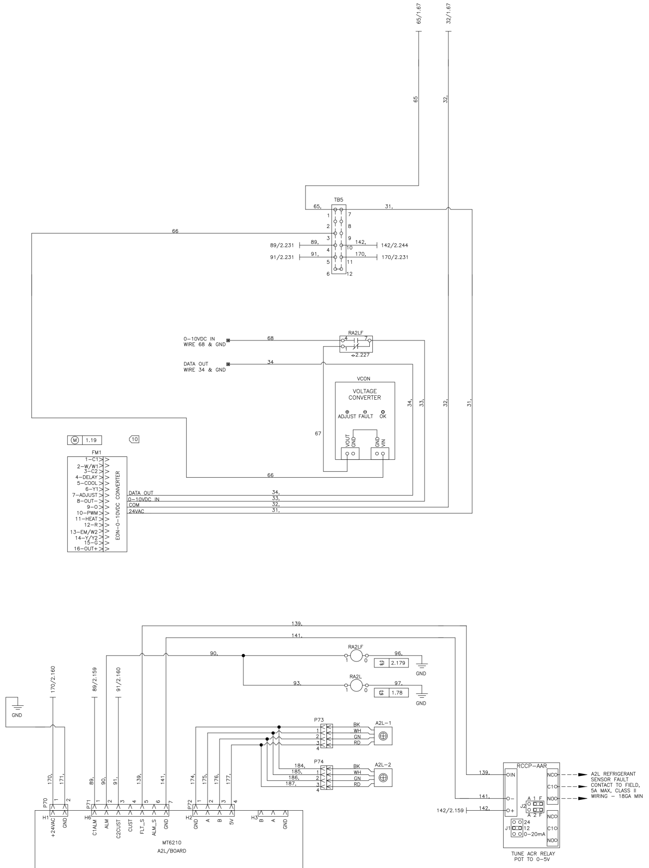
Figure 92: Variable Airflow 208-230V /60 Hz/1 Ph – Motor Switchbox, Non-Electric Heat Units
