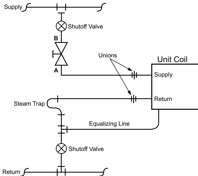
Figure 146: 2-Way Steam End of Cycle Valve Piping
