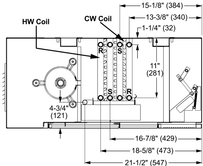
Figure 56: Chilled Water and Hot Water Unit (Cooling Coils V[5], S[6], W[7], Y[8]; Heating Coils 65, 66, 67)
