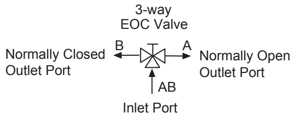
Figure 137: 3-Way Valve Piping Connections
