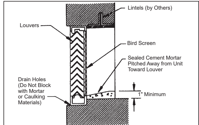
Figure 134: Flanged Wall Louver Installation Detail
