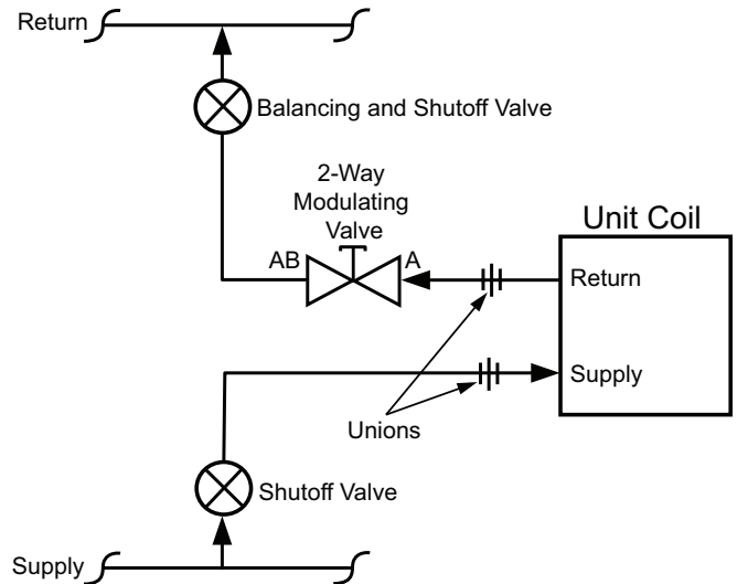
Figure 144: 2-Way Chilled Water Modulating Valve Piping
