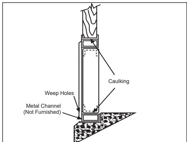
Figure 135: Panel Wall Louver Installation Detail
