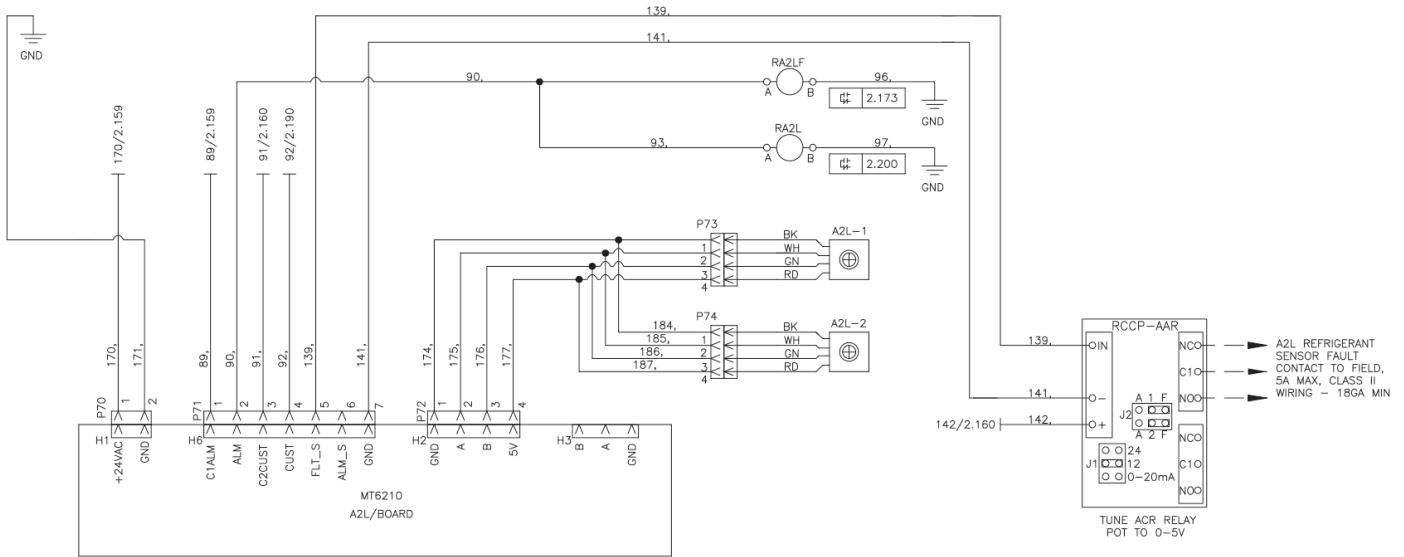
Figure 80: Electromechanical Controls – A2L Leak Mitigation
