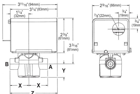
Figure 71: 2-Way EOC Steam Valve Dimensions
