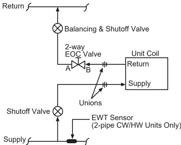
Figure 138: 2-Way Hot Water EOC Valve Piping
