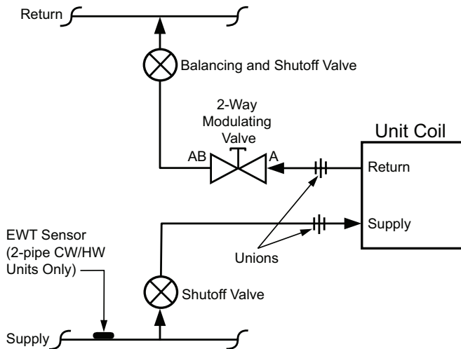
Figure 142: 2-Way Hot Water Modulating Valve Piping
