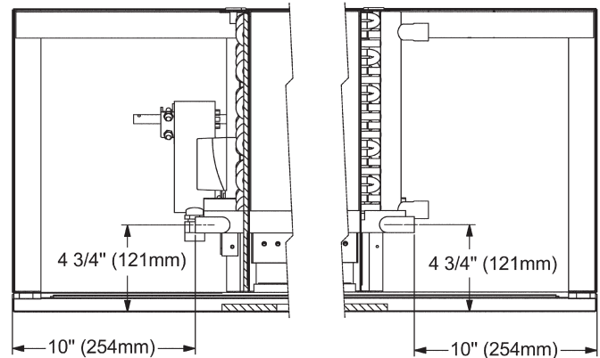
Figure 67: Condensate Drain
