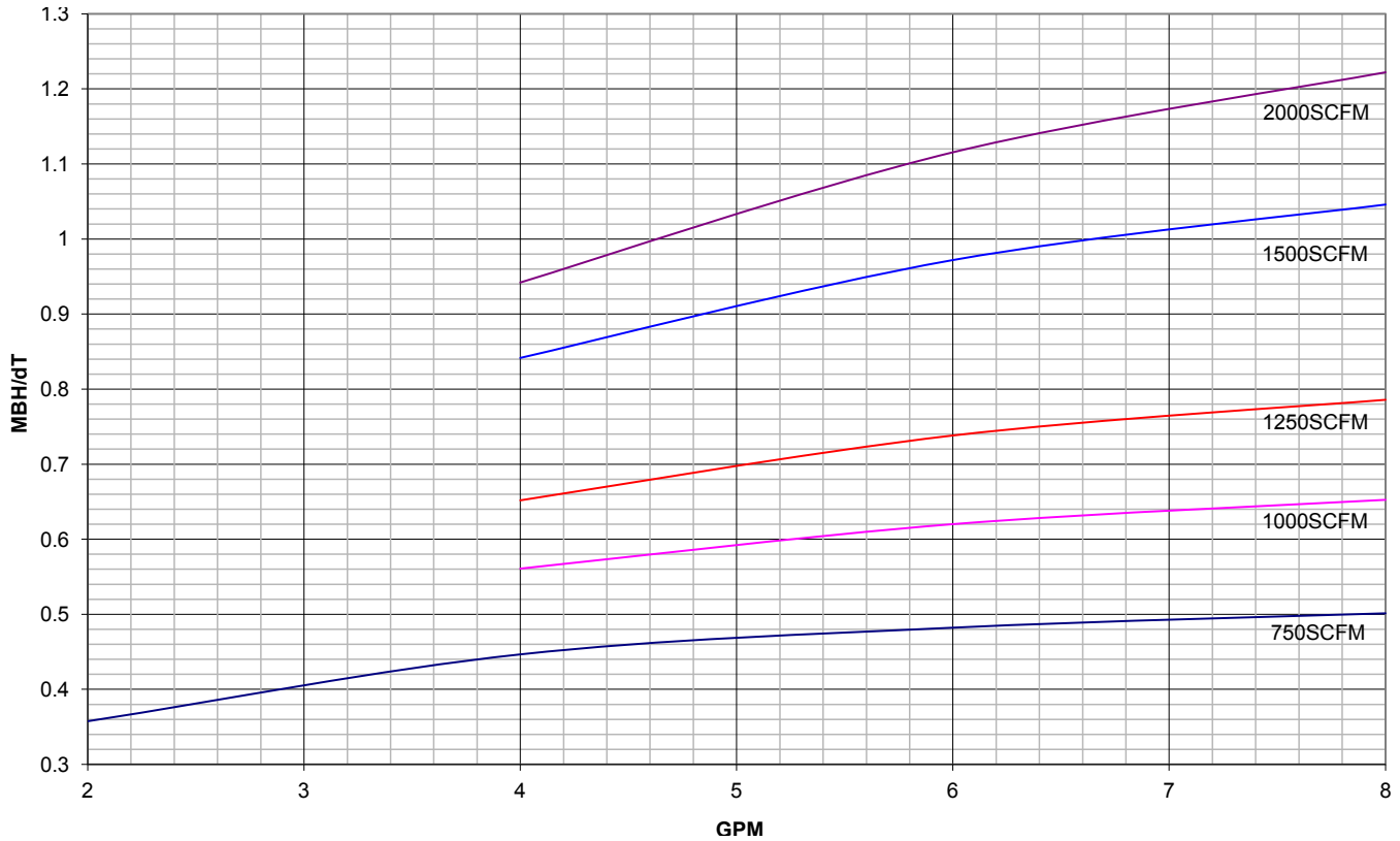
Figure 76: 2-Row Hot Water Coil (Parallel Flow)
