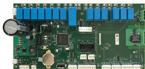
Figure 104: MicroTech Control Board
