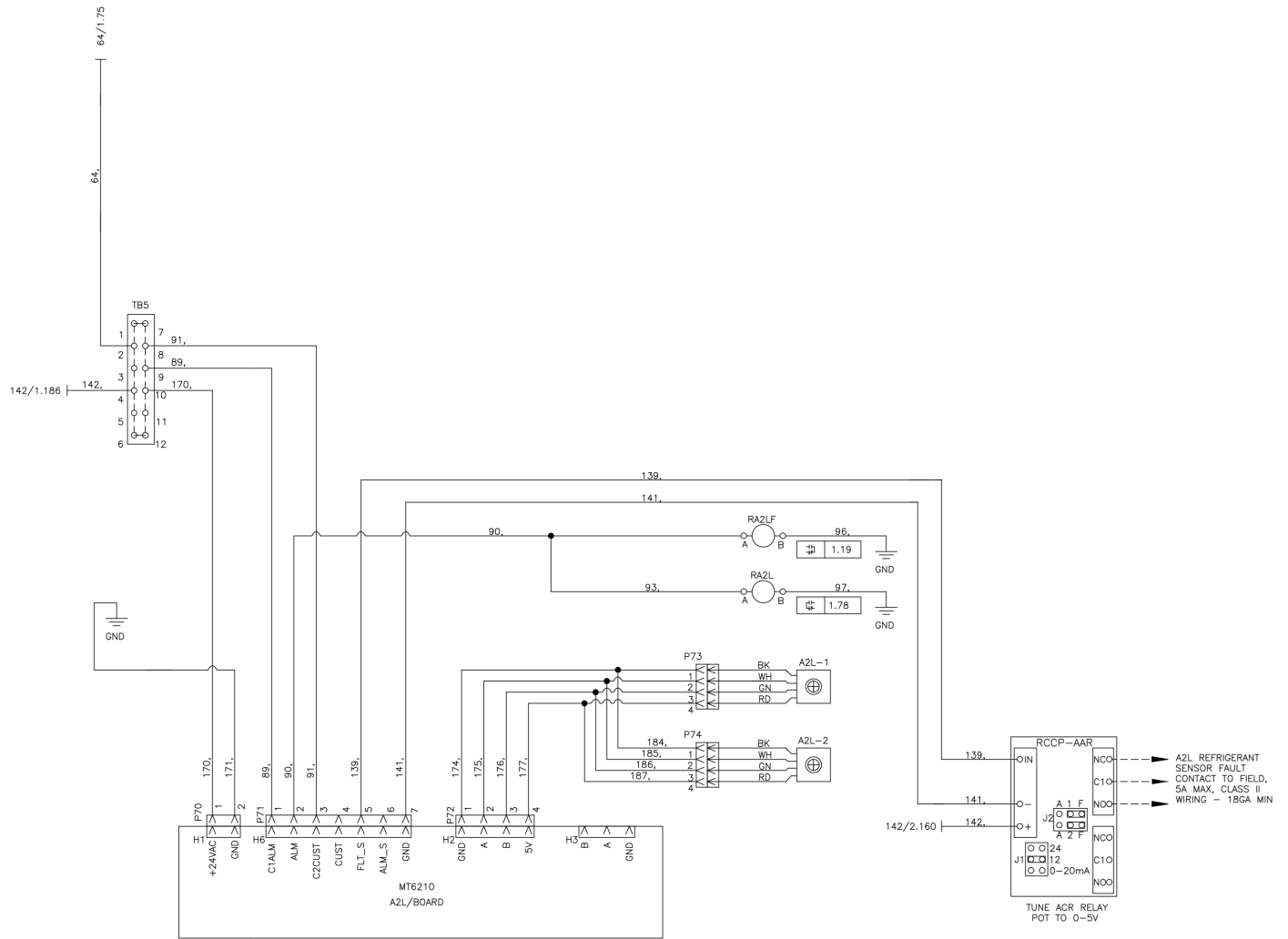
Figure 99: Controls by Others – Field Installed - 120 V/60 Hz/1 Ph
