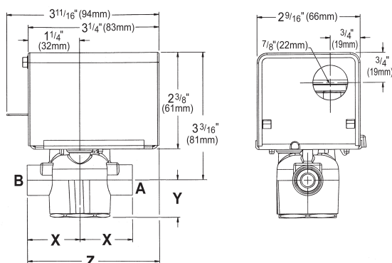
Figure 69: 2-Way EOC Valve Dimensions
