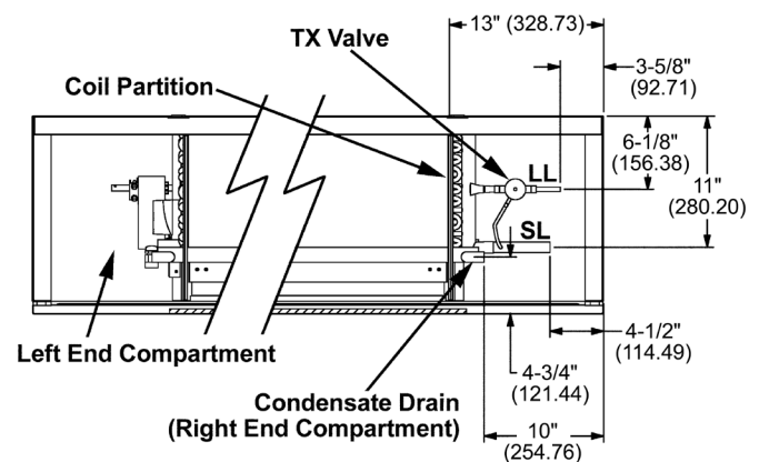
Figure 68: Condensate Drain and DX Coil Connections
