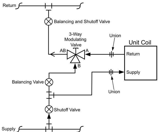
Figure 145: 3-Way Chilled Water Modulating Valve Piping
