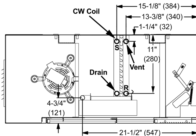
Figure 65: Chilled Water Cooling Only Unit (Coils V[5], S[6], W[7], Y[8])
