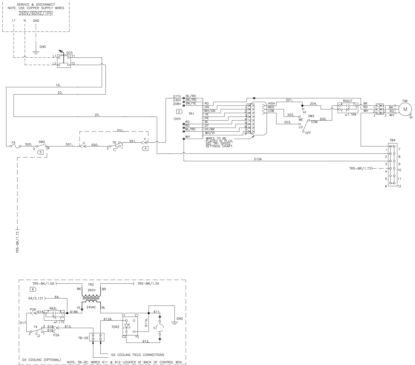
Figure 100: Controls by Others – Field Installed - 265 V/60 Hz/1 Ph
