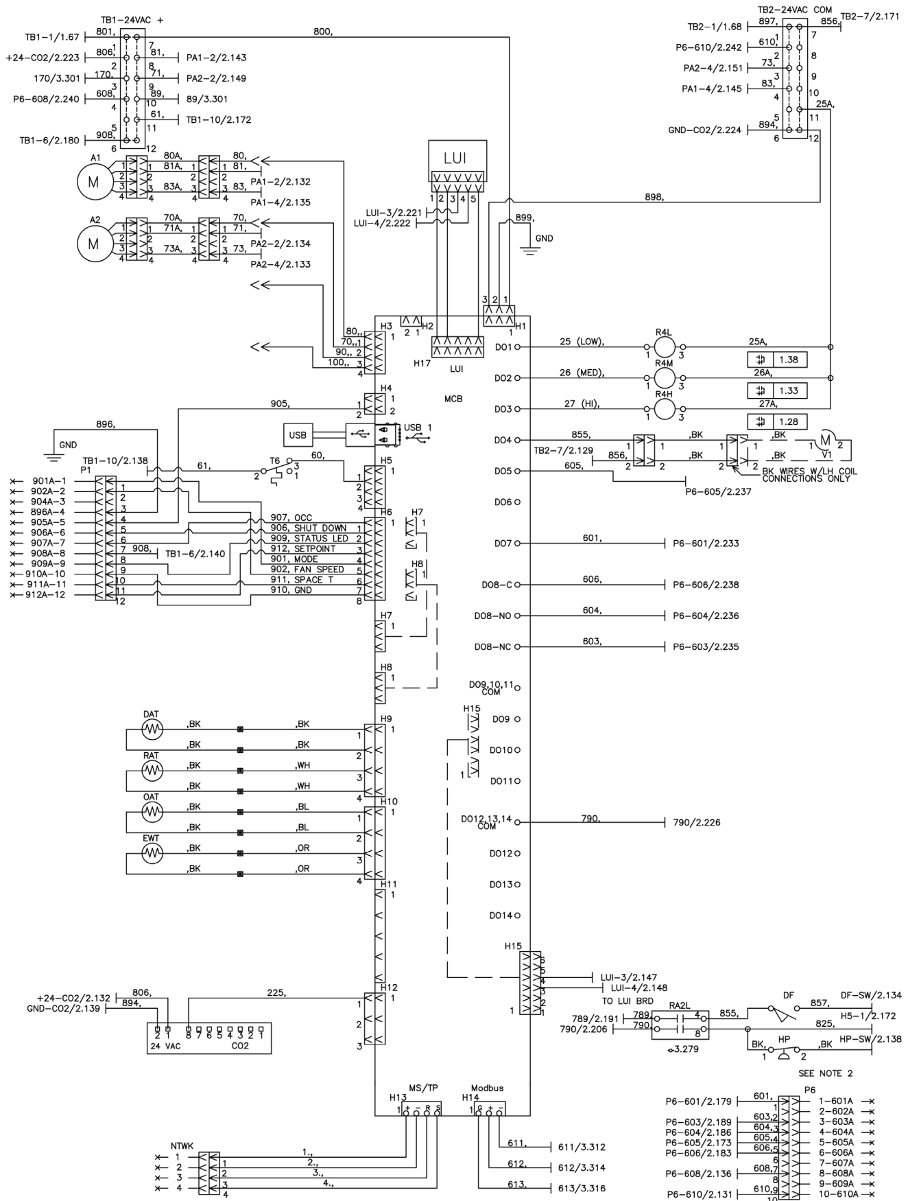
Figure 81: Typical MicroTech Wiring – 115 Volt/60 Hz /1 Ph
