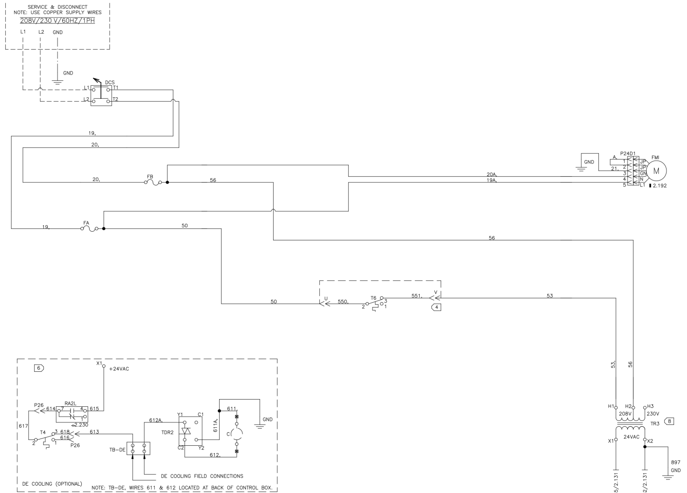
Figure 91: Variable Airflow 208-230V /60 Hz/1 Ph – Motor Switchbox, Non-Electric Heat Units
