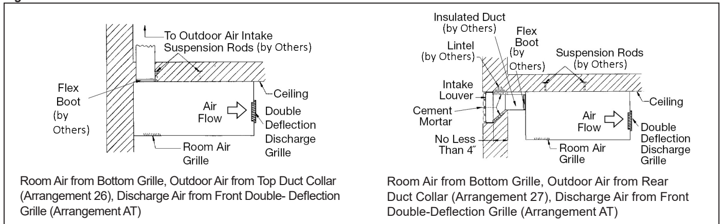
Figure 122: 40" Units
