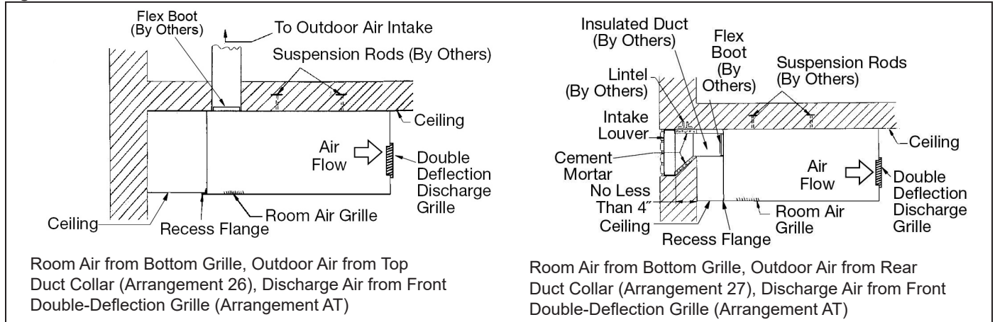
Figure 123: 36" Units
