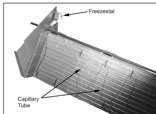
Figure 8: Freezestat
