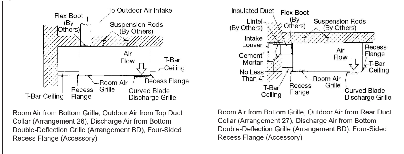
Figure 126: 40" Units
