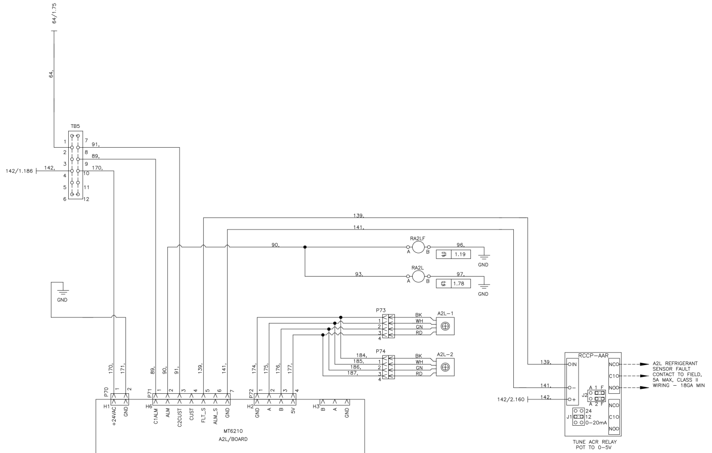
Figure 101: Controls by Others – Field Installed - 265 V/60 Hz/1 Ph
