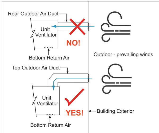
Figure 132: Outdoor Air Arrangement With Prevailing Winds
