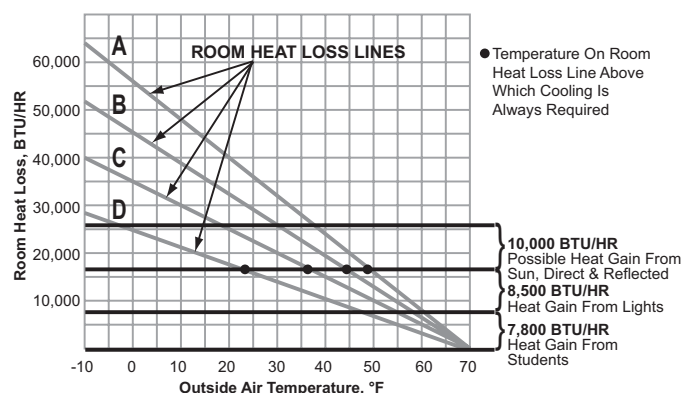
Figure 112: Heat Gain Vs. Heat Loss In Occupied Classrooms
