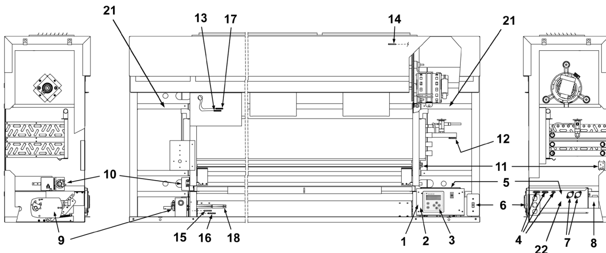
Figure 107: MicroTech Sensor and Component Locations
