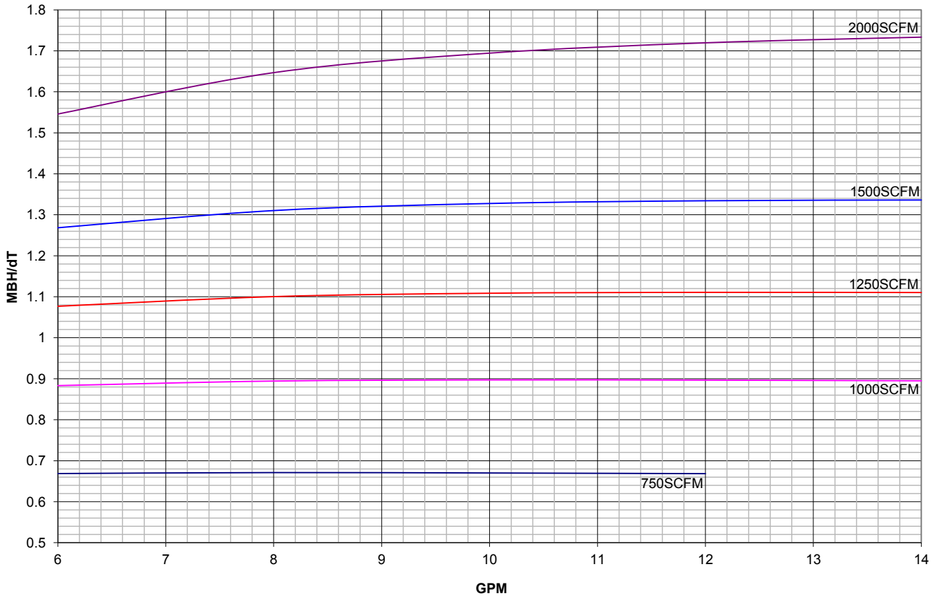
Figure 78: 4-Row, 2-Pipe Cold Water/Hot Water Coil (Counter Flow)
