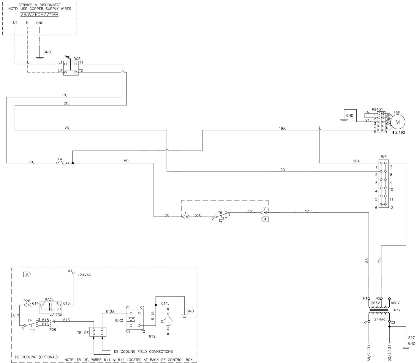
Figure 95: Variable Airflow 265 V/60 Hz/1 Ph – Motor Switchbox, Non-Electric Heat Units
