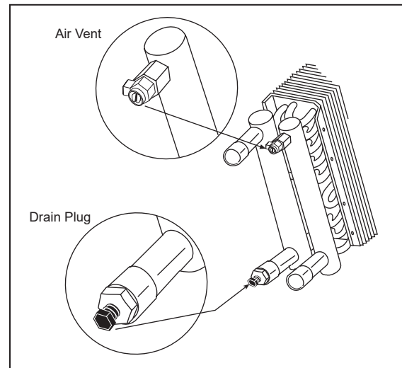
Figure 115: Manual Air Vent and Drain Plug
