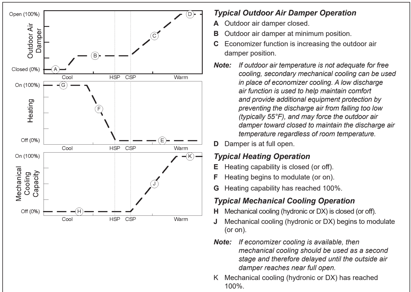
Figure 119: ASHRAE Cycle II Operation
