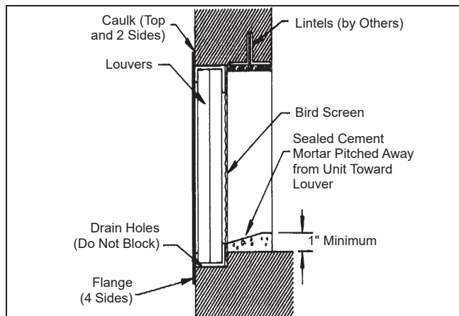
Figure 135: Panel Wall Louver Installation Detail
