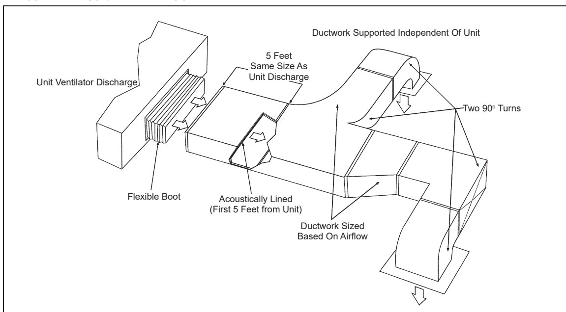
Figure 129: Suggested Supply Air Ducting per ASHRAE and SMACNA Publications
