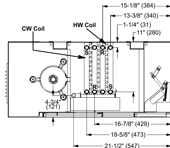
Figure 50: Chilled and Hot Water Unit (Cooling Coils V[5], S[6], W[7] Y[8]; Heating Coils 65, 66, 67)
