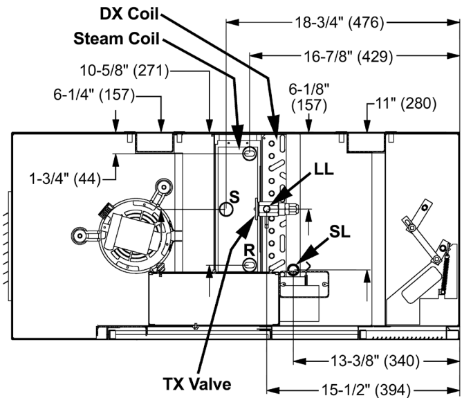
Figure 60: Direct Expansion and Steam Unit (Cooling Coil G[9], M[0], Heating Coils 68, 69)
