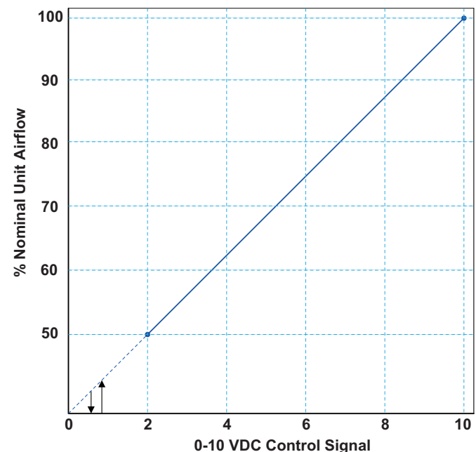
Figure 118: 0-10VDC Motor Operation
