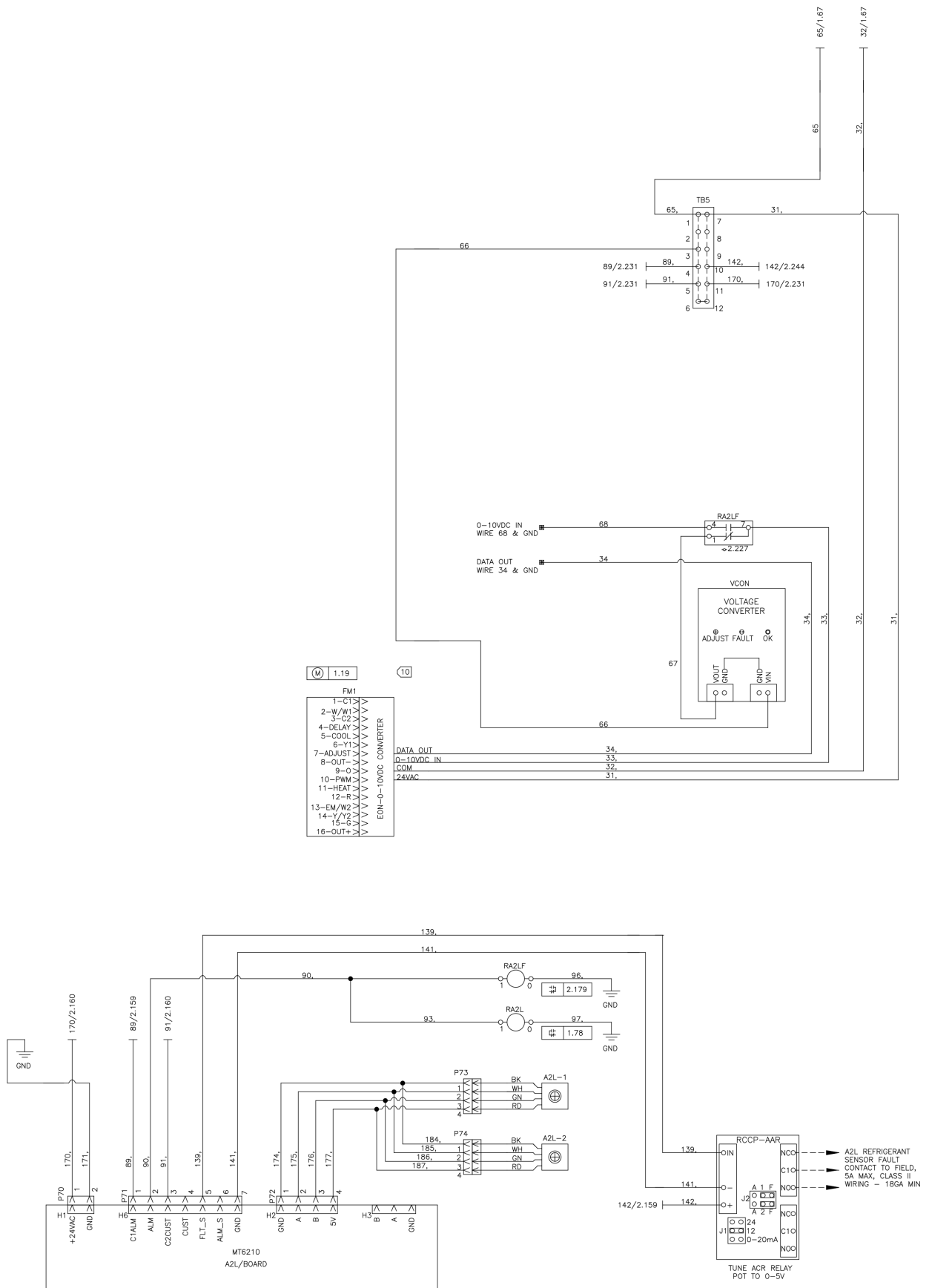
Figure 94: Variable Airflow 115 V/60 Hz/1 Ph – Motor Switchbox, Non-Electric Heat Units
