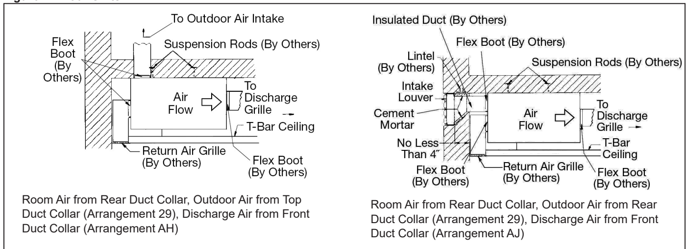
Figure 127: 36" Units
