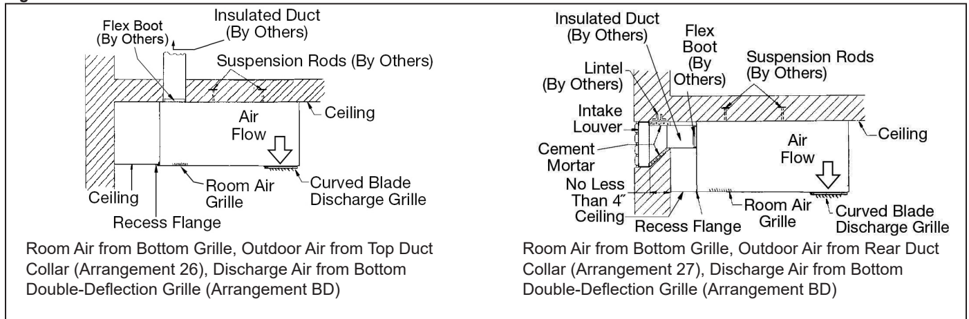
Figure 124: 40" Units
