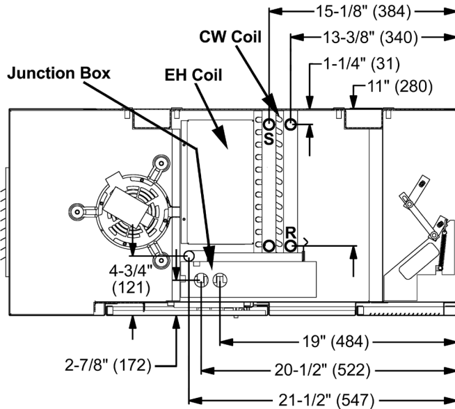
Figure 58: Chilled Water (1st Position) and Electric Heating (Cooling Coils V[5], S[6], W[7]; Heating Coil 12, 13)
