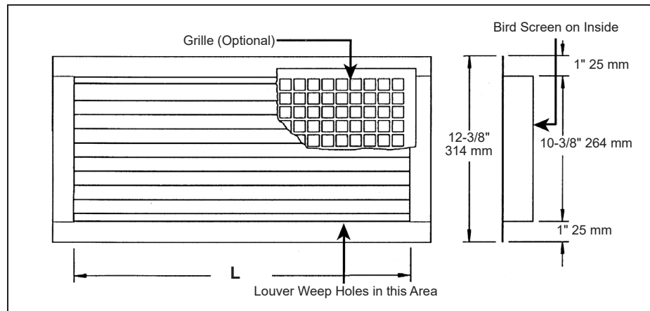
Figure 72: Louver with Flange (Horizontal Blades Shown)
