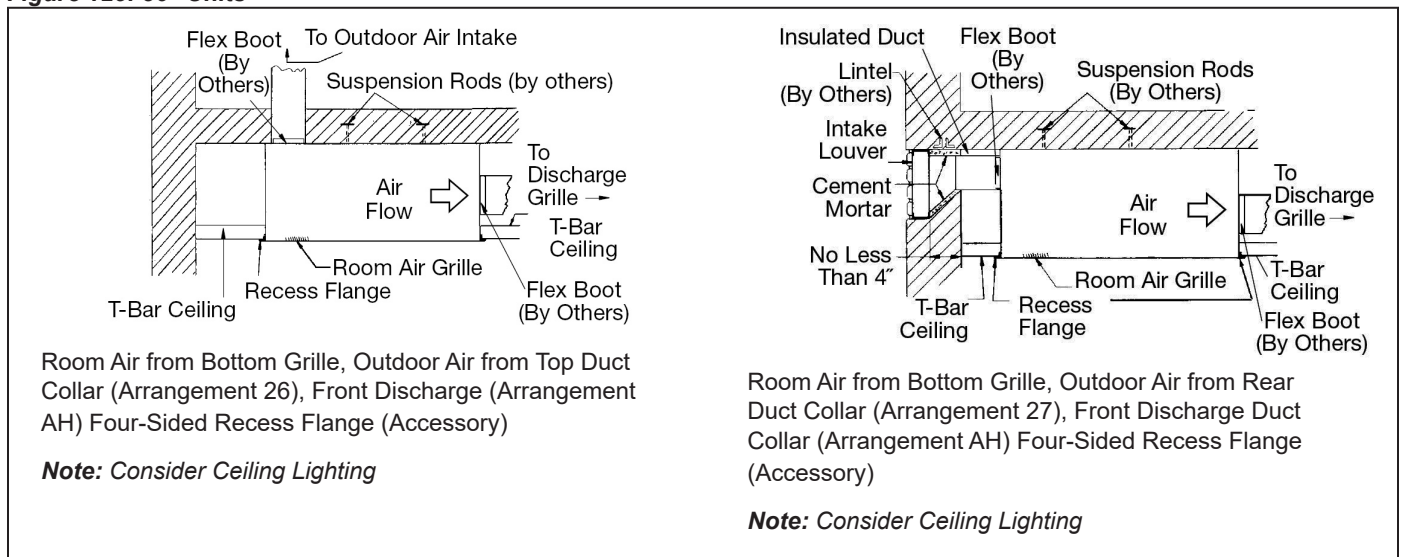
Figure 125: 36" Units
