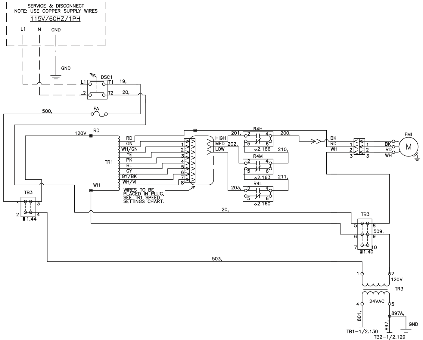
Figure 82: Typical MicroTech Wiring Diagram – Service and Disconnect, 115 Volt/60 Hz/1 Ph
