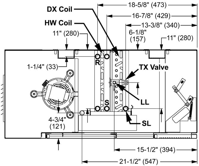
Figure 59: Direct Expansion and Hot Water Unit (Cooling Coil G[9], M[0], Heating Coils 65, 66, 67)
