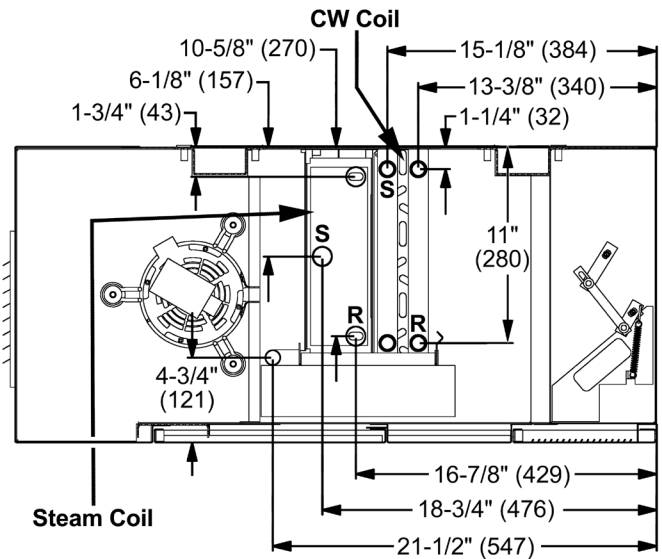
Figure 51: Chilled Water and Steam Unit (Cooling Coils V[5], S[6]; Heating Coils 68, 69)
