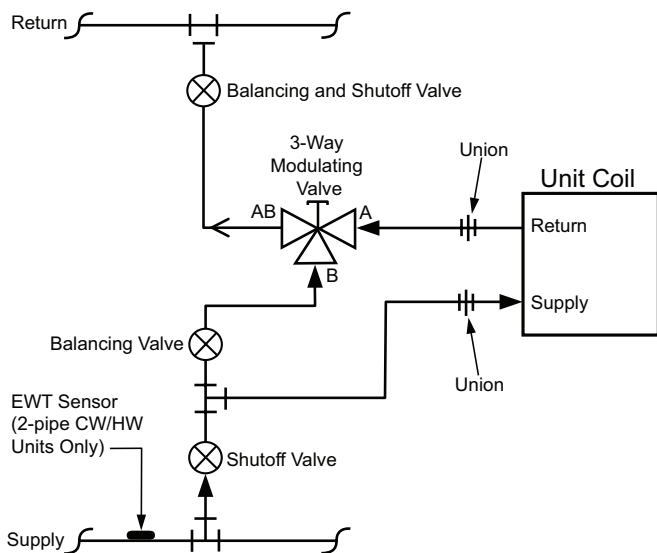
Figure 143: 3-Way Hot Water Modulating Valve Piping
