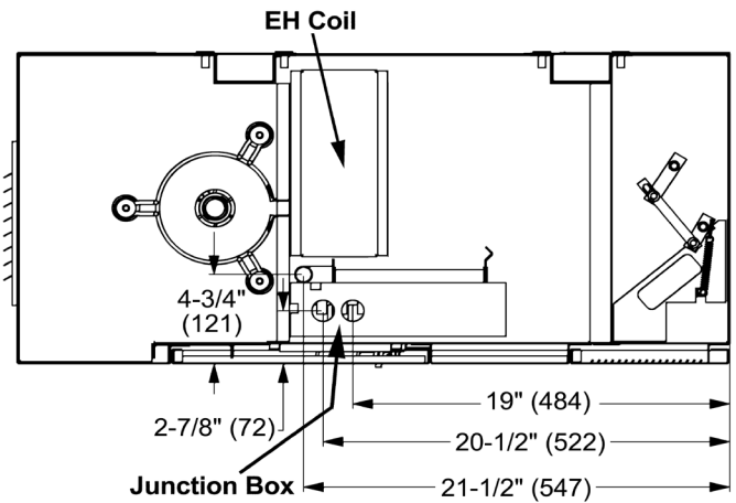
Figure 64: Electric Heating Only Unit (Coils 12, 13)
