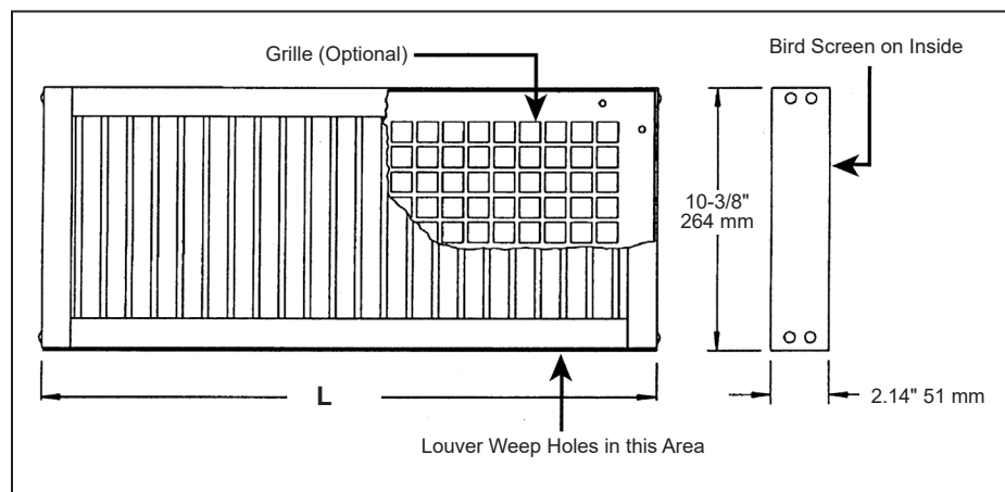
Figure 73: Louver without Flange (Vertical Blades Shown)
