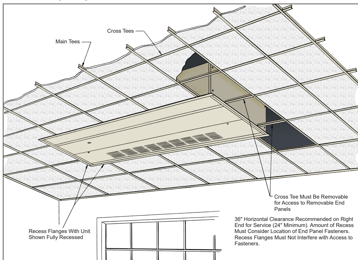
Figure 120: Accessibility to Fully Recessed Units
