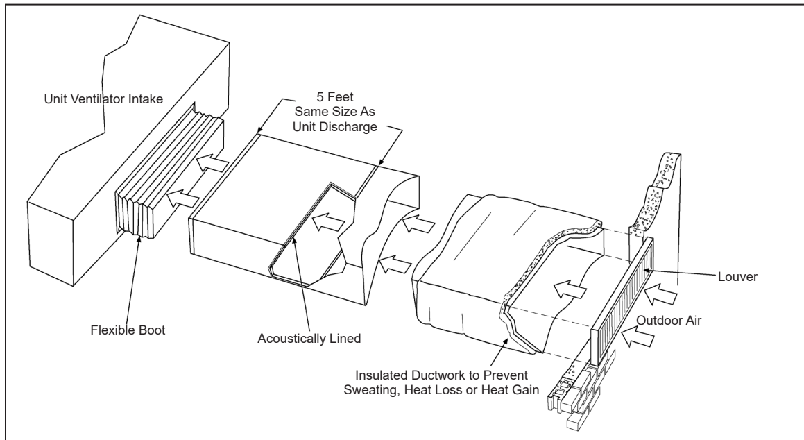
Figure 131: Suggested Outdoor Air Ducting (Insulated) per ASHRAE and SMACNA Publications
