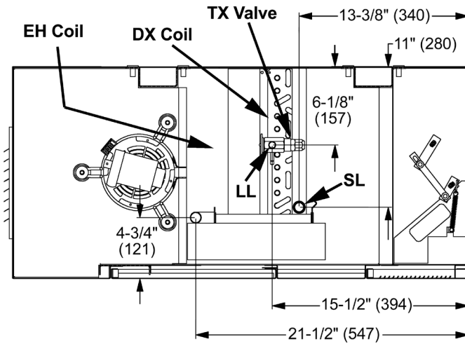
Figure 61: Direct Expansion and Electric Heating Unit (Cooling Coil G[9], M[0], Heating Coils 12, 13)
