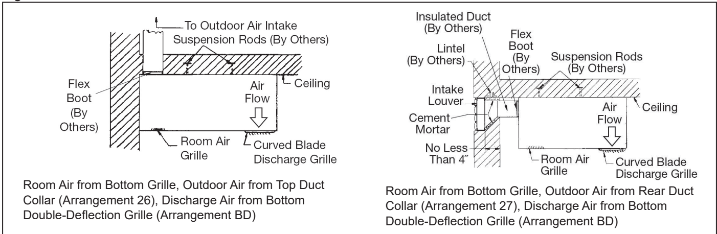
Figure 122: 40" Units
