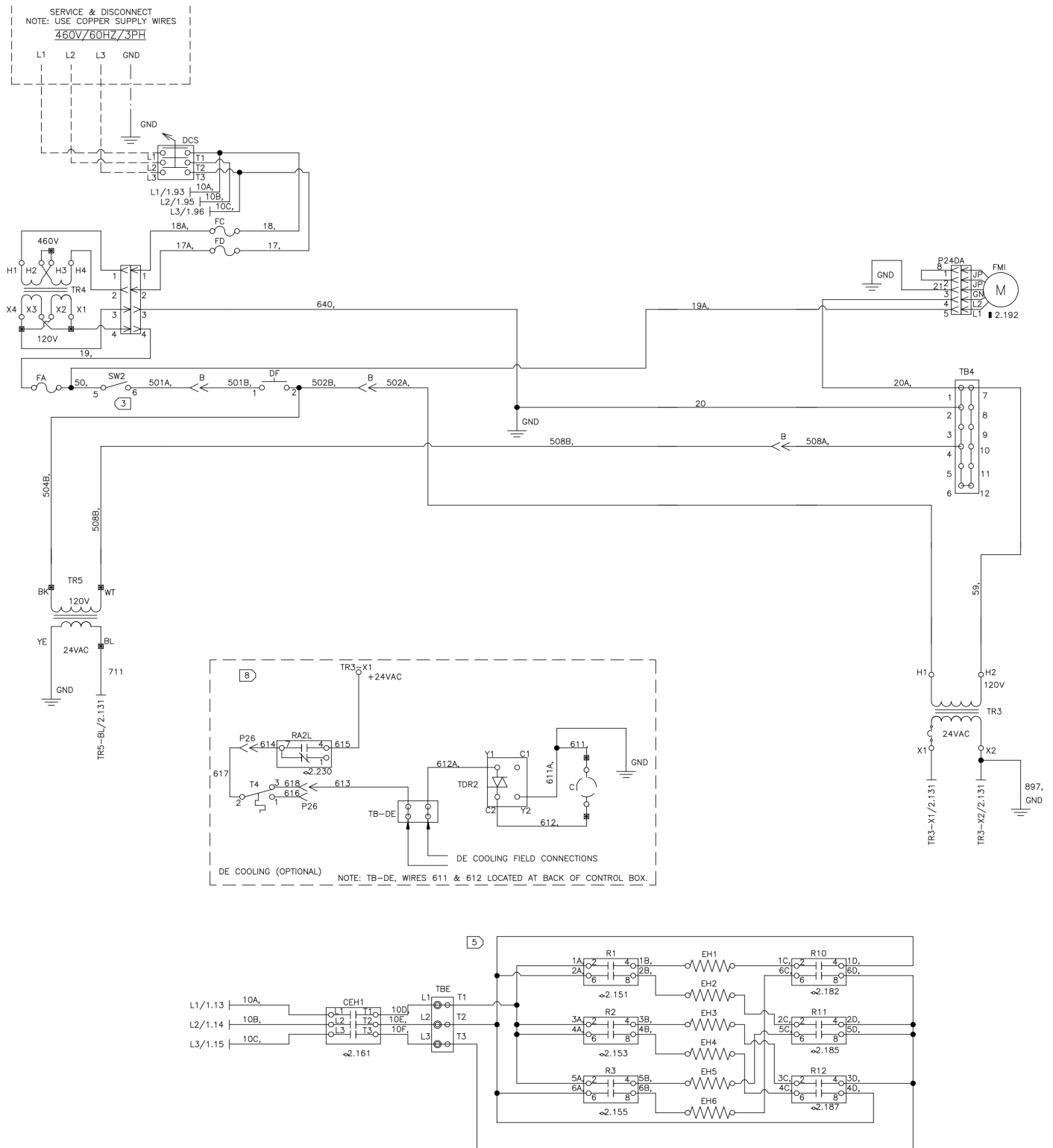
Figure 102: Electric Heat Wiring Diagram – Typical 460 V/60 Hz/3 Ph
