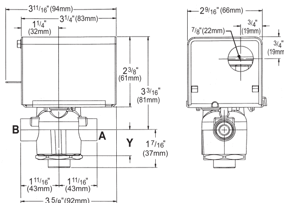
Figure 70: 3-Way EOC Valve Dimensions
