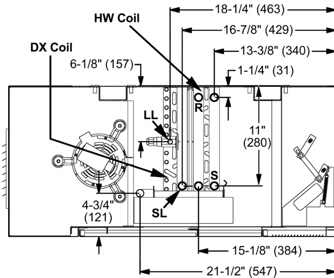
Figure 53: Direct Expansion and Hot Water Unit (Cooling Coil G[9], M[0], Heating Coils 65, 66, 67)
