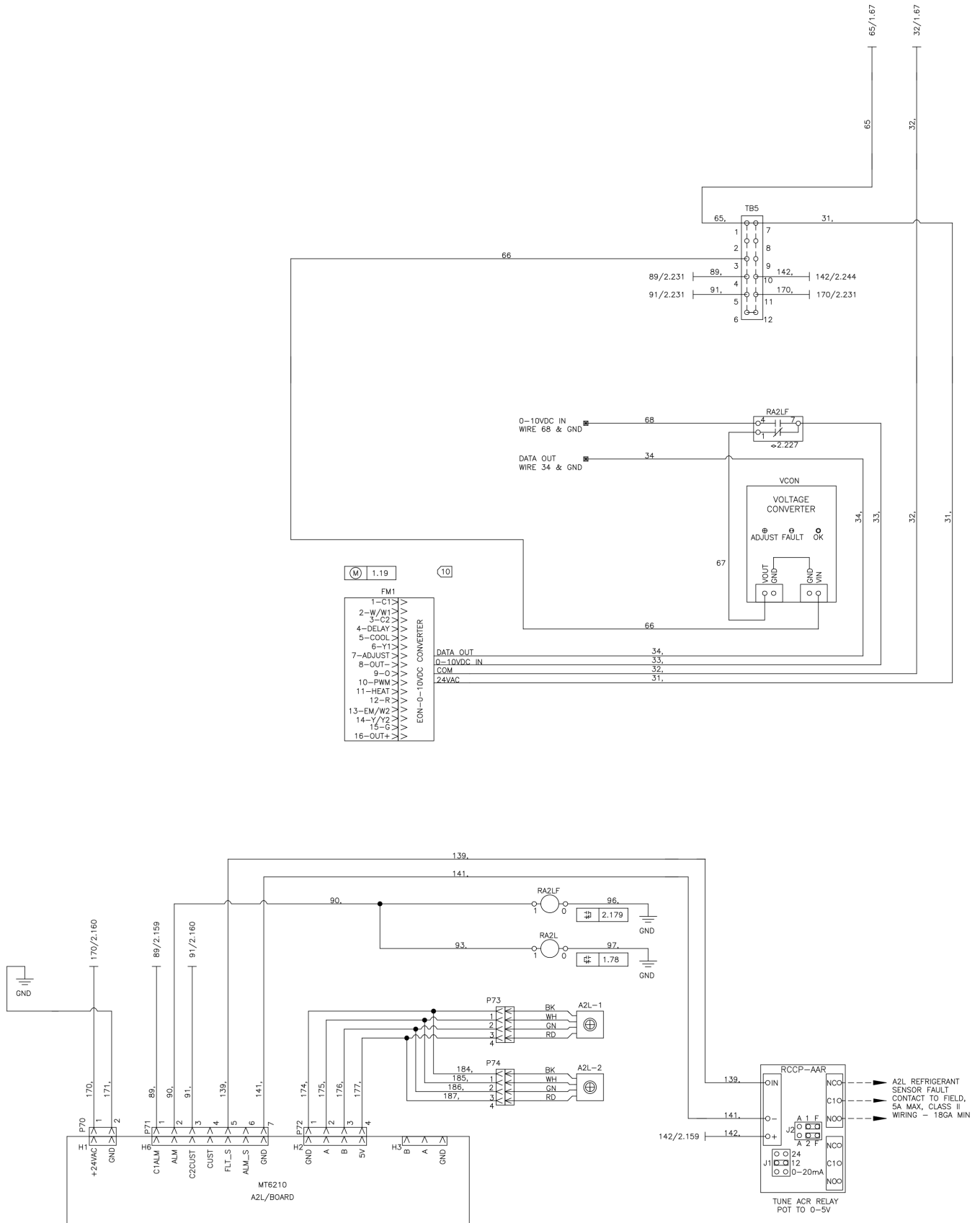
Figure 96: Variable Airflow 265 V/60 Hz/1 Ph – Motor Switchbox, Non-Electric Heat Units
