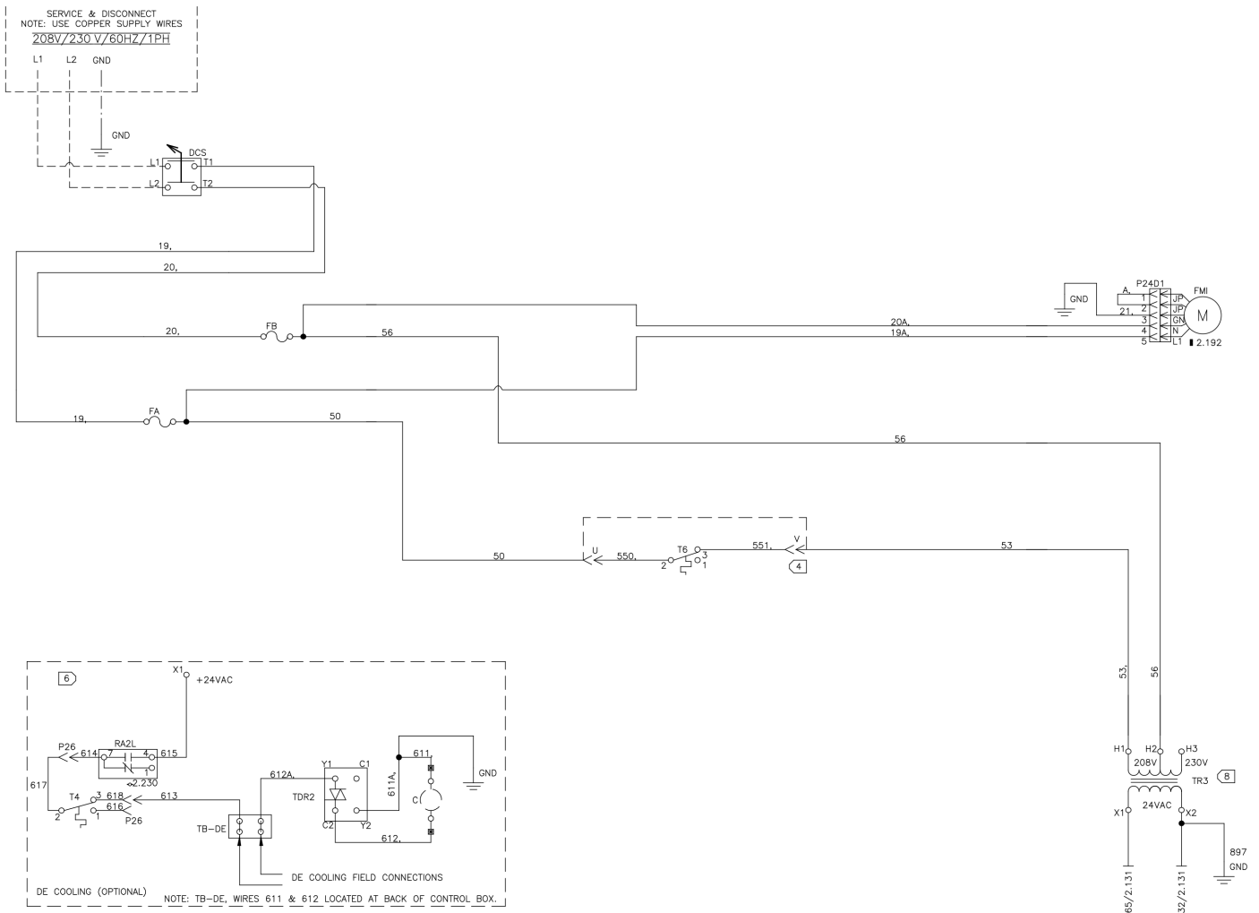
Figure 7: Variable Airflow 208-230V /60 Hz/1 Ph – Motor Switchbox, Non-Electric Heat Units
