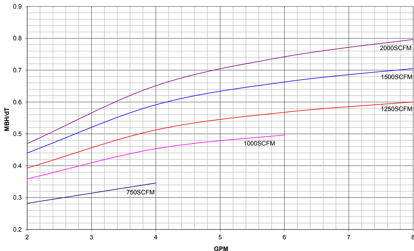
Figure 78: 1-Row Hot Water Coil
