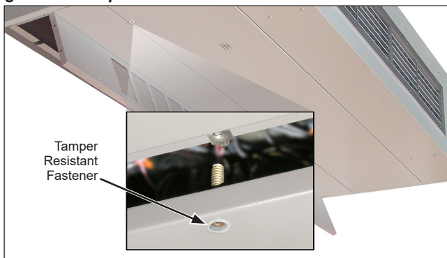
Figure 19: Tamper-Resistant Fastener
