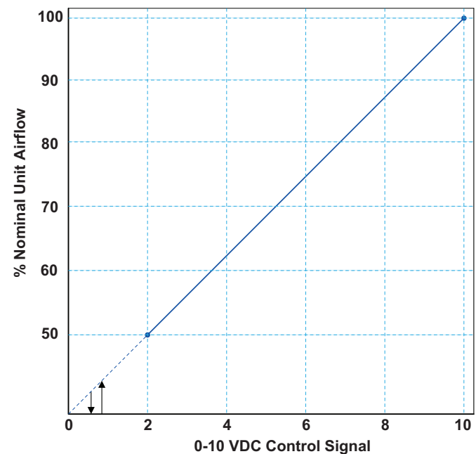
Figure 102: 0-10VDC Motor Operation
