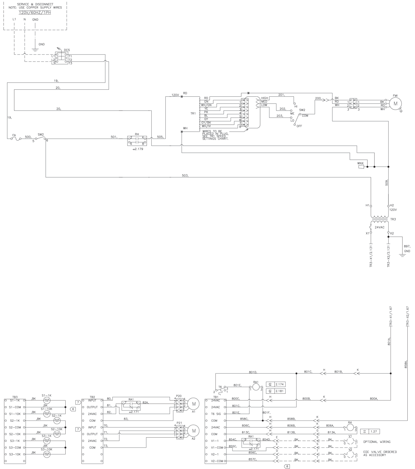
Figure 5: Digital Ready Face and Bypass Control - 120 V/60 Hz/1 Ph
