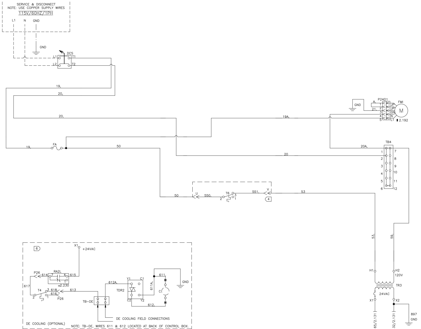
Figure 9: Variable Airflow 115 V/60 Hz/1 Ph – Motor Switchbox, Non-Electric Heat Units
