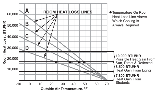
Figure 70: Heat Gain Vs. Heat Loss In Occupied Classrooms
