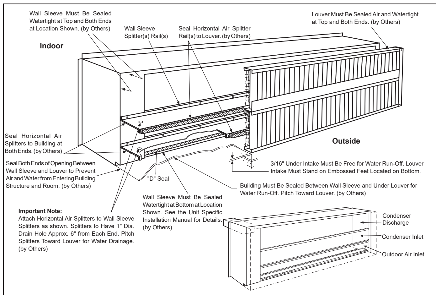
Figure 84: Recessed Wall Sleeve with Horizontal Air Splitters
