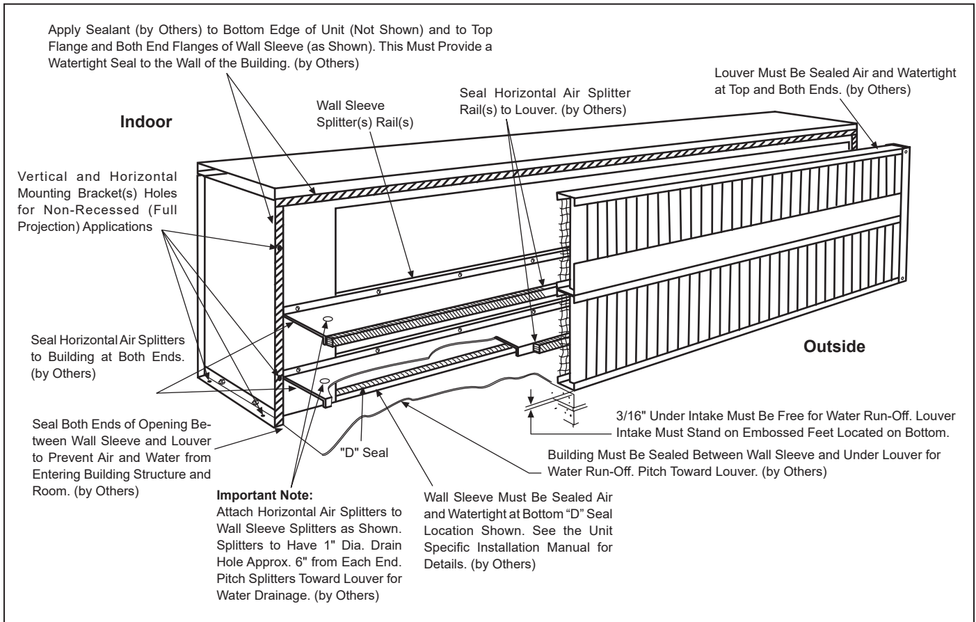
Figure 86: Recessed Wall Sleeve - Direct Sealing Wall Sleeve to Louver
