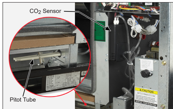
Figure 65: CO 2 Sensor For Demand Control Ventilation
