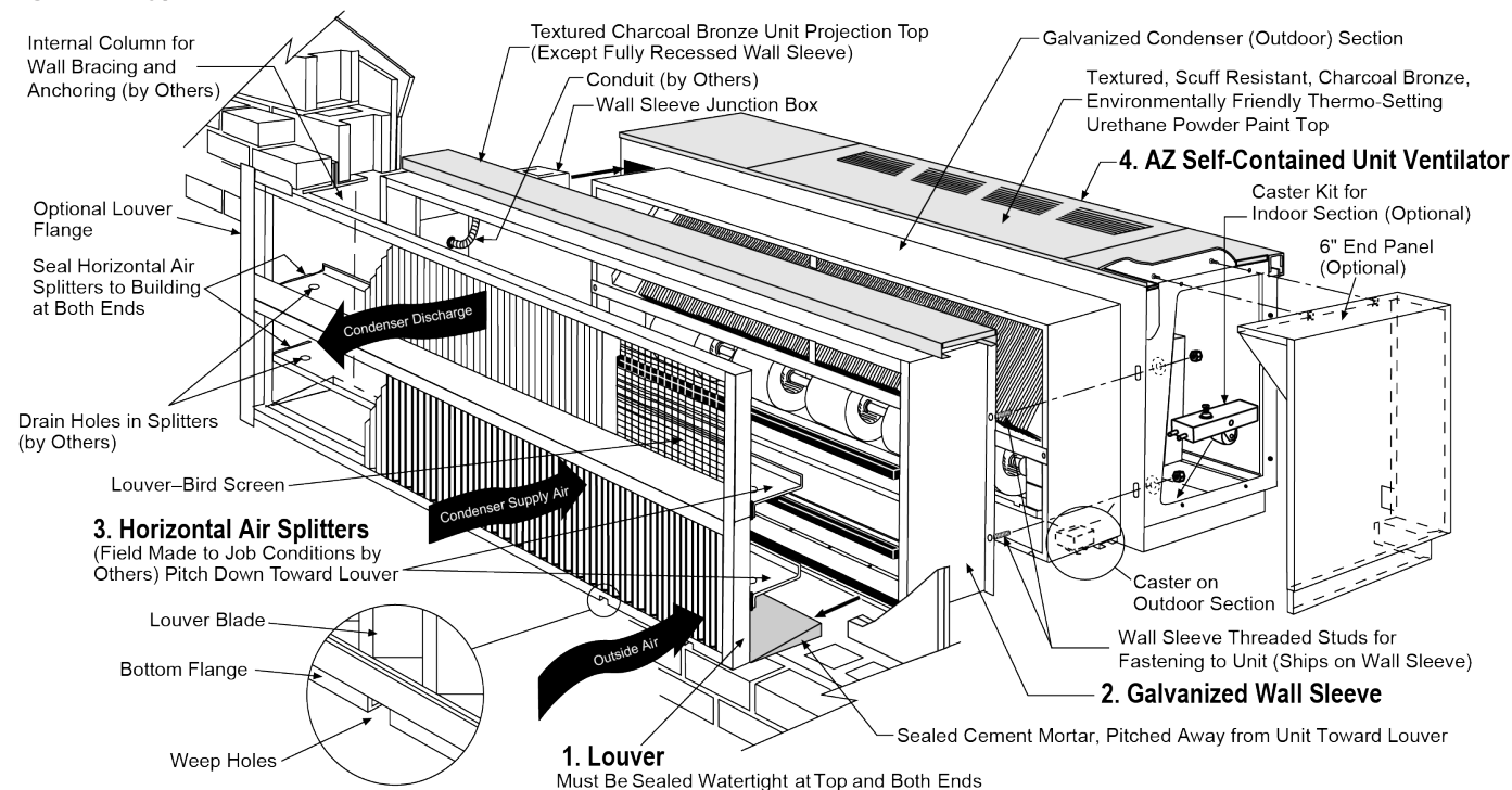
Figure 75: Typical Self-Contained Unit Ventilator Installation
