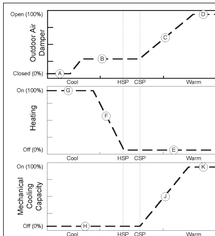
Figure 74: ASHRAE Cycle II Operation
