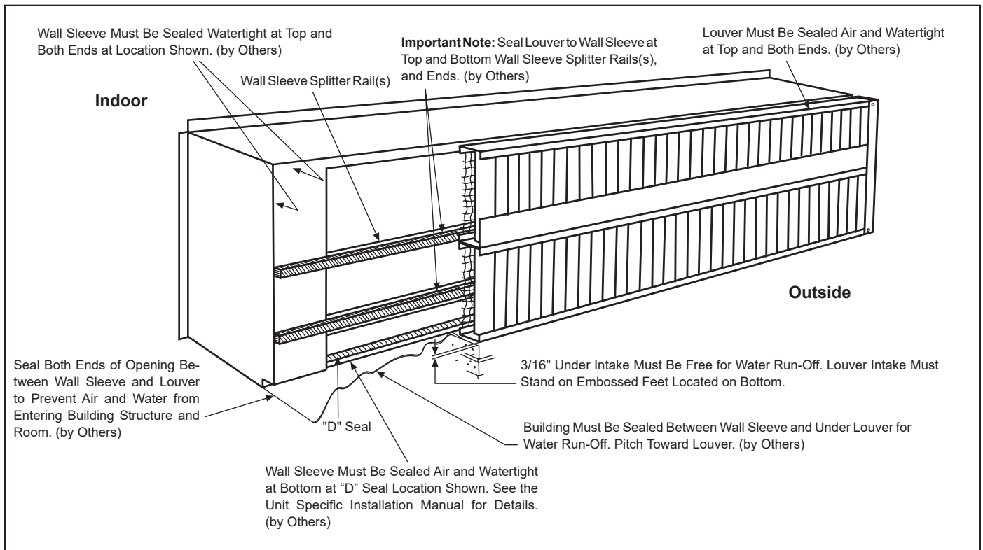
Figure 86: Recessed Wall Sleeve - Direct Sealing Wall Sleeve to Louver
