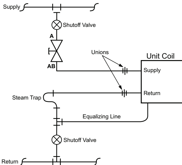
Figure 94: 2-Way Steam Modulating Valve Piping
