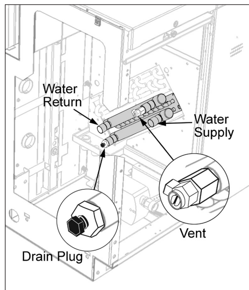
Figure 73: Manual Air Vent & Drain Plug
