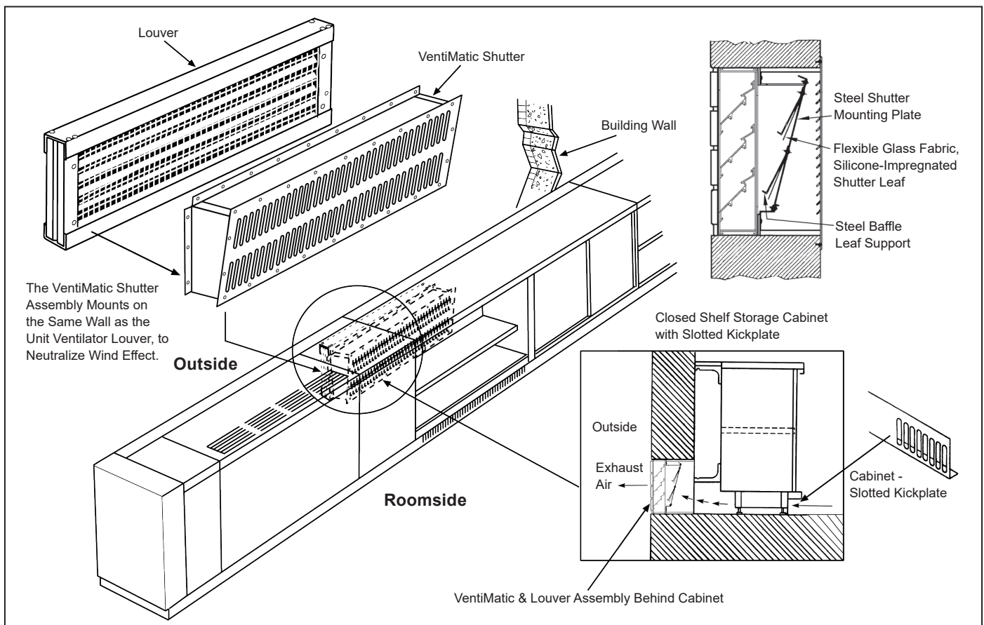
Figure 88: VentiMatic Shutter Installation
