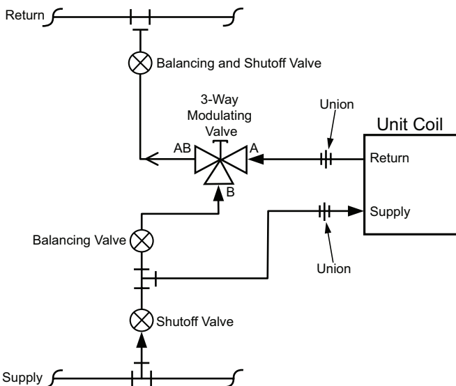
Figure 92: 3-Way Hot Water Modulating Valve Piping
