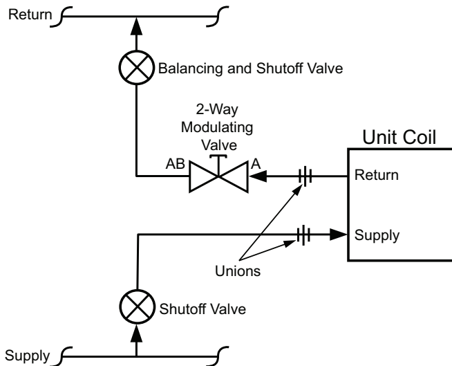
Figure 91: 2-Way Hot Water Modulating Valve Piping
