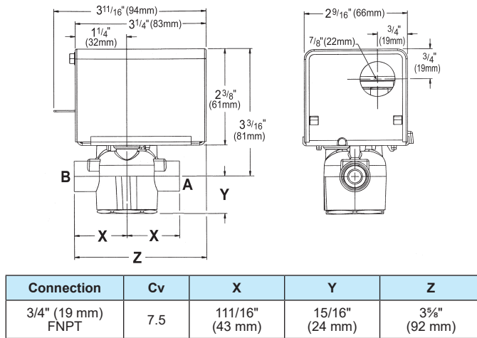
Figure 46: 2-Way EOC Steam Valve Dimensions
