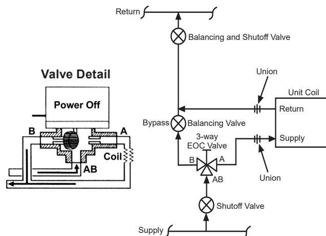
Figure 90: 3-Way Hot Water EOC Valve Piping
