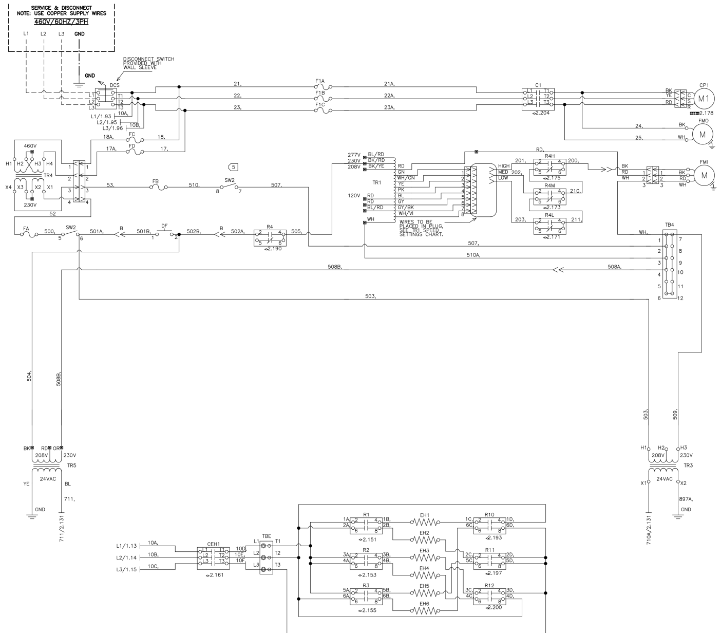
Figure 60: Electric Heat Wiring Diagram – Typical 460 V/60 Hz/3 Ph
