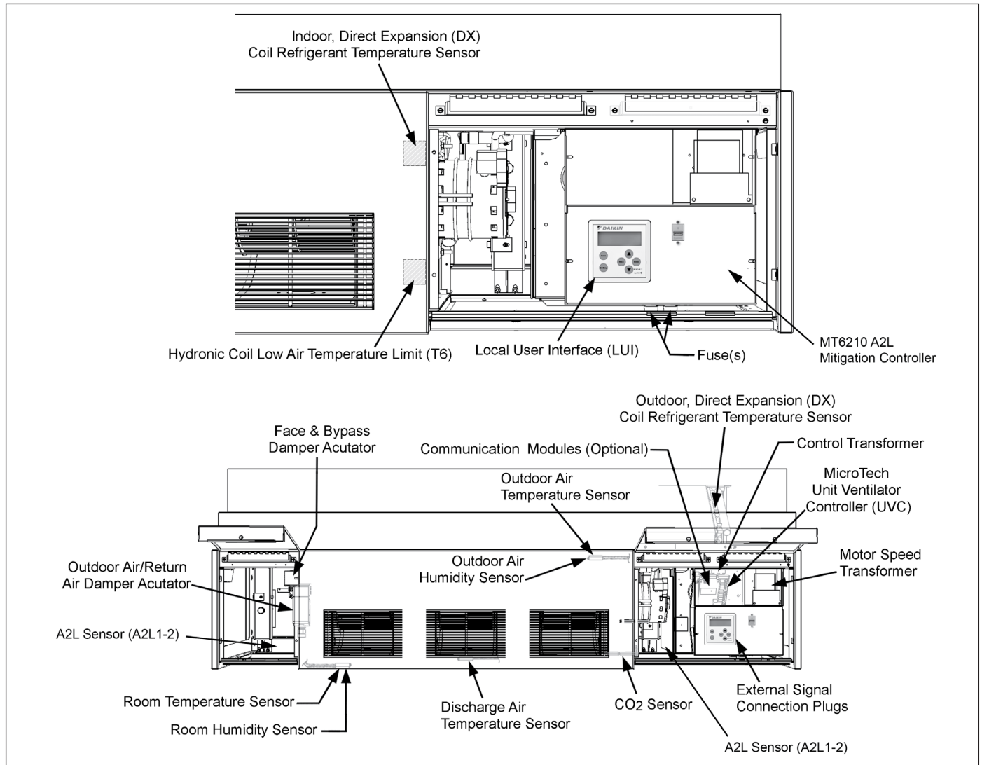
Figure 64: MicroTech Sensor and Component Locations
