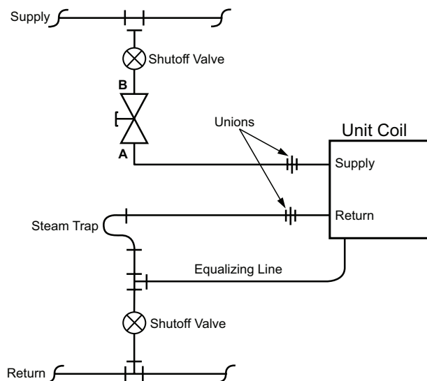
Figure 93: 2-Way Steam End of Cycle Valve Piping
