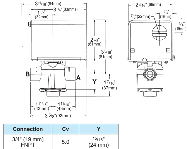
Figure 47: 3-Way EOC Valve Dimensions
