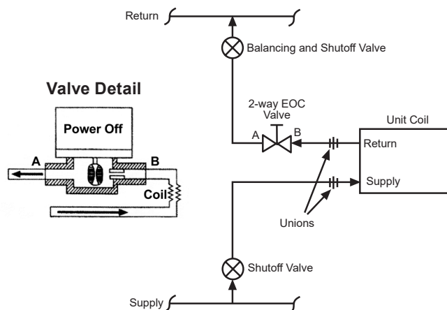
Figure 89: 2-Way Hot Water EOC Valve Piping
