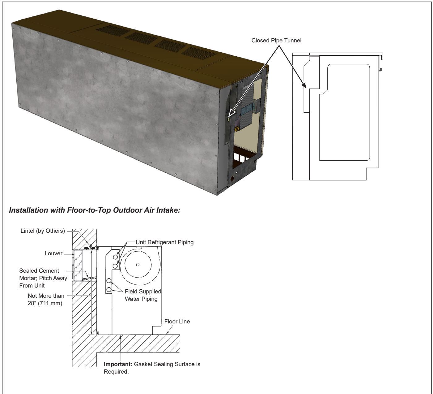
Figure 22: 21 \frac{1}{8} " Arrangement AB
