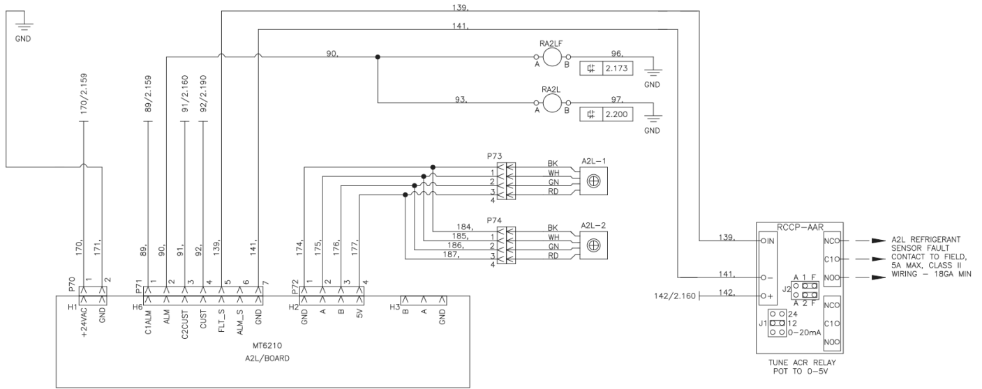
Figure 41: Electromechanical Controls – A2L Leak Mitigation
