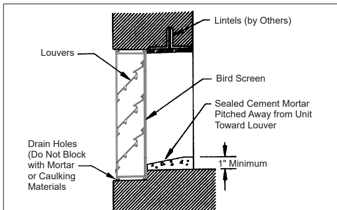
Figure 63: Recessed Wall Louver Installation Detail
