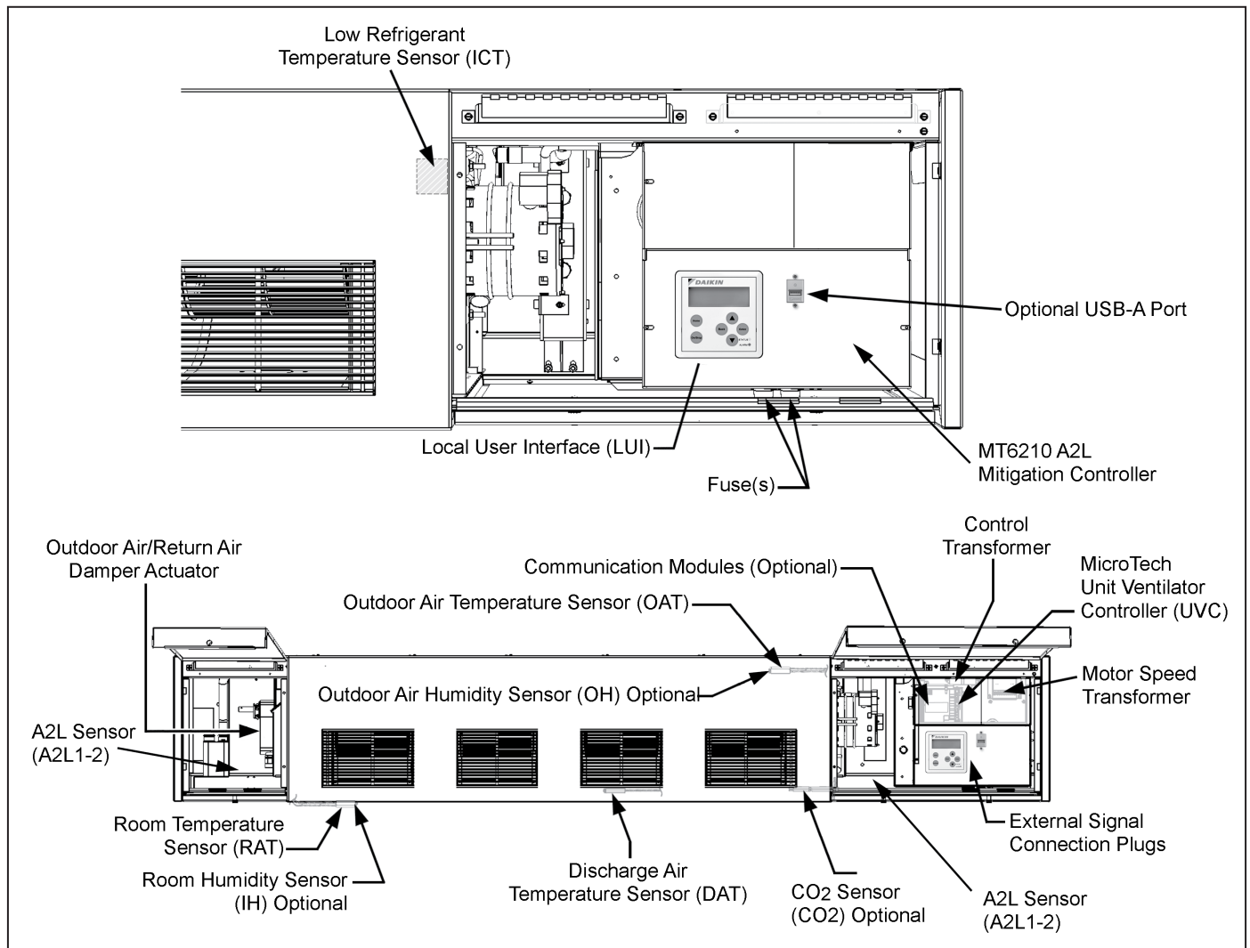
Figure 51: MicroTech Sensor and Component Locations
