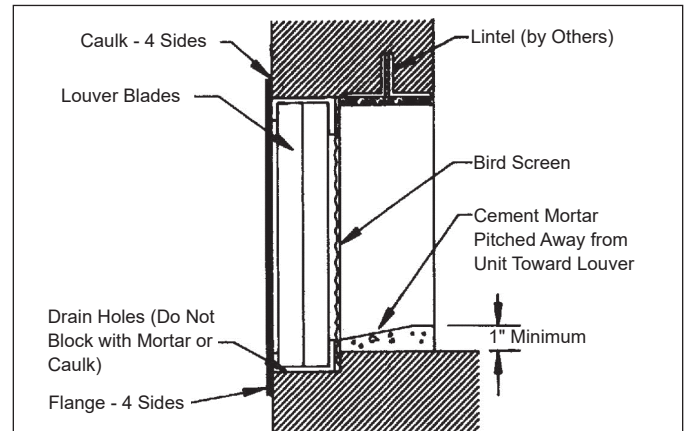
Figure 64: Flanged Wall Louver Installation Detail
