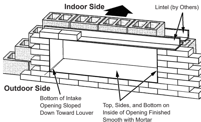
Figure 61: Typical Wall Opening with Lintels
