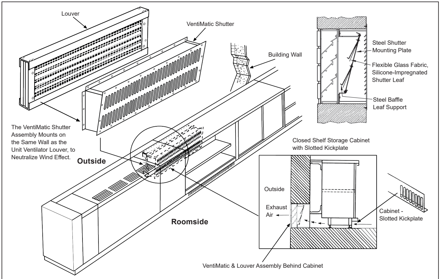
Figure 67: VentiMatic Shutter Installation
