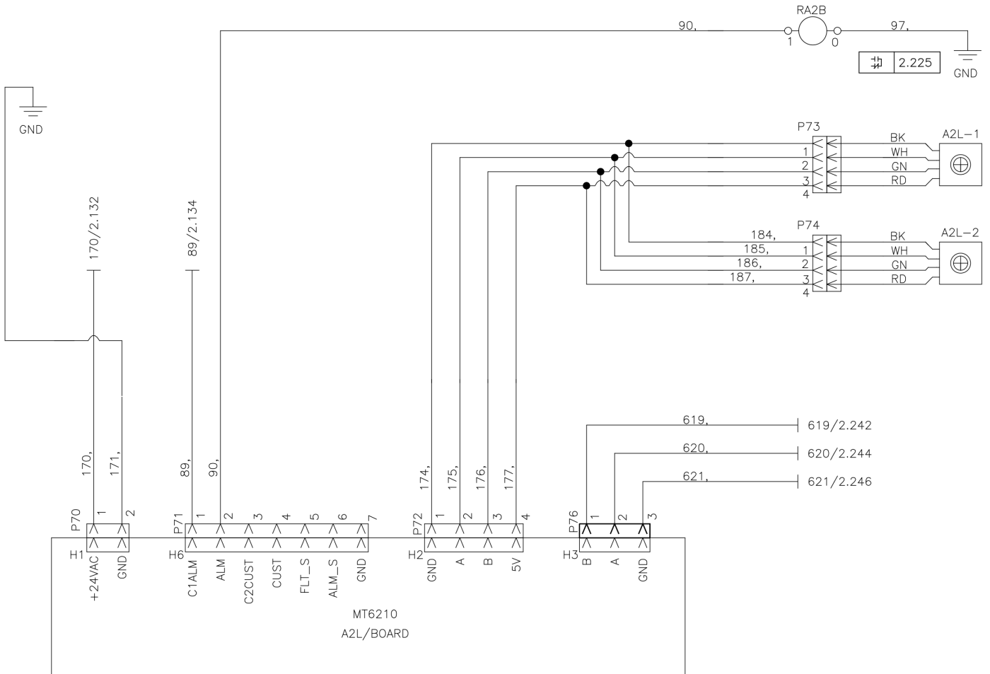
Figure 42: MicroTech Controls – A2L Leak Mitigation
