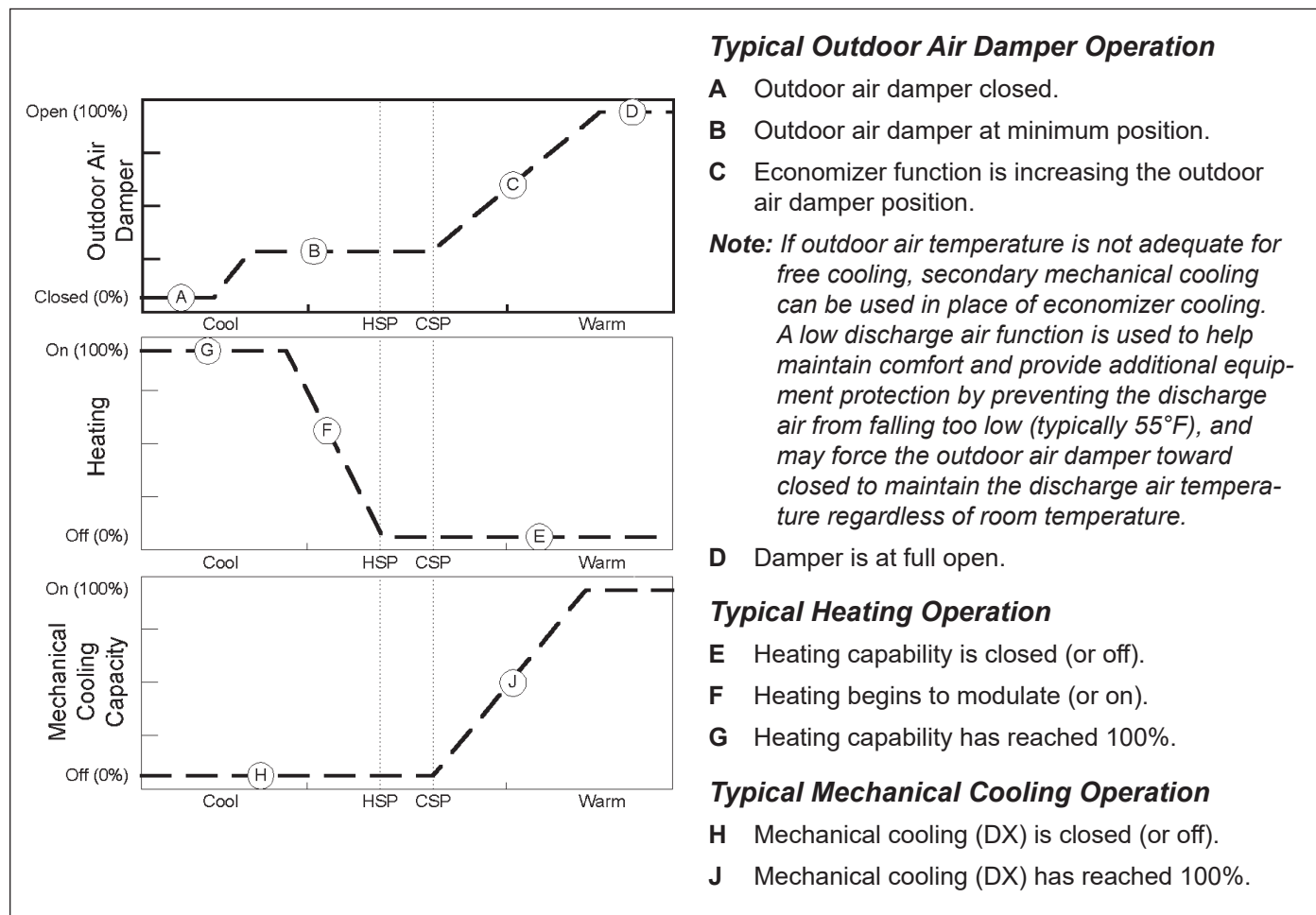
Figure 60: ASHRAE Cycle II Operation
