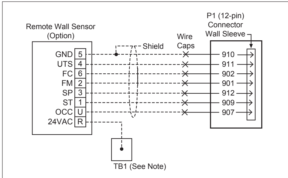
Figure 45: Wall-Mounted Temperature Sensor Wiring
