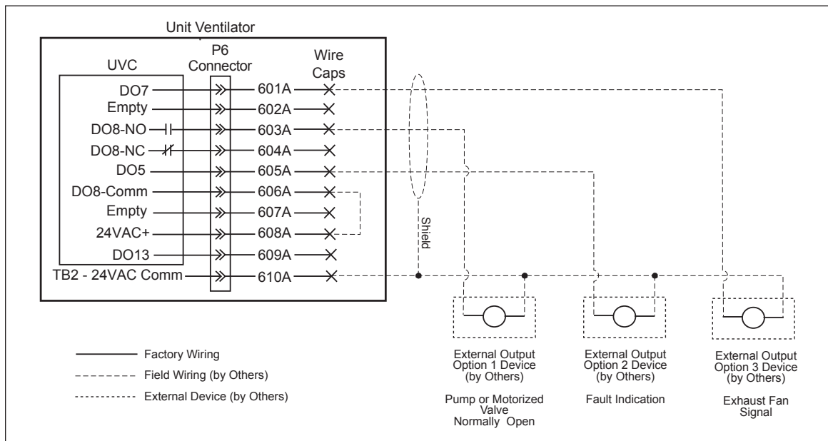
Figure 47: External Output Wiring - Single Unit
