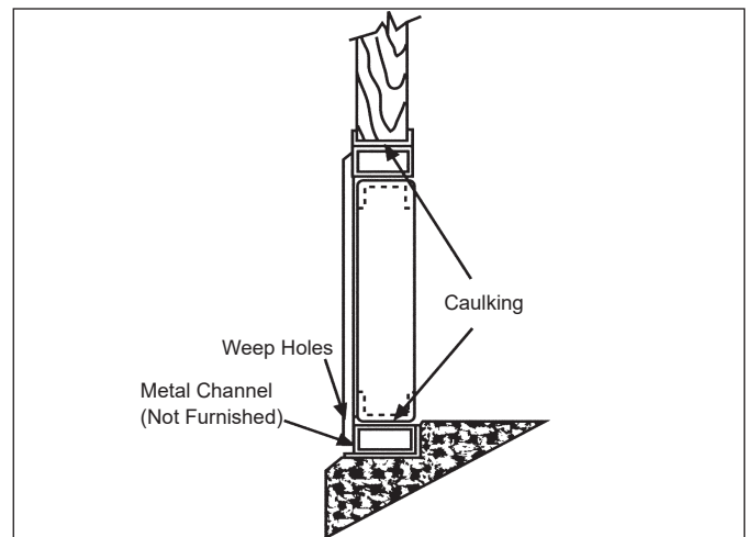
Figure 65: Panel Wall Louver Installation Detail
