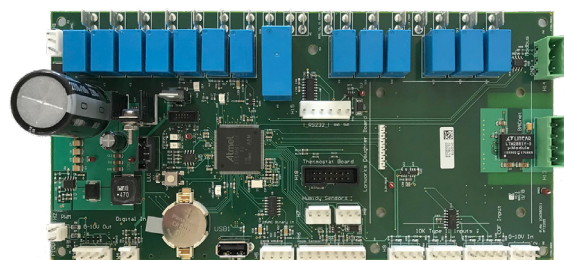
Figure 49: MicroTech Control Board
