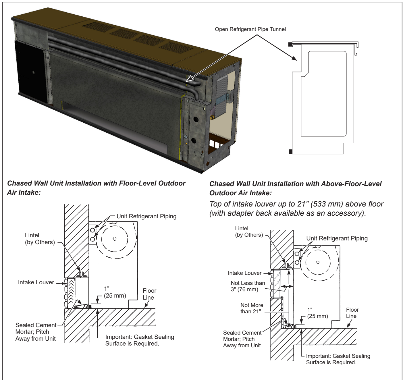
Figure 17: 16 5/8" Arrangement AL with Open Refrigerant Piping
