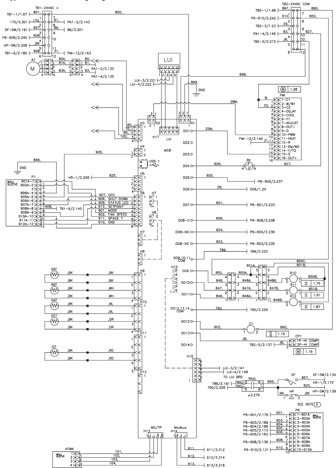
Figure 43: Typical MicroTech Wiring Diagram - 460V/60Hz/3Ph
