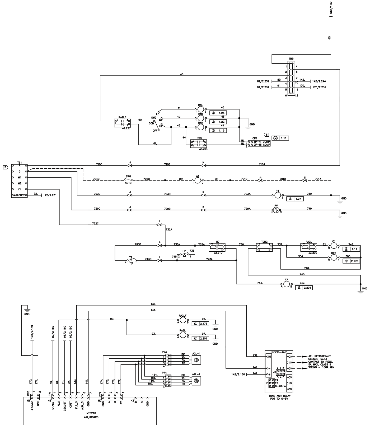
Figure 39: Typical Electromechanical Wiring Diagram - Thermostat Control with Normally Open Heat, 460V/60Hz/3Ph
