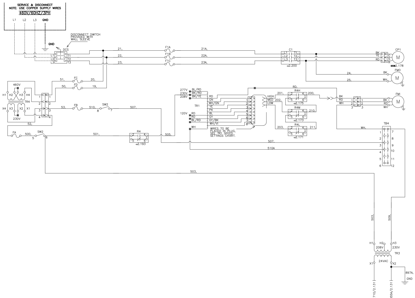
Figure 40: Typical Electromechanical Wiring Diagram - Thermostat Control with Normally Open Heat, 460V/60Hz/3Ph
