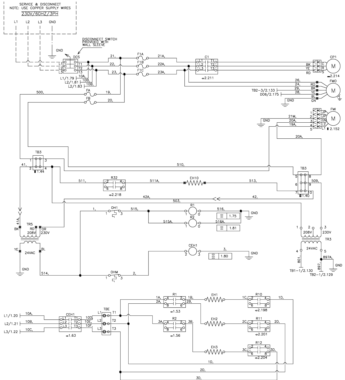
Figure 35: Typical MicroTech Wiring Diagram - Service and Disconnect - 230V/60Hz/3Ph
