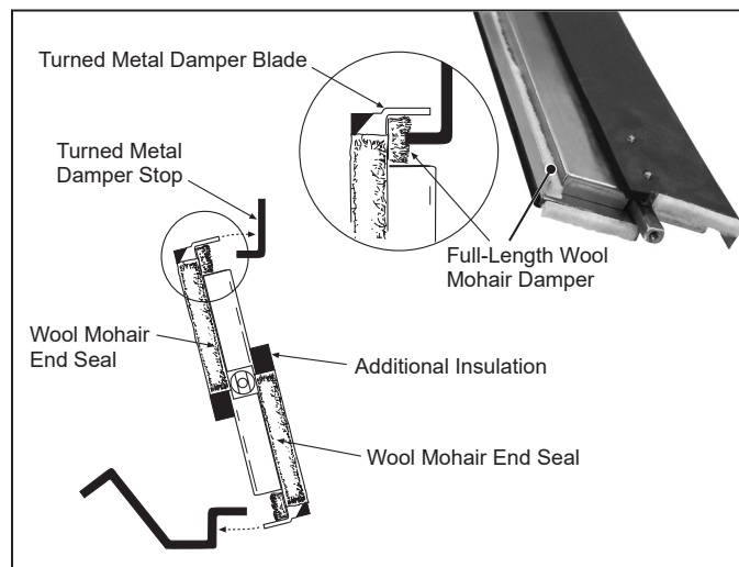
Figure 16: Outdoor Damper Seals Out Cold Weather
