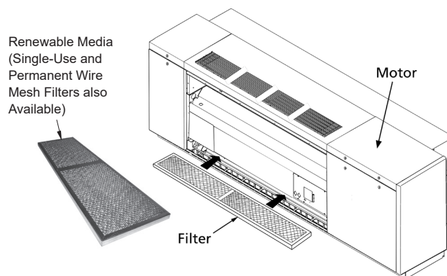
Figure 10: Easy Access to Filter
