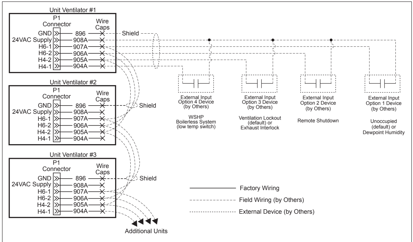
Figure 38: External Input Wiring Examples with or without Daisy Chaining of Units
