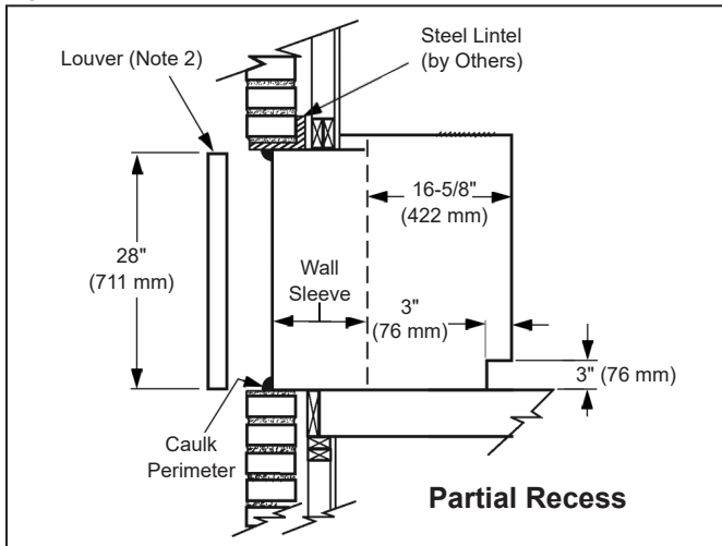
Figure 53: Wall Penetrations Detail - Partial Recess
