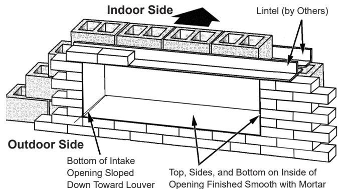
Figure 55: Typical Wall Opening with Lintels
