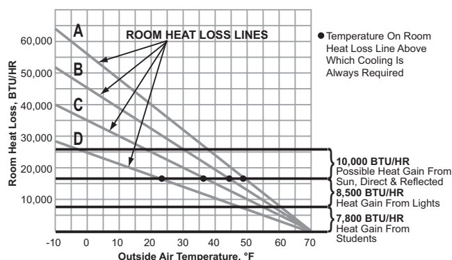
Figure 49: Heat Gain Vs. Heat Loss In Occupied Classrooms
