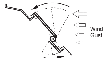
Figure 17: Room Air Damper Auto-Closed by Wind Gusts
