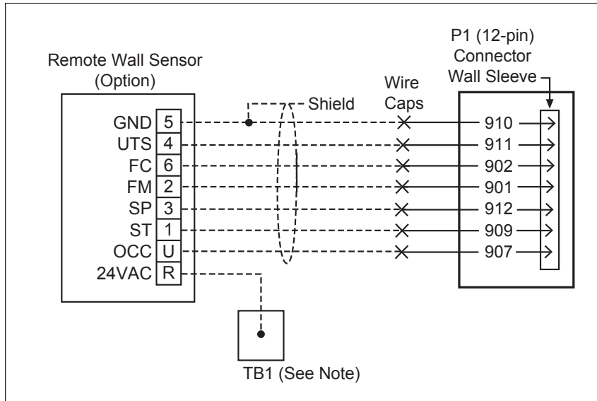
Figure 37: Wall-Mounted Temperature Sensor Wiring for Wall Sensor
