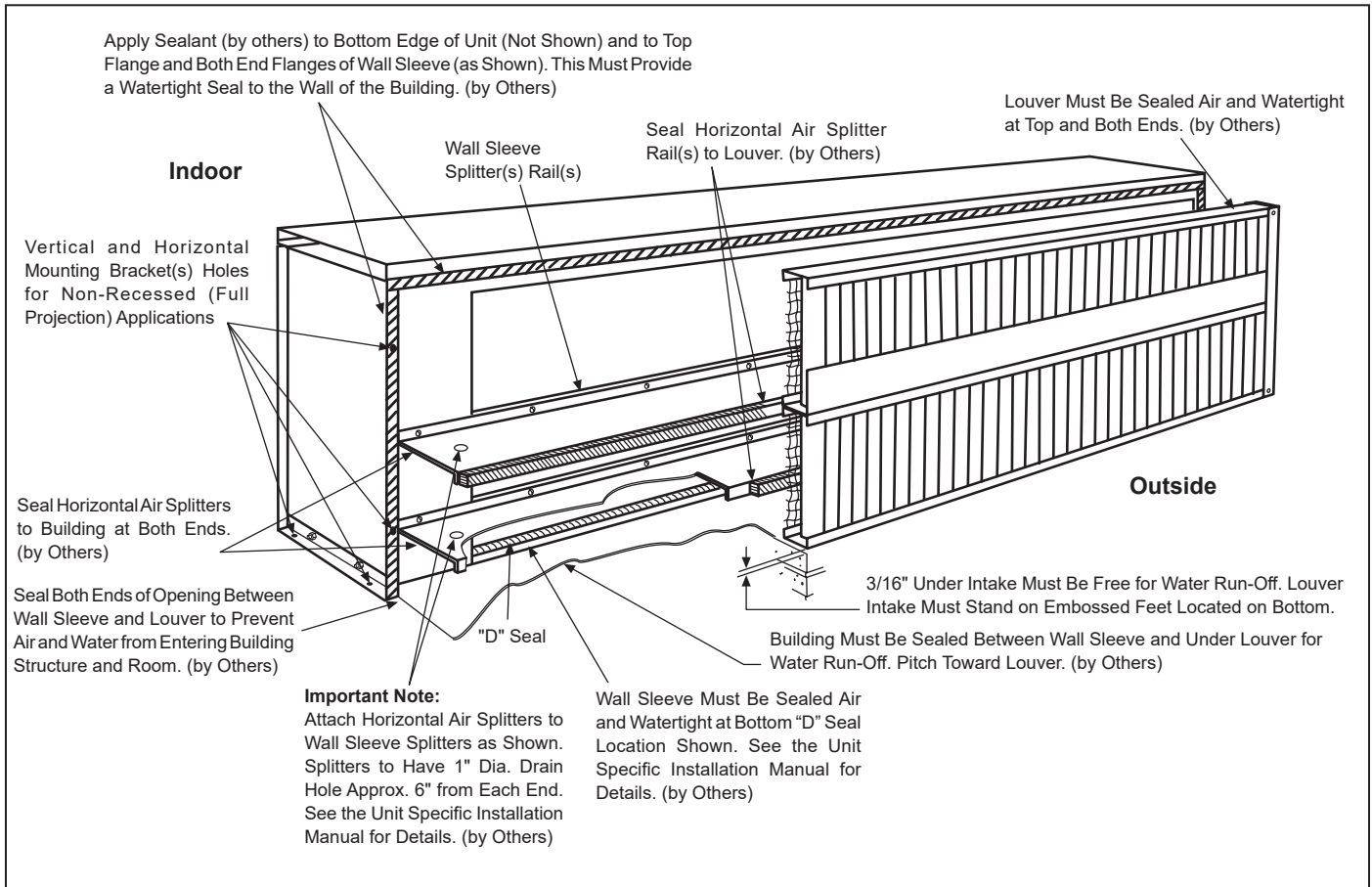
Figure 62: Recessed Wall Sleeve - Direct Sealing Wall Sleeve to Louver
