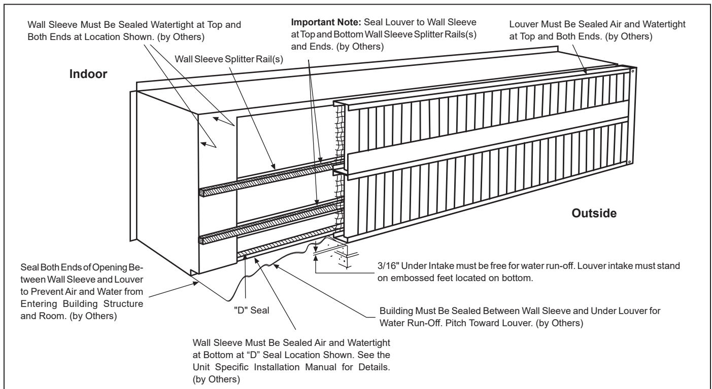
Figure 62: Recessed Wall Sleeve - Direct Sealing Wall Sleeve to Louver
