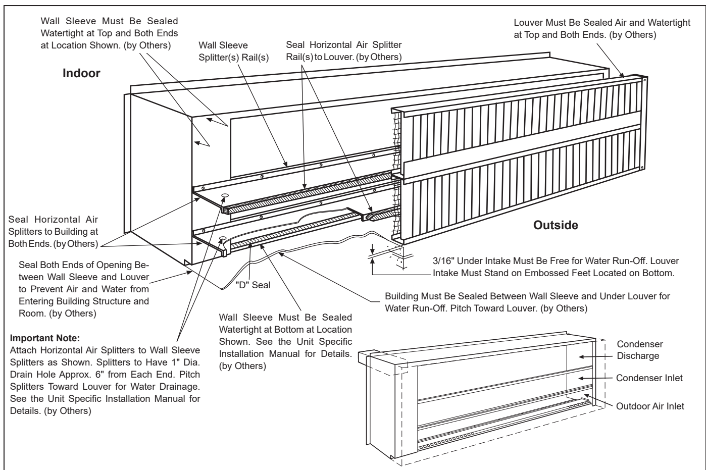
Figure 60: Recessed Wall Sleeve with Horizontal Air Splitters
