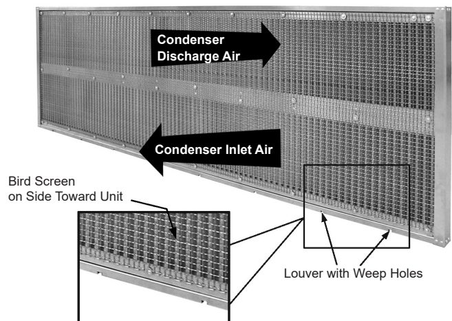
Figure 31: Vertical Blade Louver, Without Flange Inside View
