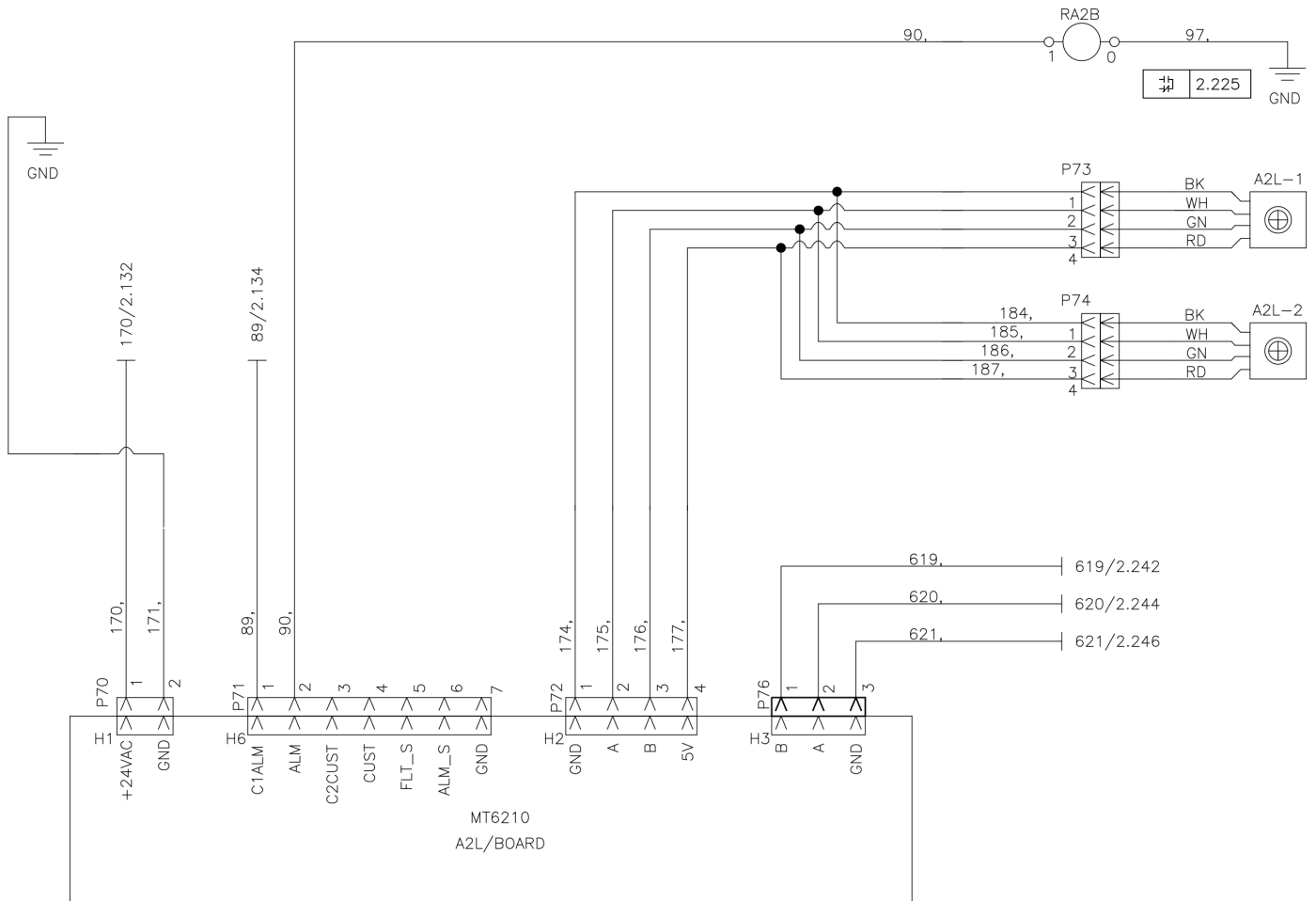
Figure 36: MicroTech Controls – A2L Leak Mitigation
