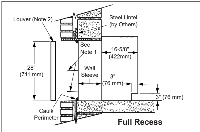
Figure 52: Wall Penetrations Detail - Full Recess
