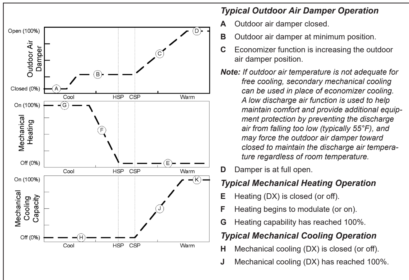
Figure 50: ASHRAE Cycle II Operation
