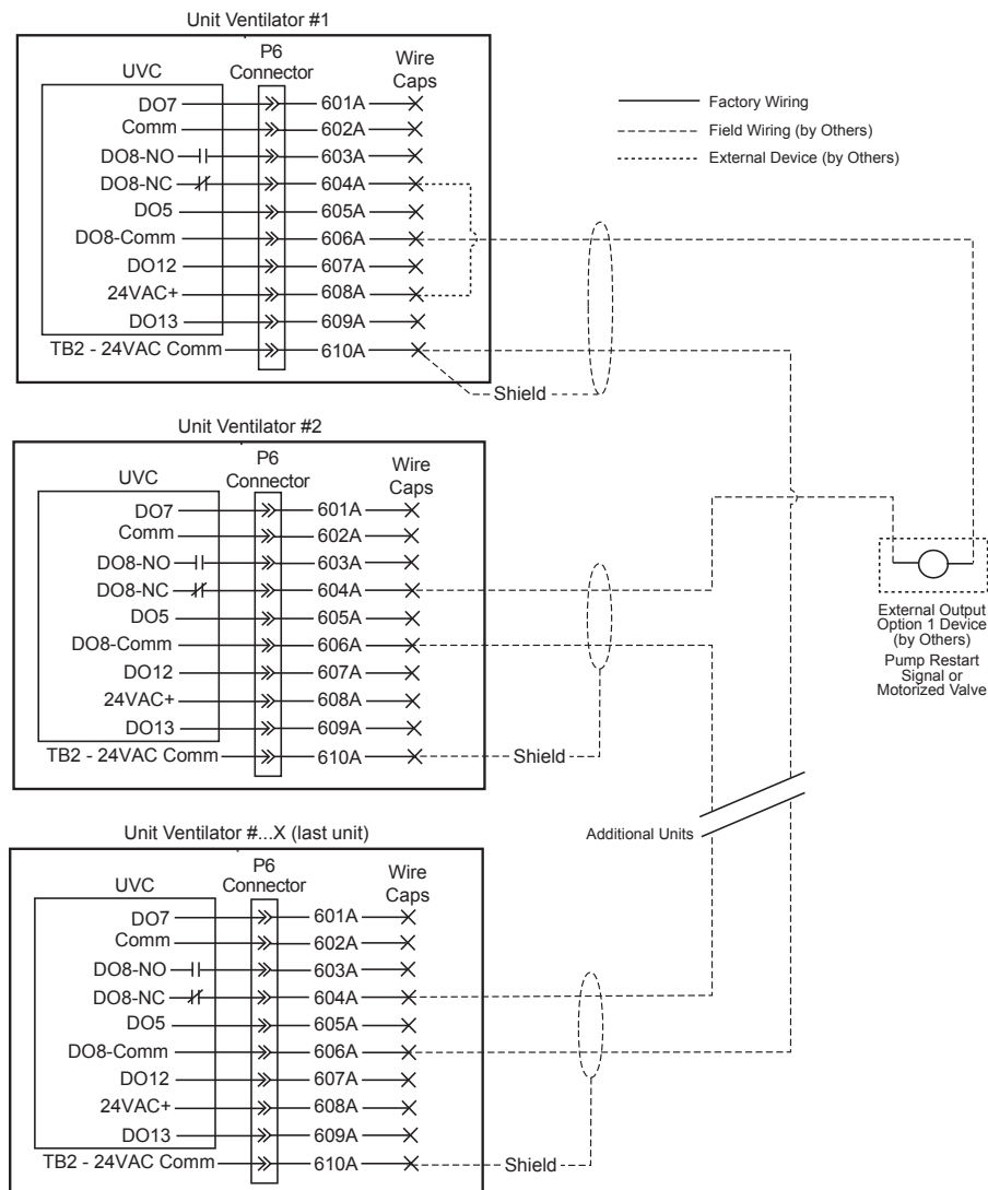
Figure 40: External Output Wiring - Multiple Units Shown
