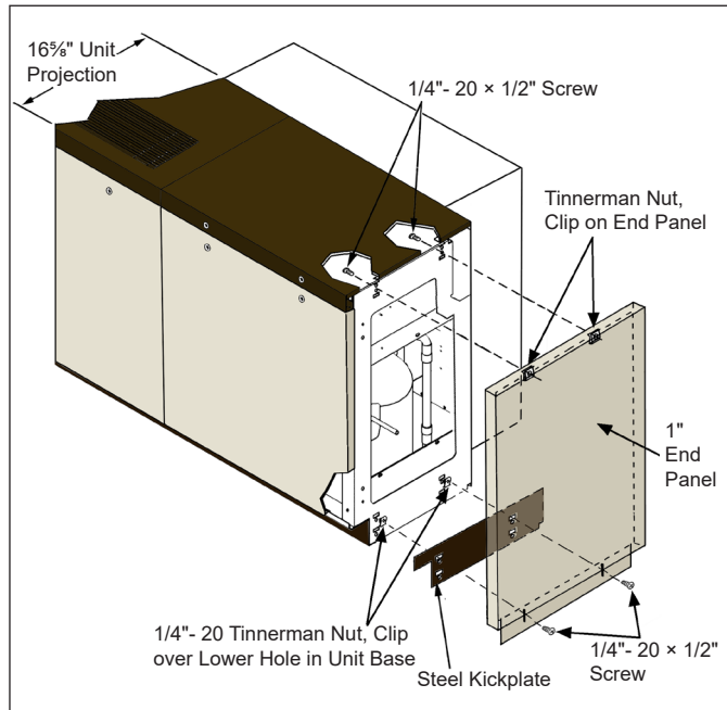
Figure 19: 1" End Panel
