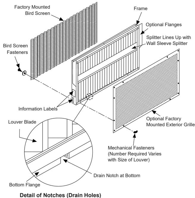
Figure 28: Typical Wall Louver and Grille
