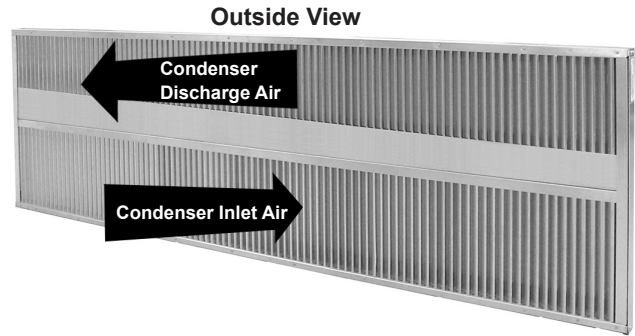
Figure 30: Grille Detail
