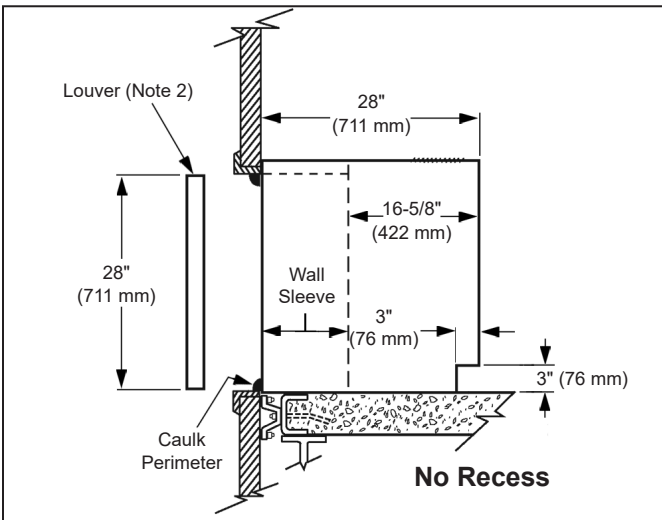
Figure 54: Wall Penetrations Detail - No Recess
