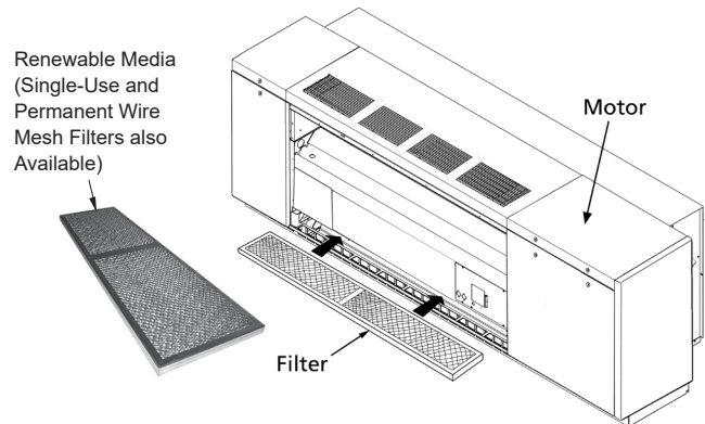
Figure 10: Easy Access to Filter
