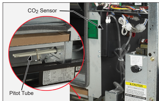
Figure 43: CO 2 Sensor for Demand Control Ventilation
