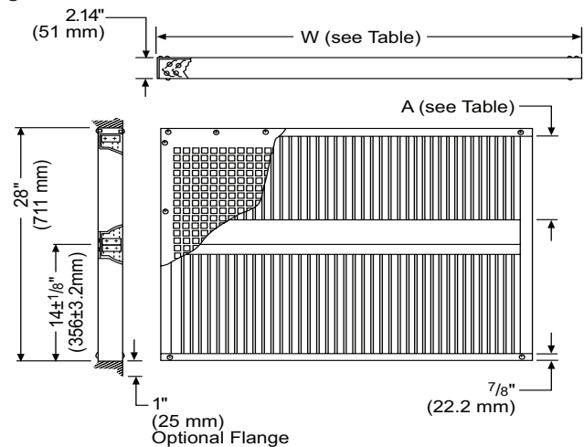
Figure 30: Grille Detail
