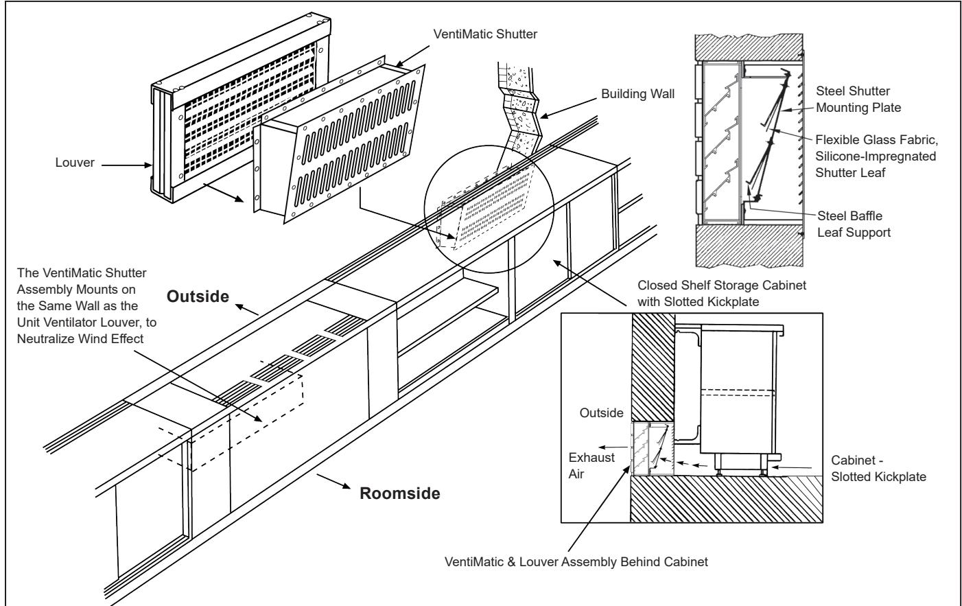
Figure 64: VentiMatic Shutter Installation
