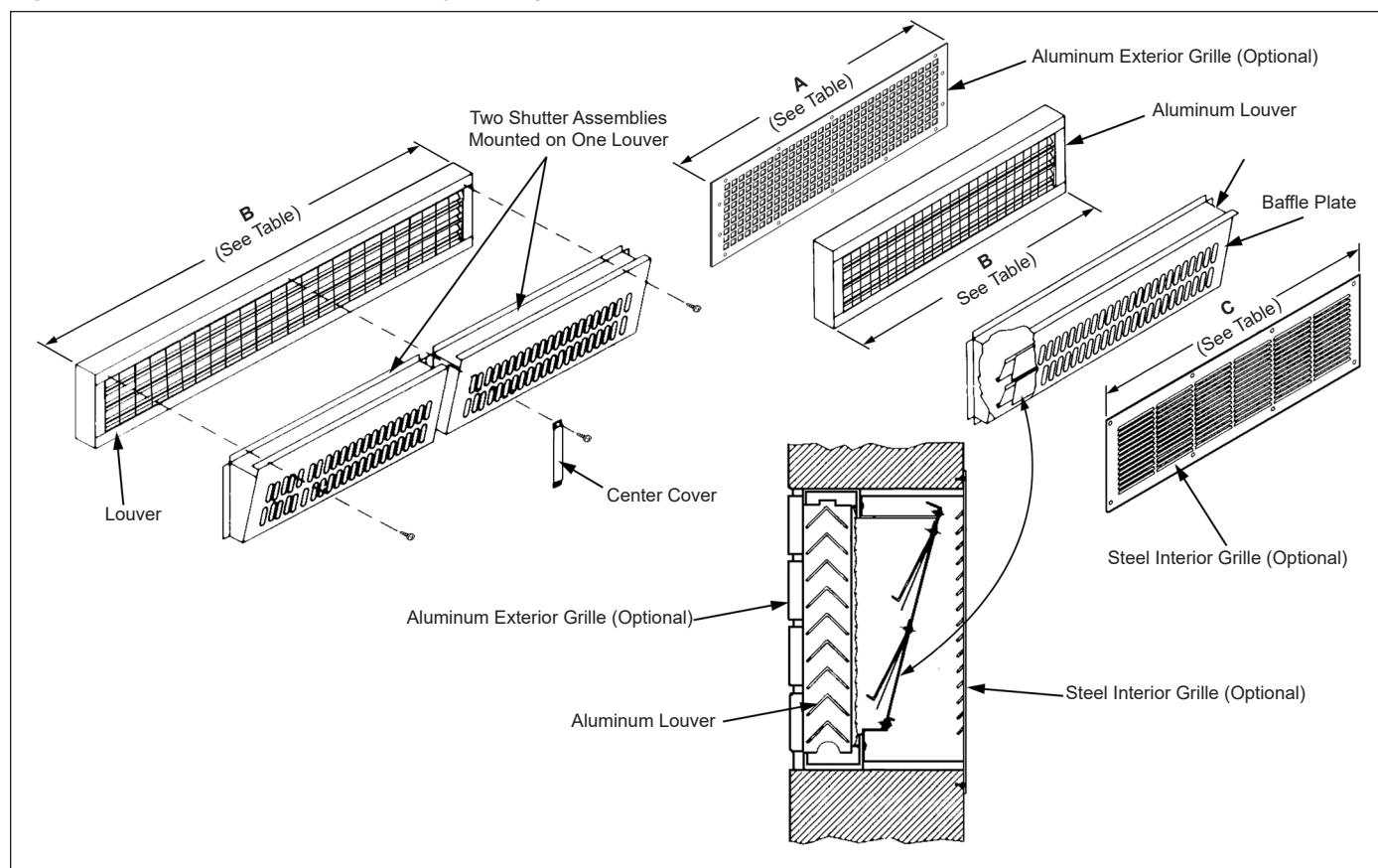
Figure 32: VentiMatic Shutter Assembly with Optional Grille
