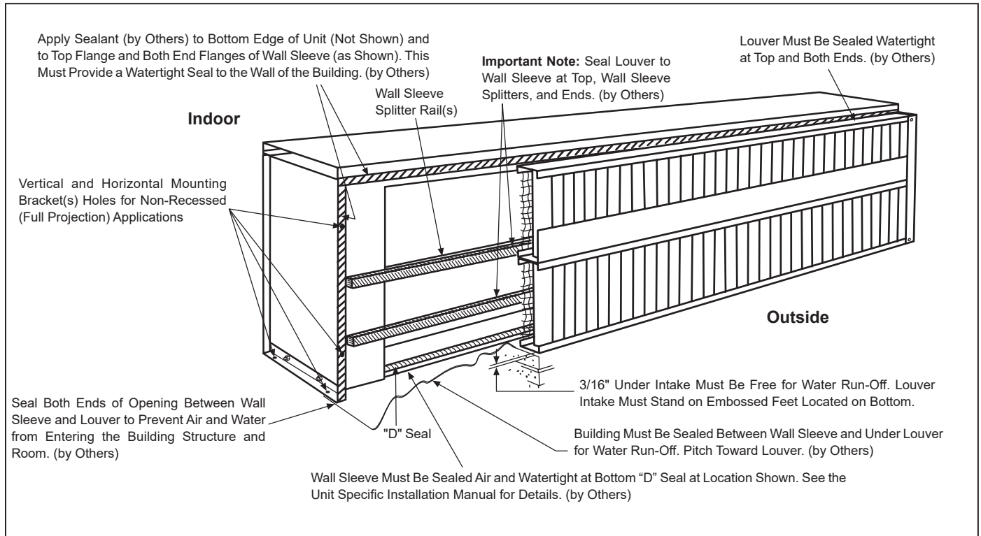
Figure 63: Sealing Full Projection Wall Sleeve to Louver Intake Without Horizontal Air Splitters
