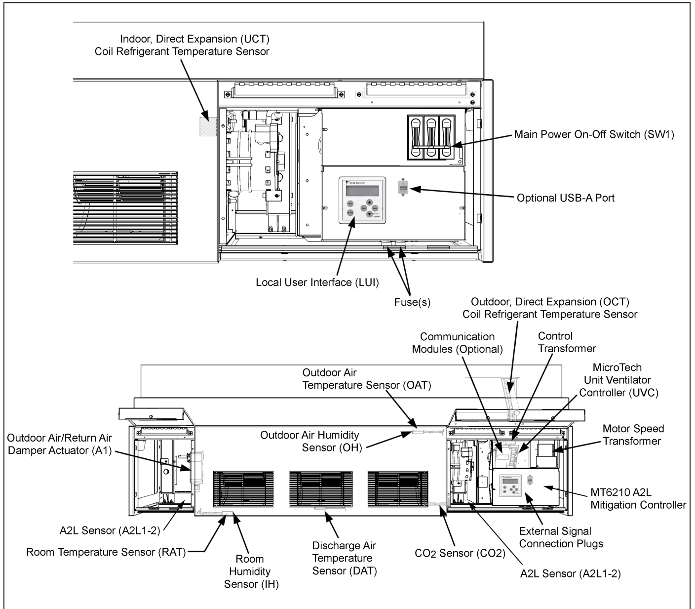
Figure 44: MicroTech Control Sensor and Component Locations
