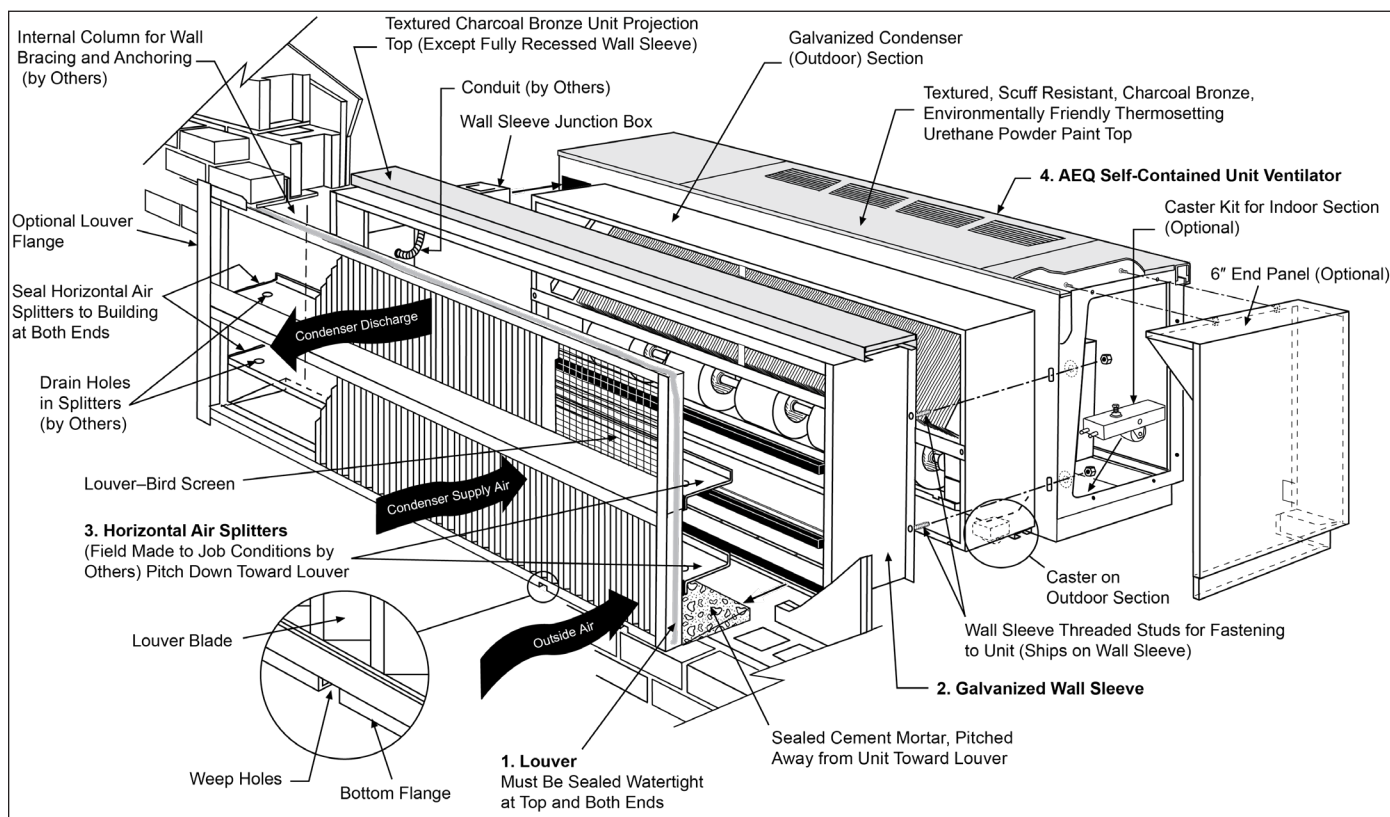
Figure 51: Typical Self-Contained Unit Ventilator Installation
