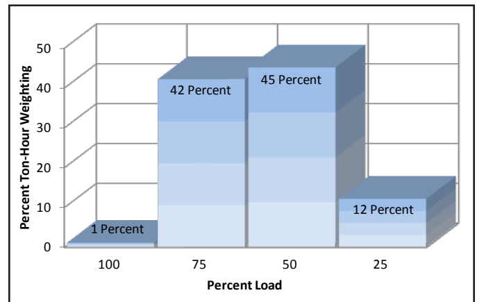
Figure 3: IPLV Defined by AHRI Standard 550/590
