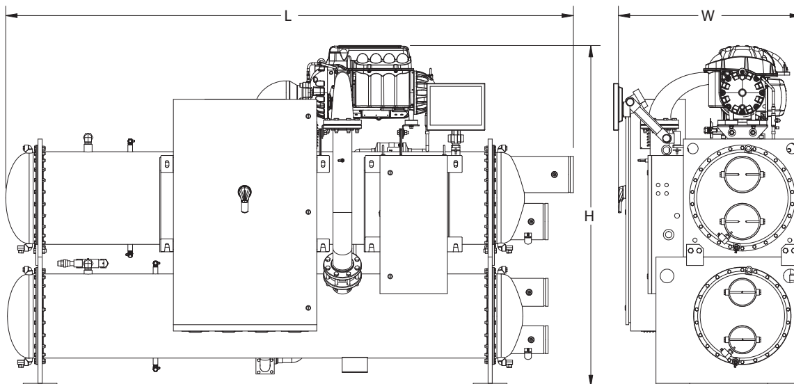
Figure 4: WMC145S (2-pass, right-hand configuration, with grooved connections)
