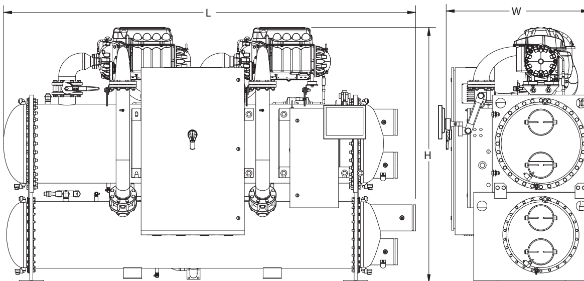
Figure 5: WMC145-400D (2-pass, right-hand configuration, with grooved connections)
