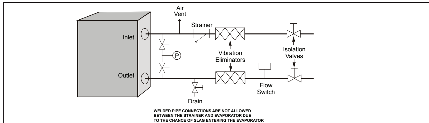
Figure 10: Typical Chilled Water Piping, Braze Plate
