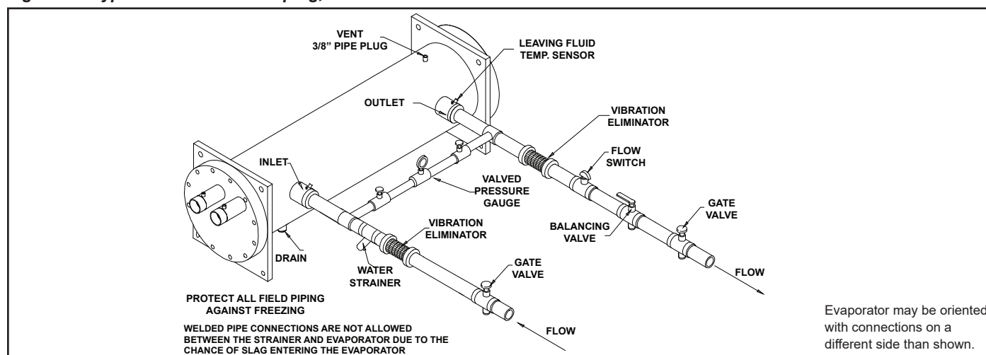
Figure 11: Typical Chilled Water Piping, Shell and Tube
