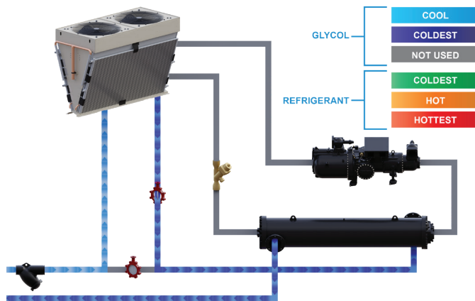
Figure 3: Integrated Waterside Economizer Operation
