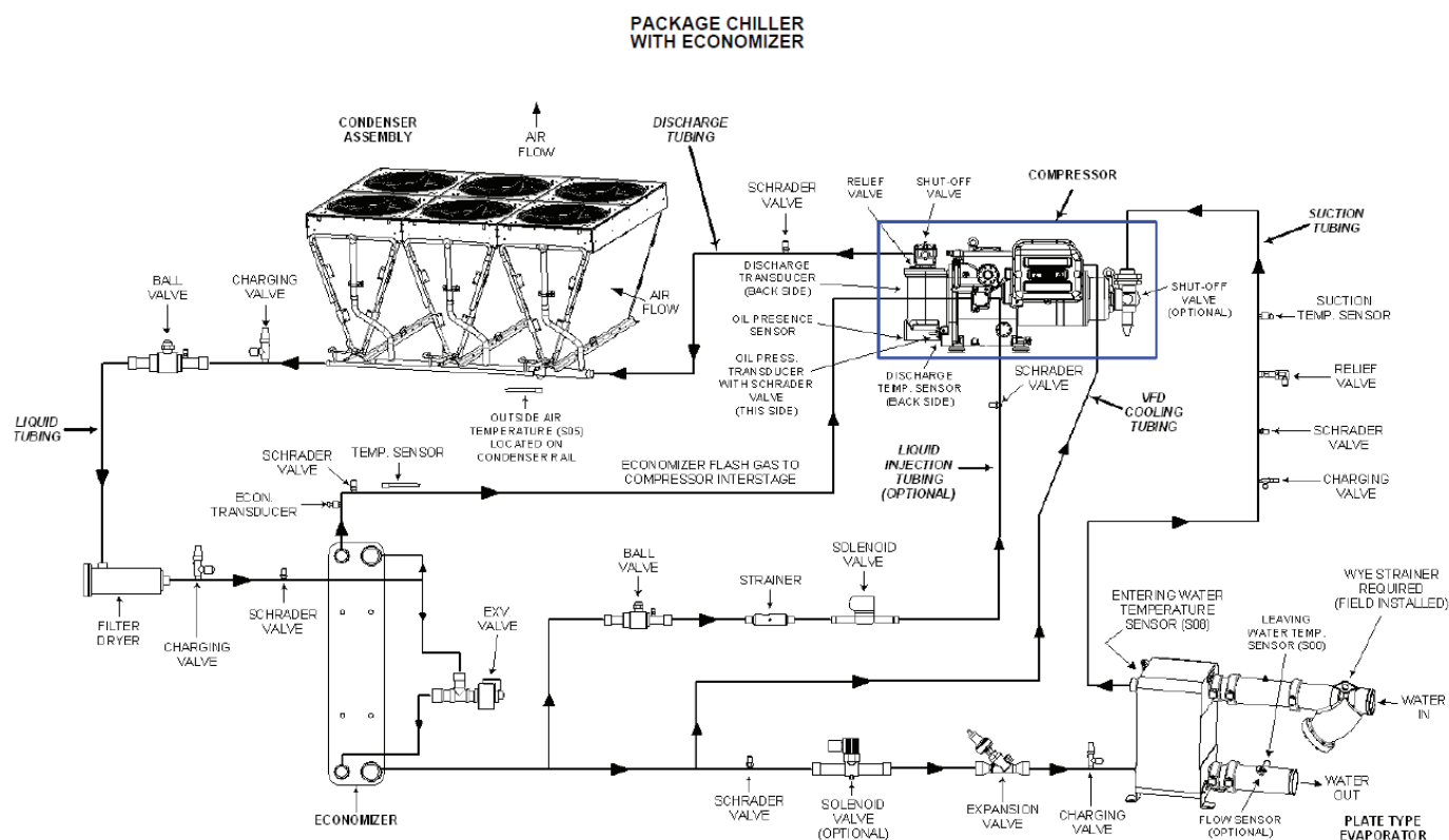
Figure 12: Refrigeration System Diagram, Braze Plate Evaporator (shown with optional refrigerant-side economizer)
