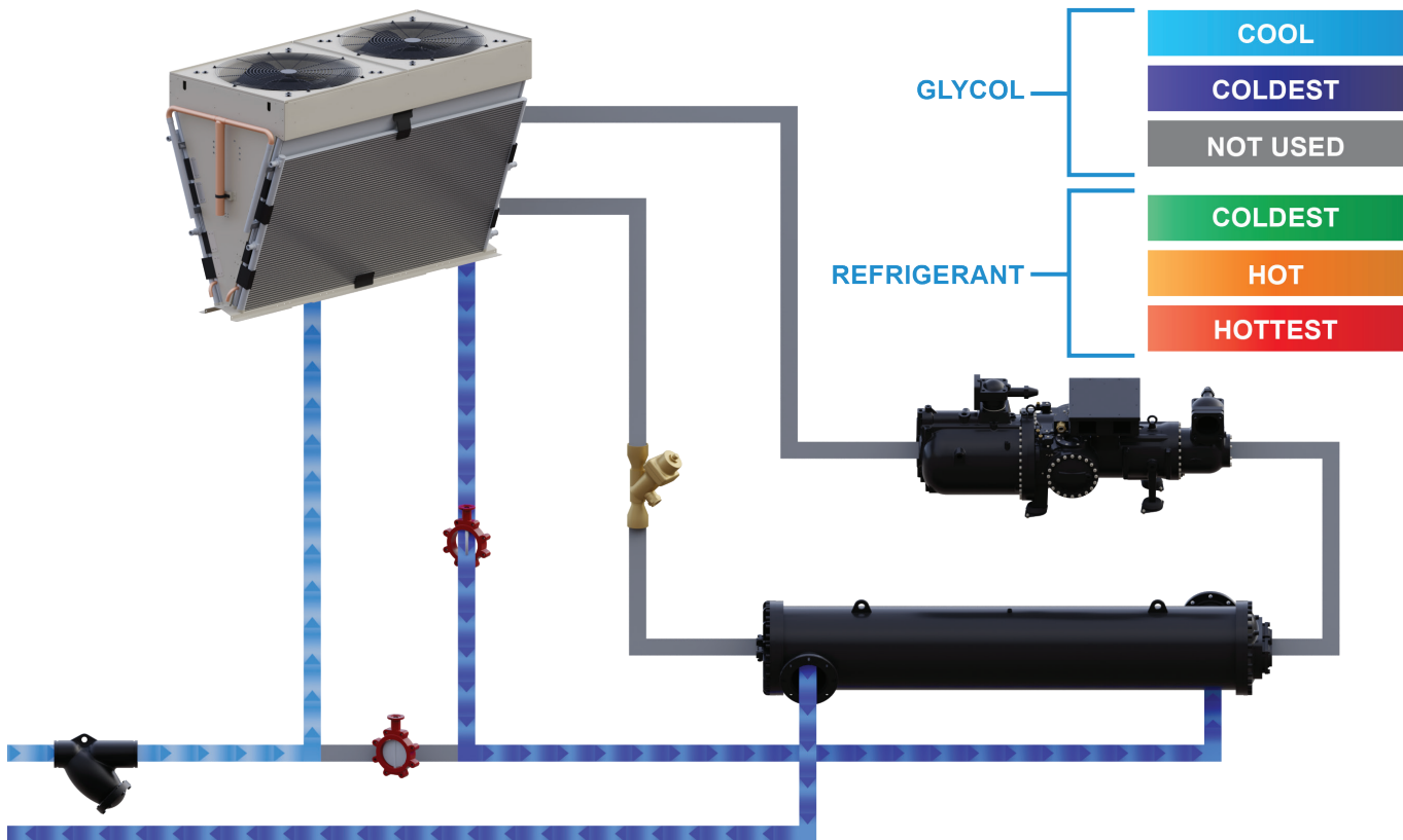
Figure 16: Integrated Waterside Economizer Operation
