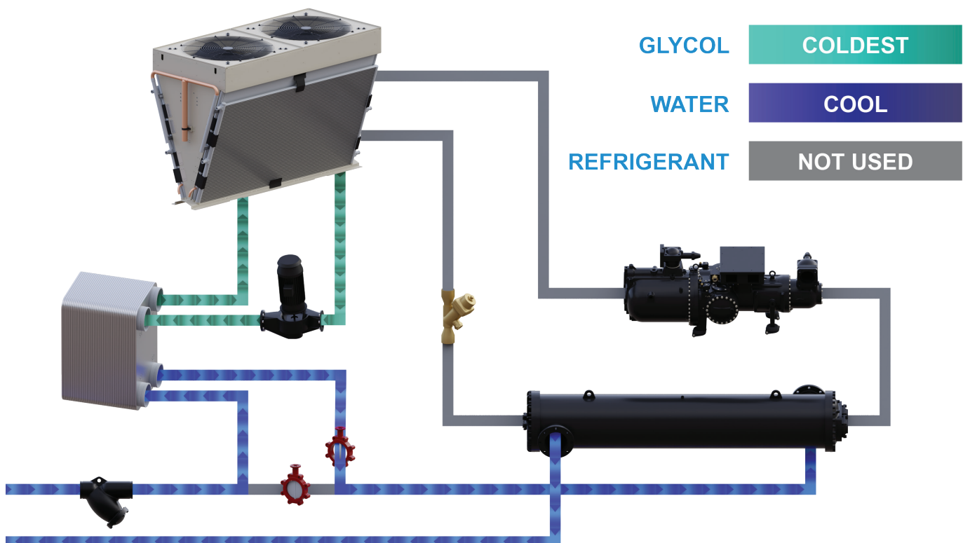
Figure 18: Closed Loop Waterside Economizer
