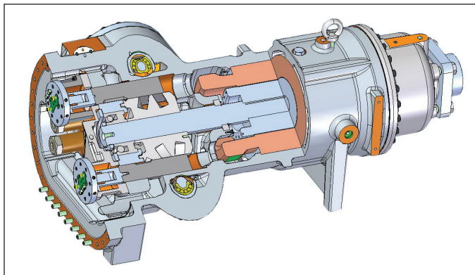
Figure 1: VVR® Compressor Technology
