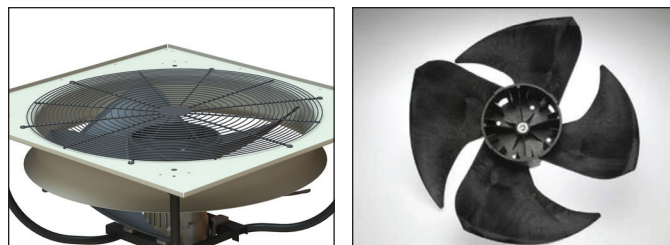
Figure 2: Shrouded Fan Assembly with Molded Blade
