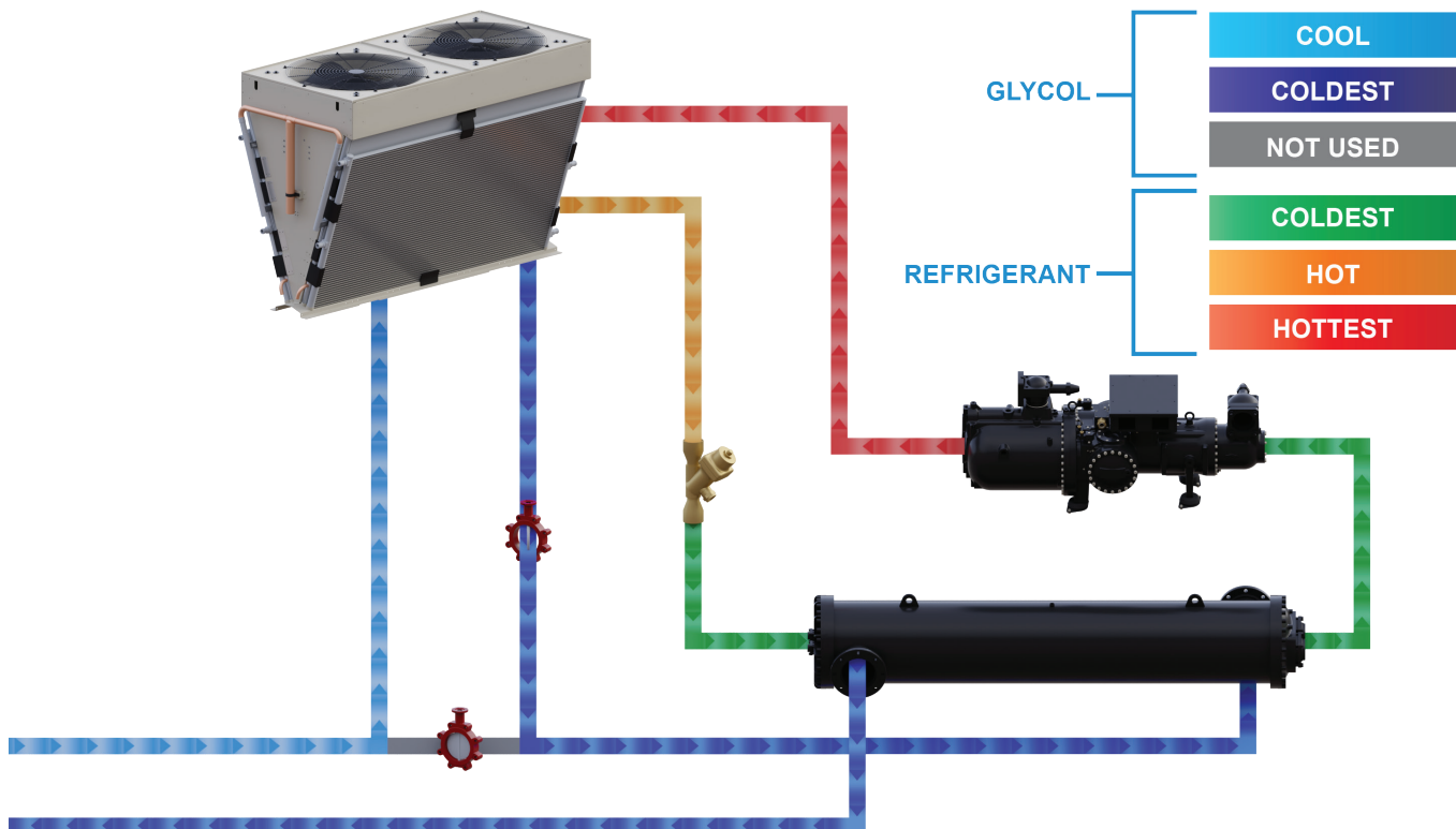
Figure 15: Hybrid Cooling Mode Operation
