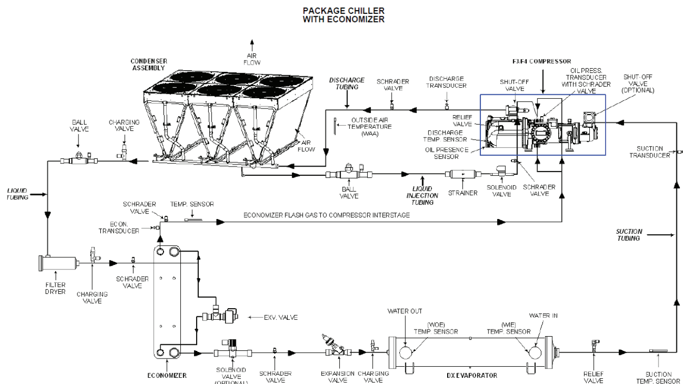
Figure 13: Refrigeration System Diagram, Shell and Tube Evaporator (shown with optional refrigerant-side economizer)
