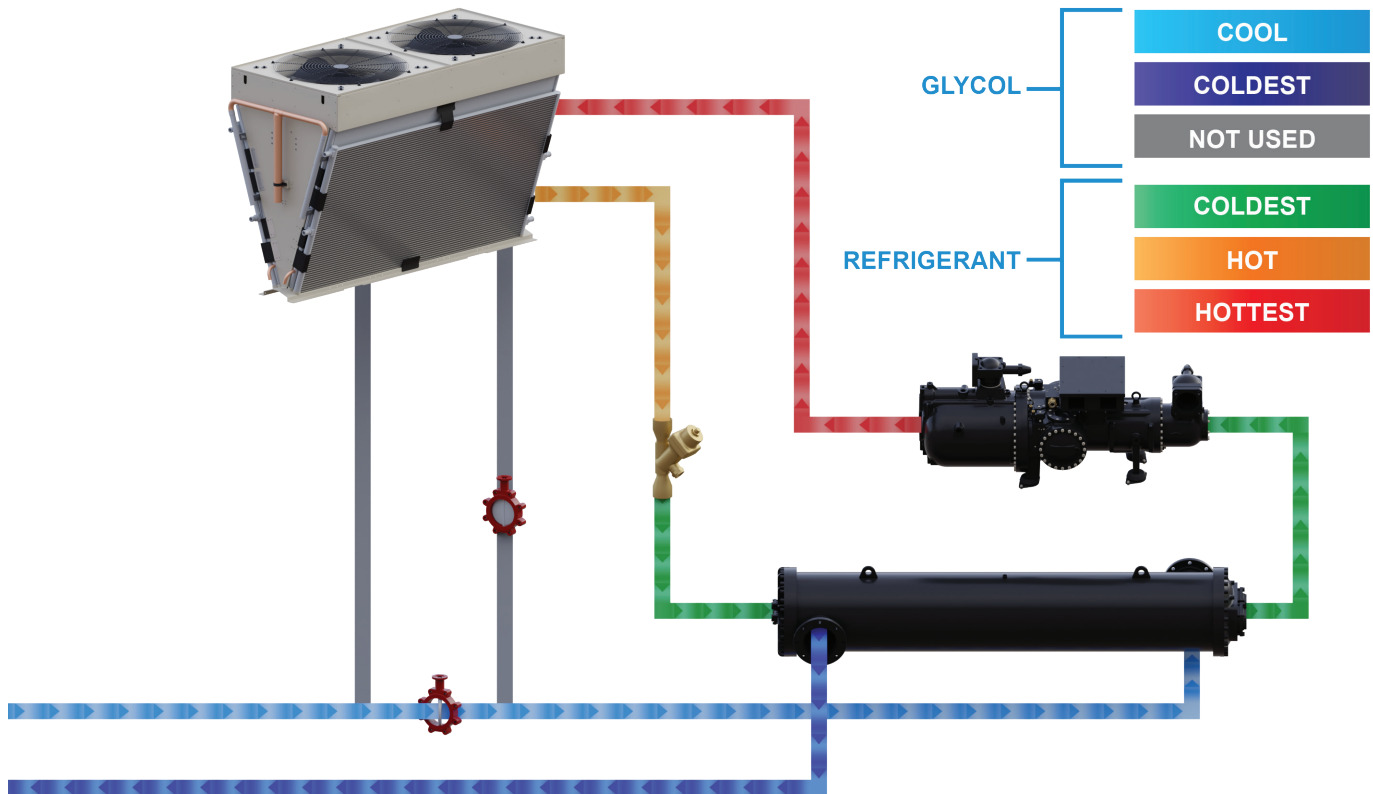
Figure 17: Mechanical Cooling Operation Only
