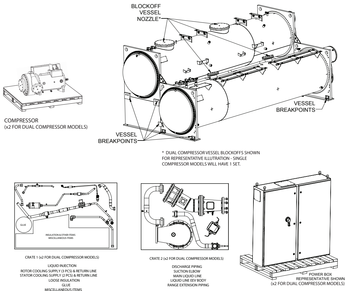
Figure 7: “Partial Disassembly” - Representative Illustration
