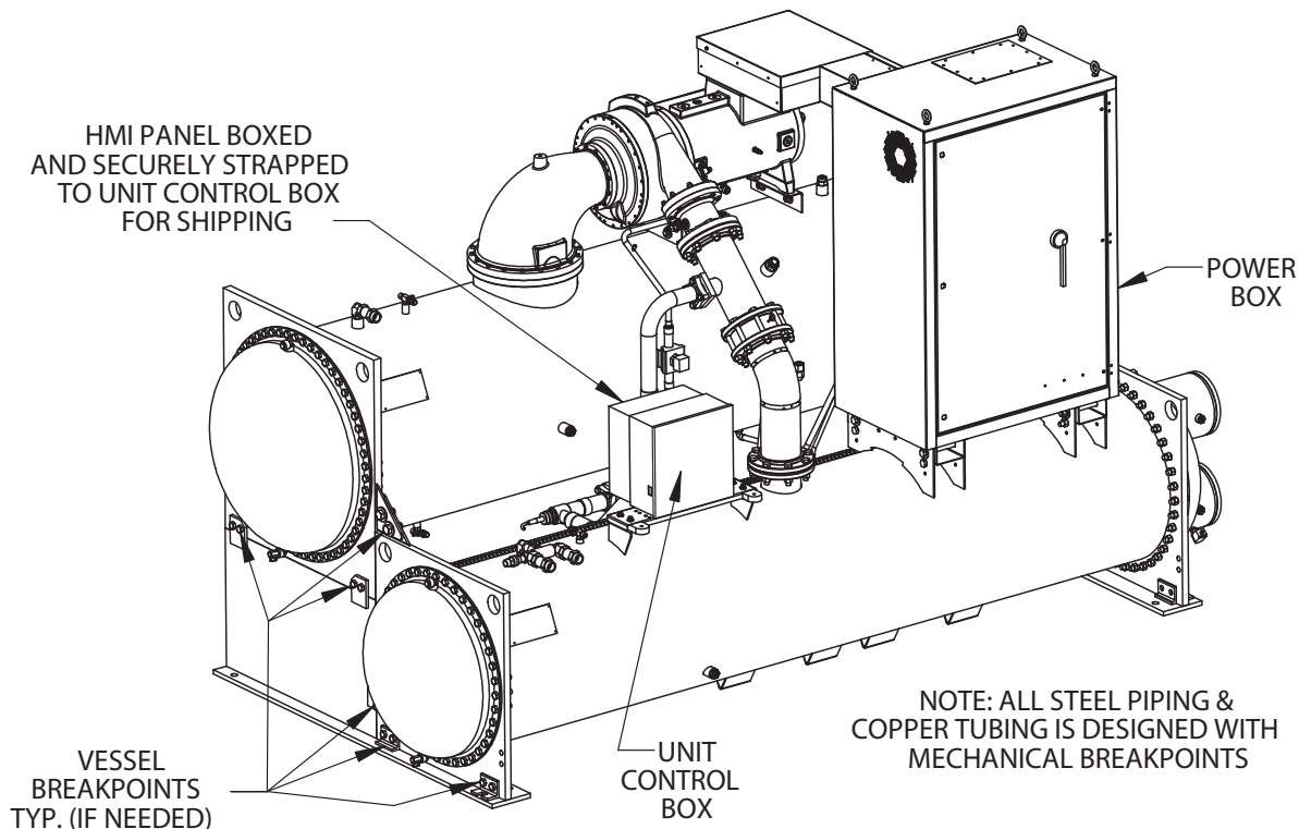
Figure 6: “Bolt-Together Construction” - Representative Illustration
