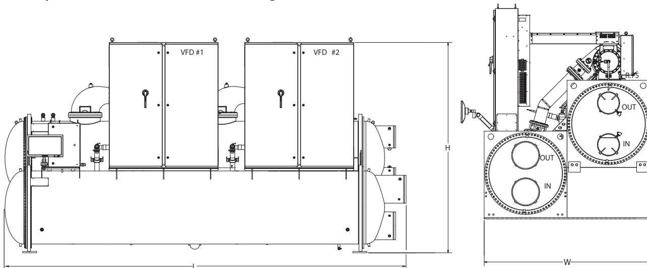
Figure 3: Representative WME Dimensional Drawing
