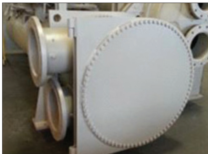
Figure 5: Marine Waterbox, Flanged Connections
