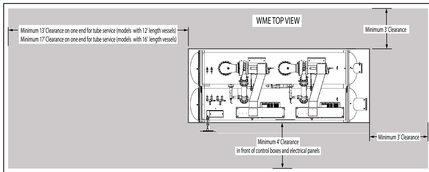
Figure 4: Minimum Clearances Based on Standard Waterboxes
