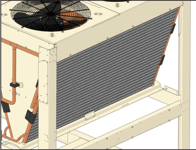
Figure 3: Microchannel Coil
