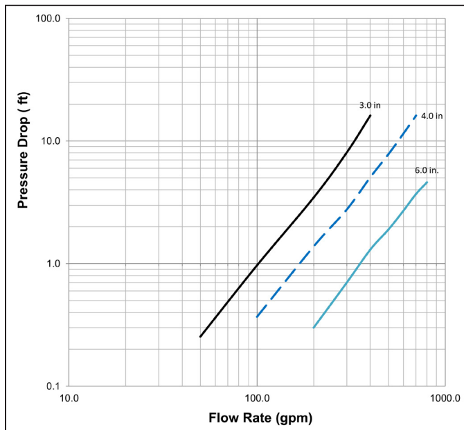
Figure 10: Strainer Pressure Drop
