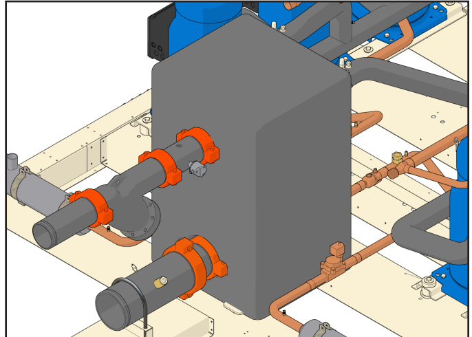
Figure 2: Brazed-Plate Evaporator
