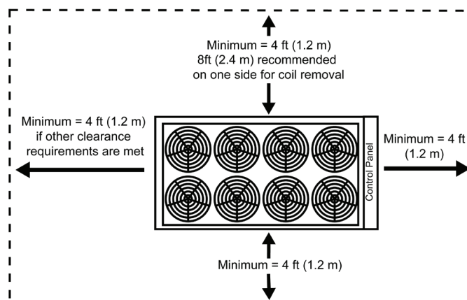
Figure 2: Service Clearance
