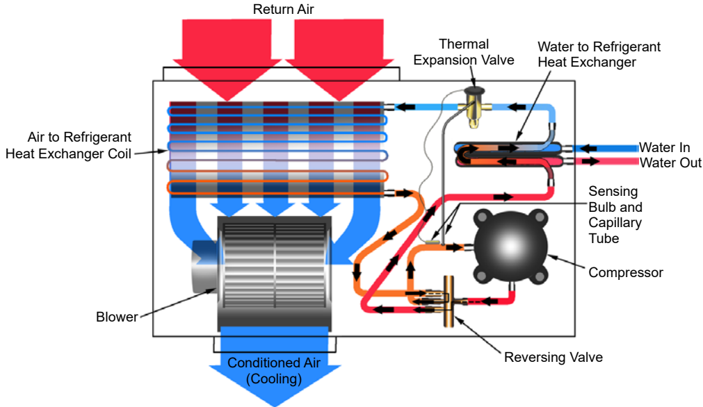
Figure 14: Heating refrigeration cycle
