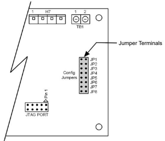
Figure 12: I/O expansion module configuration jumper terminals
