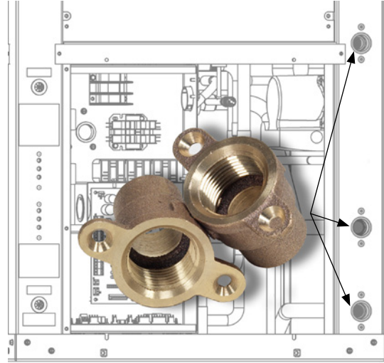
Figure 4: Flush FPT water fittings
