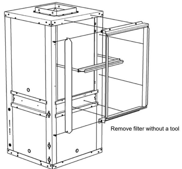
Figure 1: Optional 2" or 4" filter rack
