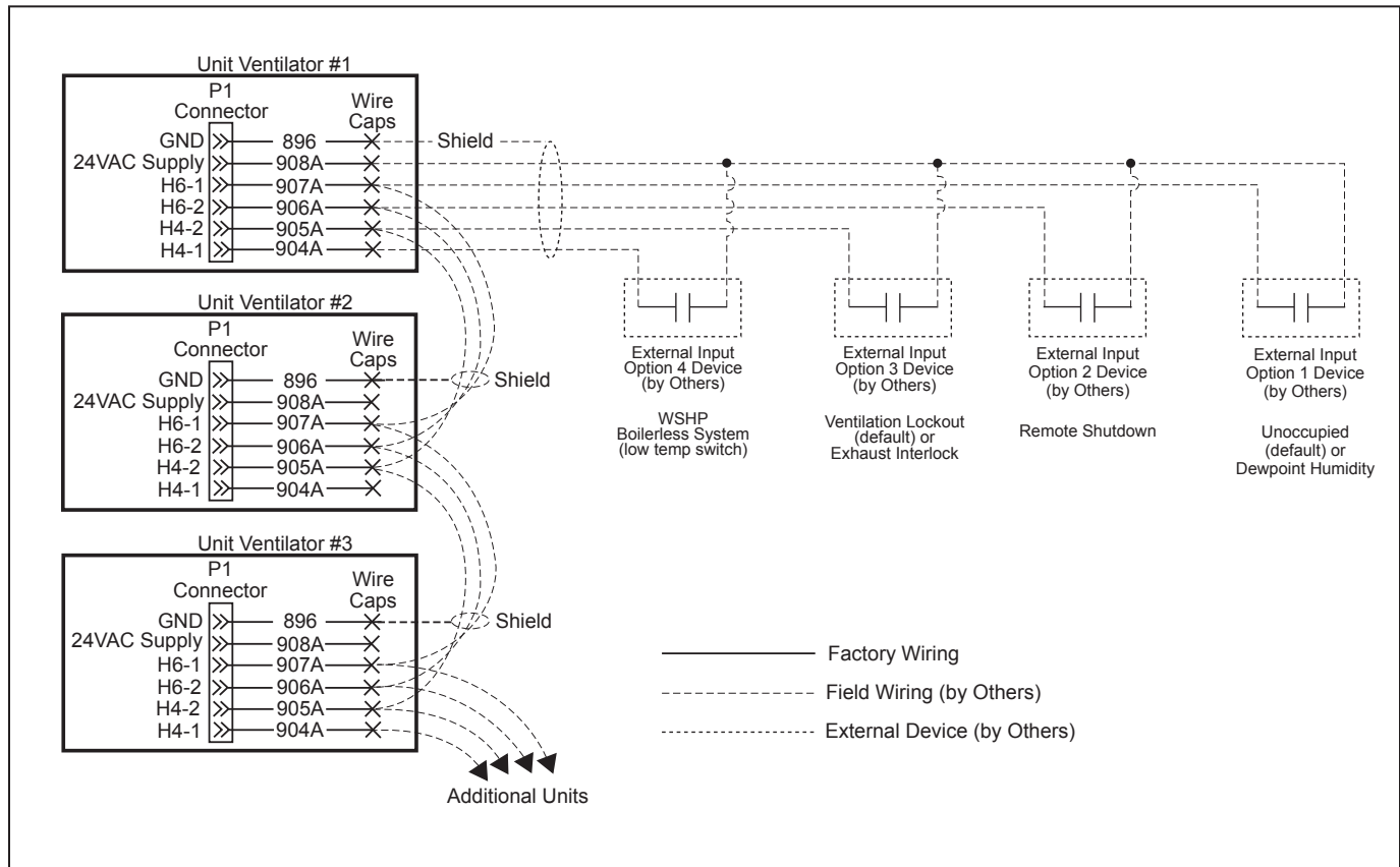
Figure 93: External Input Wiring Examples with or without Daisy Chaining of Units
