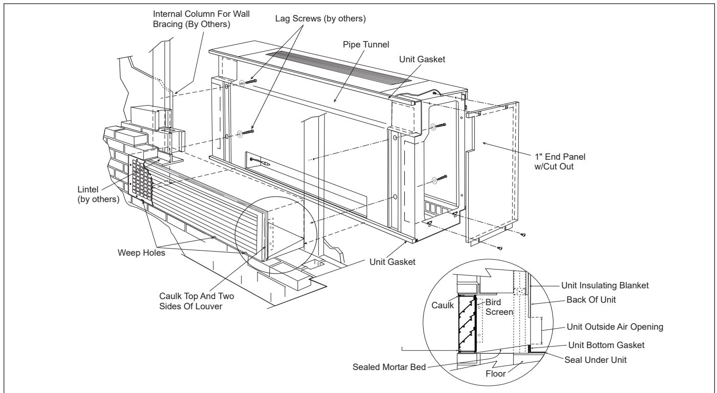
Figure 120: Recessed Wall Louver Installation Detail
