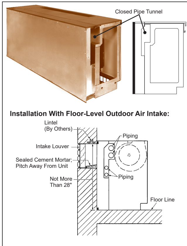
Figure 25: Arrangement AB
