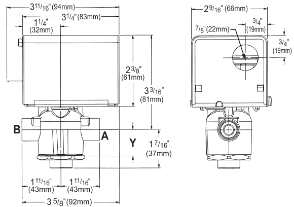
Figure 79: 3-Way EOC Valve Dimensions
