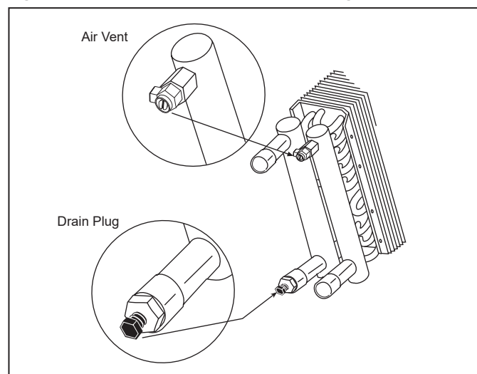
Figure 112: Manual Air Vent and Drain Plug
