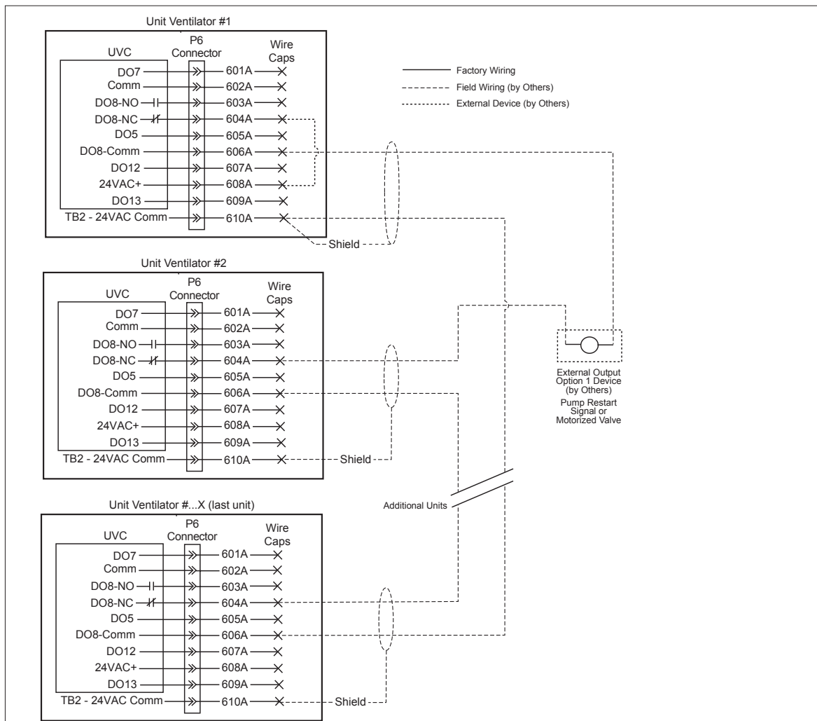
Figure 95: External Output Wiring - Multiple Units Shown
