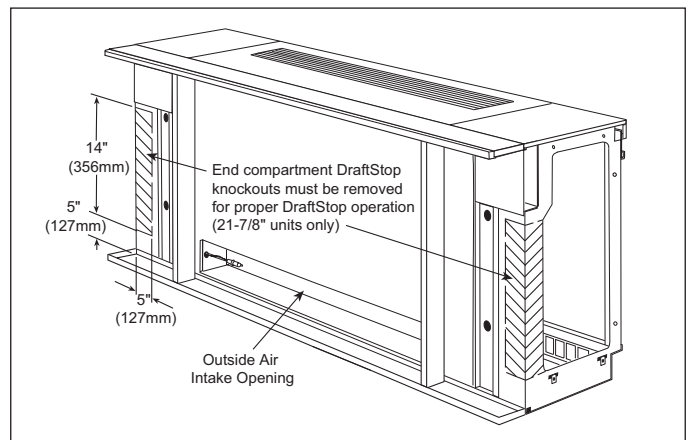
Figure 124: DraftStop Knockouts
