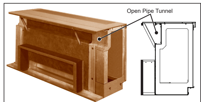
Figure 22: Arrangement AK
