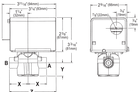
Figure 78: 2-Way EOC Valve Dimensions
