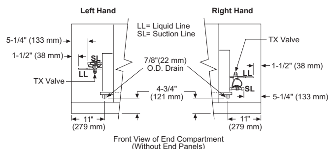
Figure 76: Condensate Drain and DX Coil Connections
