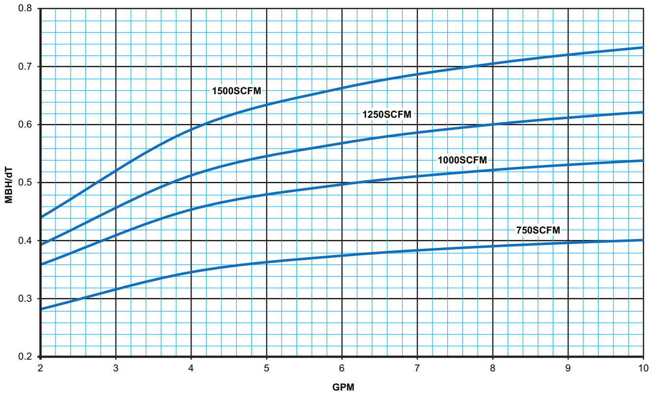
Figure 86: 2-Row Hot Water Coil (Parallel Flow)
