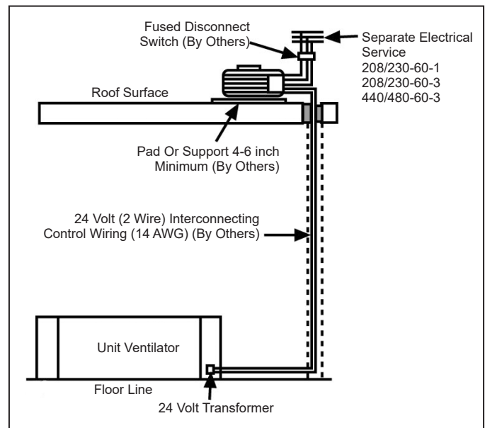
Figure 113: Typical DX System Wiring
