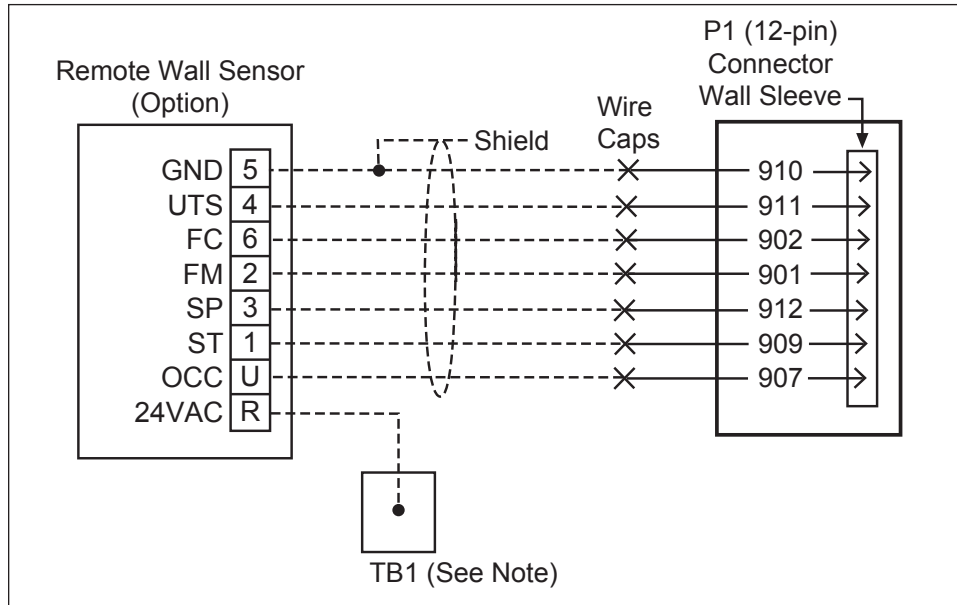
Figure 92: Wall-Mounted Temperature Sensor Wiring
