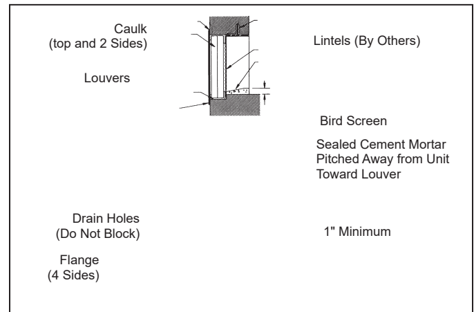
Figure 118: Flanged Wall Louver Installation Detail
