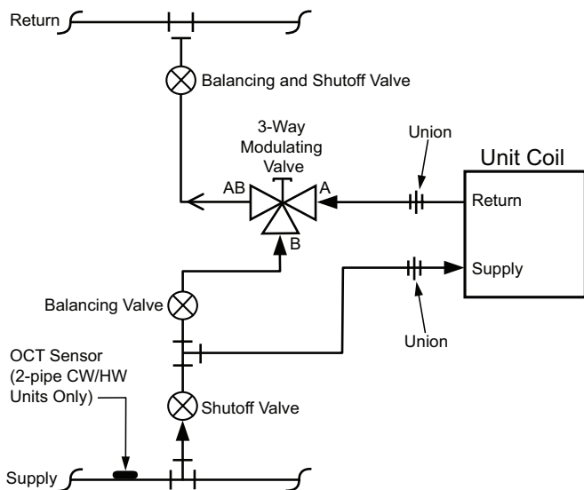
Figure 131: 3-Way Hot Water Modulating Valve Piping
