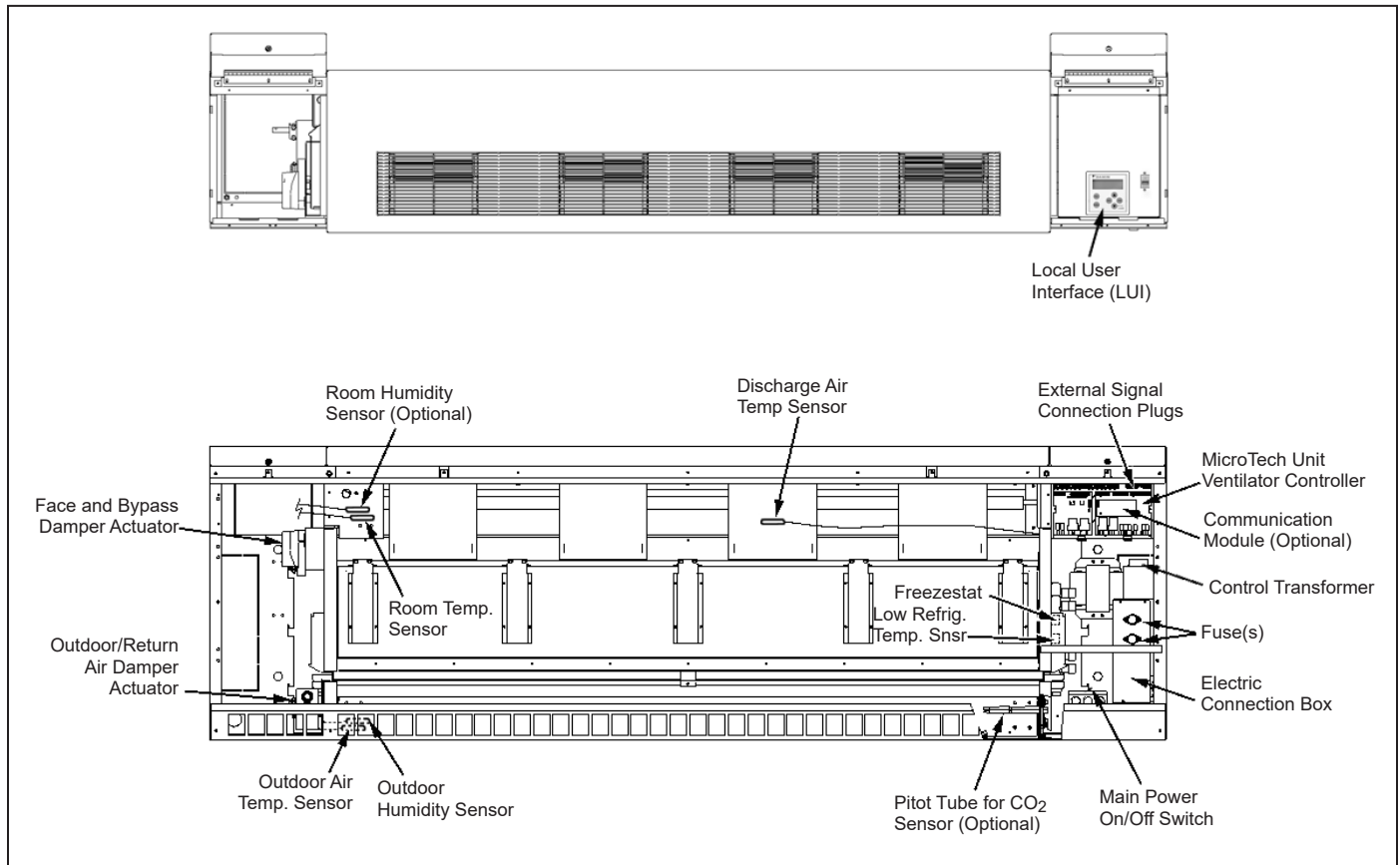
Figure 103: MicroTech Sensor and Component Locations
