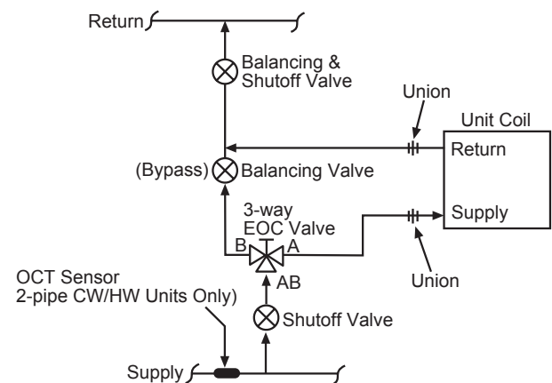
Figure 127: 3-Way Hot Water EOC Valve Piping
