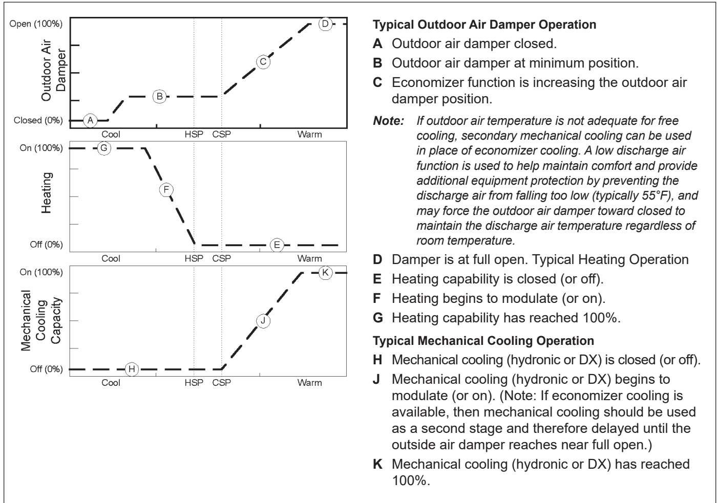
Figure 116: ASHRAE Cycle II Operation
