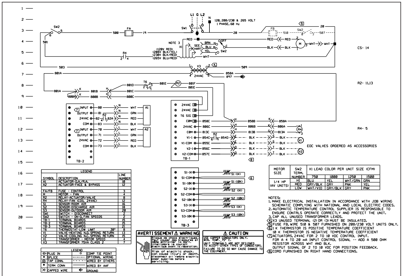
Figure 97: AV Digital Ready, Face and Bypass, Hydronic
