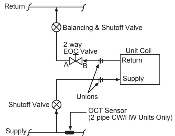
Figure 126: 2-Way Hot Water EOC Valve Piping
