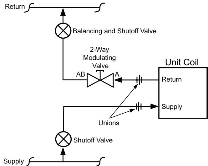
Figure 132: 2-Way Chilled Water Modulating Valve Piping
