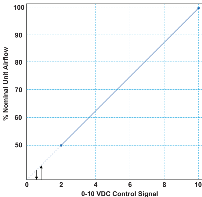
Figure 115: 0-10VDC Motor Operation
