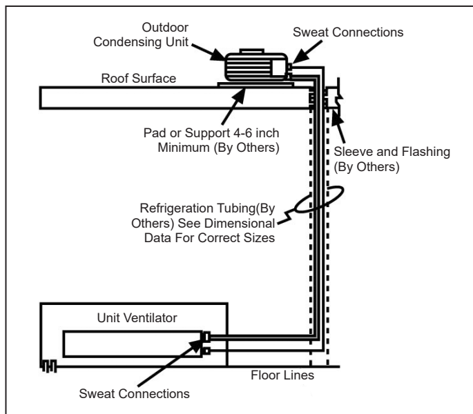
Figure 114: Typical DX System Piping
