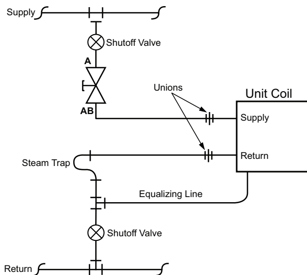
Figure 135: 2-Way Steam Modulating Valve Piping
