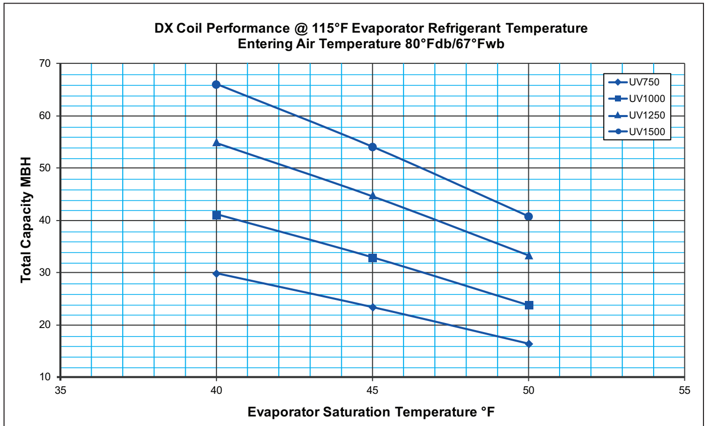
Figure 89: 2" DX Coil Estimated Performance (Mbh at 115°F Liquid Temperature)
