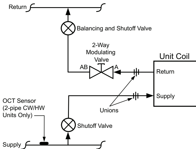
Figure 130: 2-Way Hot Water Modulating Valve Piping
