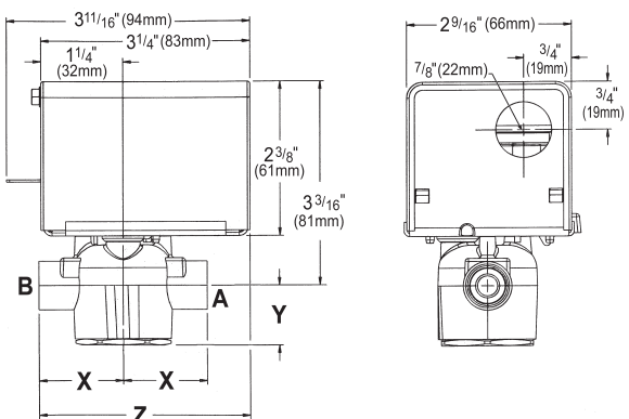
Figure 80: 2-Way EOC Steam Valve Dimensions
