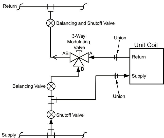
Figure 133: 3-Way Chilled Water Modulating Valve Piping
