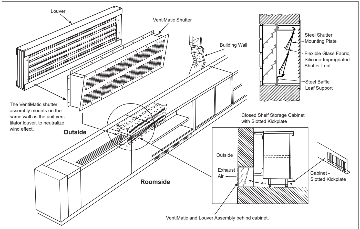
Figure 122: VentiMatic Shutter Installation
