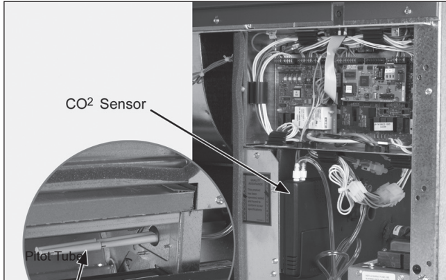
Figure 104: CO 2 Sensor For Demand Control Ventilation
