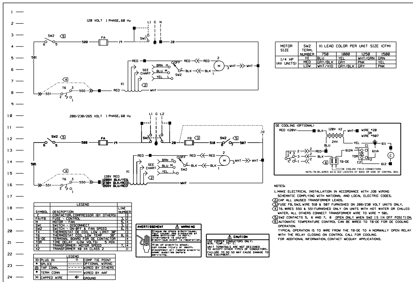
Figure 98: Typical Wiring Diagram for Units with Controls by Others
