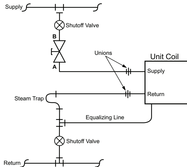
Figure 134: 2-Way Steam End of Cycle Valve Piping
