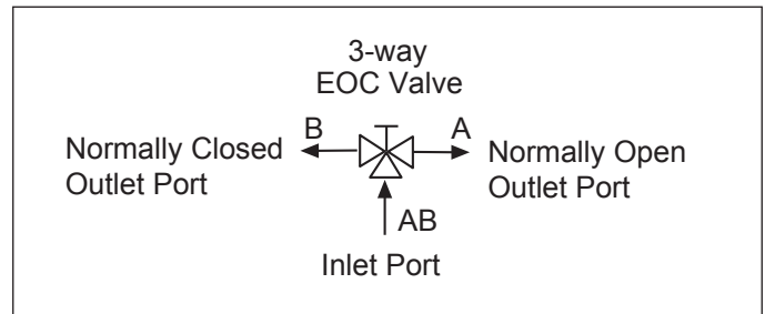
Figure 125: 3-Way Valve Piping Connections
