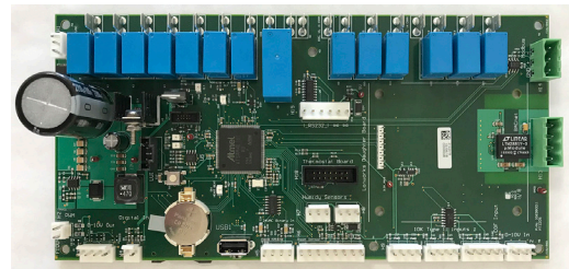
Figure 101: MicroTech Control Board
