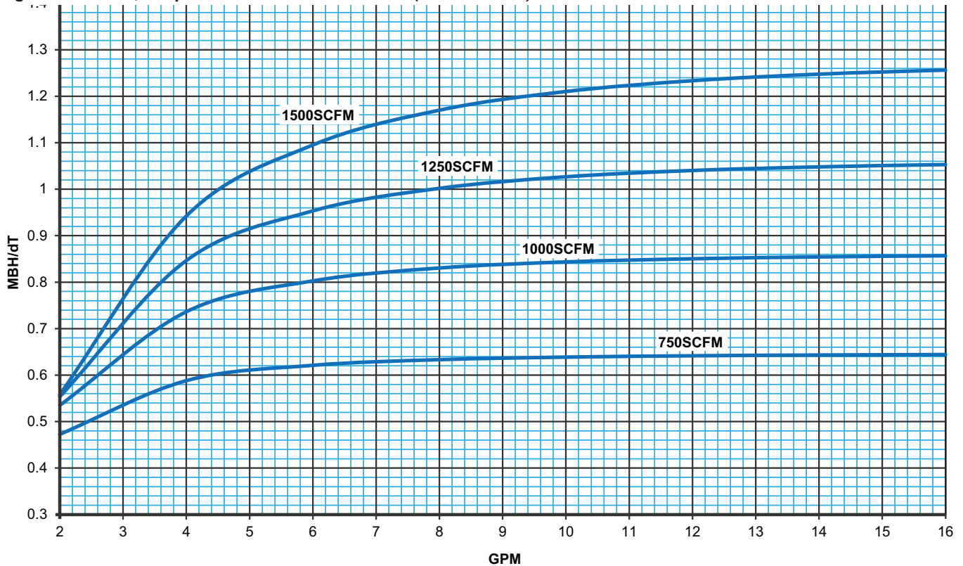
Figure 88: 4-Row, 2-Pipe Cold Water/Hot Water Coil (Counter Flow)
