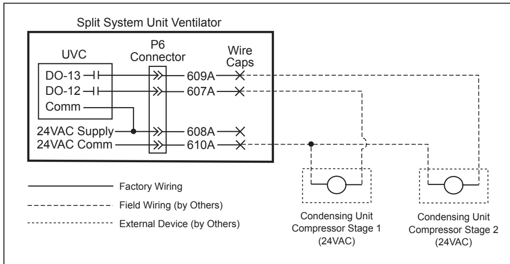
Figure 96: Split-System Condensing Unit Signal Wiring
