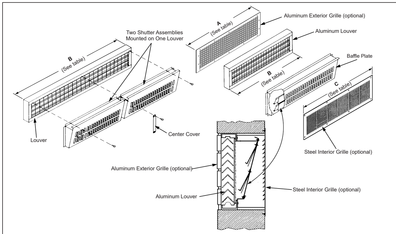
Figure 84: VentiMatic Shutter Assembly with Optional Grille
