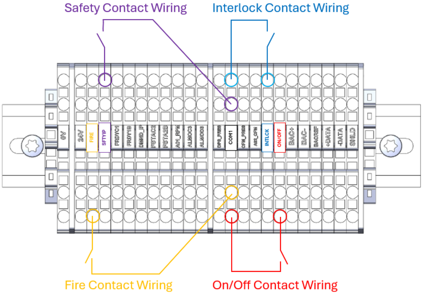
Figure 11: Field Control Wiring Diagram
