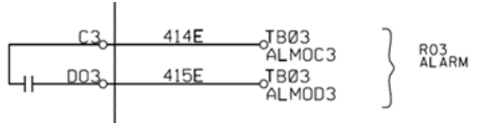
Figure 16: Alarm Output Schematic
