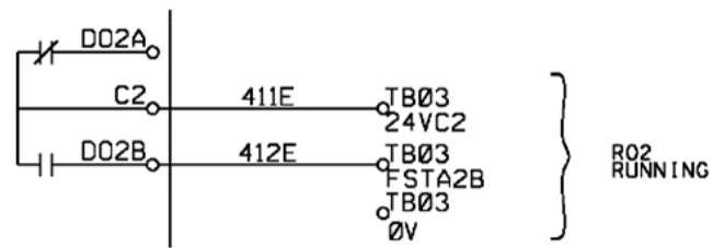
Figure 15: Running Relay Schematic
