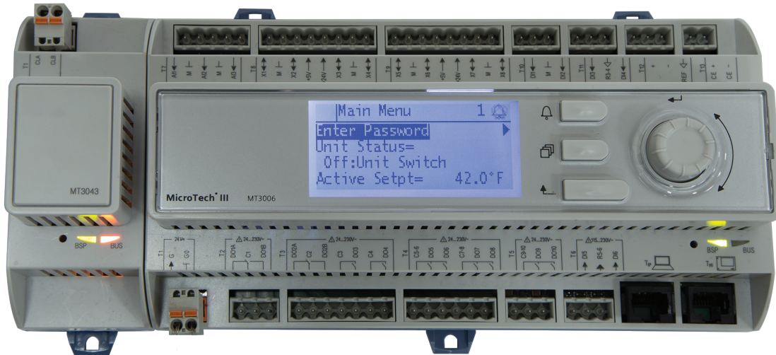
Figure 3: LonWorks Communication Module Attached to Unit Controller (MicroTech III controller shown)
