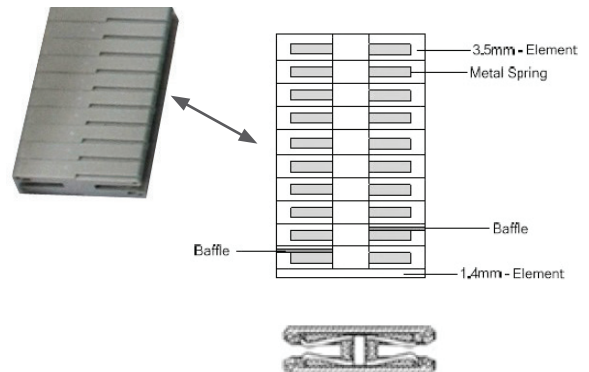
Figure 6: Board-to-Board Connector
