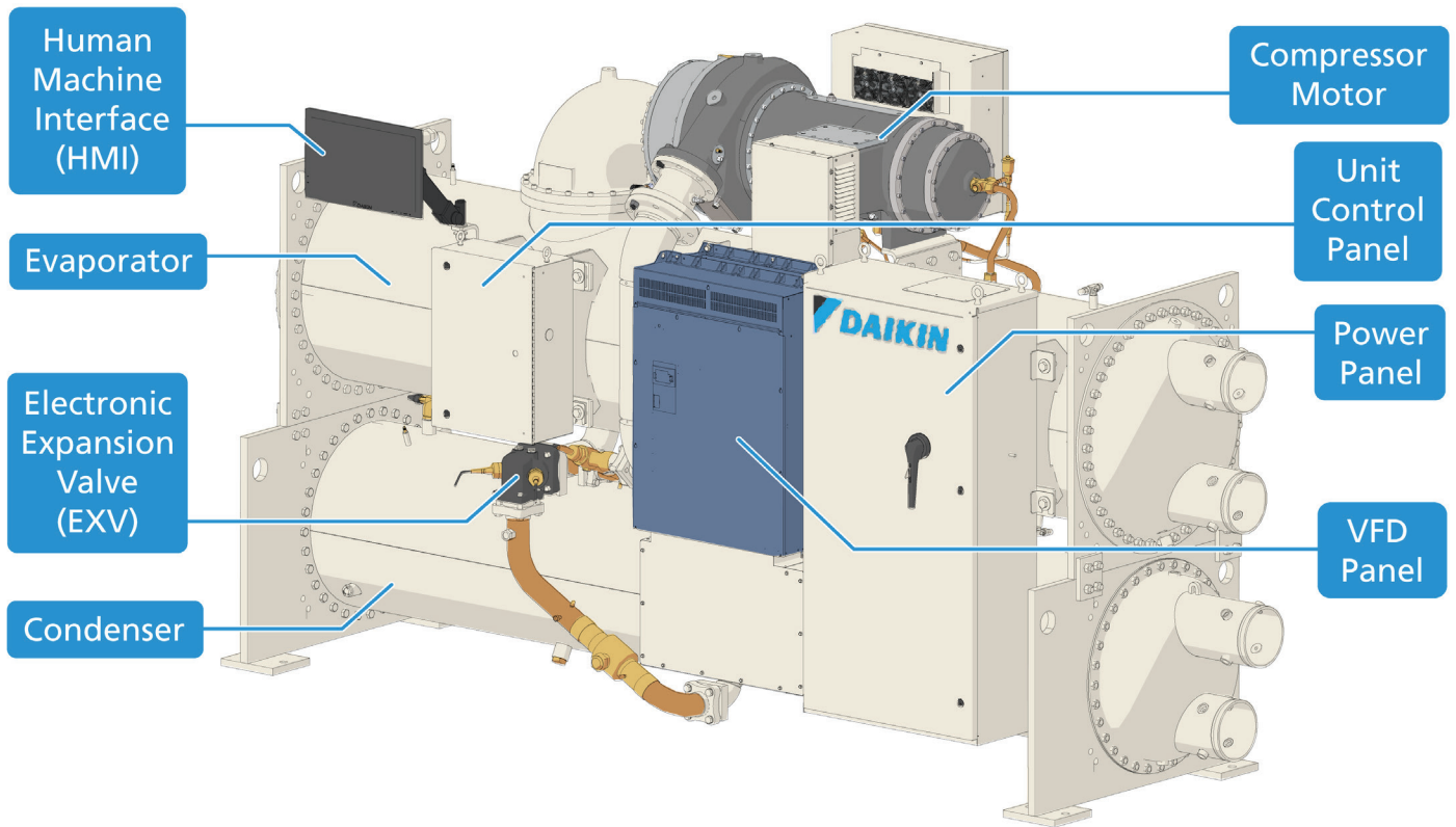
Figure 1: WME-D Major Component Locations
