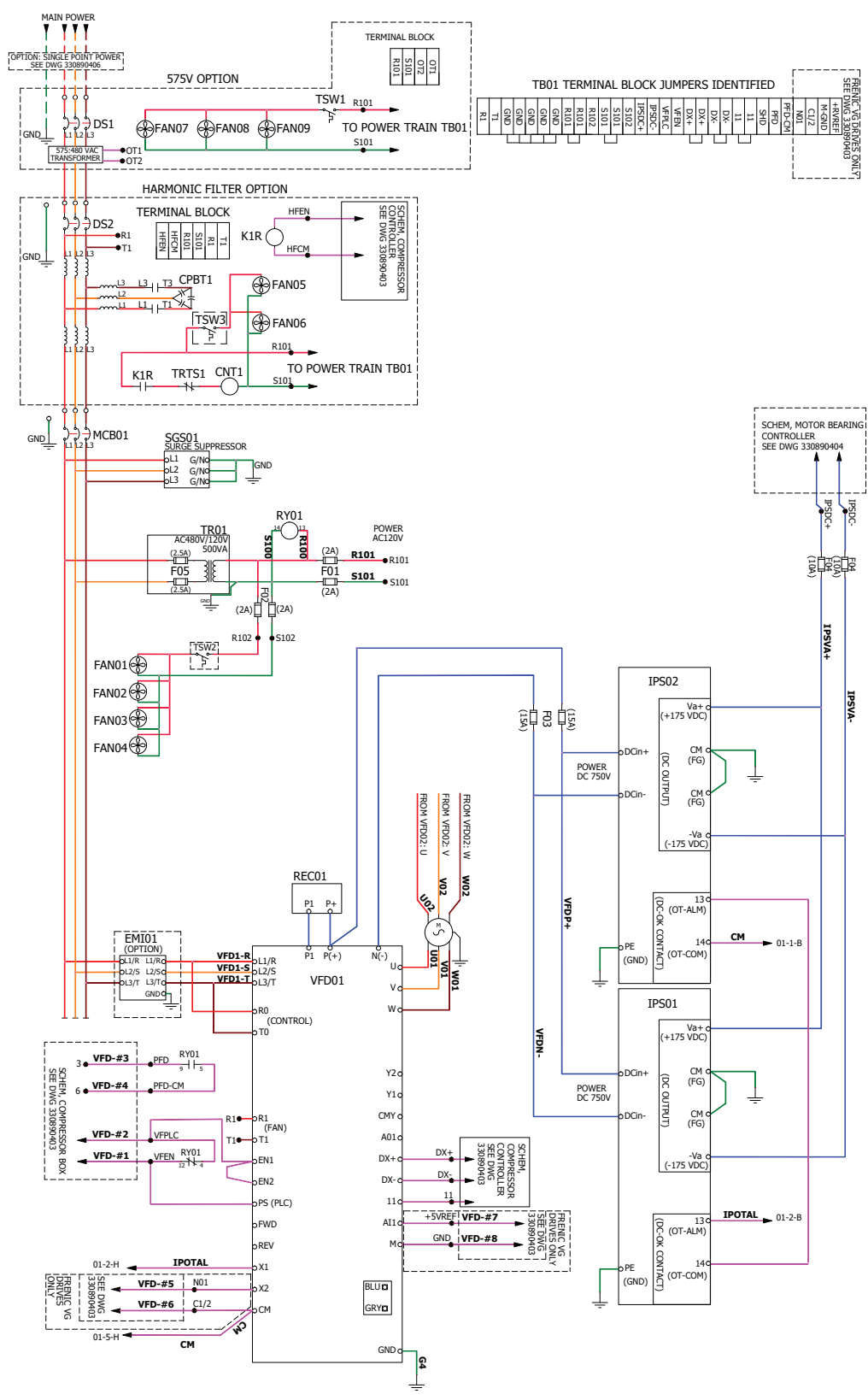
Figure 11: Power Train Schematic
