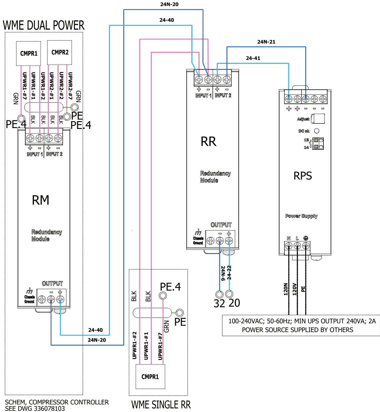
Figure 8: Power Cable Configuration (RapidRestore Option)
