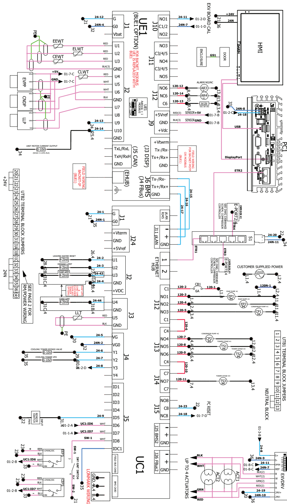
Figure 6: WME-D Unit Schematic
