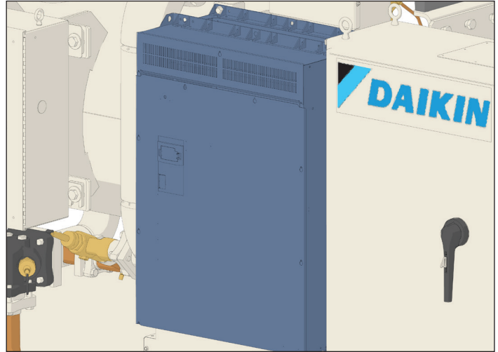
Figure 3: Unit-Mounted VFD
