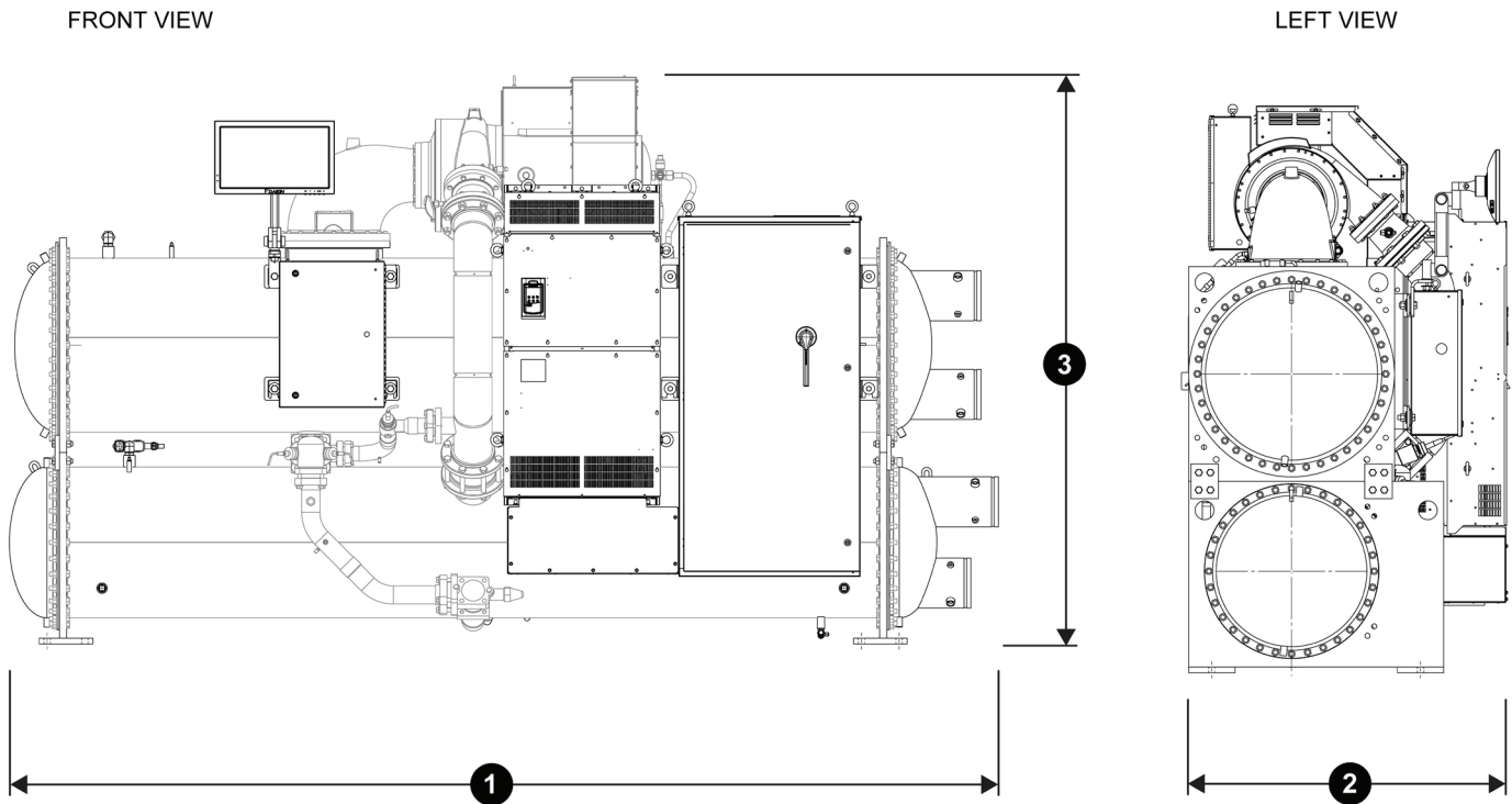
Figure 13: Representative WME-D Dimensional Drawing
