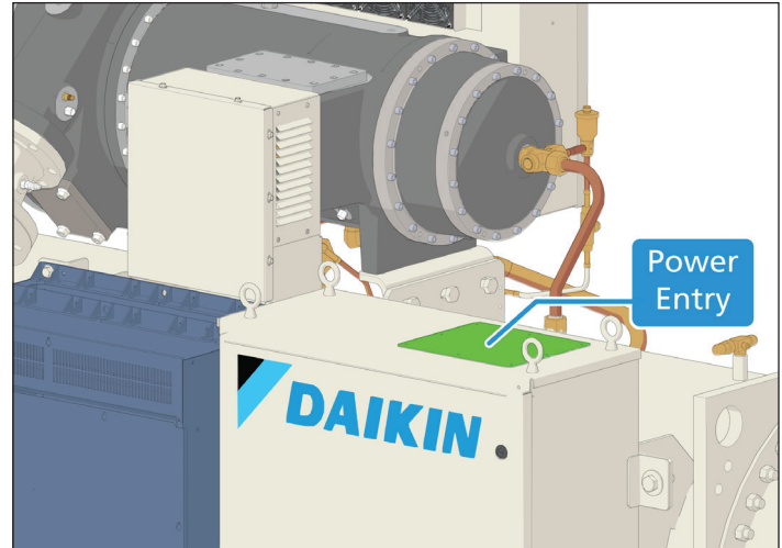
Figure 4: Unit Power Connection Point
