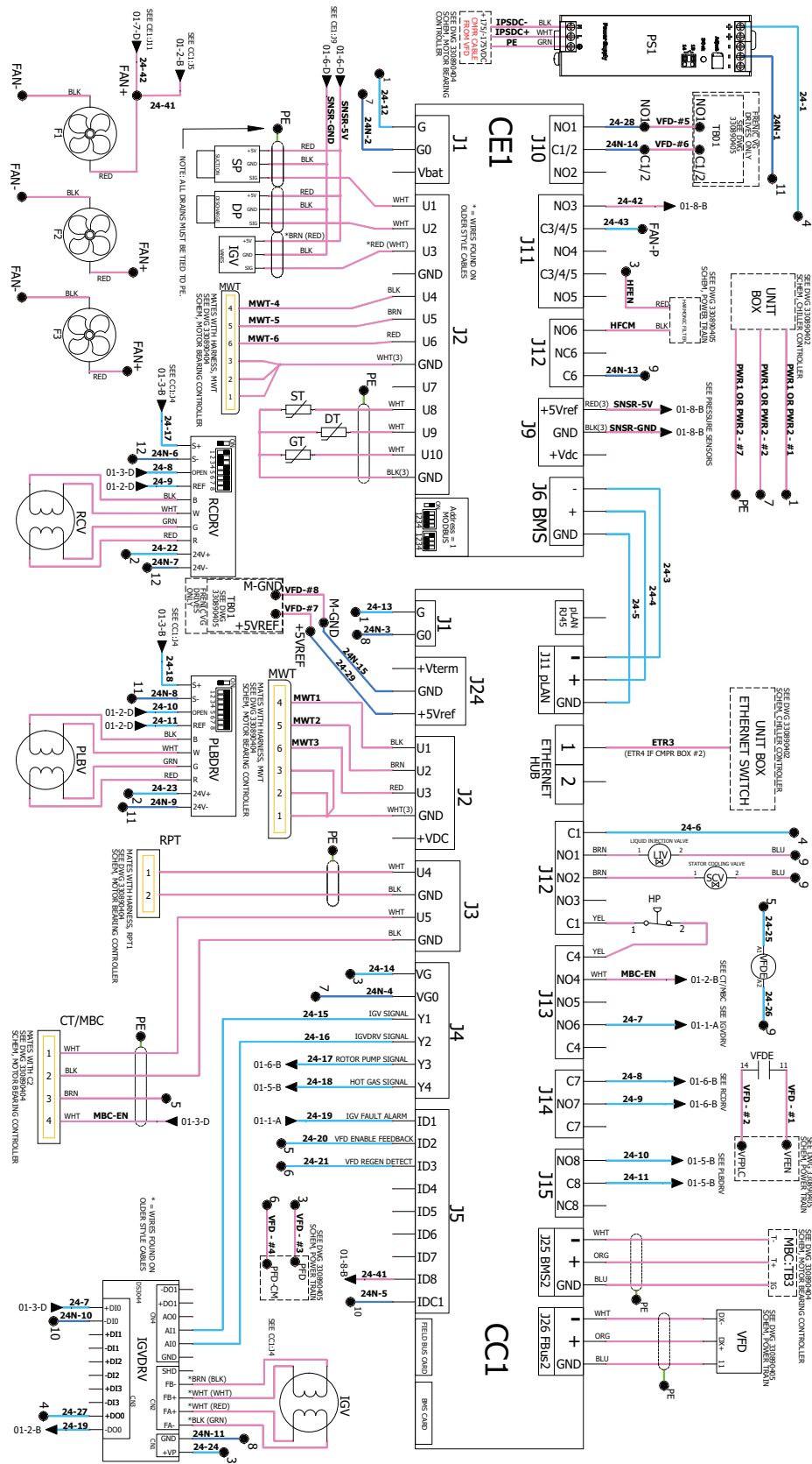
Figure 9: WME-D Compressor Schematic
