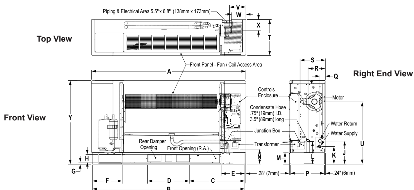
Figure 29: Flat Top – High Sill, Right Hand Piping – Unit Size 015 - 018
