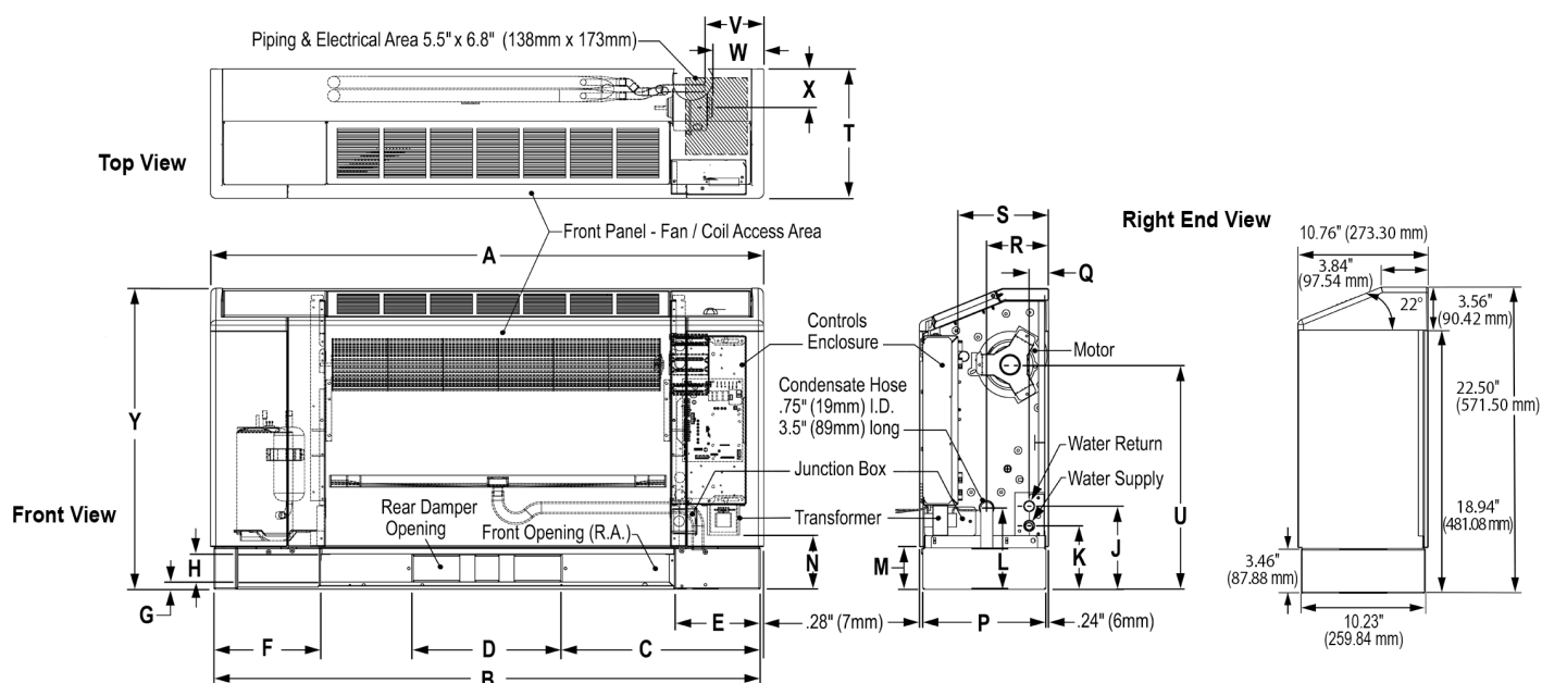
Figure 37: Slope Top – High Sill, Right Hand Piping – Unit Size 015 - 018
