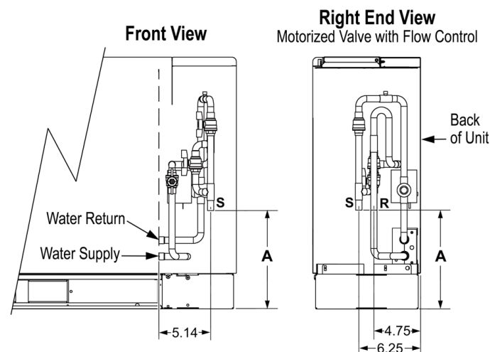
Figure 13: Right-Hand, Motorized Valve with Manual Valves
