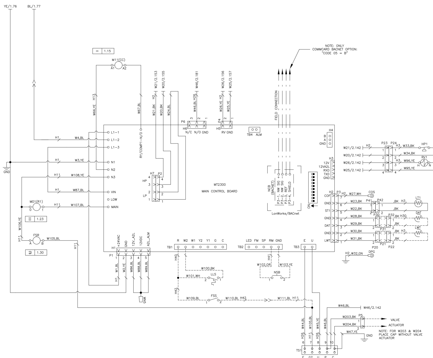
Figure 23: MicroTech Unit Control with Wall Mounted Room Temperature Sensor - 265 Volt
