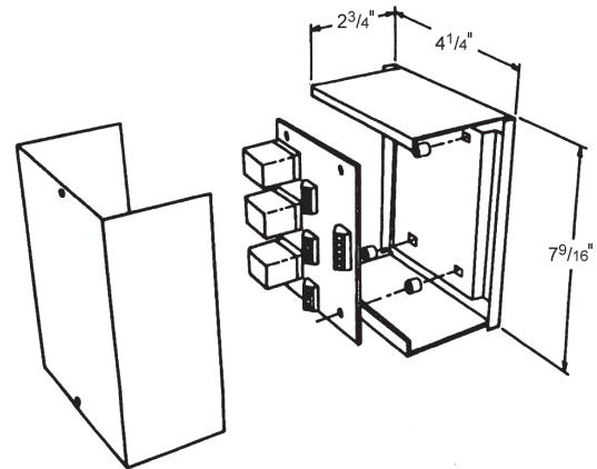
Figure 3: Multiple Unit Control Panel and Board
