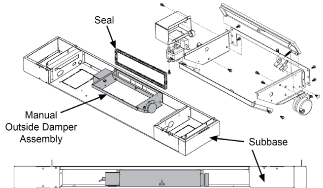
Figure 16: Motorized Outdoor Air Damper
