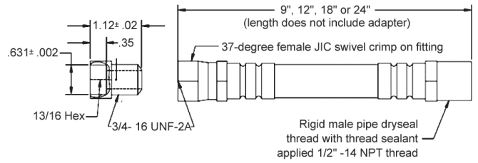
Figure 6: Hose Detail
