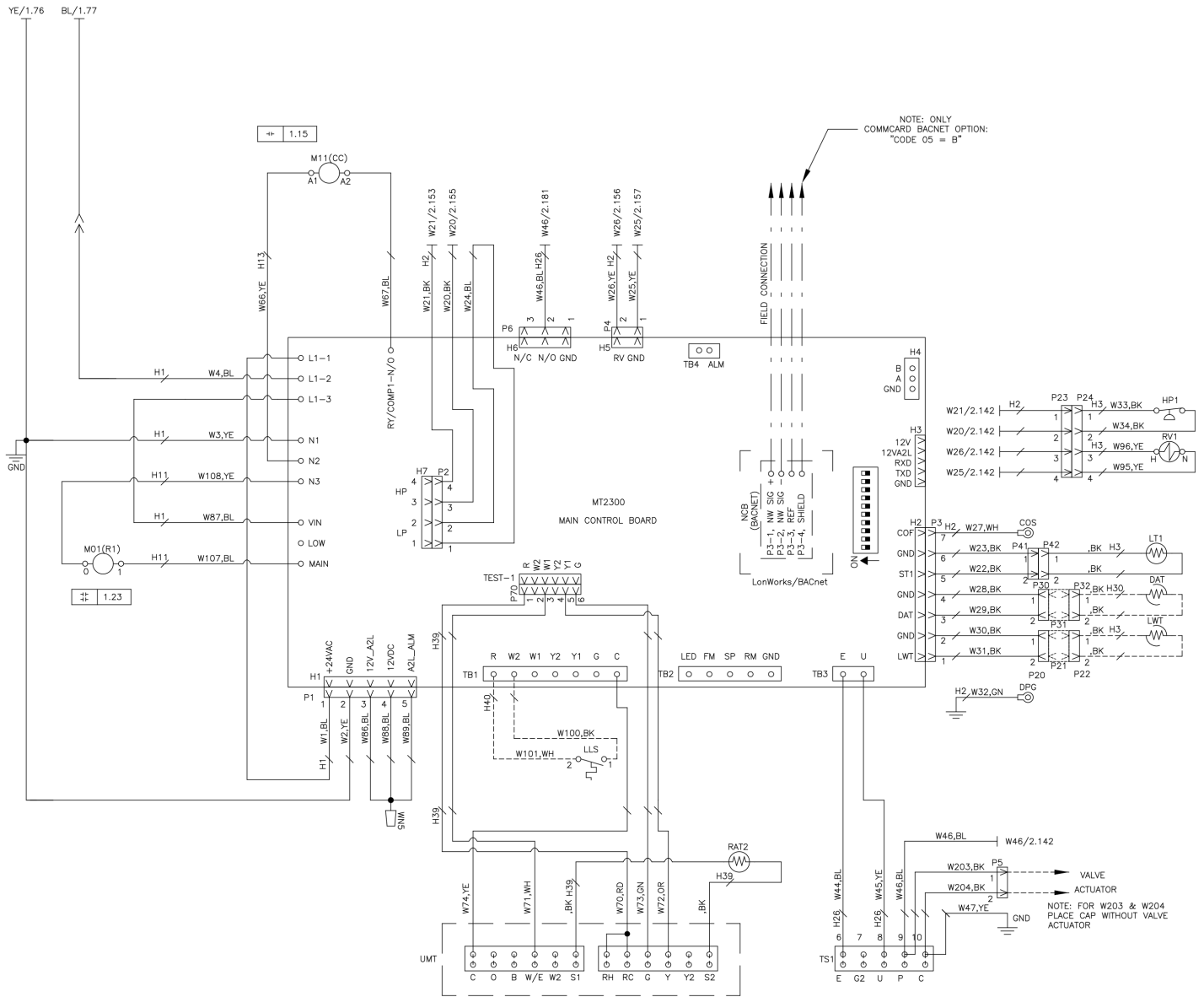
Figure 19: MicroTech Unit Control Without Electric Heat - 208-230/60/1
