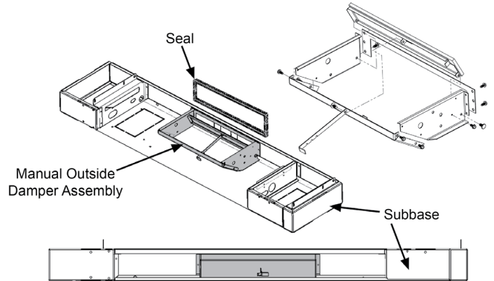
Figure 15: Manual Outdoor Air Damper
