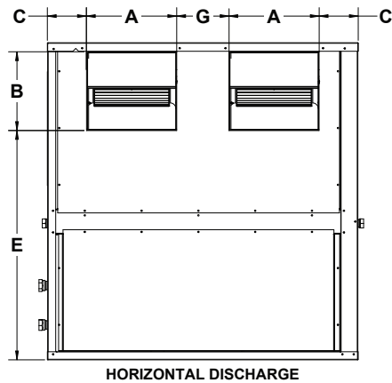
Figure 20: WSLV Discharge Air Dimensions
