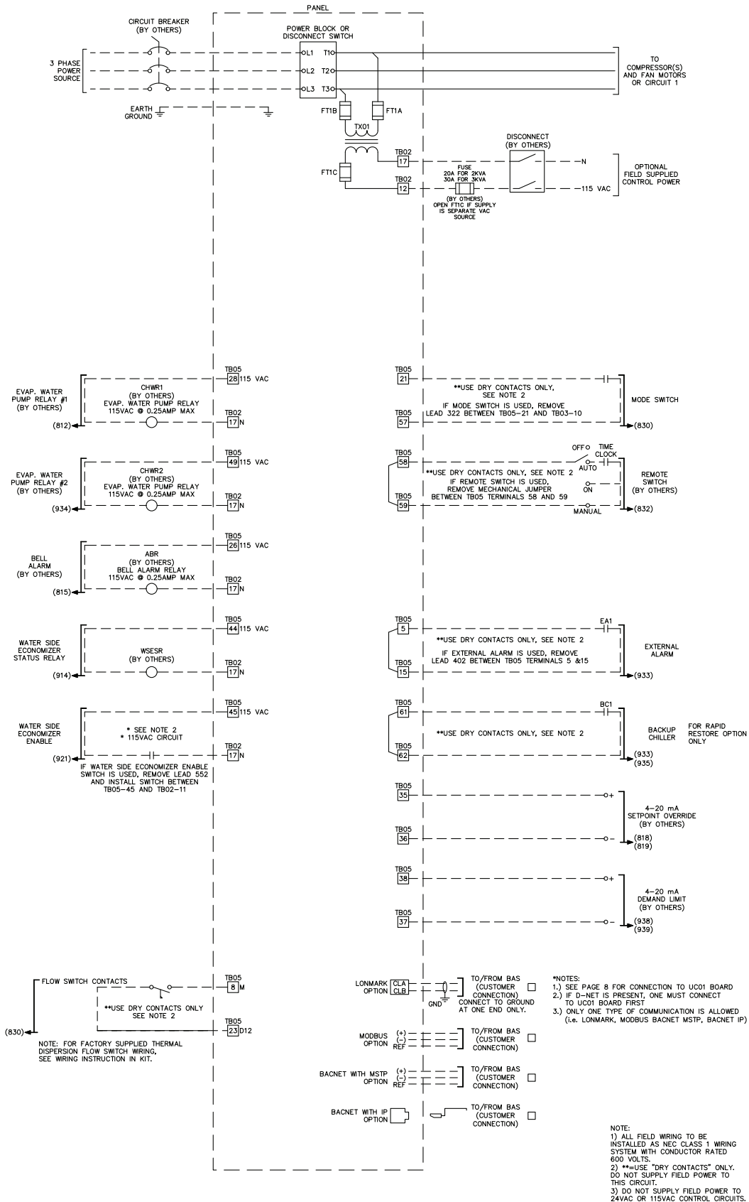
Figure 16: Field Wiring Diagram - Field
