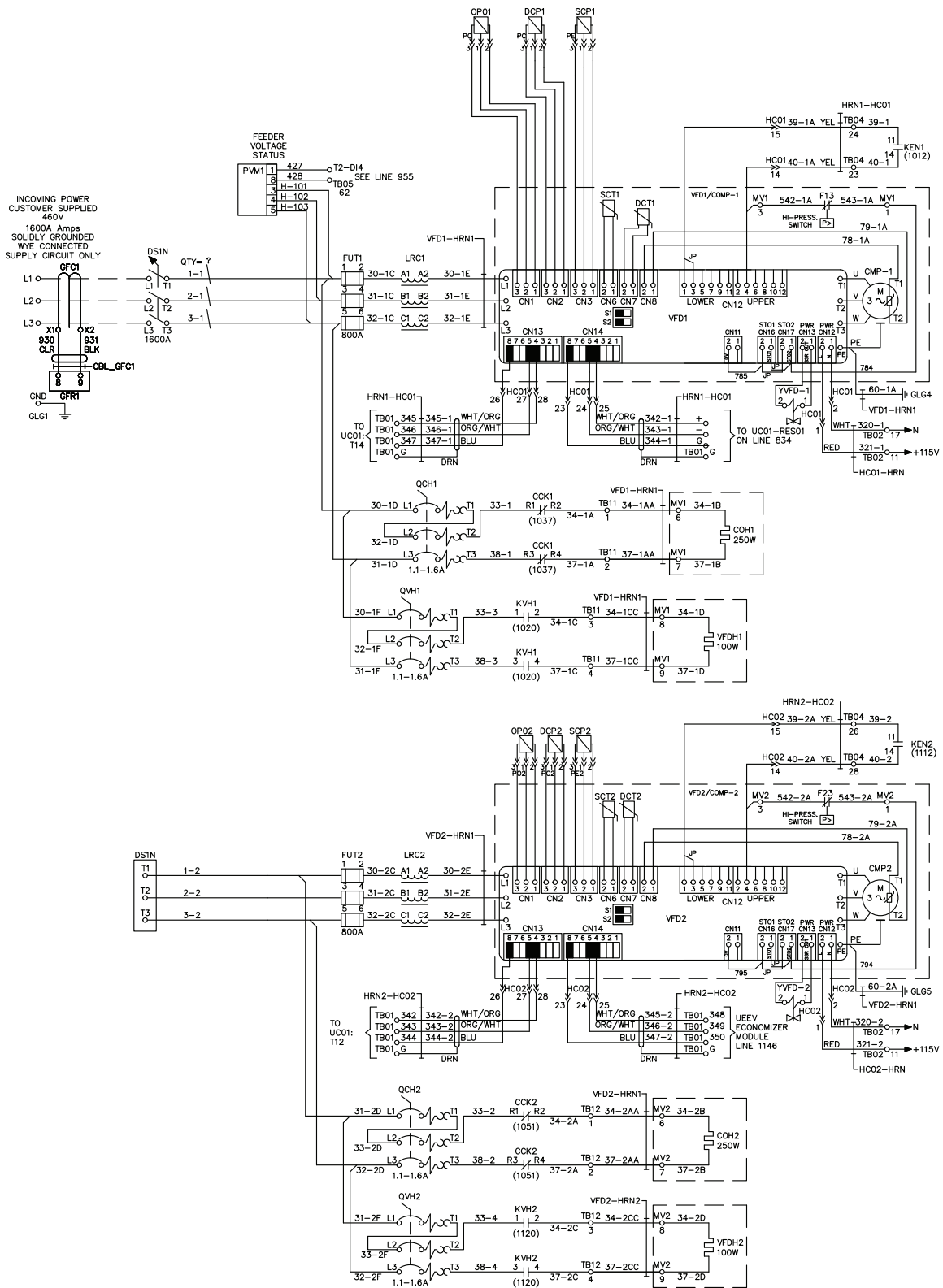
Figure 17: Power Schematic - Compressors
