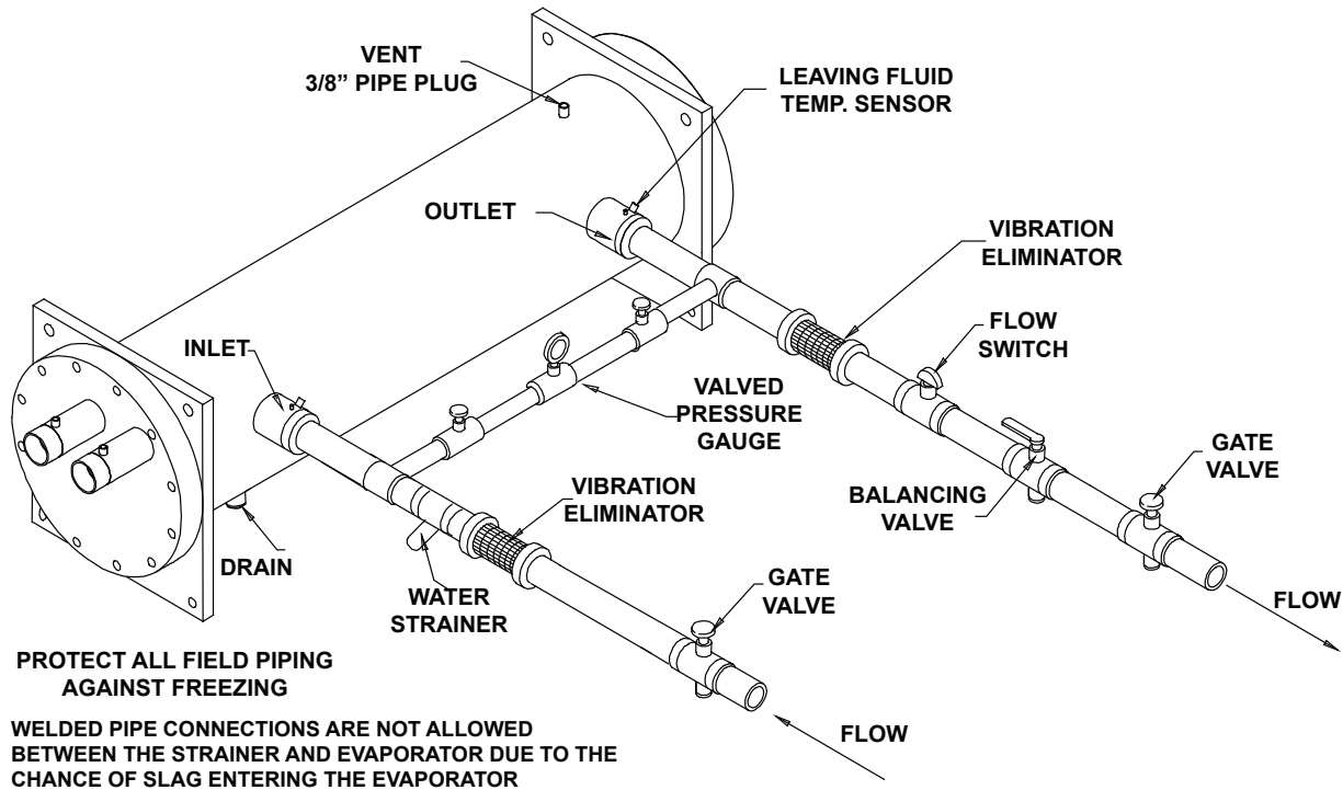
Figure 15: Typical Chilled Water Piping, Shell and Tube
