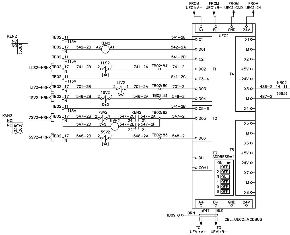
Figure 25: Expansion Control Board Schematic #2
