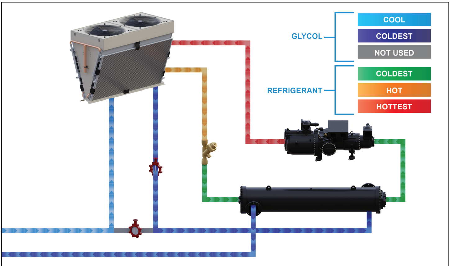
Figure 7: Hybrid Cooling Mode Operation
