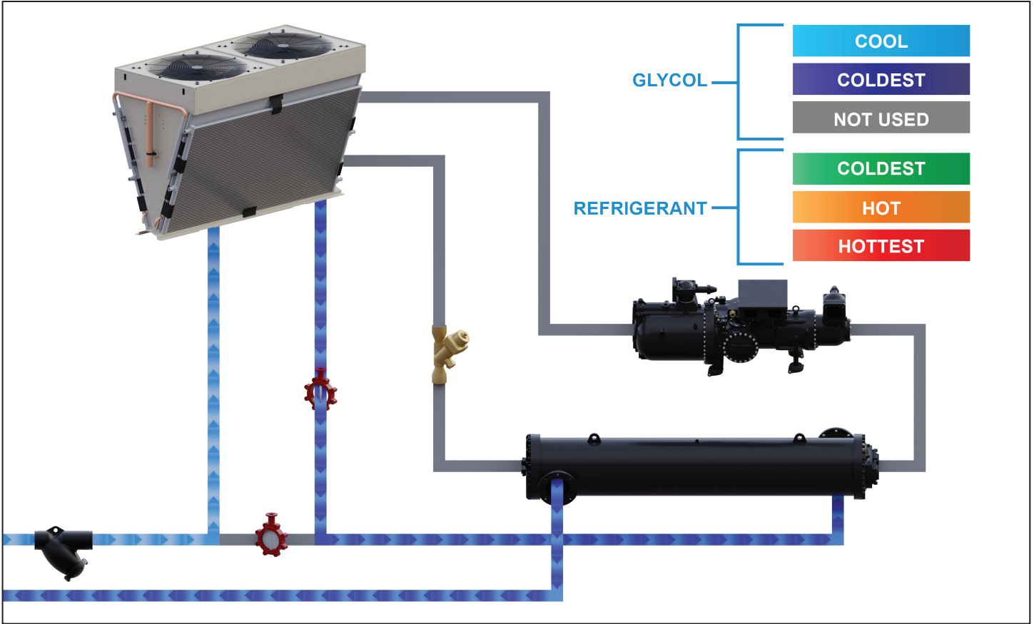
Figure 8: Integrated Waterside Economizer Operation
