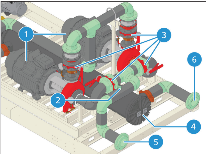
Figure 6: Dual Pump Package Standard Components
