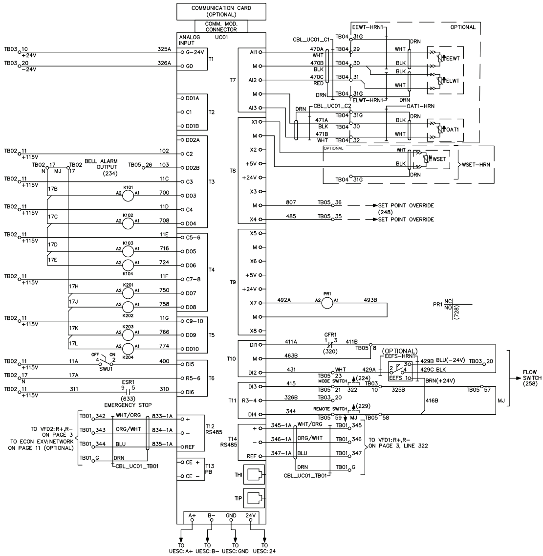
Figure 22: Main Control Board Schematic
