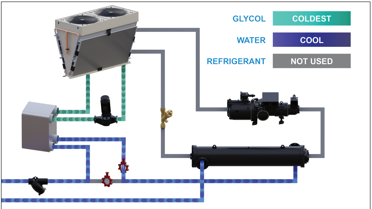
Figure 10: Closed Loop Waterside Economizer
