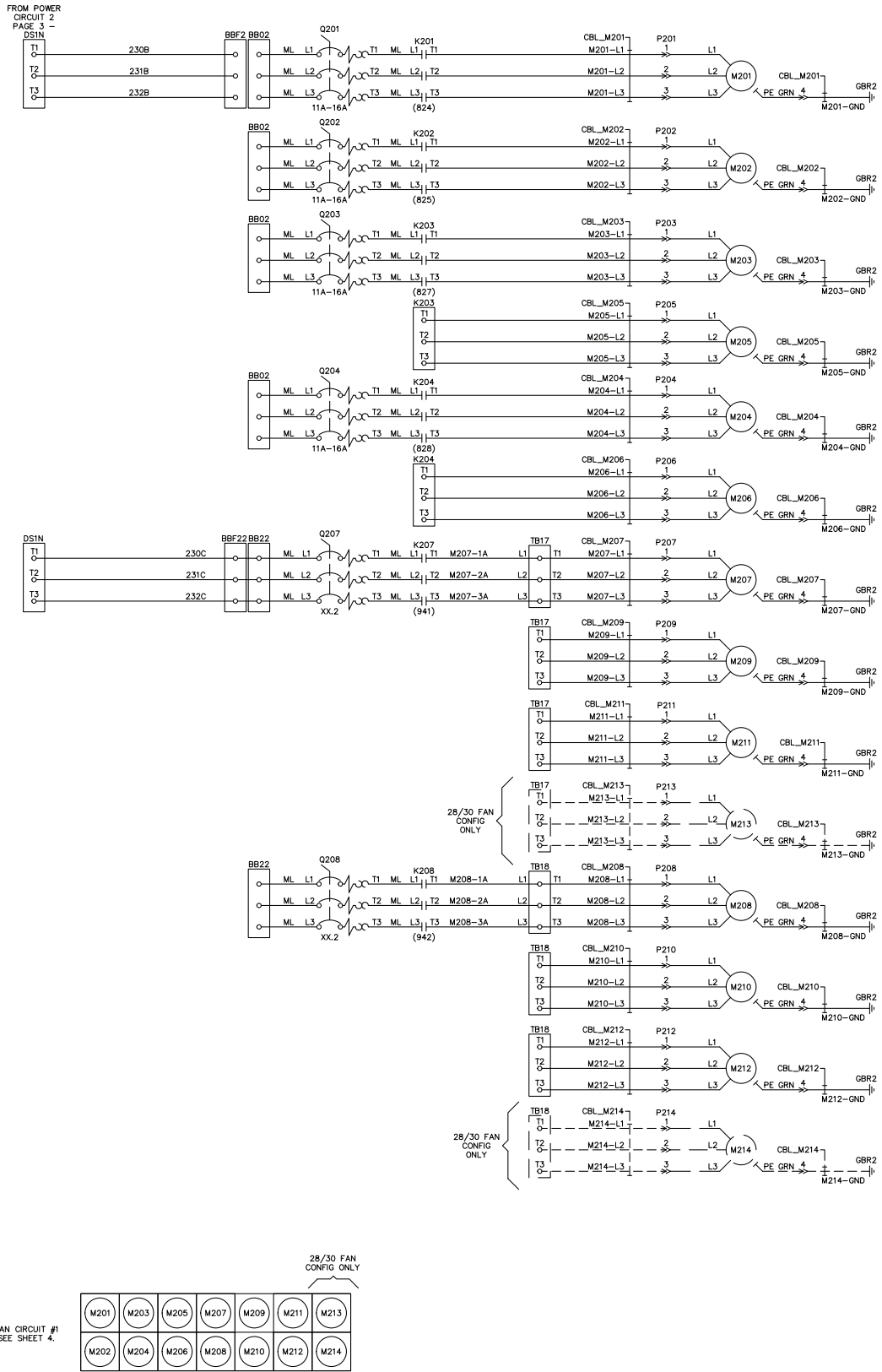
Figure 19: Power Schematic - Fan Circuit #2
