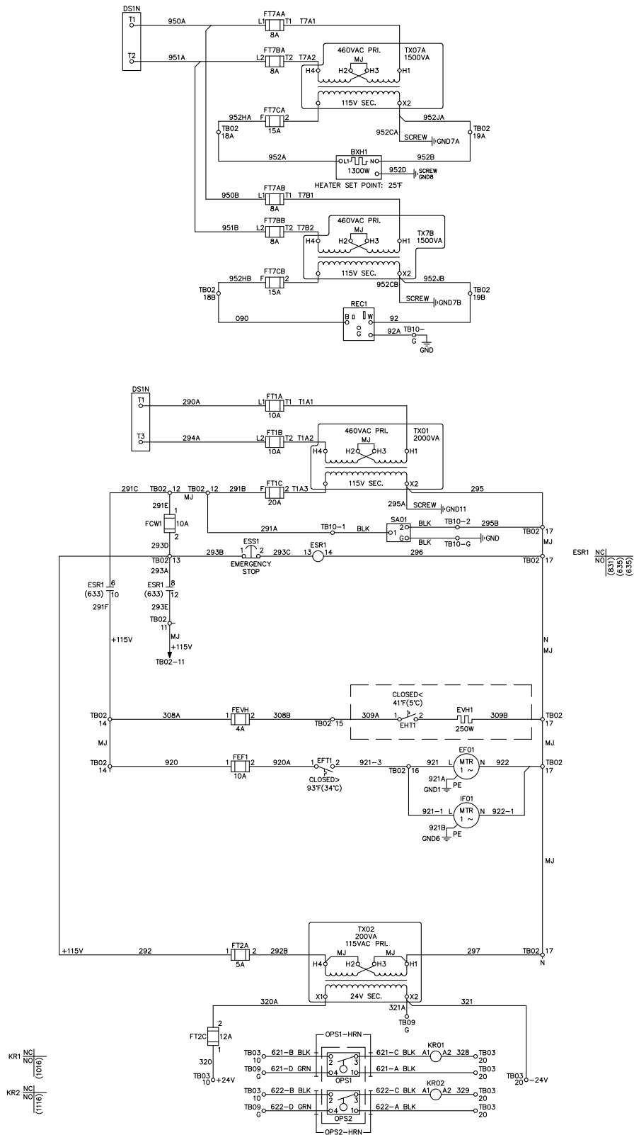
Figure 20: Low Voltage Schematic
