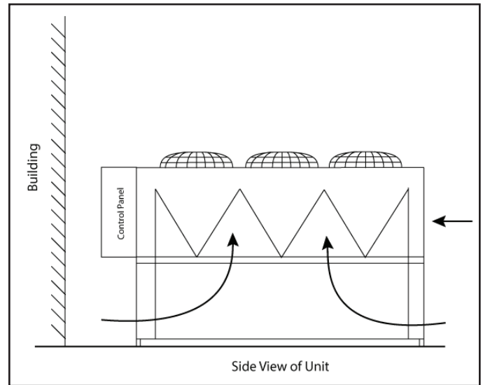
Figure 13: Representative Air Flow
