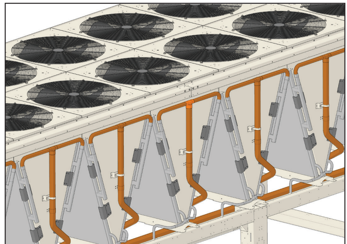
Figure 3: Shrouded Fan Assembly with Molded Blades
