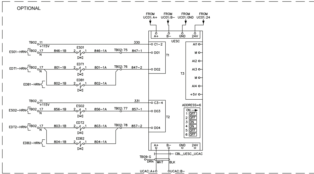
Figure 23: Expansion Control Board Schematic
