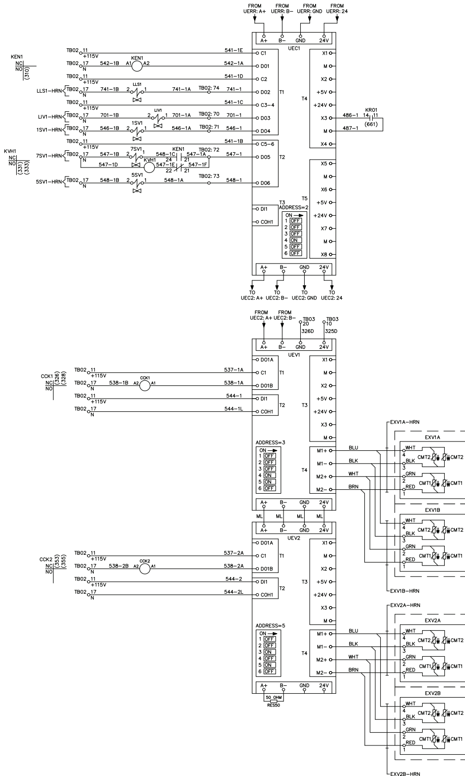
Figure 24: Expansion Control Board Schematic
