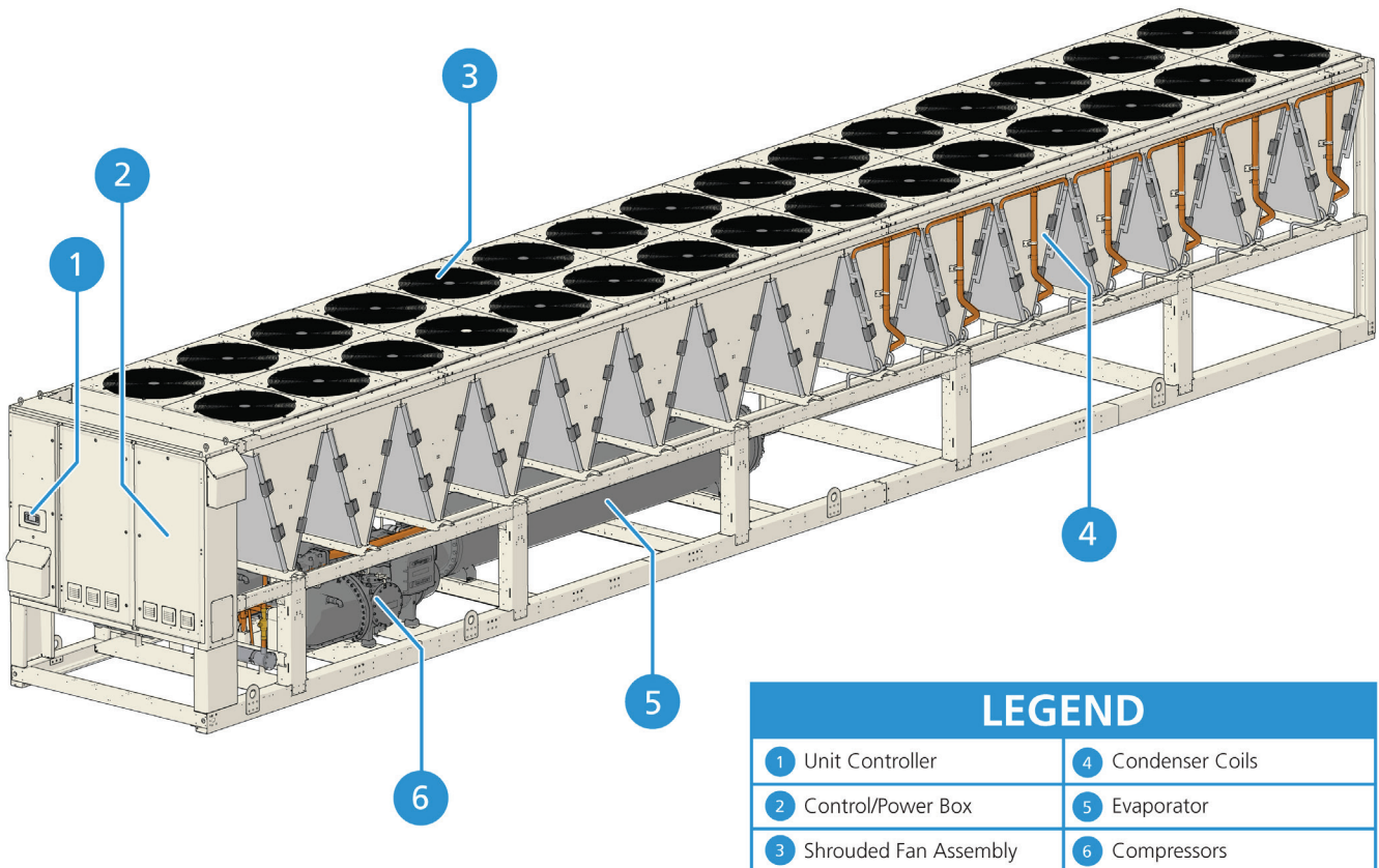
Figure 1: Pathfinder AWV-C Component Locations
