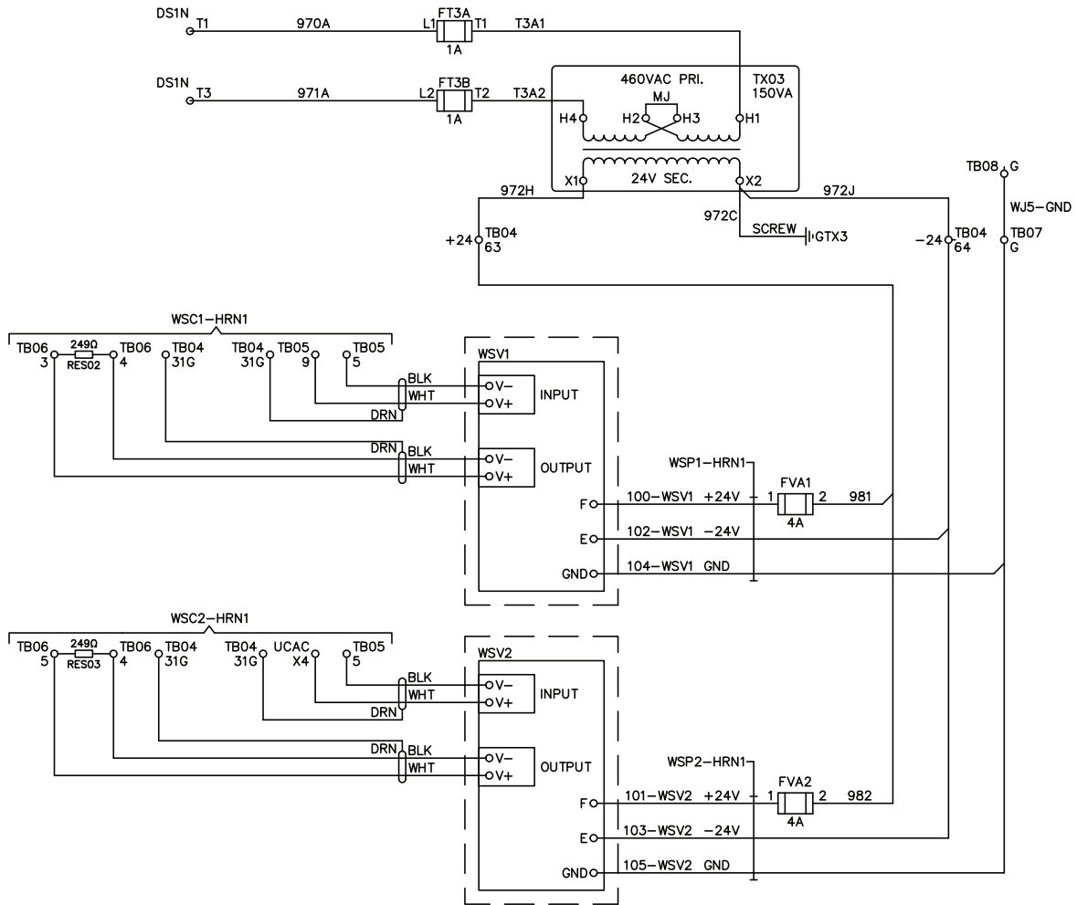
Figure 21: Optional IWSE Schematic (Open Loop)
