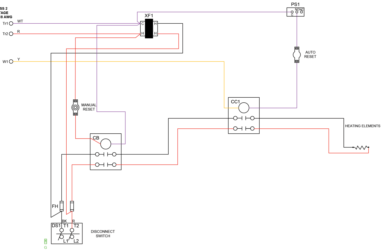
Figure 42: 208/240/408V, Fused Disconnect, Single Phase, 1 Stage EH
