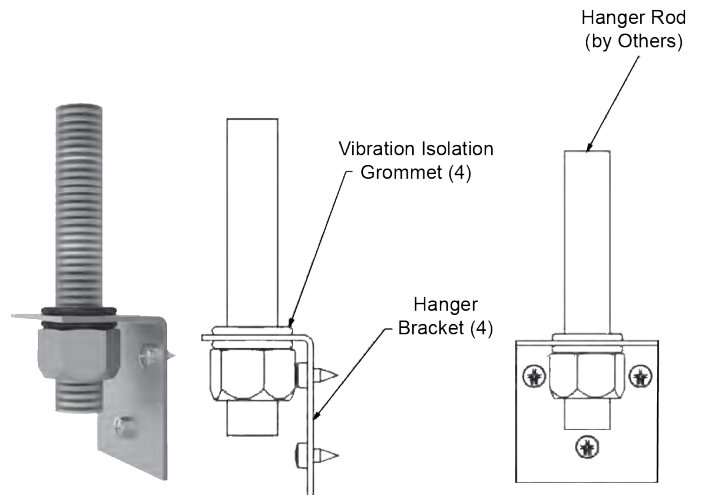
Figure 31: Hanger Brackets
