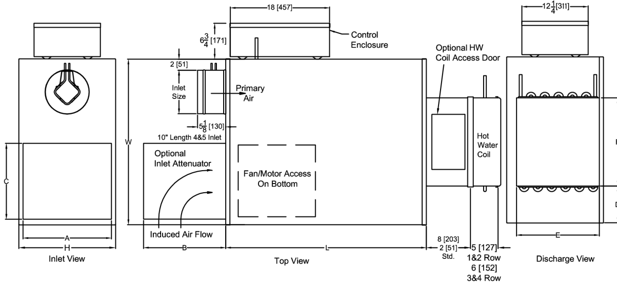
Figure 21: MQFVI-500 ECM Parallel Fan Powered Air Terminal Unit with Hot Water Coil Mounted on Discharge
