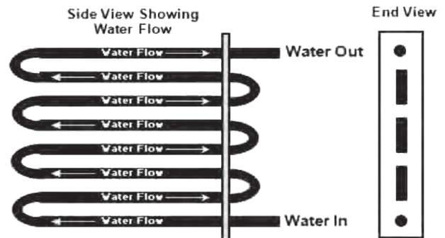
Figure 38: Coil Water Flow
