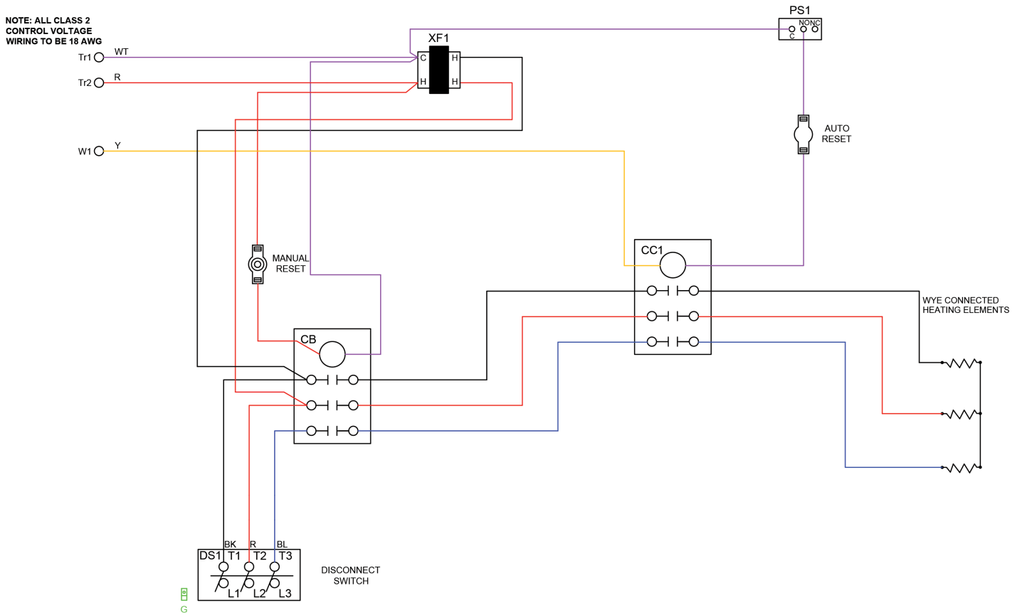
Figure 41: 208/240/408V, Three Phase, 1 Stage EH
