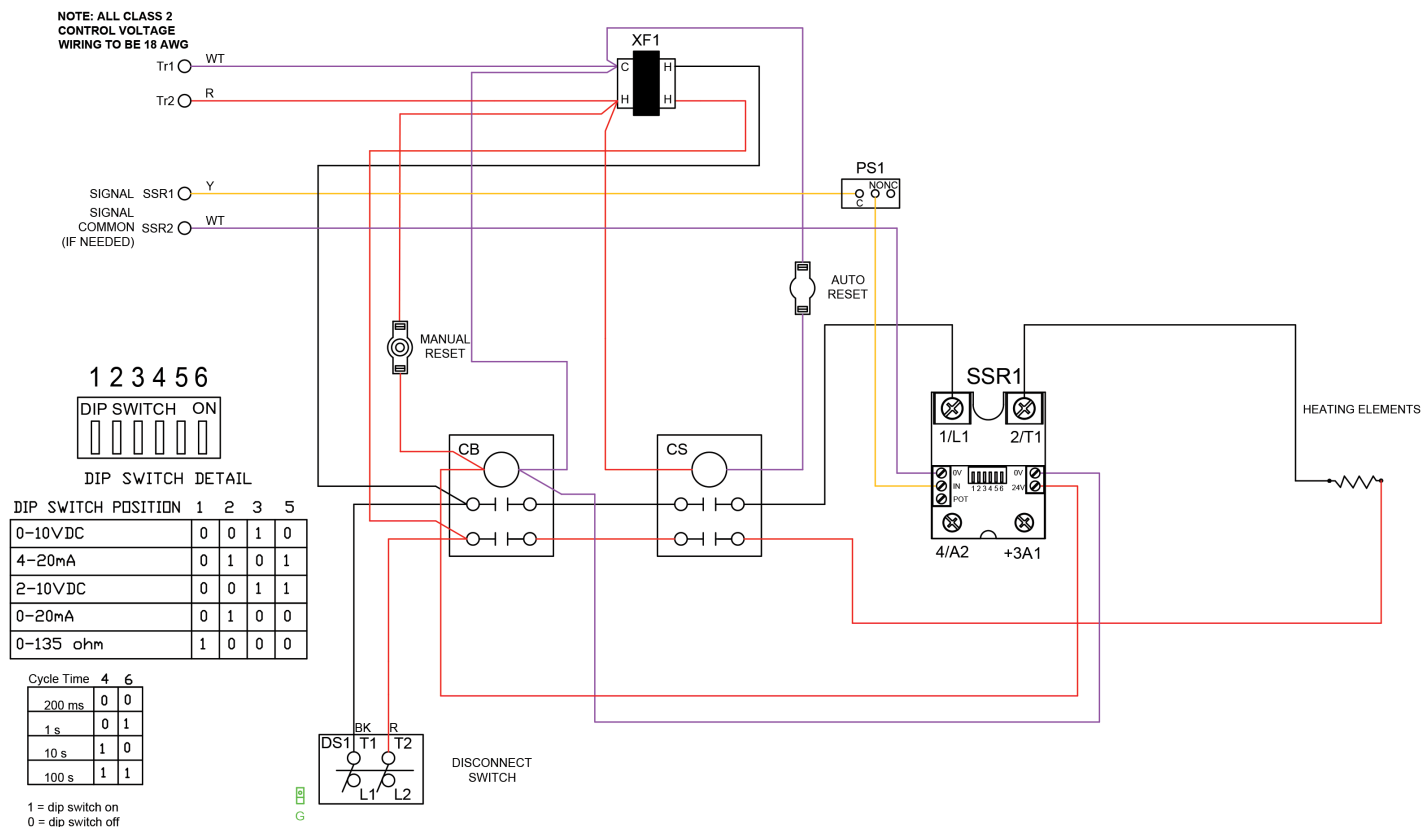
Figure 39: 208/240/408V, Single Phase, SCR EH
