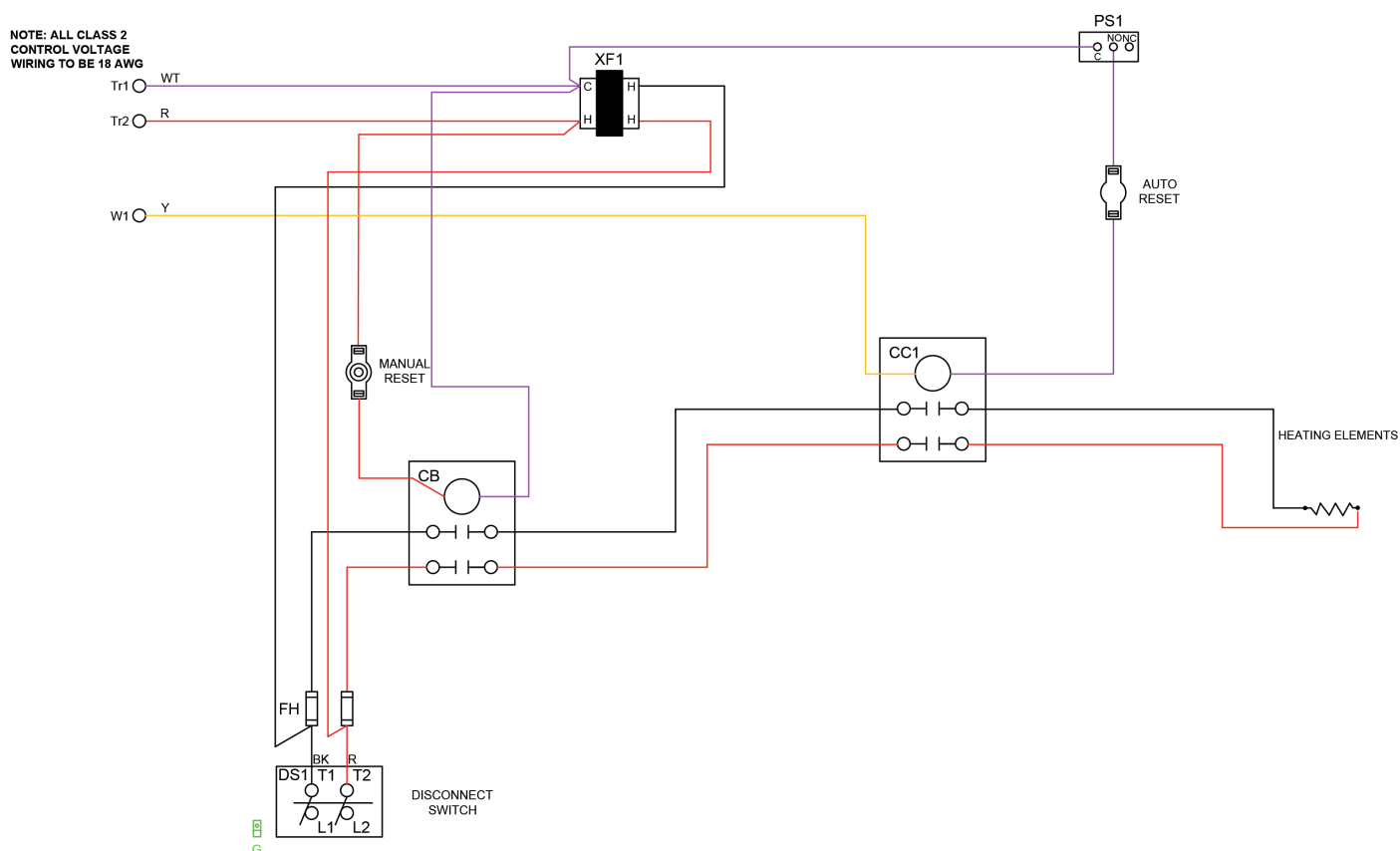
Figure 42: 208/240/408V, Fused Disconnect, Single Phase, 1 Stage EH
