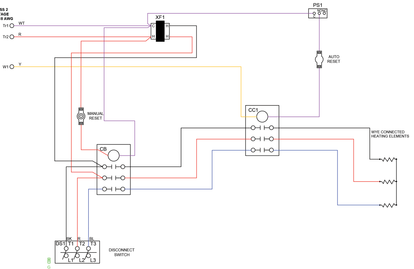
Figure 41: 208/240/408V, Three Phase, 1 Stage EH
