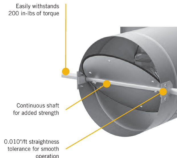
Figure 37: Damper Blade Construction
