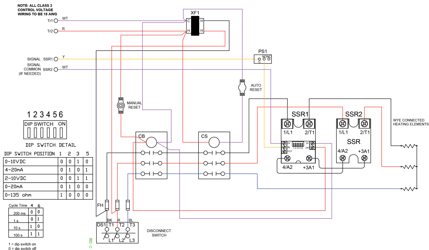
Figure 40: 208/240/408V, Fused Disconnect, Three Phase, SCR EH
