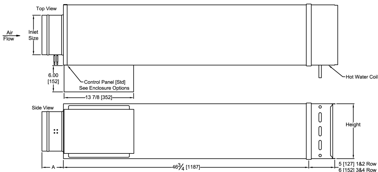
Figure 6: MQTH-500 Single Duct Air Terminal Unit with Integral Attenuator and Hot Water Coil
