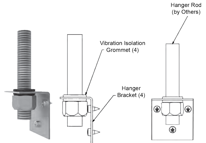
Figure 31: Hanger Brackets
