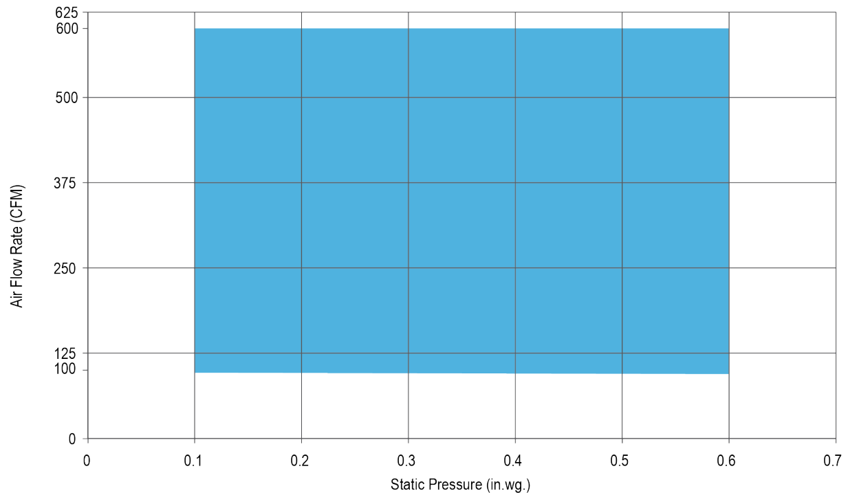
Figure 23: MQFVI-500 ECM Fan Performance Curves Unit Size 1
