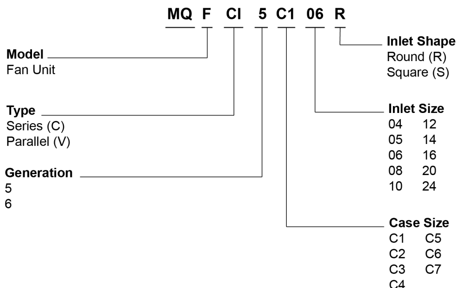
Figure 7: Fan Powered Terminal Units Nomenclature
