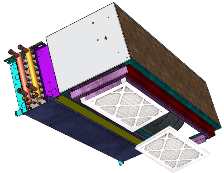
Figure 13: Factory-Installed Valve & Piping Packages - Connecting Pipe Locations: 2-Pipe Cooling or Heating
