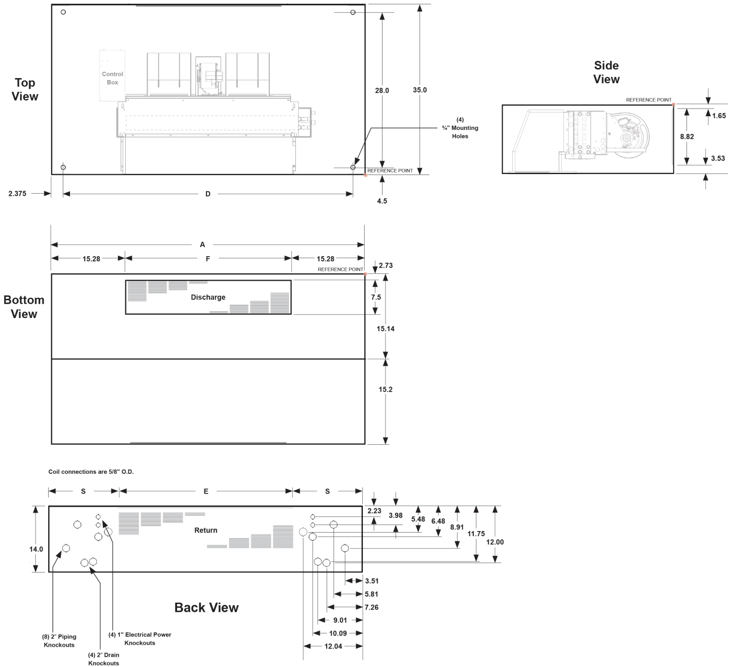
Figure 20: Dimensions – Cabinet Fan Coil, Bottom Discharge – Rear Return
