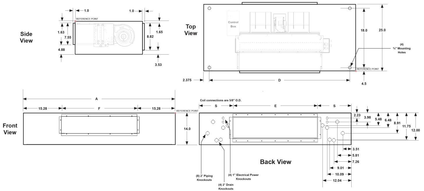
Figure 18: Dimensions – Cabinet Fan Coil, Front Discharge – Rear Return
