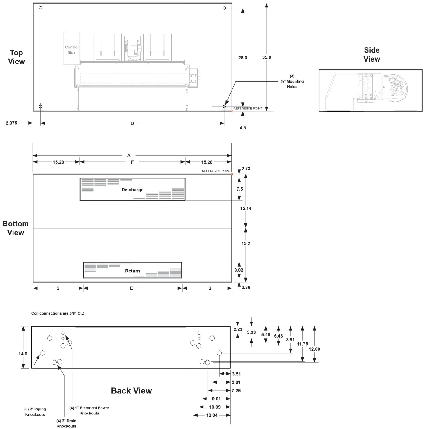
Figure 21: Dimensions – Cabinet Fan Coil, Bottom Discharge – Bottom Return
