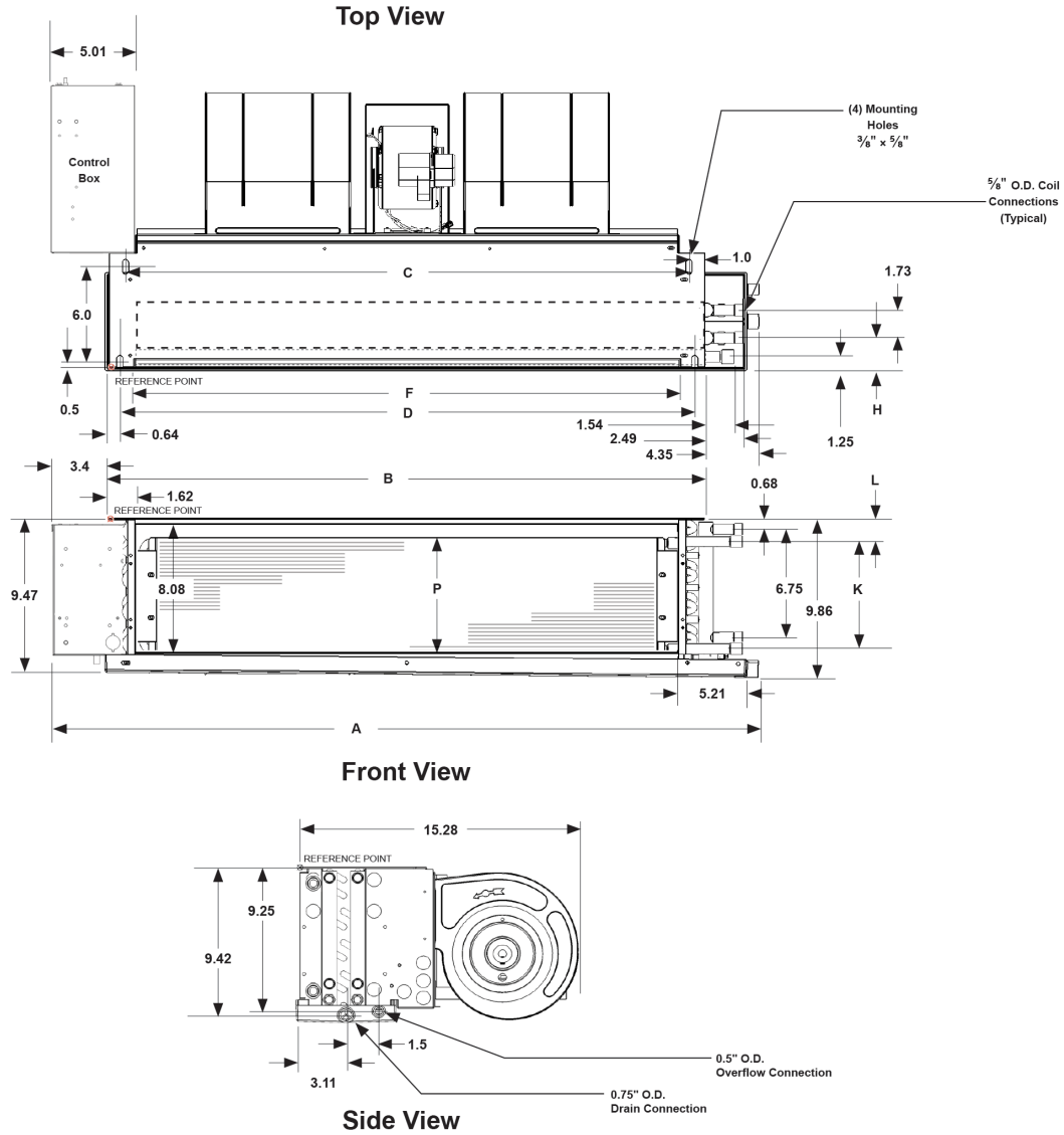
Figure 15: Dimensions – Hideaway Fan Coil, Front Discharge – Free Return
