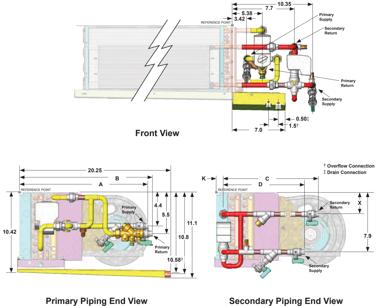
Figure 14: Factory-Installed Valve & Piping Packages - Connecting Pipe Locations: 4-Pipe Cooling and Heating, Same-Side
