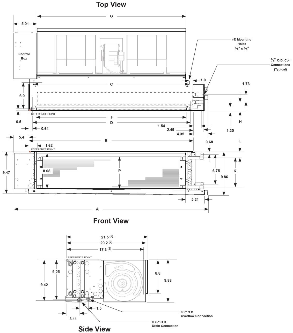
Figure 16: Dimensions – Hideaway Fan Coil With Plenum, Front Discharge – Rear Return
