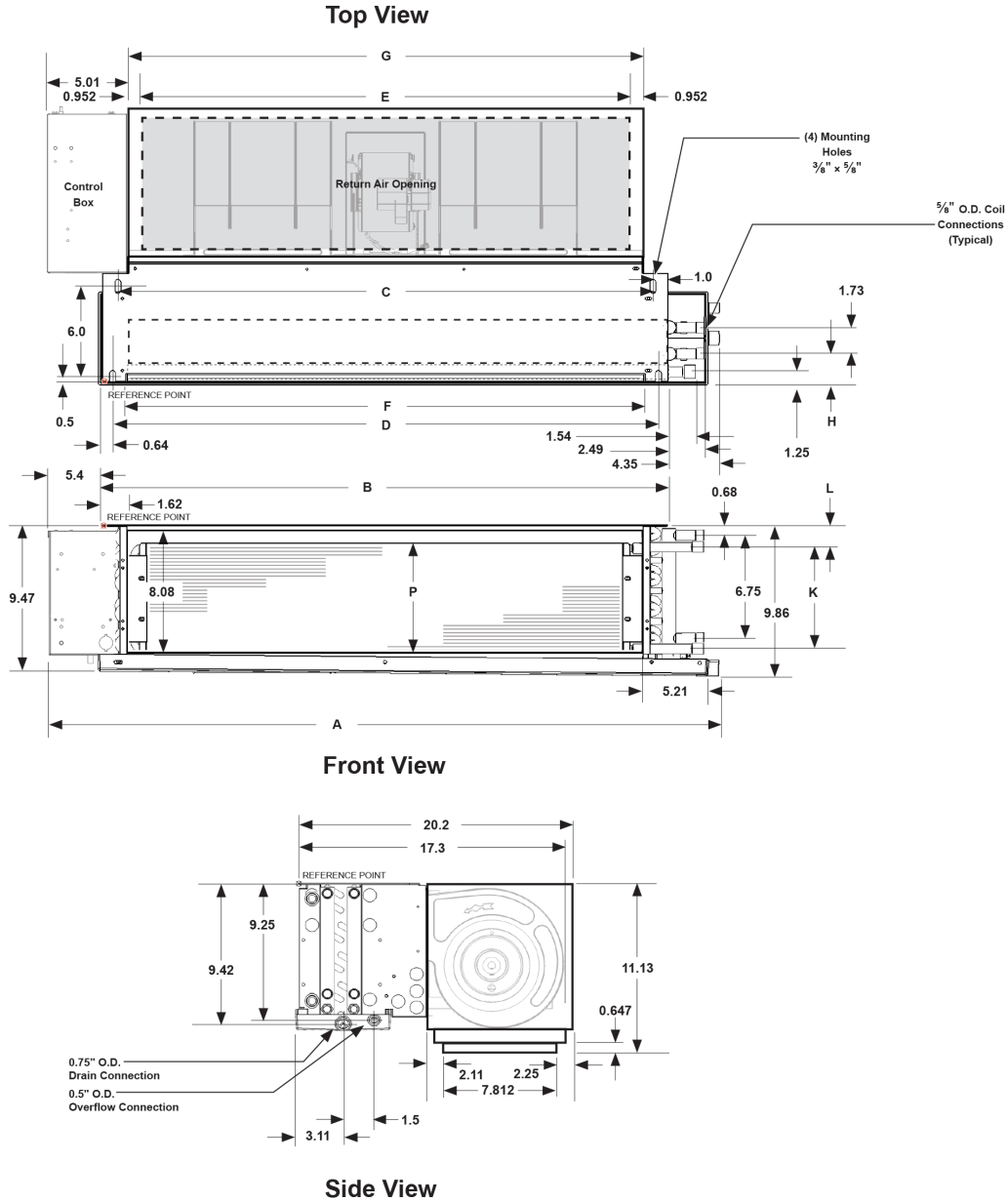
Figure 17: Dimensions – Hideaway Fan Coil With Plenum, Front Discharge – Bottom Return
