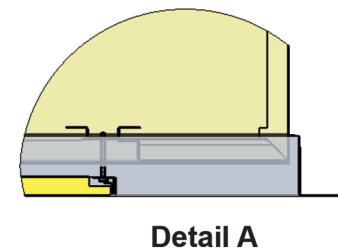
Plate to cabinet connection for fully recessed units
