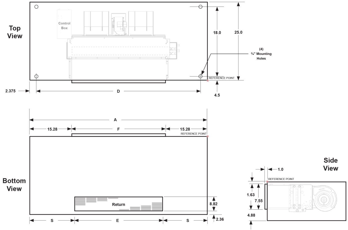
Figure 19: Dimensions – Cabinet Fan Coil, Front Discharge – Bottom Return
