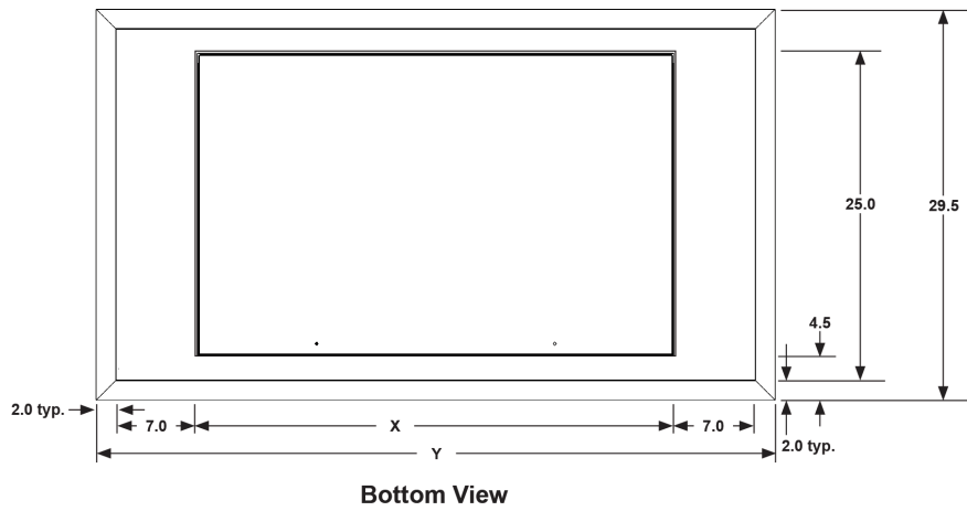
Figure 22: Dimensions – Recessed Cabinet Fan Coil with and Without Ceiling Plate
