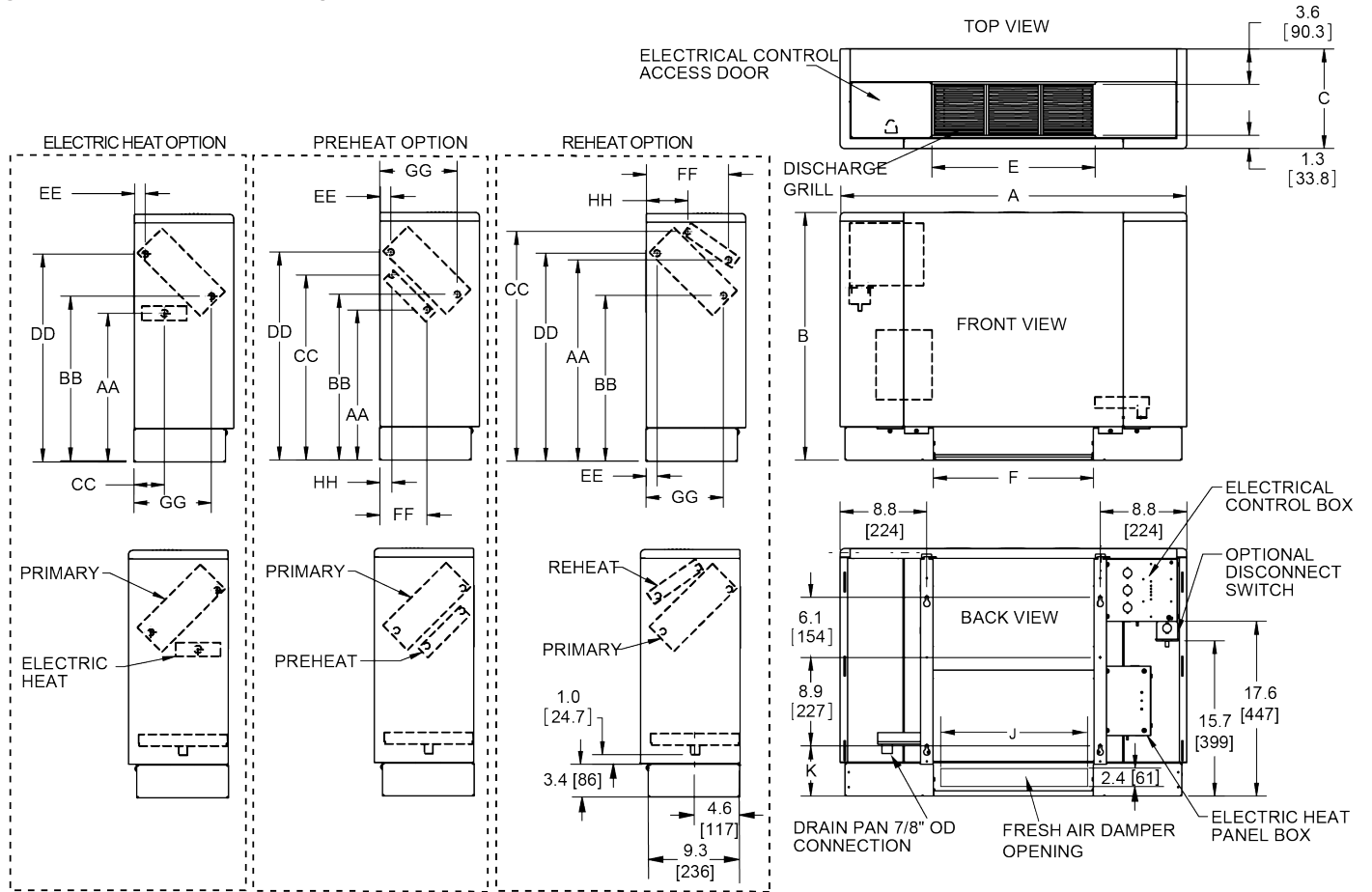
Figure 13: Dimensions: Flat Top Fan Coils
