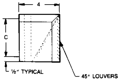
Figure 18: Fresh Air Intake Box Dimensions
