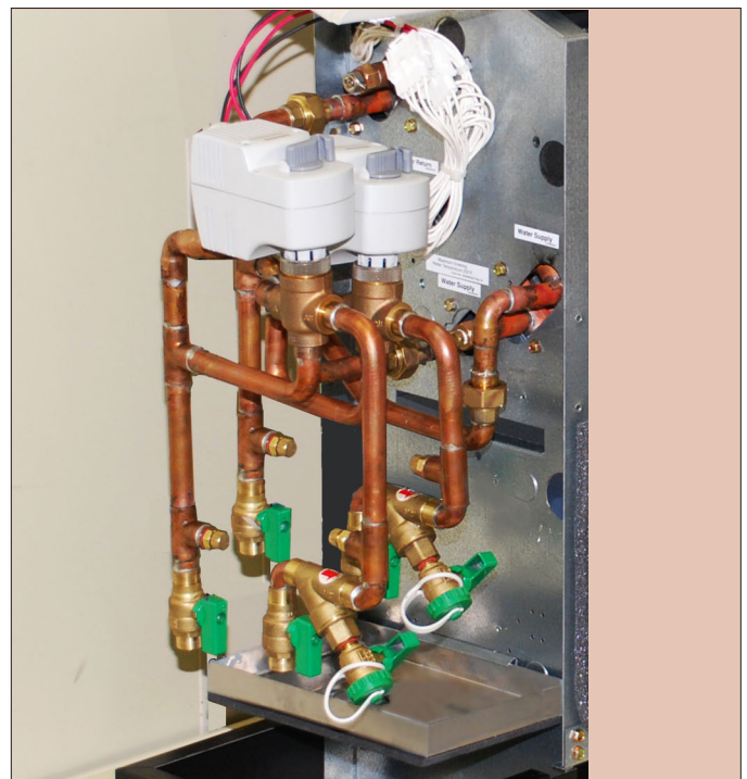
Figure 3: Four-Pipe Deluxe Valve and Piping Package
