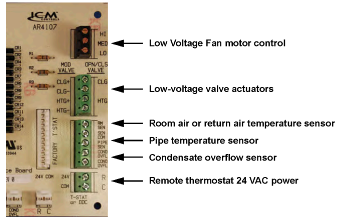
Figure 1: LV Interface Board 24 VAC connections
