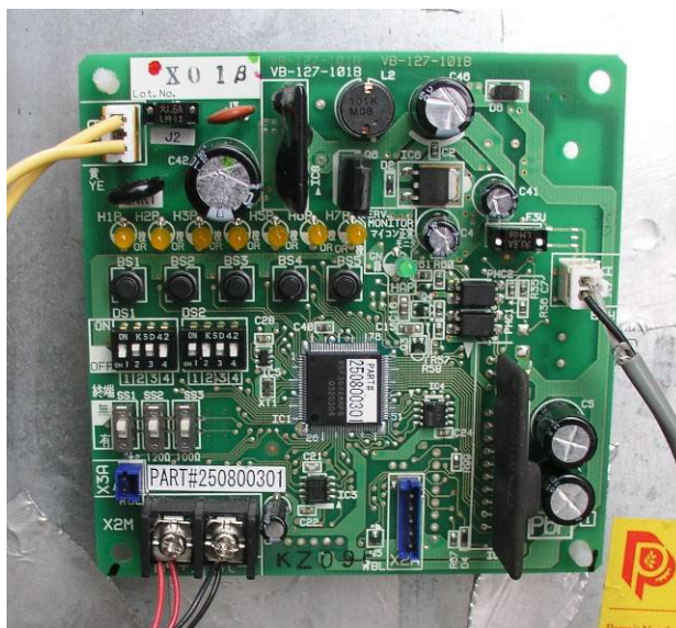
Figure 4, DIII-NET Communication Gateway mounted in unit
