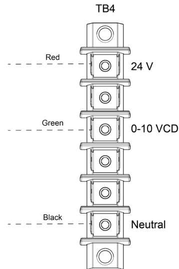
Figure 25: Terminal Block 4 Diagram
