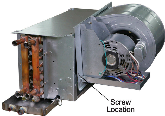
Figure 58: Removing Fan Deck Assembly
