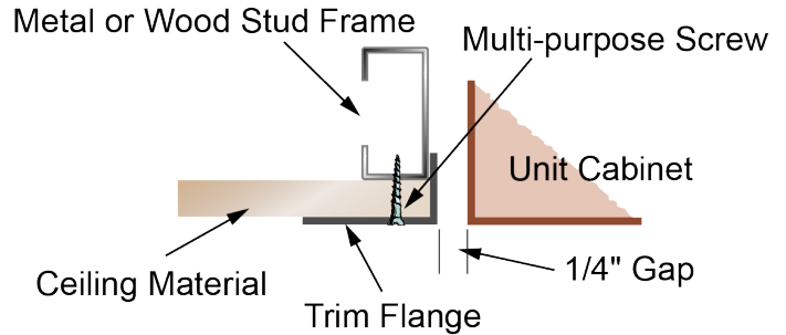
Figure 20: Trim Flange Securing Detail
