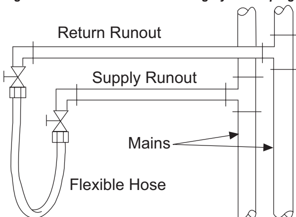
Figure 51: Connections for Flushing System Piping
