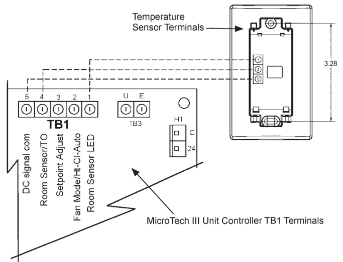
Figure 26: Temperature Sensor Wiring to MicroTech III Unit Controller
