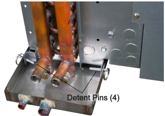
Figure 56: Drain Pan Attachment to Coil Section
