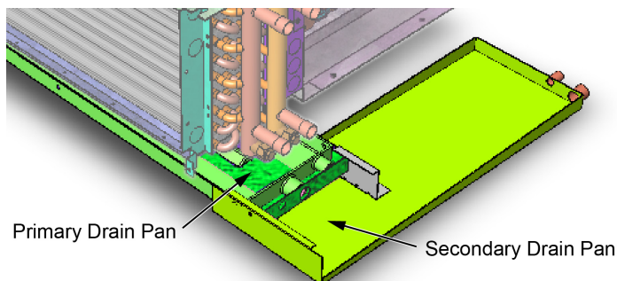
Figure 55: Primary and Secondary Drain Pans
