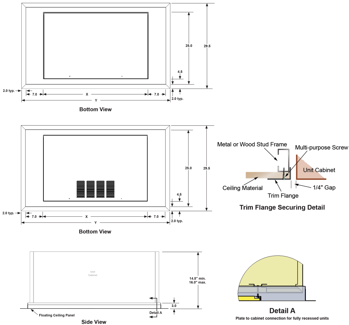
Figure 50: Dimensions – Recessed Cabinet Fan Coil with and Without Ceiling Plate
