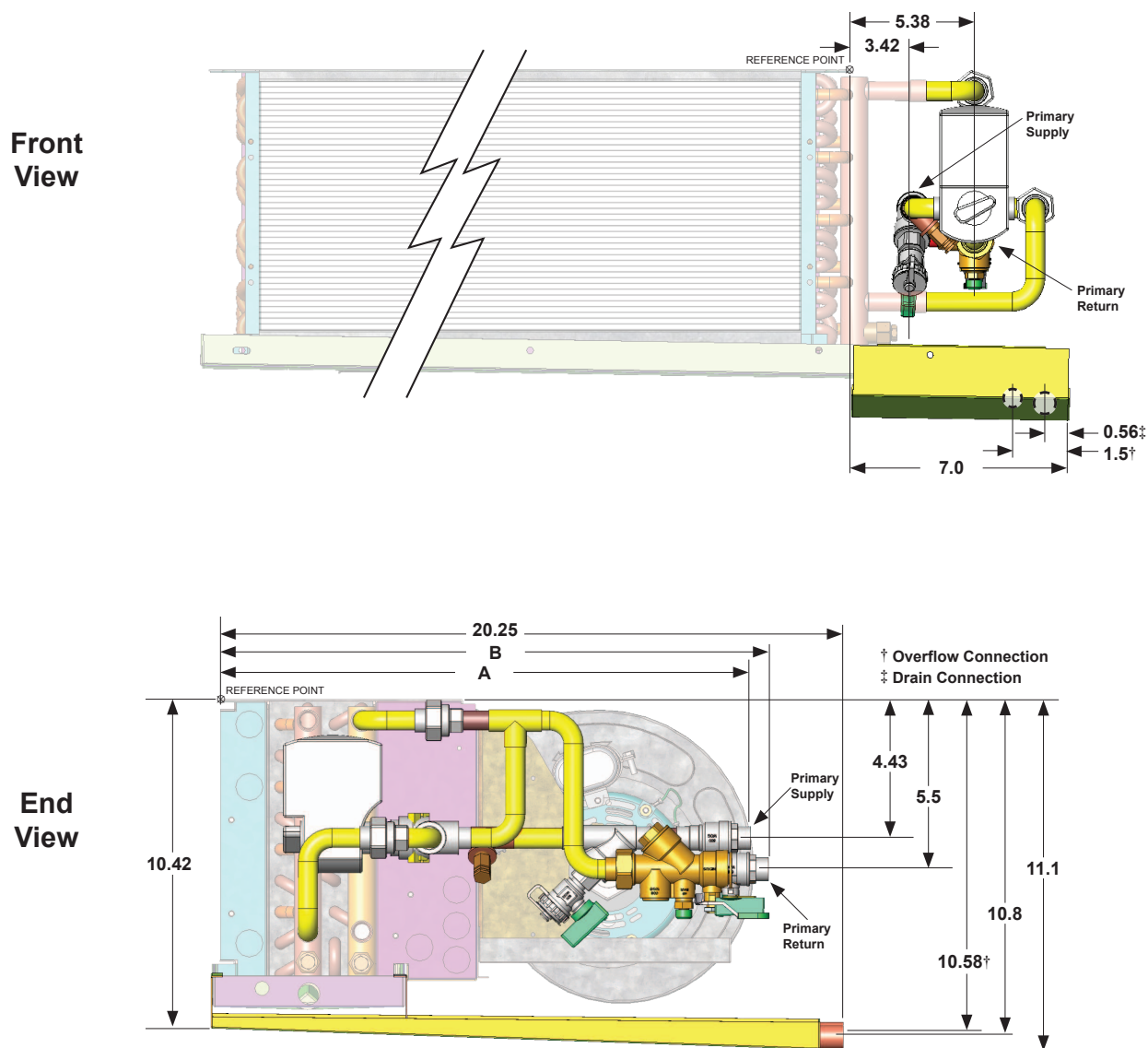
Figure 16: Connecting Pipe Locations: 2-Pipe Cooling or Heating (Deluxe Package Shown)
