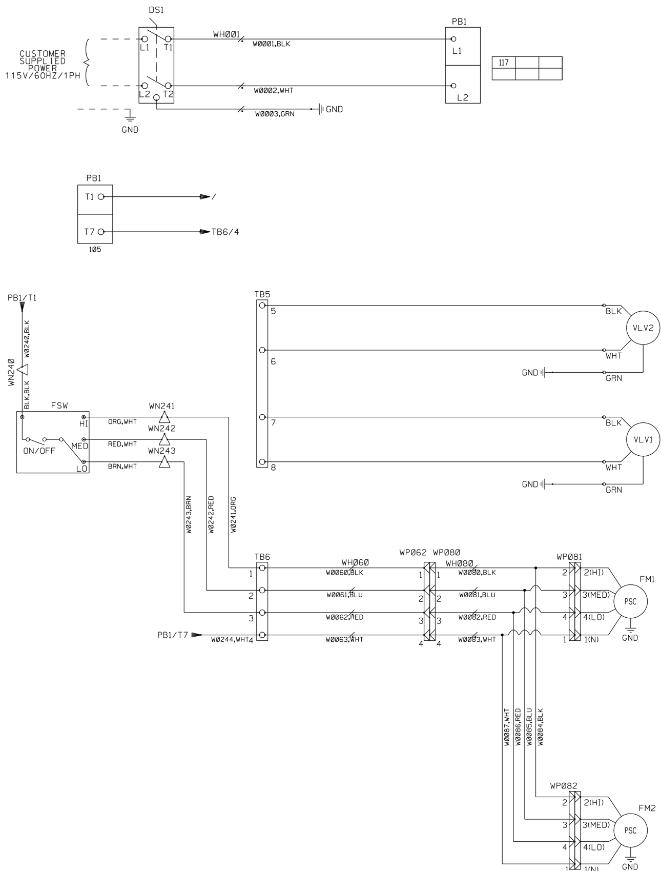
Figure 42: Fan Coil Wiring Diagram – Unit Mounted 3 Speed Switch, Low Voltage Valves
