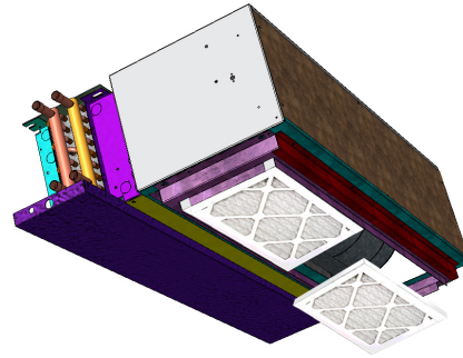
Figure 52: Filter Removal for Units with Bottom Returns
