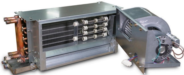
Figure 54: Exposed Electric Heater Assembly
