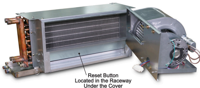
Figure 34: Electric Heat Over-Temp Reset Button Location
