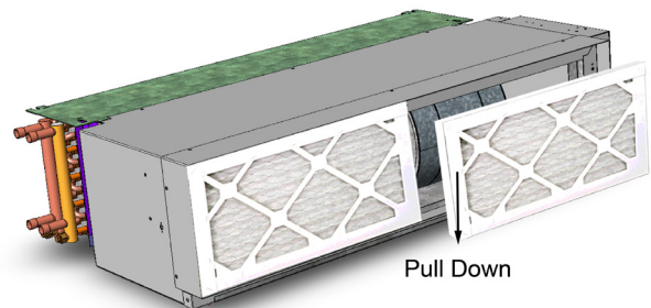
Figure 53: Filter Removal for Units with Rear Returns
