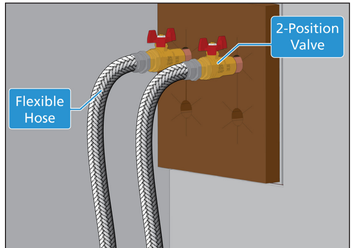
Figure 39: Supply and Return Hose Connections
