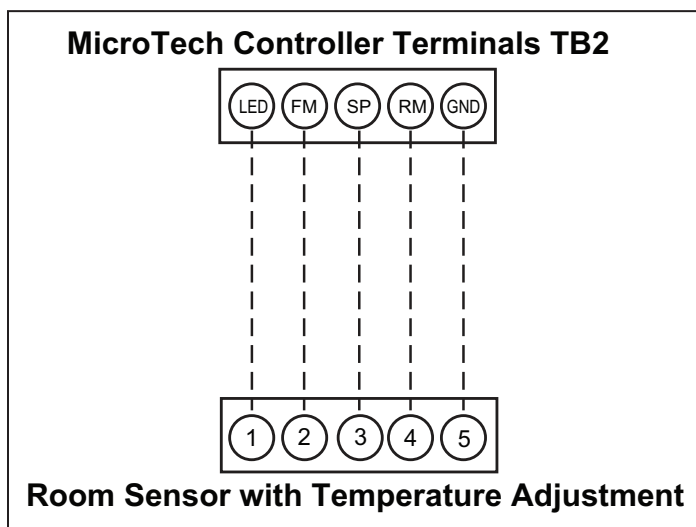
Figure 35: Room Sensor with Temperature Adjustment Wiring
