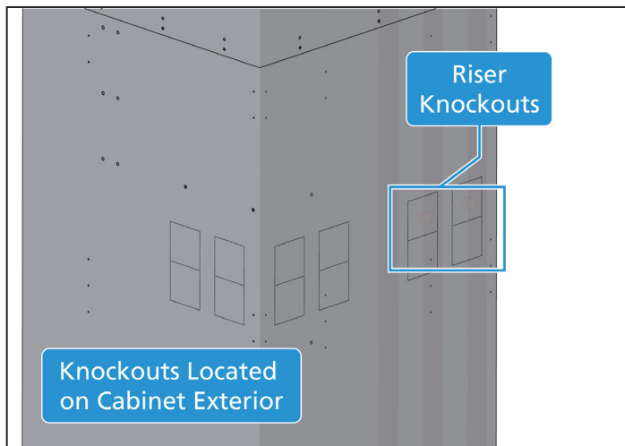
Figure 26: Riser Knockouts - Cabinet Exterior
