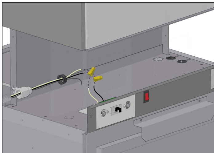
Figure 29: Wire to Unit Switch
