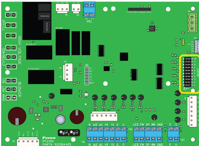
Figure 59: Location of Configuration DIP Switches on the MT2300 Unit Controller
