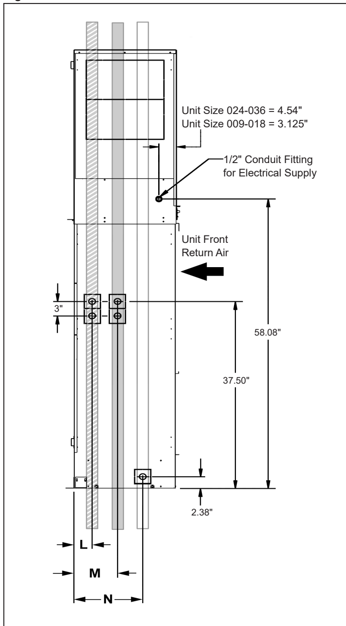
Figure 19: Riser Stub-Outs Knockouts Locations
