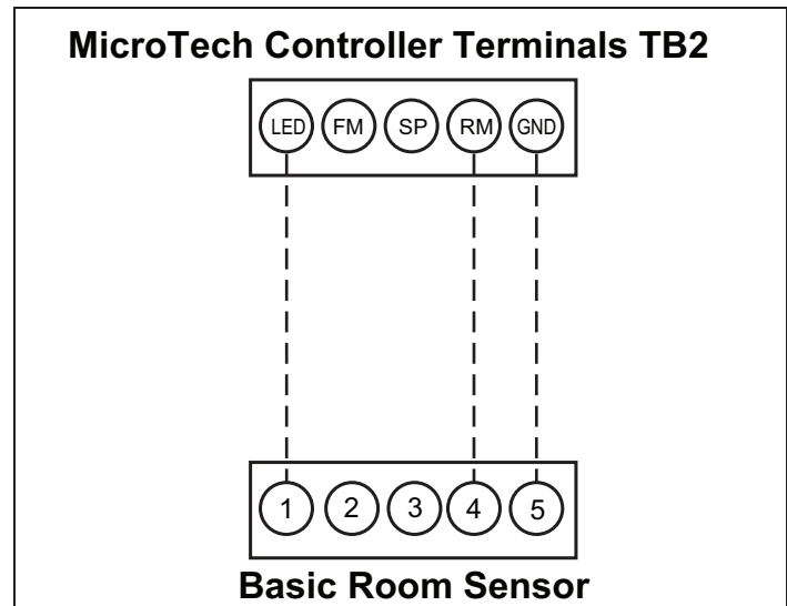
Figure 33: Basic Sensor – P/N 669529001
