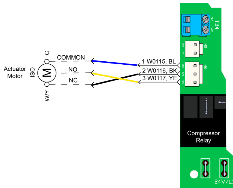
Figure 56: MT2300 wiring to an existing motorized valve from a previously installed unit with MicroTech III controller
