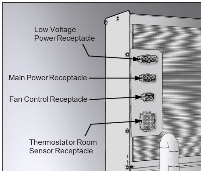
Figure 44: Plug Unit Component Wiring from the Top Cabinet Section into the Proper Receptacle on the Chassis
