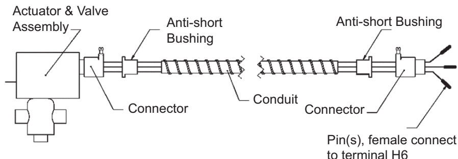
Figure 54: Normally Closed, Power Open Motorized Valve
