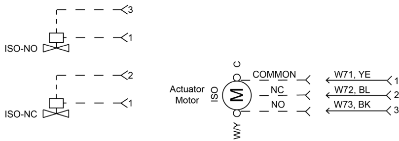
Figure 55: Motorized Valve Wiring
