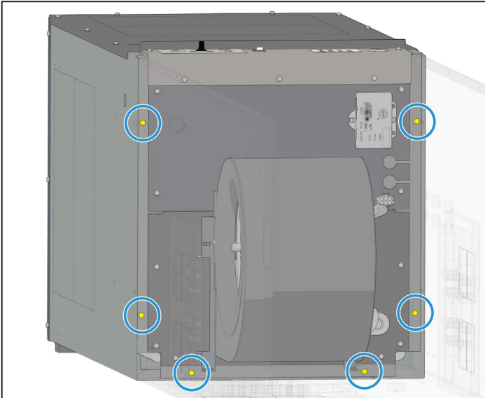
Figure 8: Cabinet Disassembly Screw Removal (Inside Unit)
