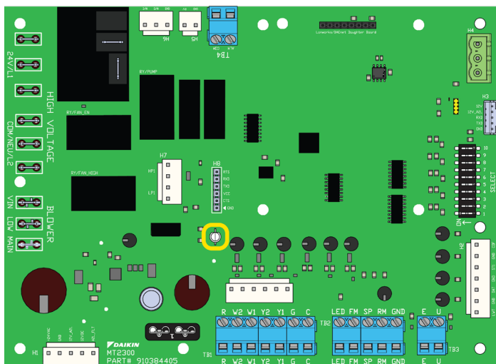
Figure 57: LED Indicator on MT2300 Board
