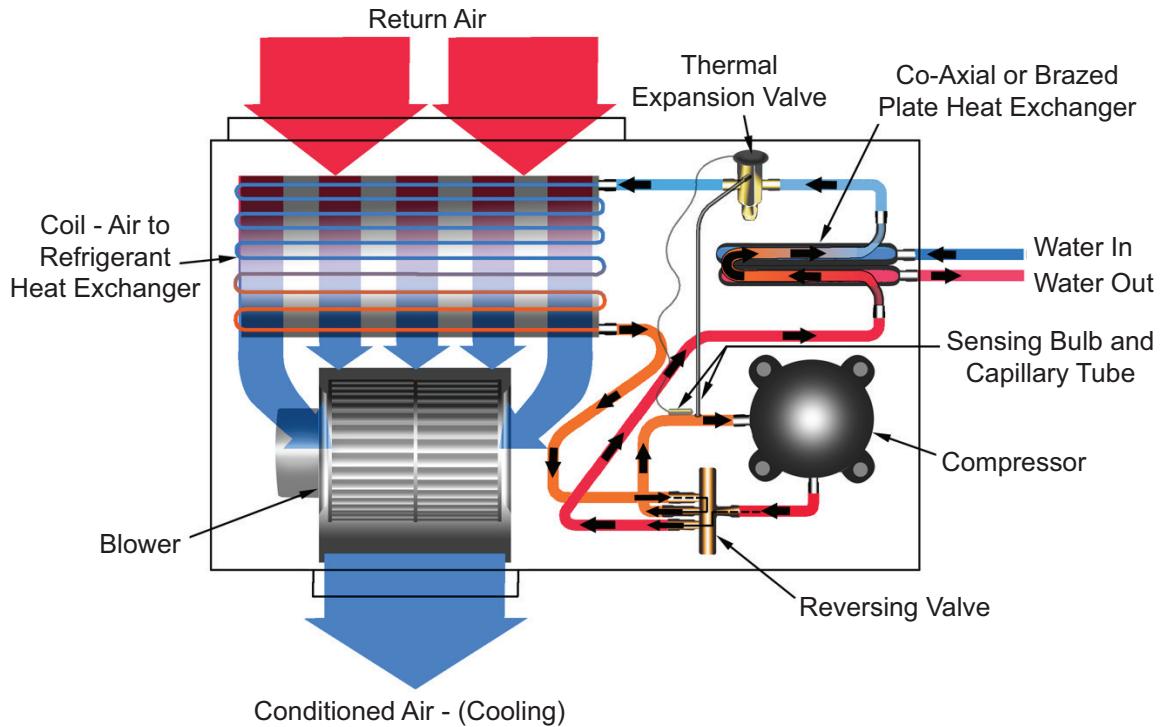
Figure 62: Cooling Mode
