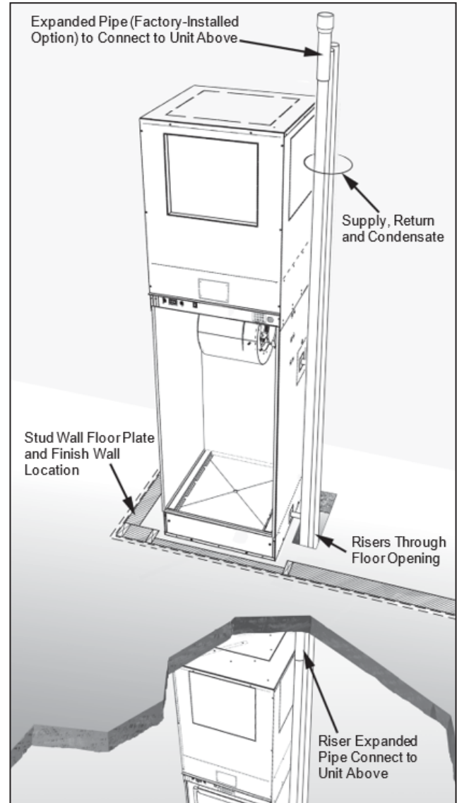
Figure 23: Position the Cabinet and Risers
