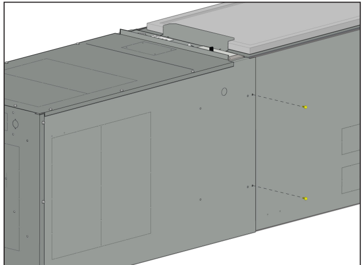
Figure 6: Cabinet Disassembly Screw Removal (Side)
