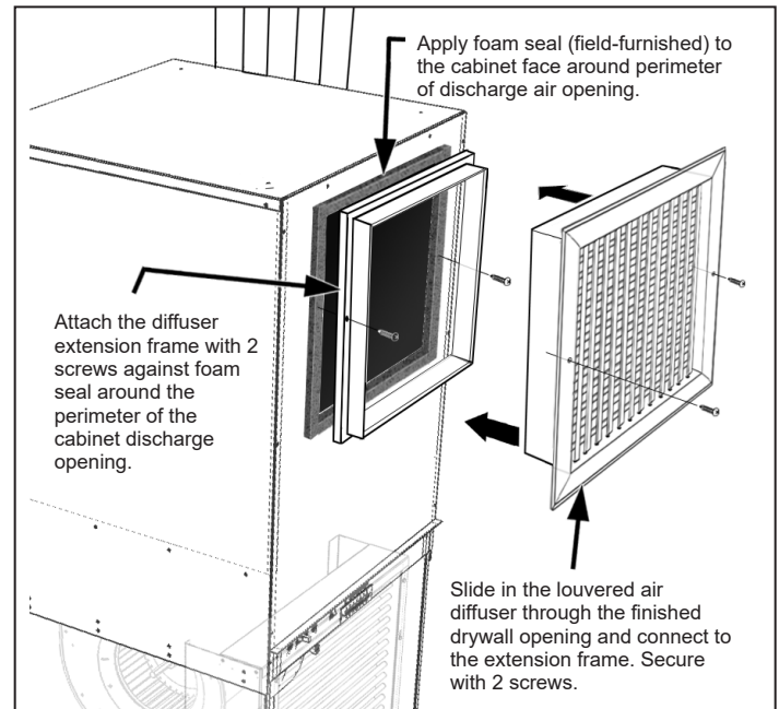
Figure 47: Installing the 3.25" Deep (2-Piece) Discharge Air Diffuser
