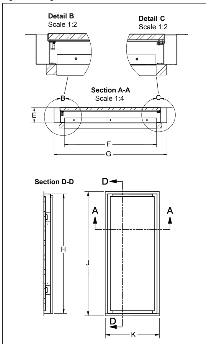
Figure 20: Hinged Panel Door
