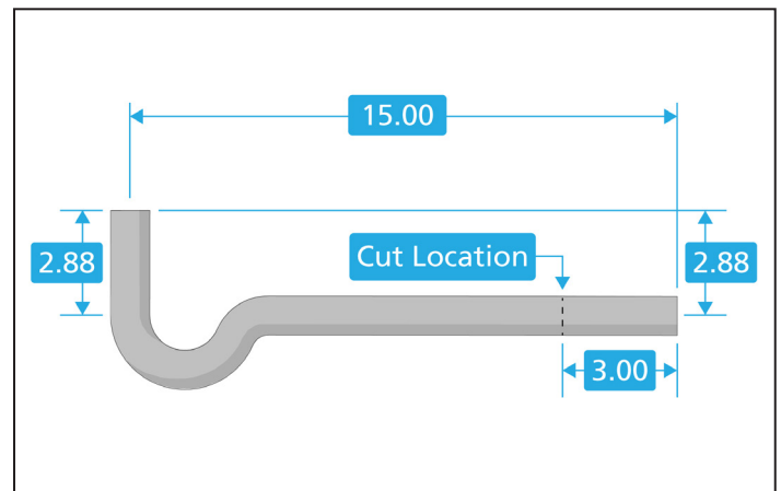
Figure 37: Drain Tube Cut Location
