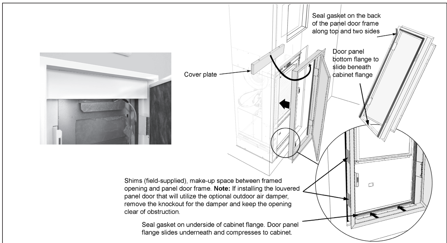
Figure 45: Installing the Return Air Panel Door (Hinged Perimeter Panel Door Shown)
