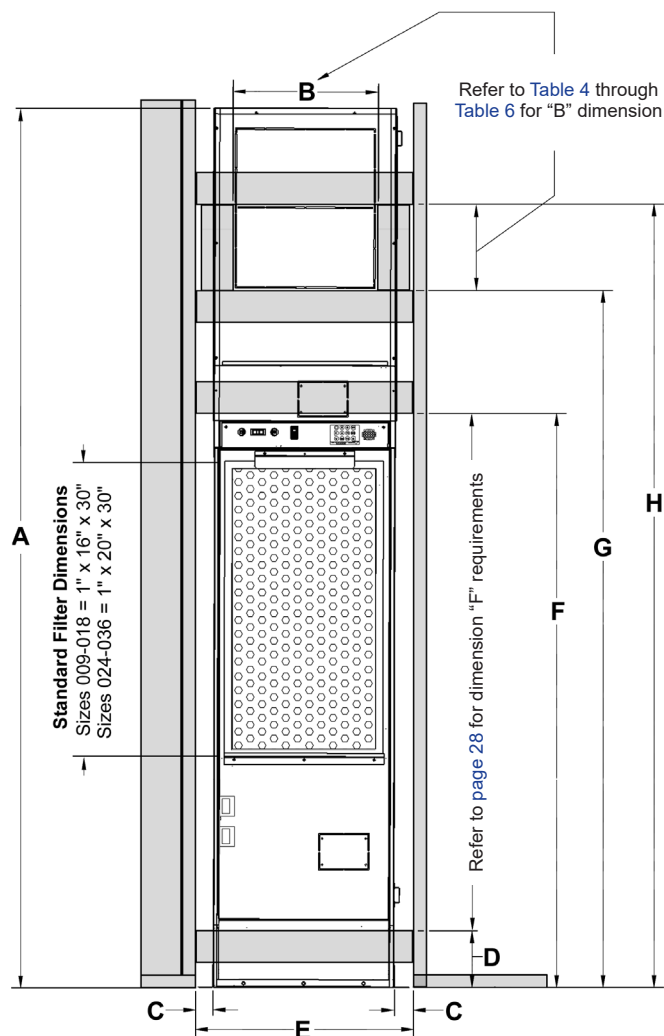
Figure 17: Framing Locations and Dimensions
