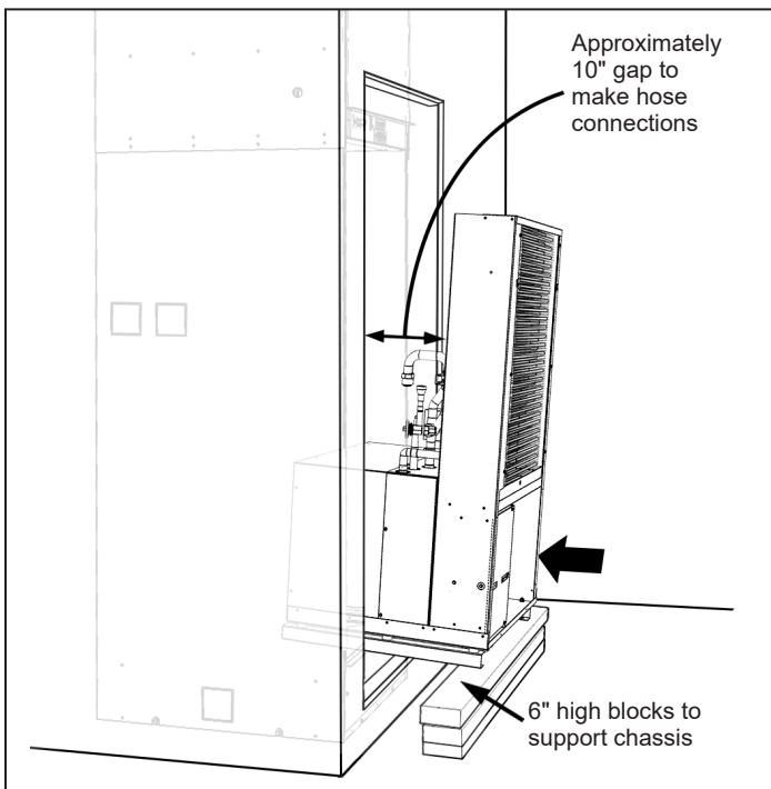
Figure 42: Slide Chassis Partially into the Unit Cabinet
