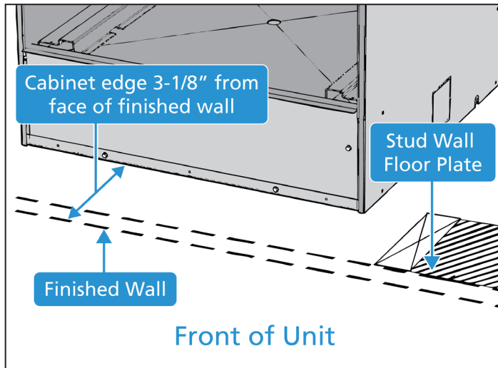
Figure 25: Critical Dimension - Cabinet Edge
