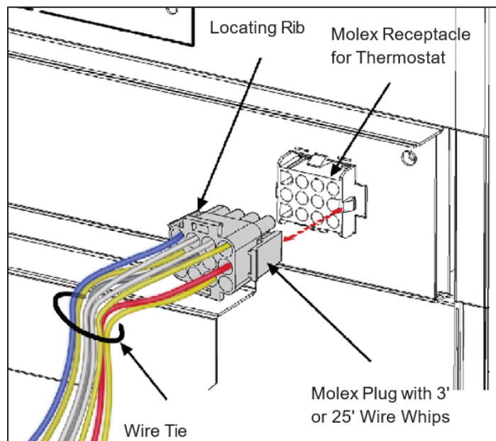
Figure 31: Plug 12-Pin Moxex with Wire Whips into the Moxex Receptacle
