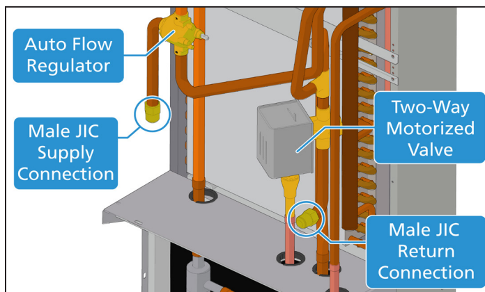
Figure 38: Typical Motorized Valve Piping
