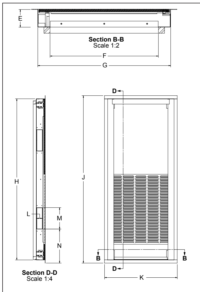
Figure 21: Louvered Panel Door
