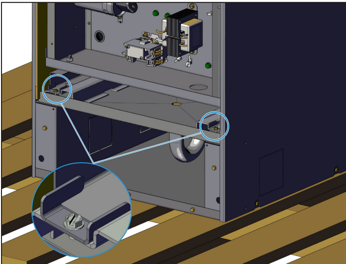
Figure 4: Remove Shipping Brackets
