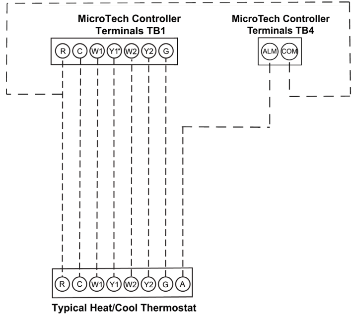
Figure 32: Wiring Example of Typical Heat/Cool Thermostat Connect Wiring Example of Typical Heat/Cool Thermostat Connections
