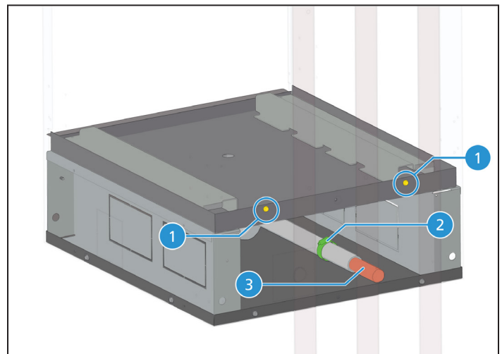
Figure 36: Drain Pan Screw Removal
