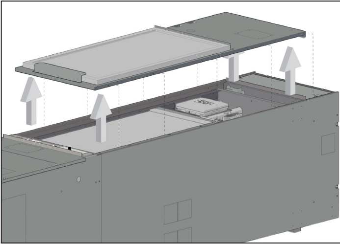
Figure 7: Cabinet Disassembly Screw Removal (Front)
