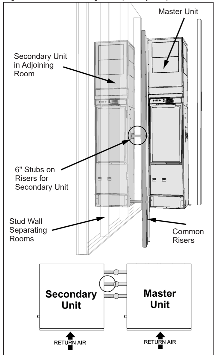
Figure 49: Twin Unit Arrangement (Side by Side)
