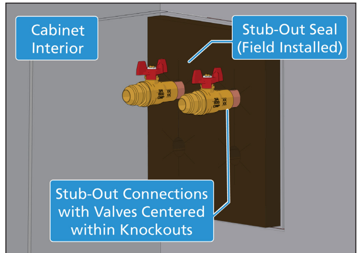
Figure 27: Stub-Out Seal (Field Installed)
