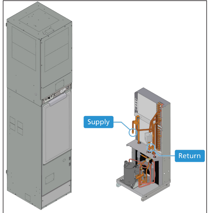
Figure 9: Unit Cabinet (WSVF) and Chassis (WSVC)
