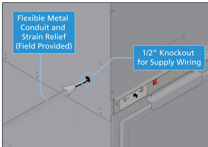
Figure 28: Supply Electric Wiring from Building to Unit
