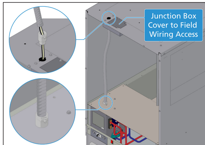
Figure 30: Power Wiring Through Top Entry
