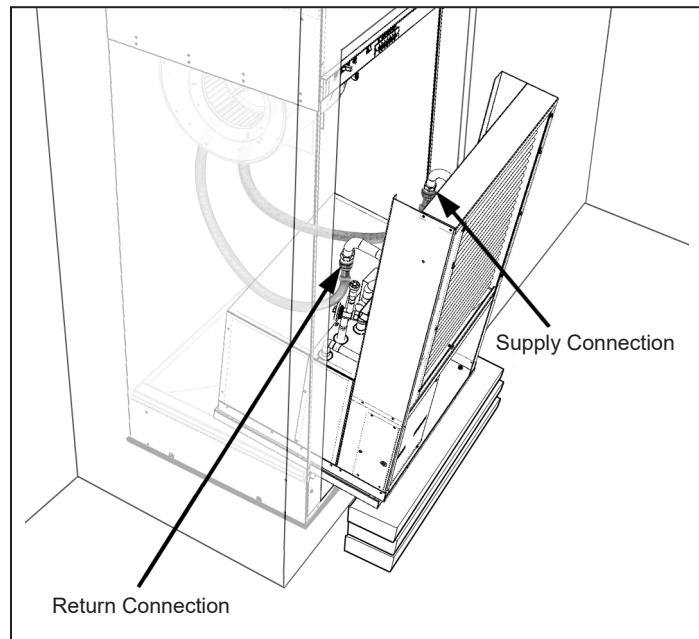
Figure 43: Leave 10" Gap for Clearance To Make Flexible Hose Connections
