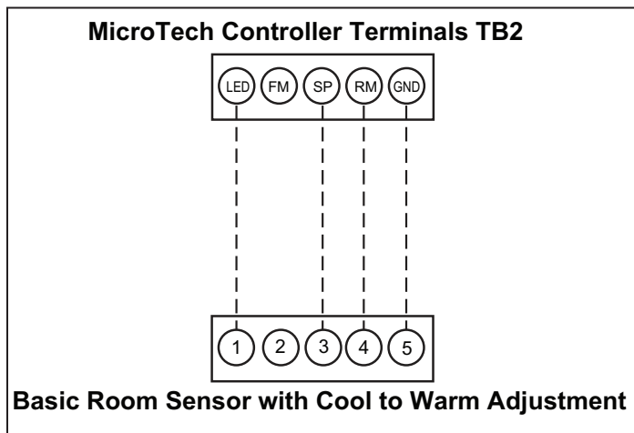
Figure 34: Example Wiring of SmartSource MicroTech Board to Basic Temperature Sensor Wiring
