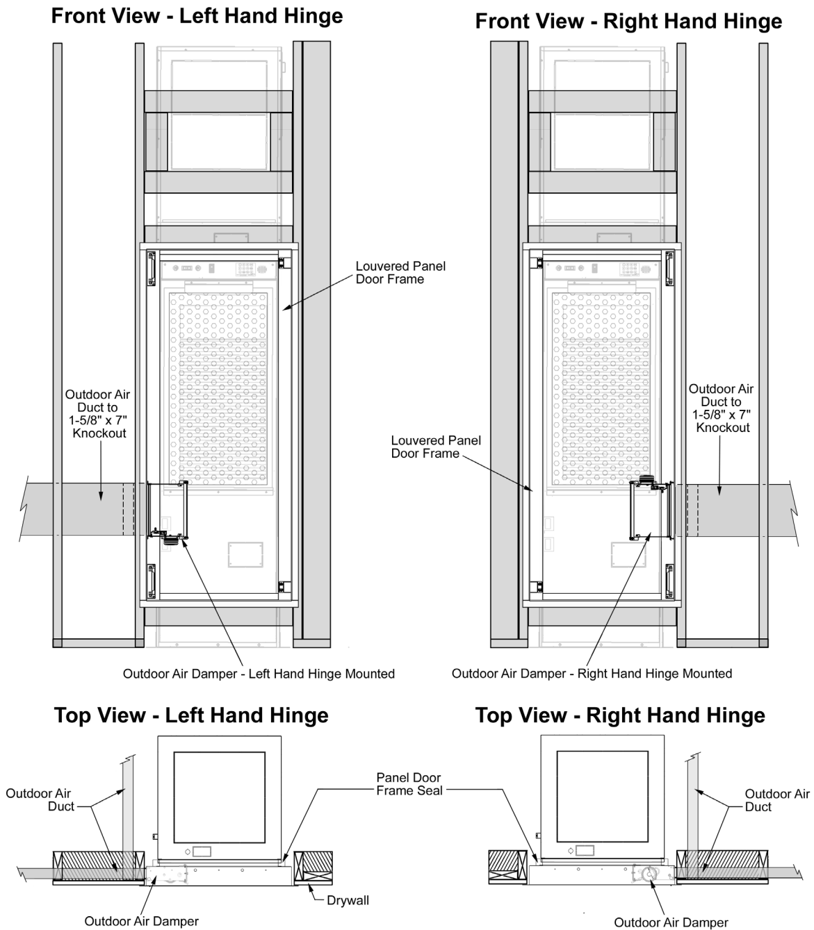
Figure 18: Louvered Panel Door with Motorized Outdoor Air Damper
