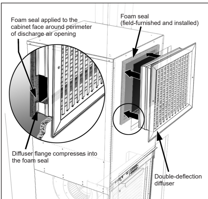
Figure 48: Installing the 1.75" Deep Discharge Air Diffuser
