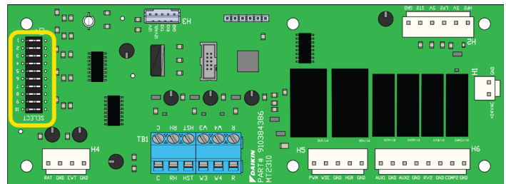
Figure 60: MT2310 I/O Expansion DIP Switches
