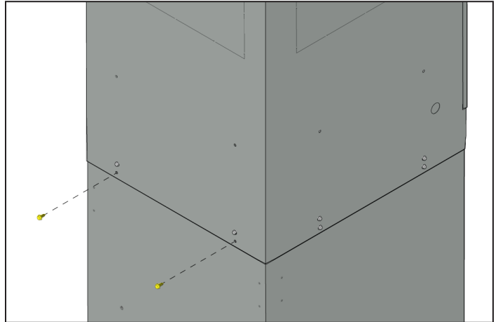
Figure 5: Cabinet Disassembly Screw Removal (Rear)
