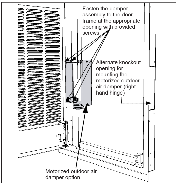
Figure 46: Fasten the Outside Air Damper Assembly to the Louver Panel Door Frame
