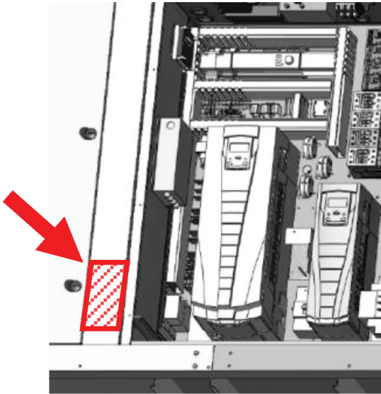
Figure 51: Recommended Location for DPS and MPS Control Enclosure Penetration
