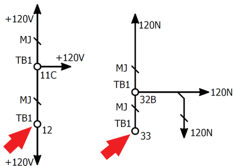
Figure 21: AWV and AWS 120VAC Wiring
