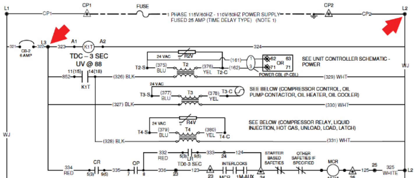
Figure 23: WSC, WDC, and WCC 120VAC Wiring
