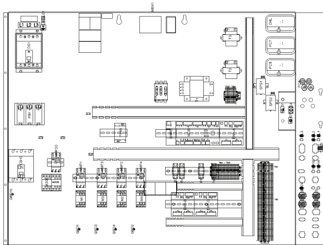
Figure 50: SWT Control Enclosure Example (460V, 6-Compressor Unit)
