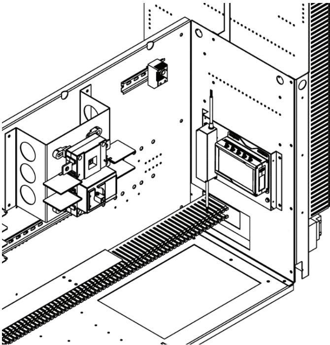
Figure 47: DPSA Mounting Location
