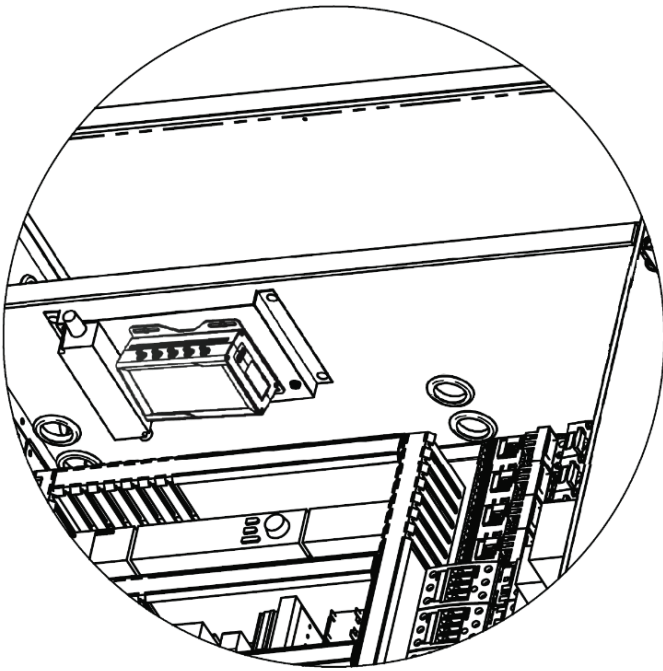
Figure 47: DPSA Mounting Location
