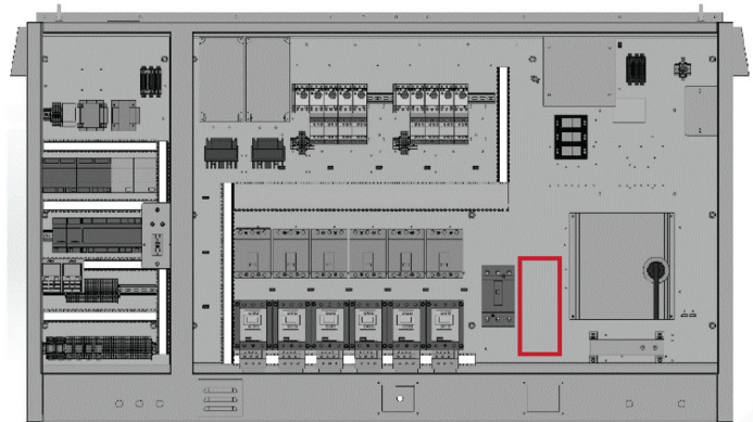
Figure 3: Component Locations – AGZ-D Large Panel
