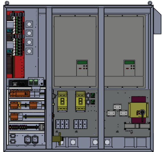
Figure 7: Typical AWS Large Panel Layout
