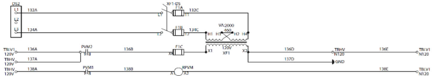
Figure 64: Typical RoofPak Unit 120VAC Wiring
