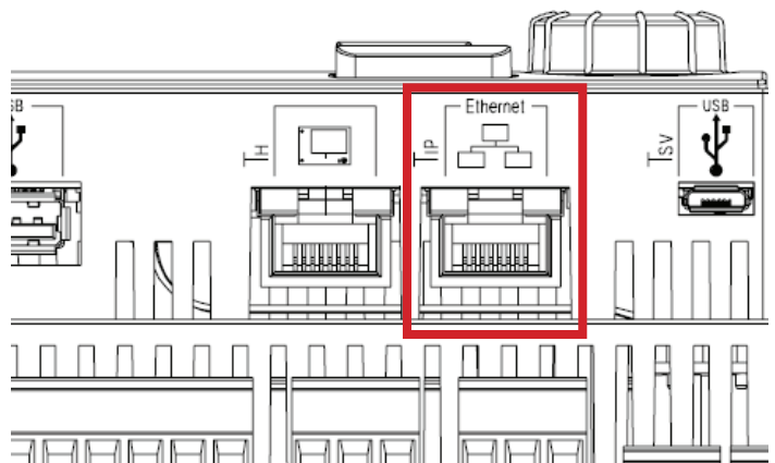
Figure 16: TIP Port Connection (MicroTech 4 shown)
