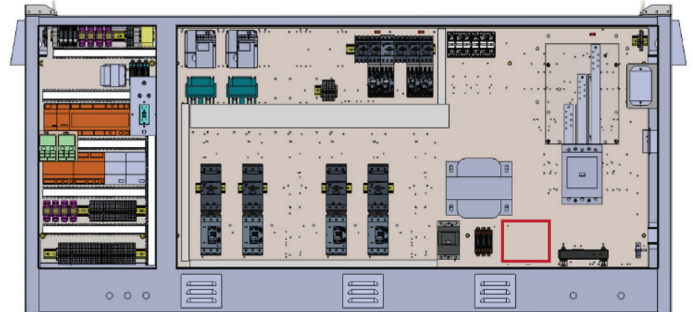
Figure 3: Component Locations – AGZ-D Large Panel
