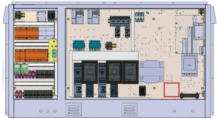
Figure 2: Component Locations – AGZ-D/E Medium Panel
