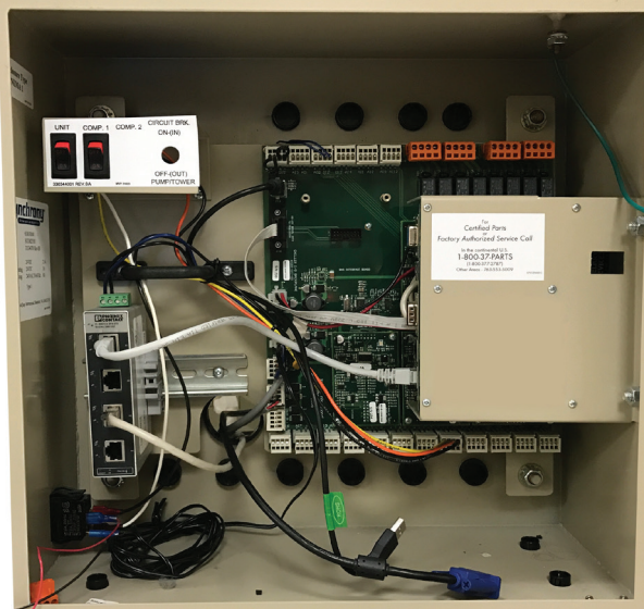
Figure 10: Typical WME Gen 1 Unit Control Panel Layout
