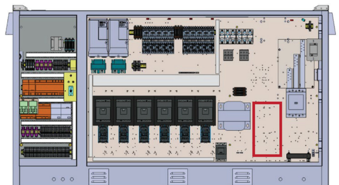
Figure 4: Component Locations – AGZ-E Large Panel
