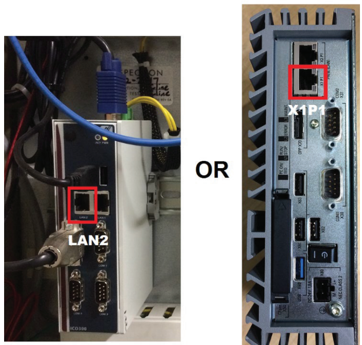
Figure 17: Connection to MicroTech II HMI PC
