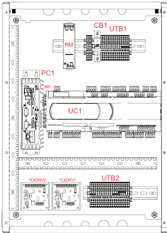
Figure 9: Typical WSC, WDC, and WCC Unit Control Panel Layout
