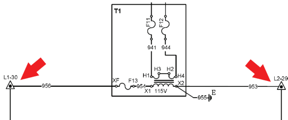
Figure 22: WMC 120VAC Wiring
