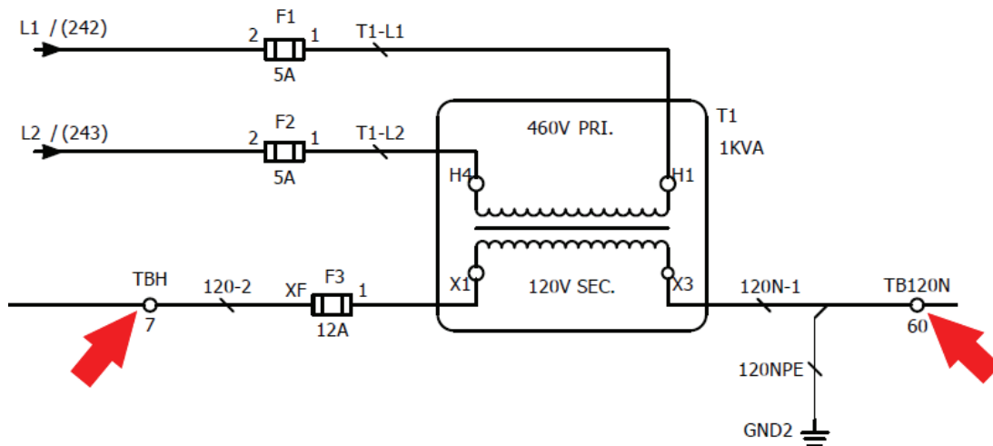
Figure 25: AMZ 120VAC Wiring
