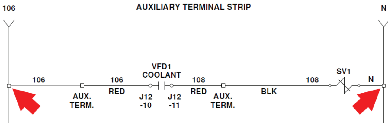
Figure 24: WME Gen 1 120VAC Wiring
