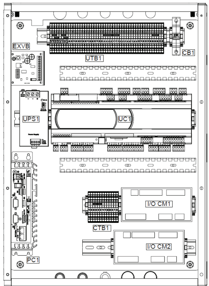
Figure 8: Typical WMC Unit Control Panel Layout
