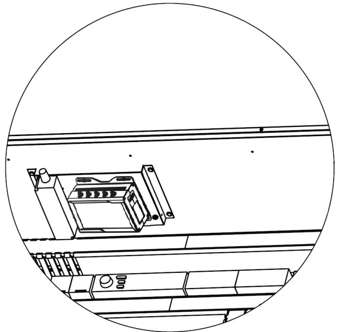
Figure 45: MPS Bracket Mounting Locations
