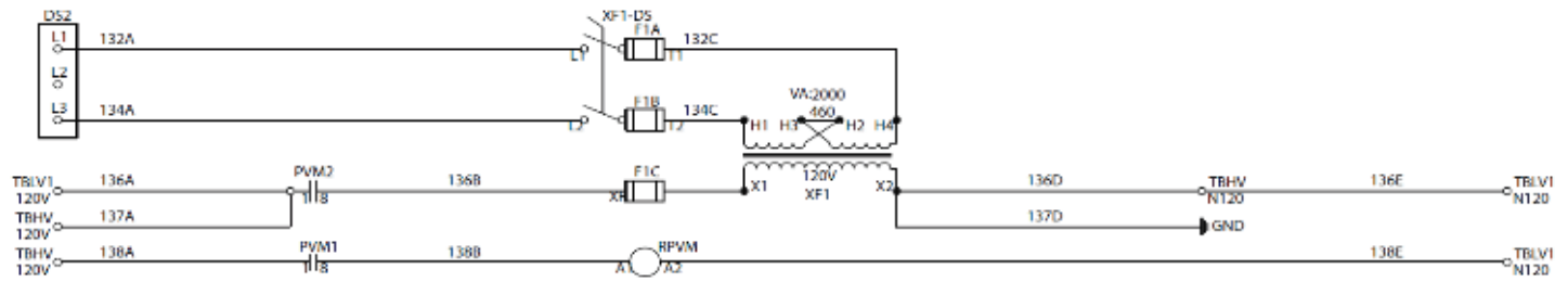
Figure 63: Typical Rebel Applied 120VAC Wiring
