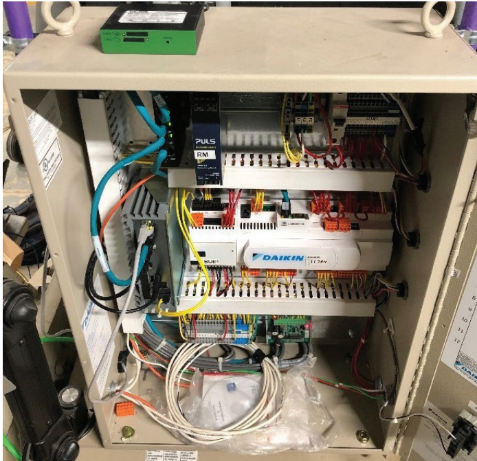
Figure 33: Modem Mounting
