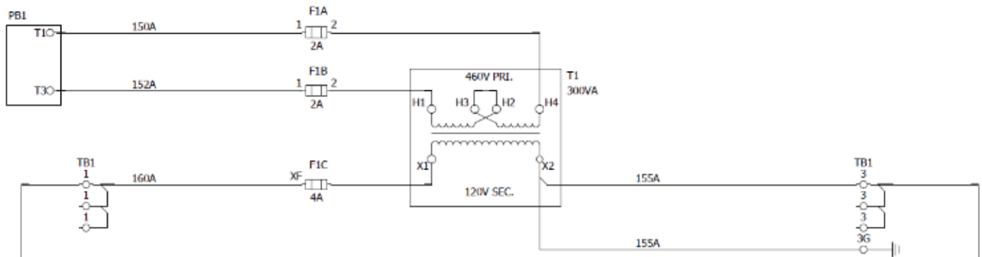
Figure 61: Typical Rebel A and B 120VAC Wiring
