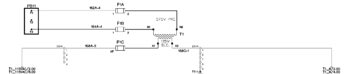
Figure 65: Typical SWP and SWT Unit 120VAC Wiring
