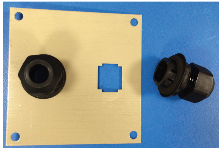
Figure 55: 5/8" Bushing for Installation Inside Control Enclosure
