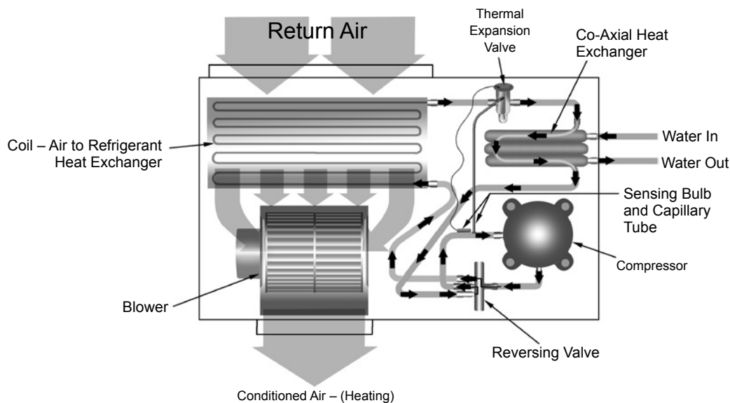
Figure 48: Heating mode
