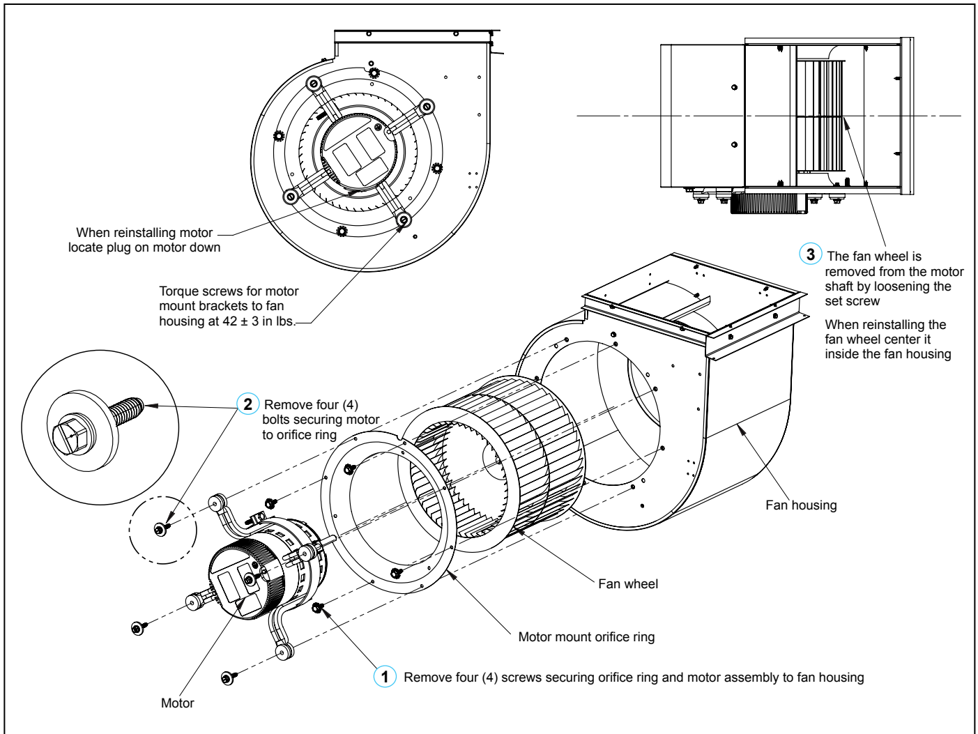
Figure 46: Disassemble motor orifice ring & motor mount screws from fan housing
