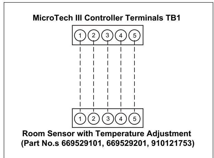
Figure 33: Room sensor with temperature adjustment wiring
