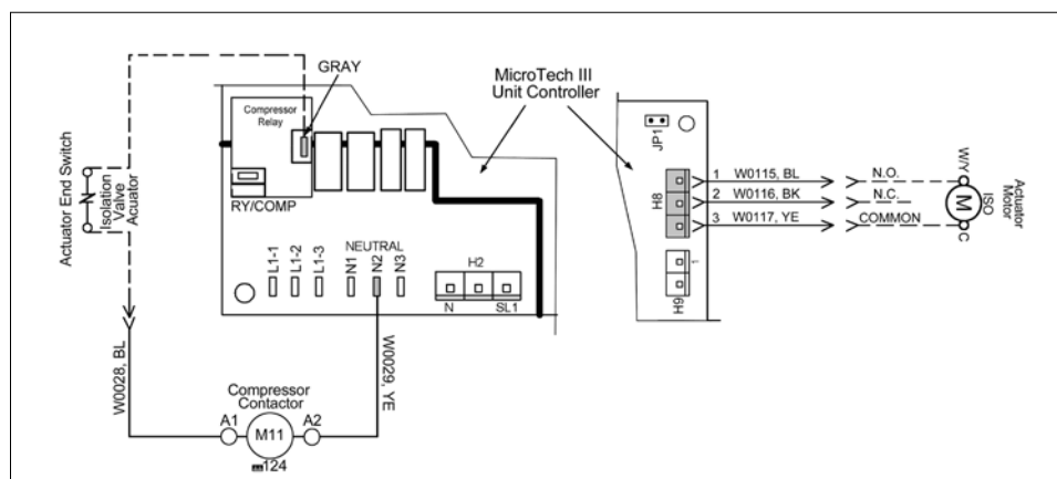
Figure 45: Motorized valve wiring
