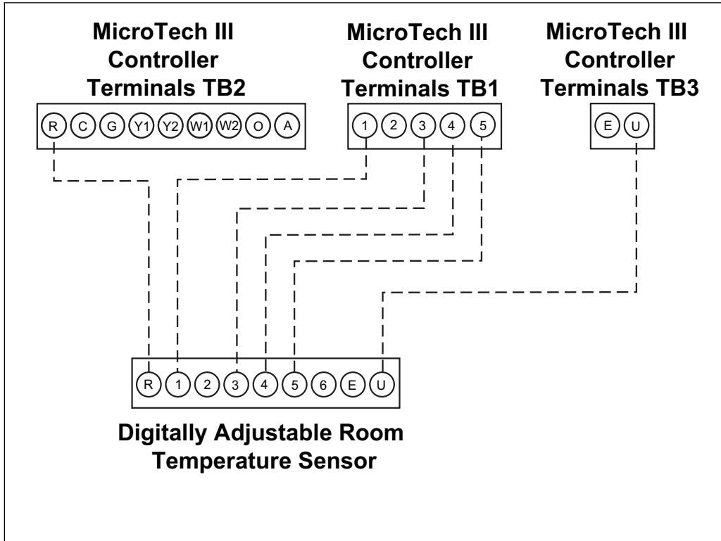
Figure 34: Digitally adjustable room temperature sensor wiring
