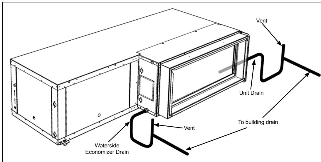
Figure 37: Unit condensate drain pipe detail with waterside economizer option
