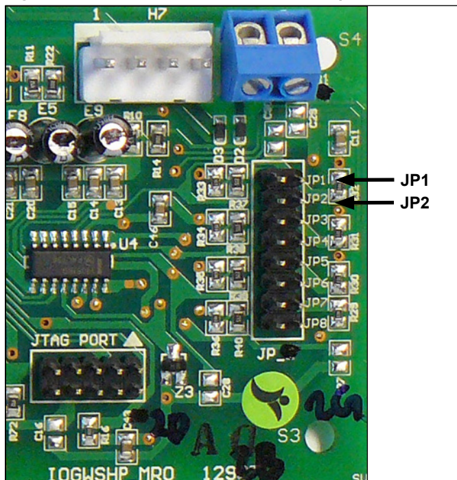
Figure 43: JP1 & JP2 location on the I/O expansion module
