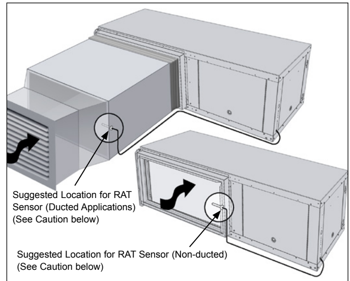
Figure 30: Return Air Temperature sensor (RAT) locations
