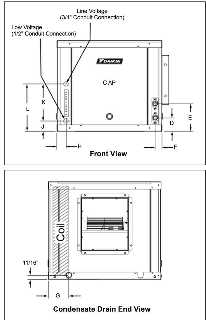
Figure 18: Piping & electrical connections locations
