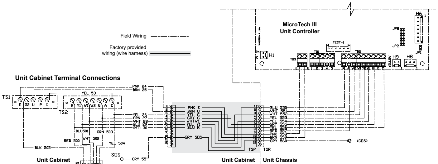
Figure 2: Wire harness kit wiring schematic
