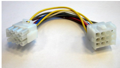
Figure 1: Wire harness kit – part number 910160410
