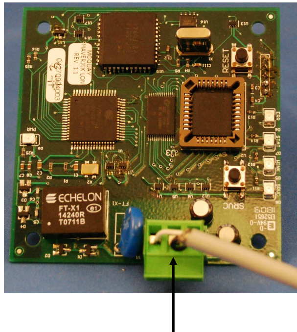
Network Connection (shown with 3-pin connector inserted)
