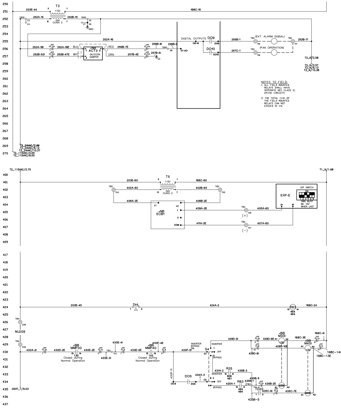
Figure 28 continued: RPS Electrical Diagram
