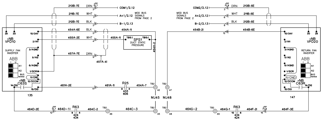
Figure 28 continued: RPS Electrical Diagram
