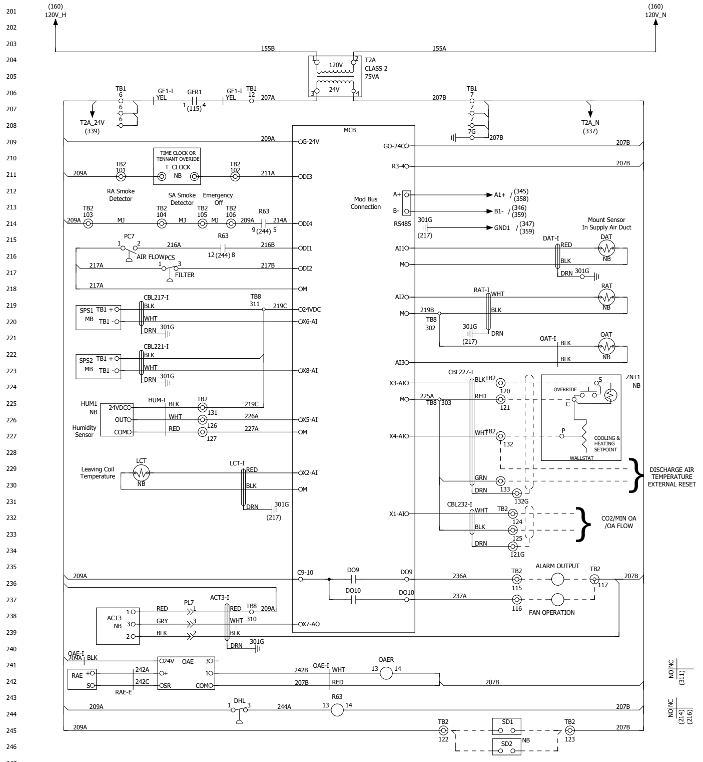
Figure 33 continued: Rebel Electrical Diagram
