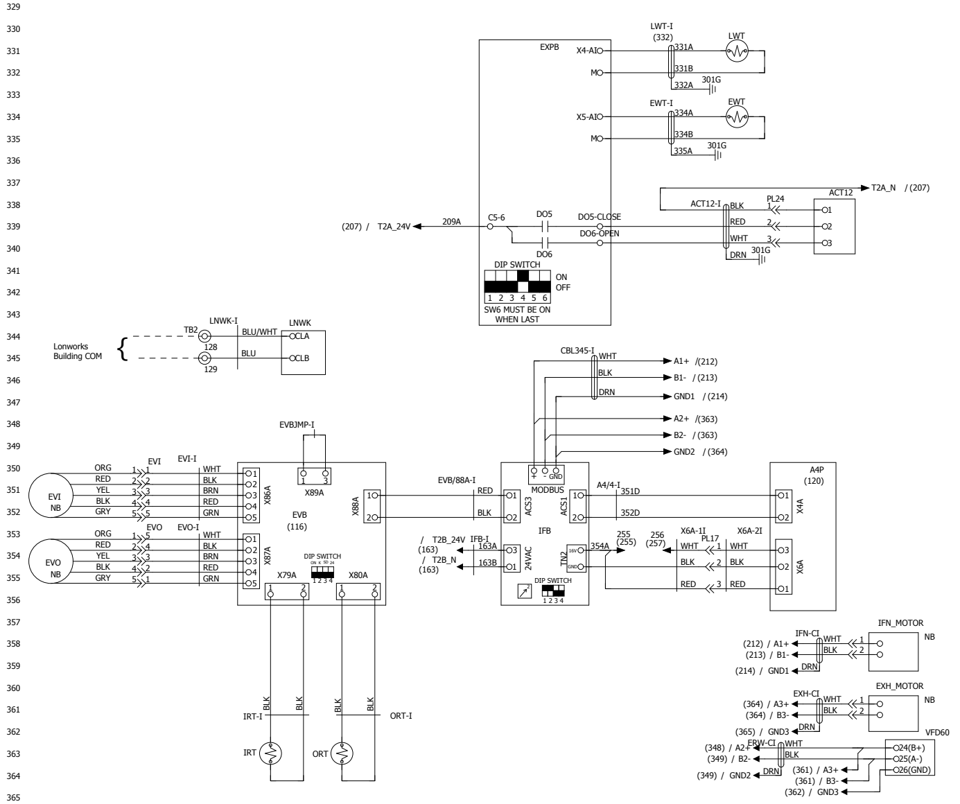
Figure 33 continued: Rebel Electrical Diagram
