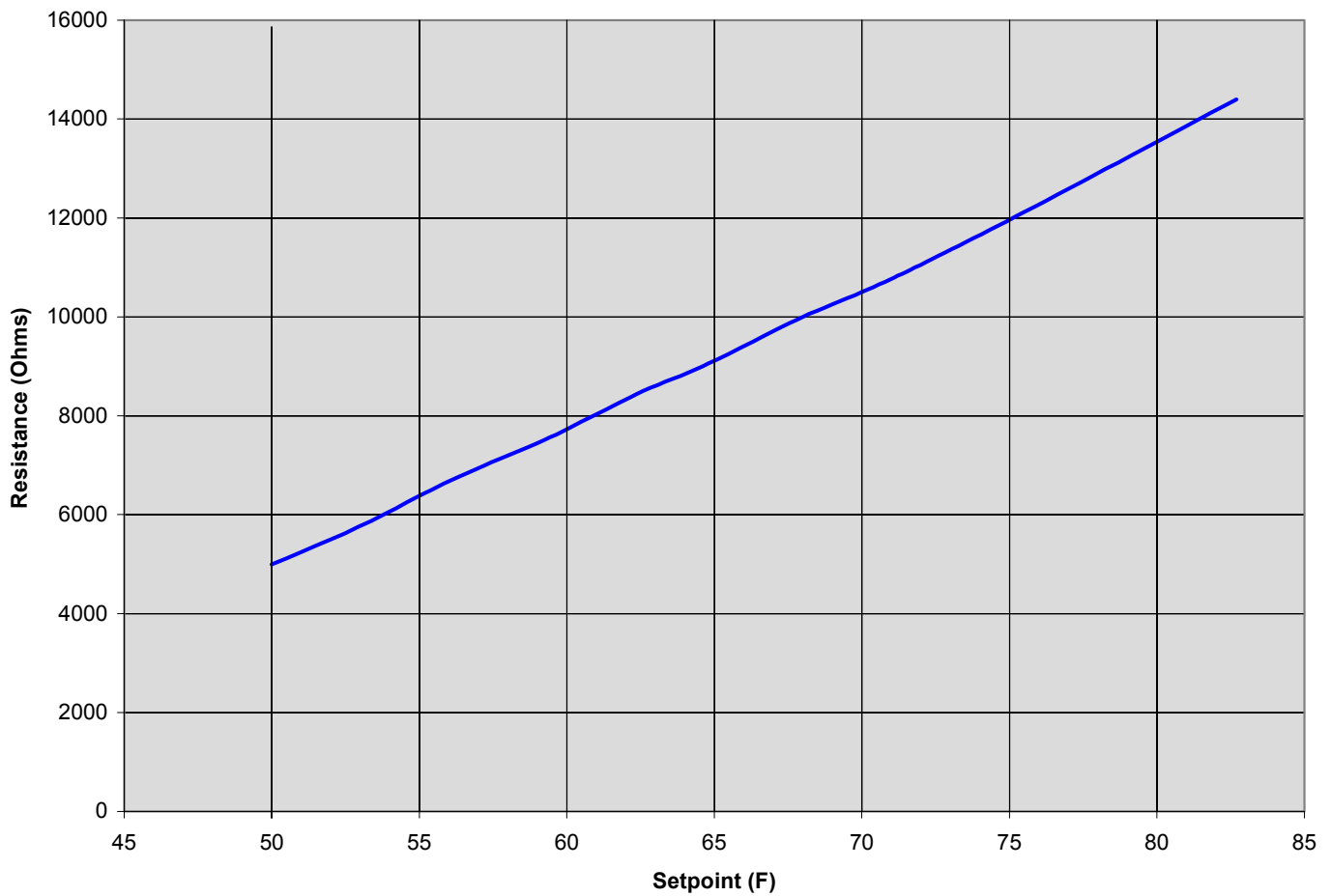
Figure 16: MicroTech III Wallstat Resistance vs. Setpoint
