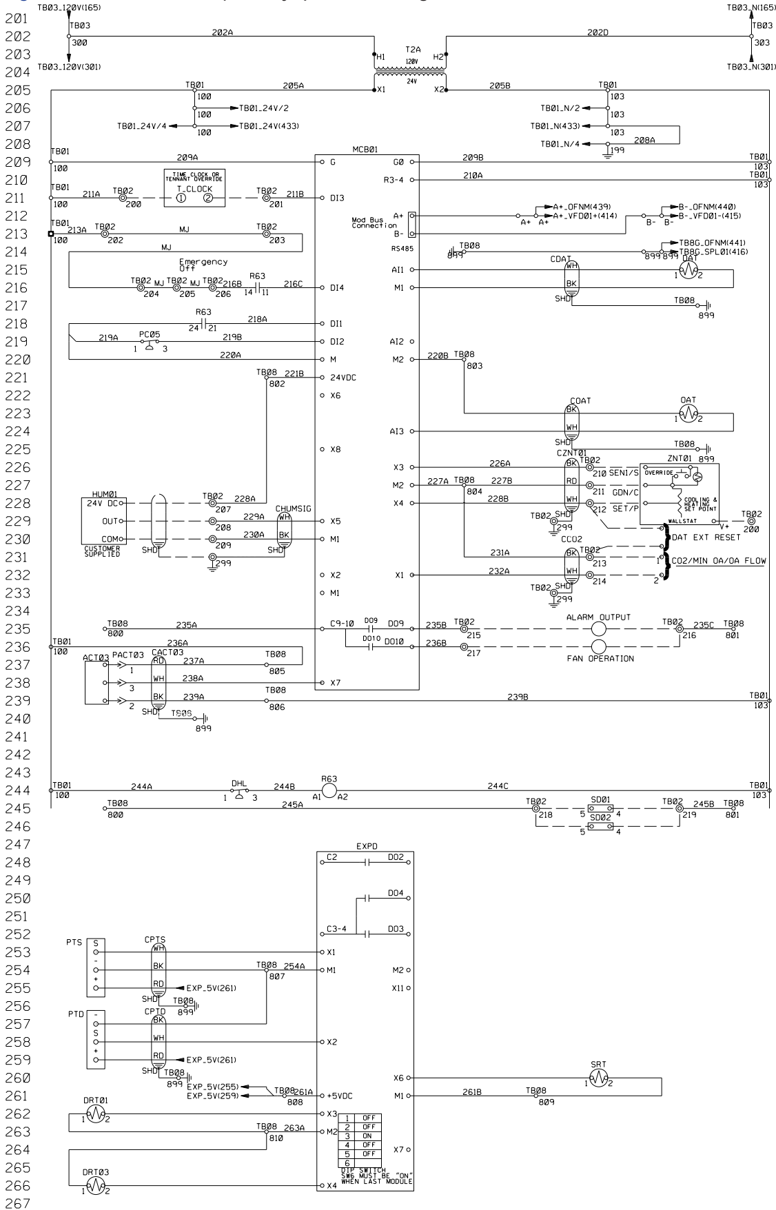
Figure 34 continued: Rebel (New Style) Electrical Diagram
