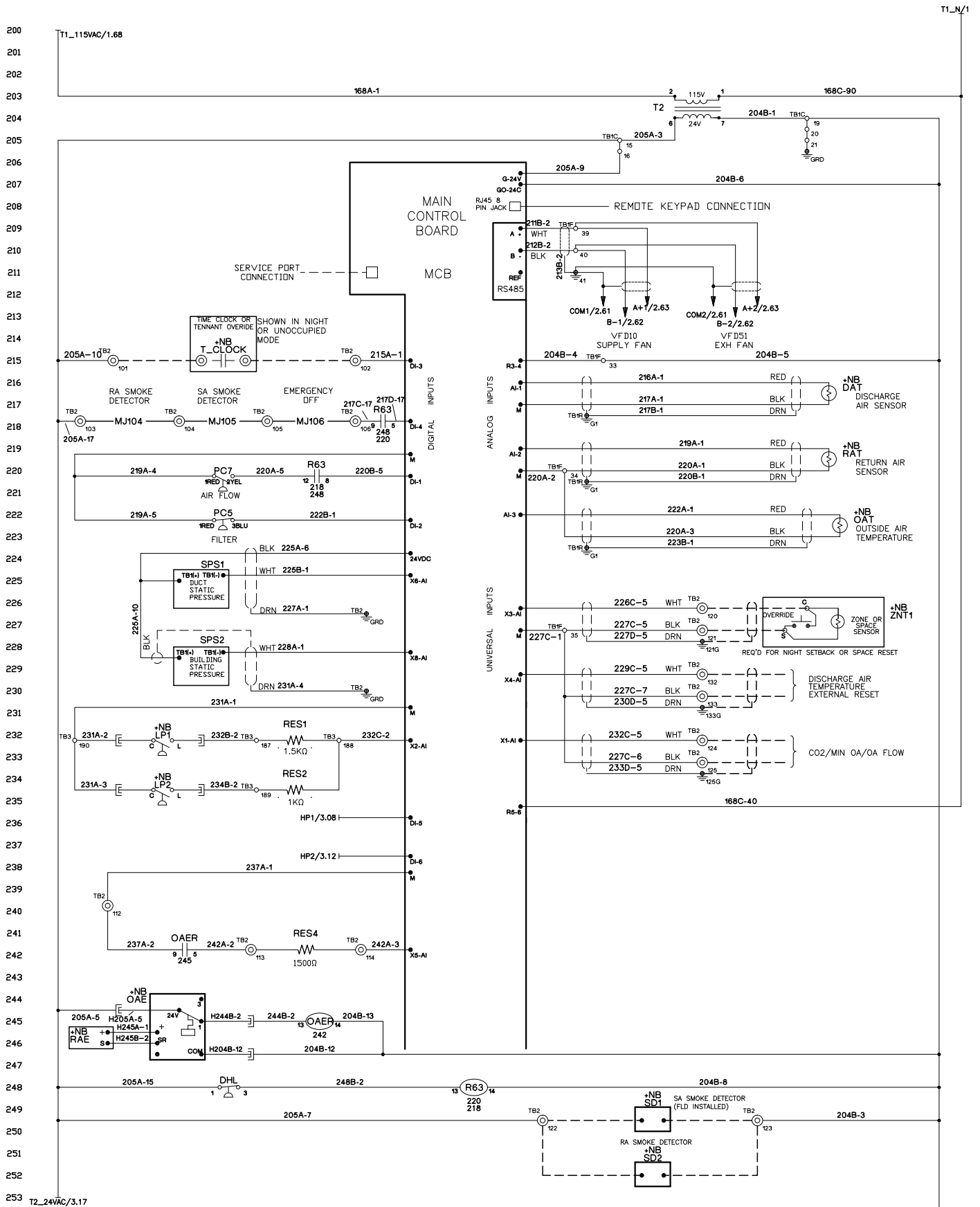
Figure 32 continued: Maverick Electrical Diagram
