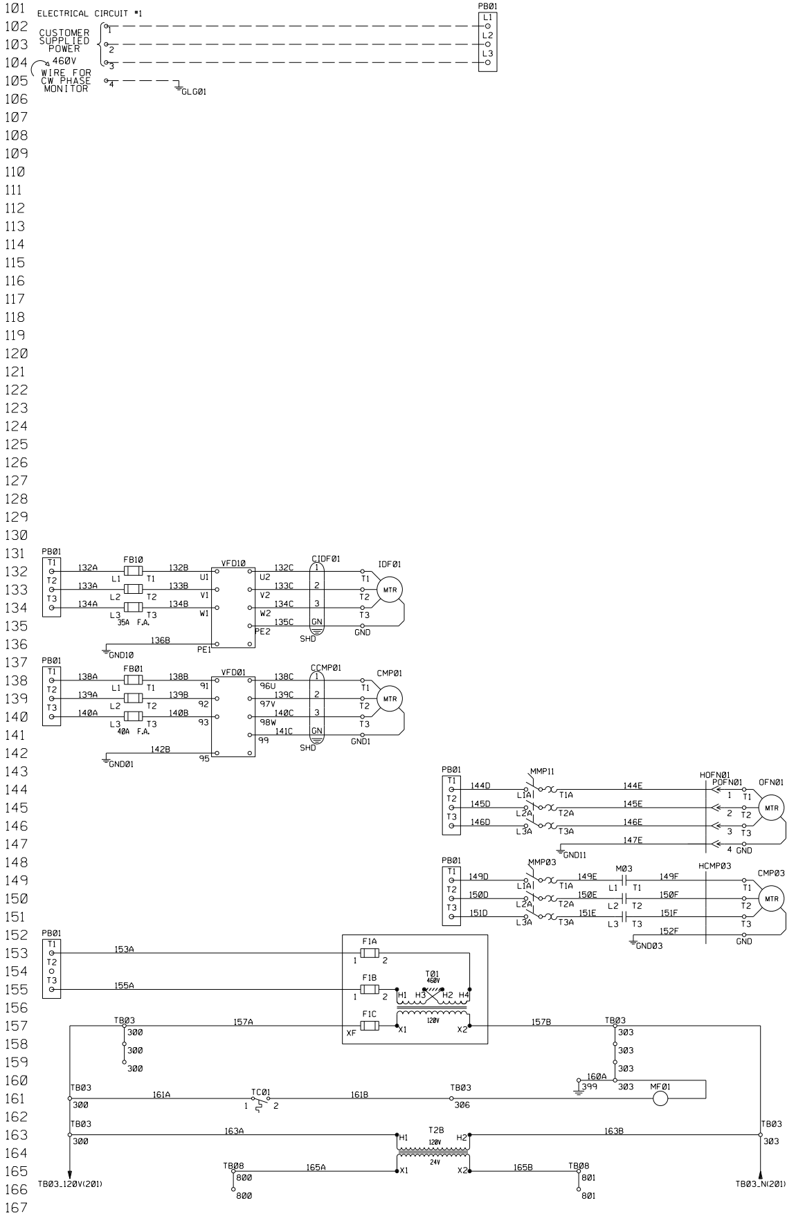
Figure 34: Rebel (New Style 16 to 28 Ton) Electrical Diagram
