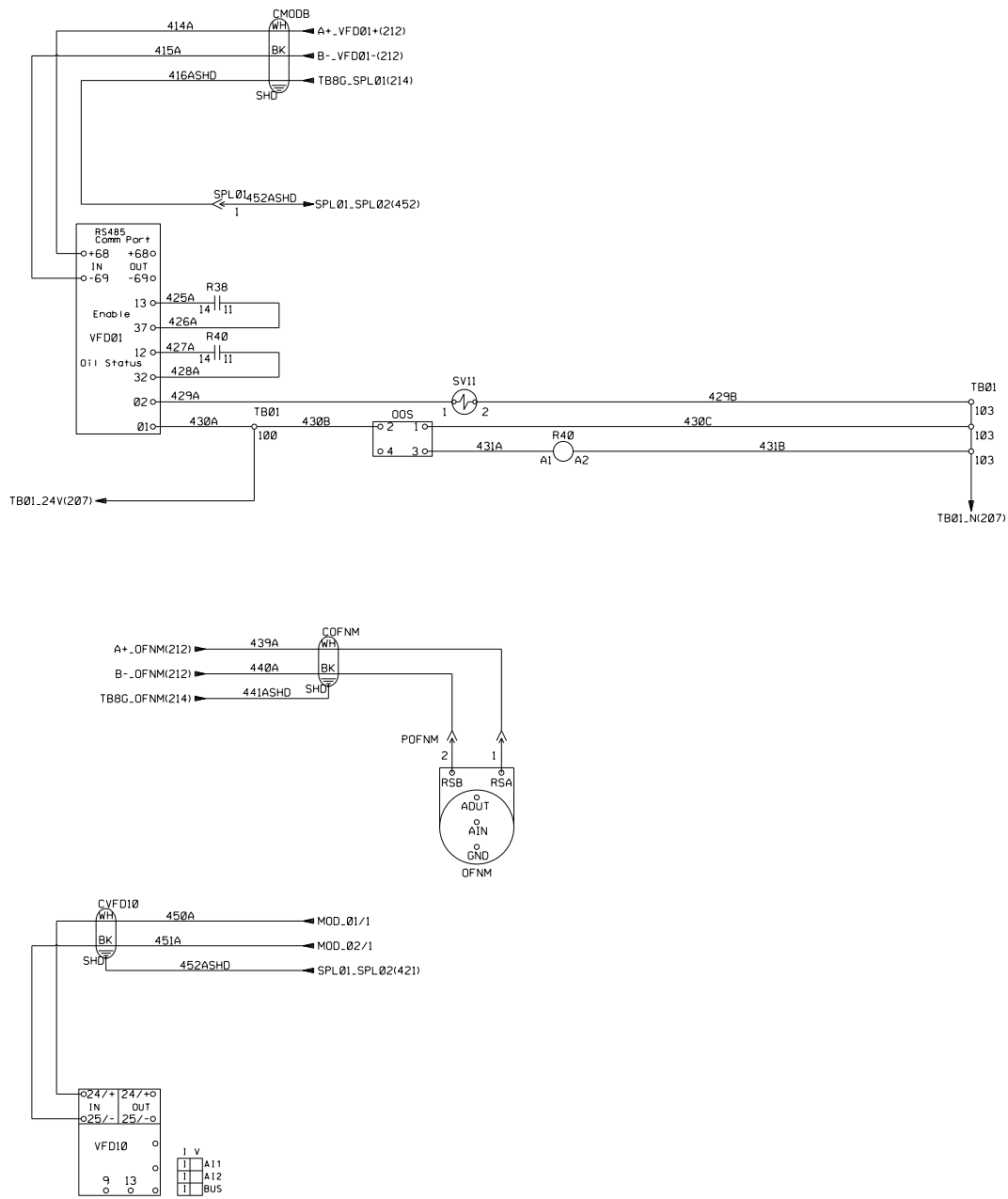
Figure 34 continued: Rebel (New Style) Electrical Diagram
