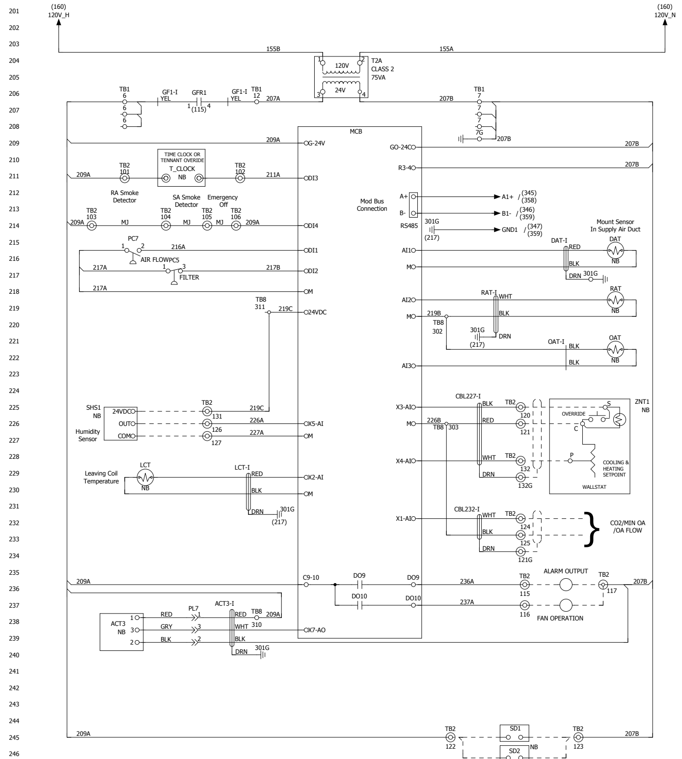
Figure 33 continued: Rebel Electrical Diagram
