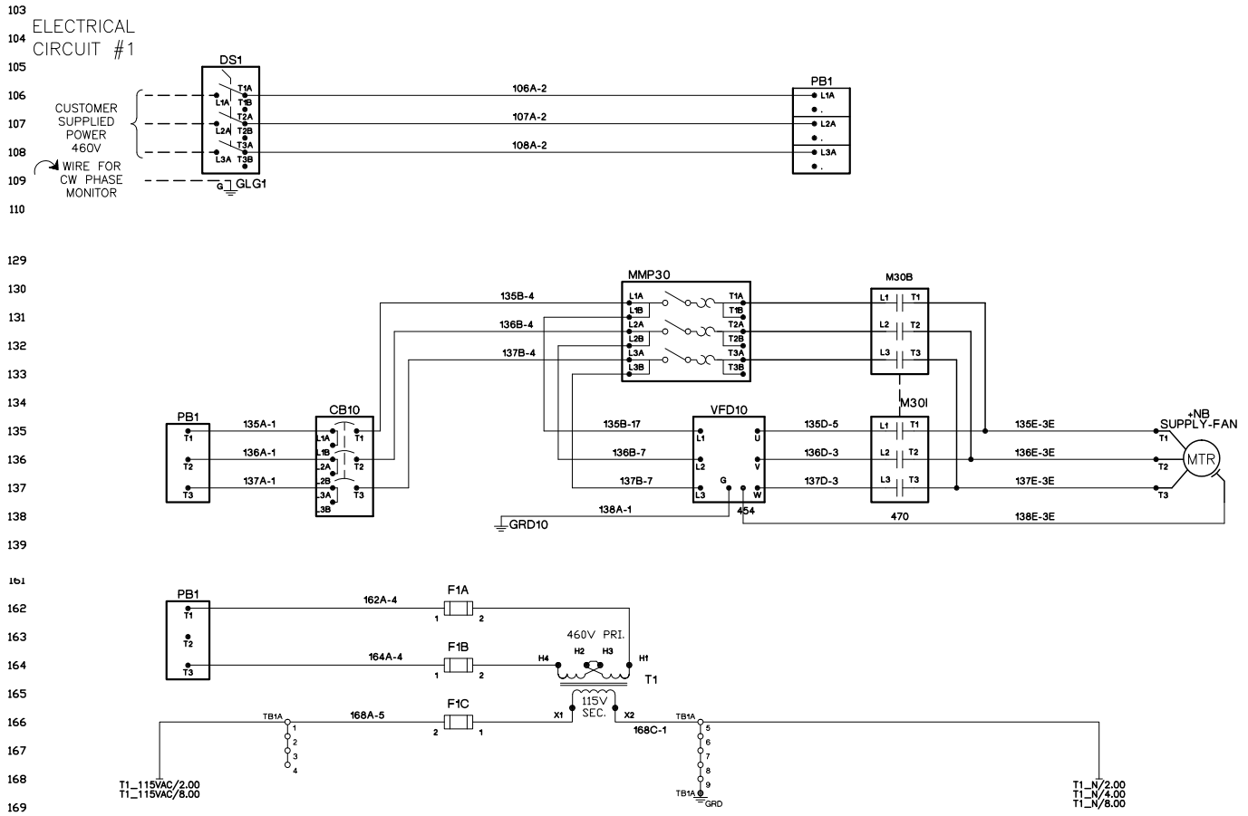
Figure 35: Self-Contained Electrical Diagram
