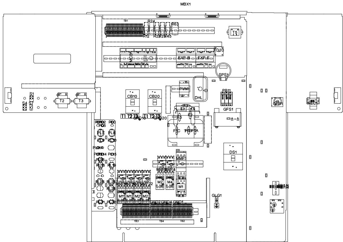
Figure 31: RPS Electrical Panel
