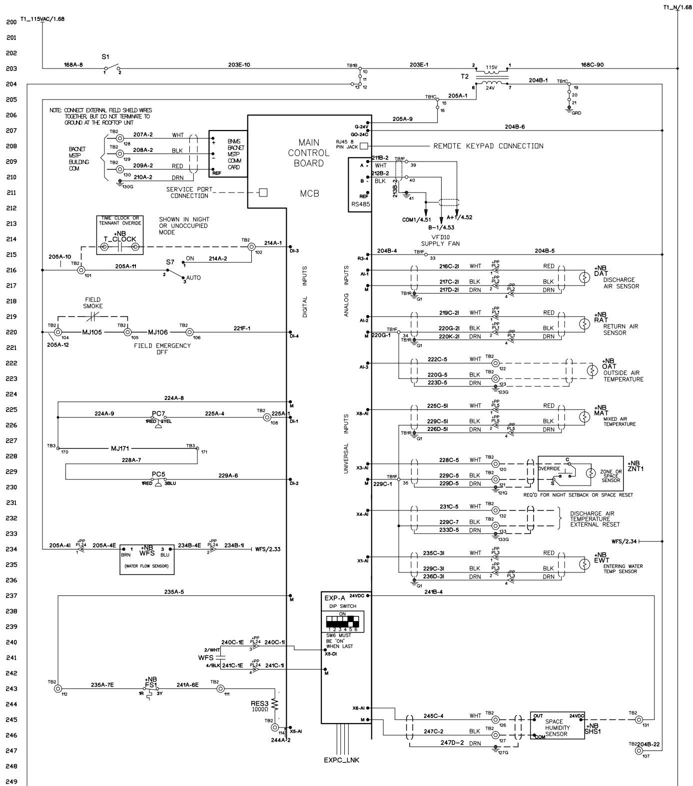
Figure 35 continued: Self-Contained Electrical Diagram
