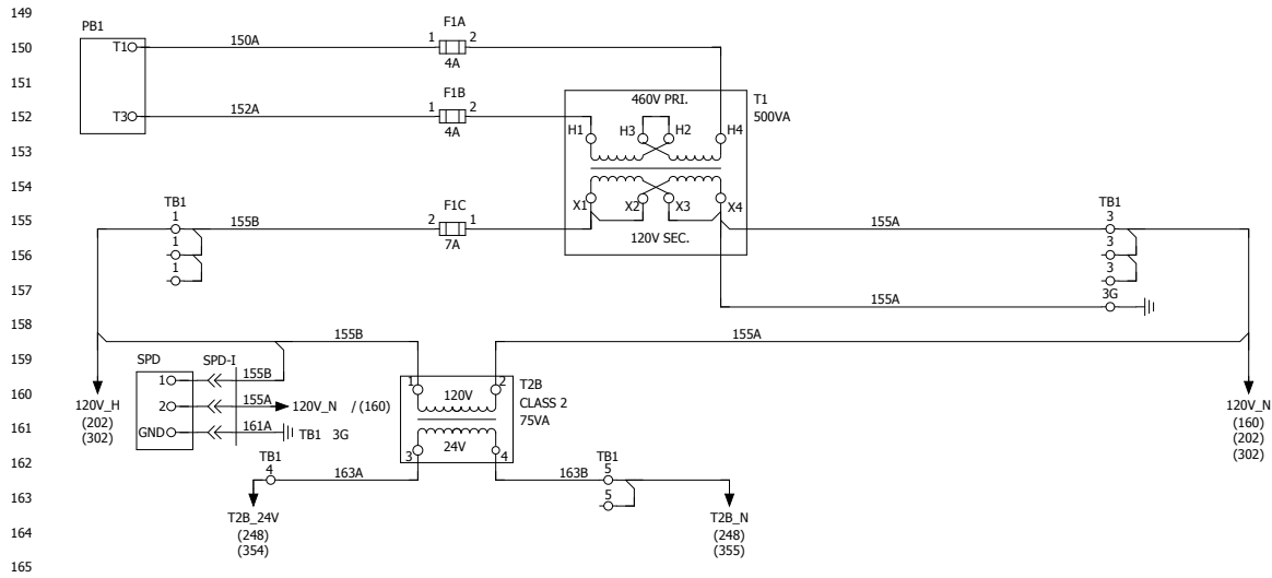
Figure 33 continued: Rebel Electrical Diagram
