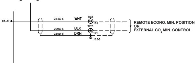
Figure 24: External Outdoor Air Damper Reset Signal Wiring Diagram
