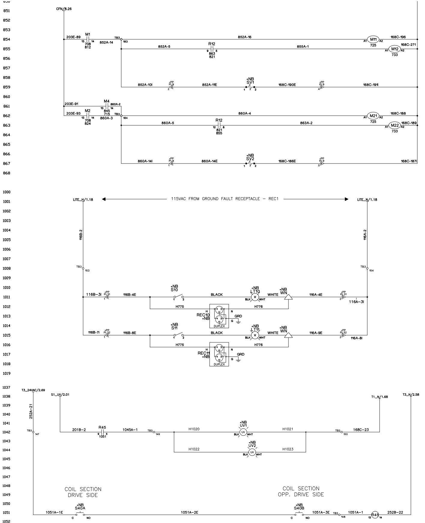
Figure 29 continued: RPS with Fixed Speed Scroll Compressors
