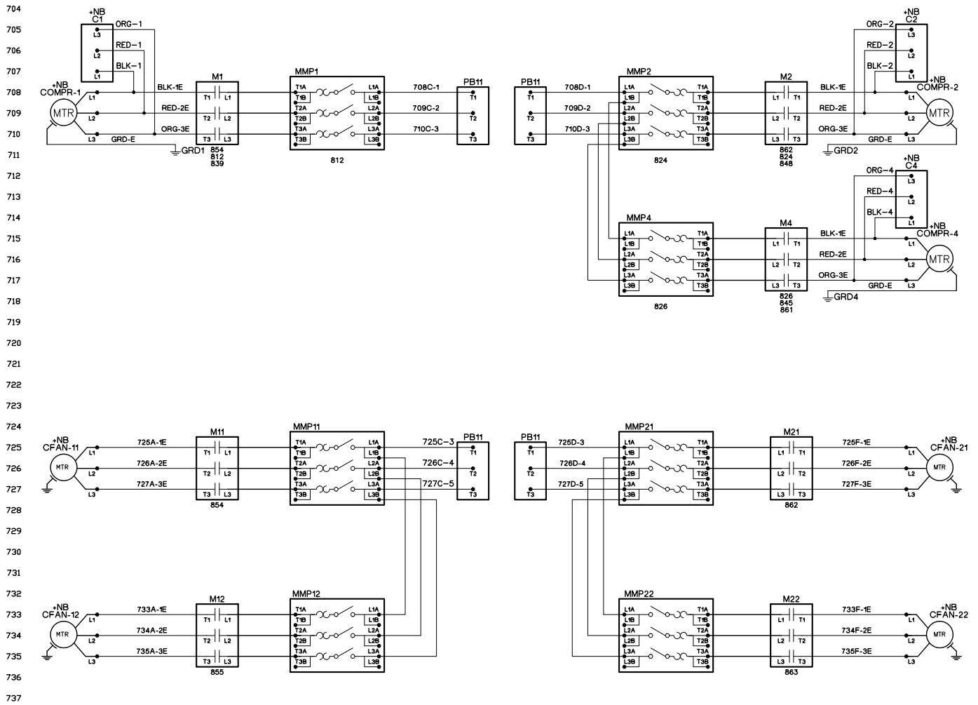
Figure 29: RPS with Fixed Speed Scroll Compressors
