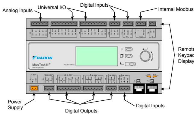
Figure 1: Main Control Board
