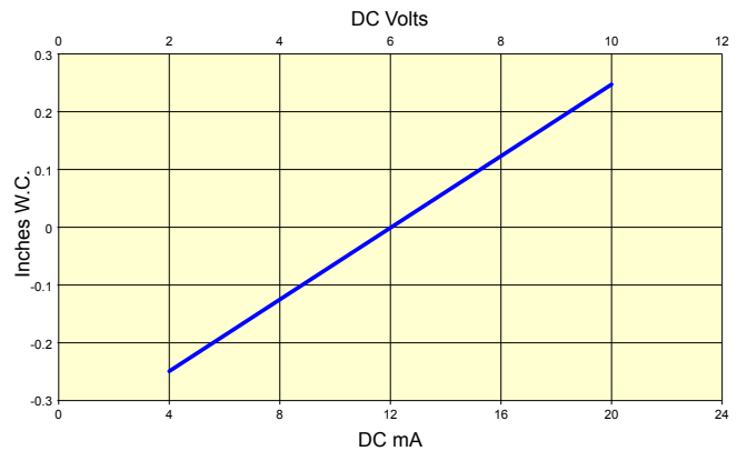
Figure 10: Building Pressure Sensor Output
