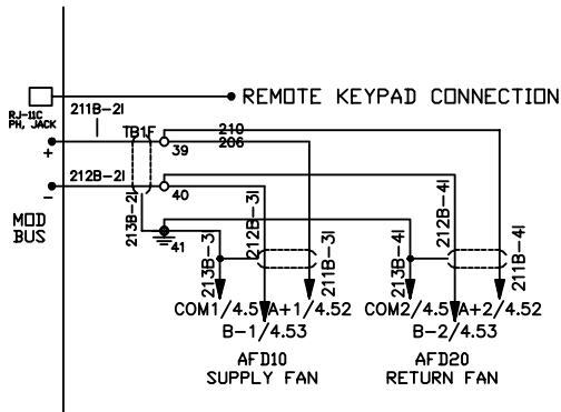
Figure 14: VFD Wiring Diagram
