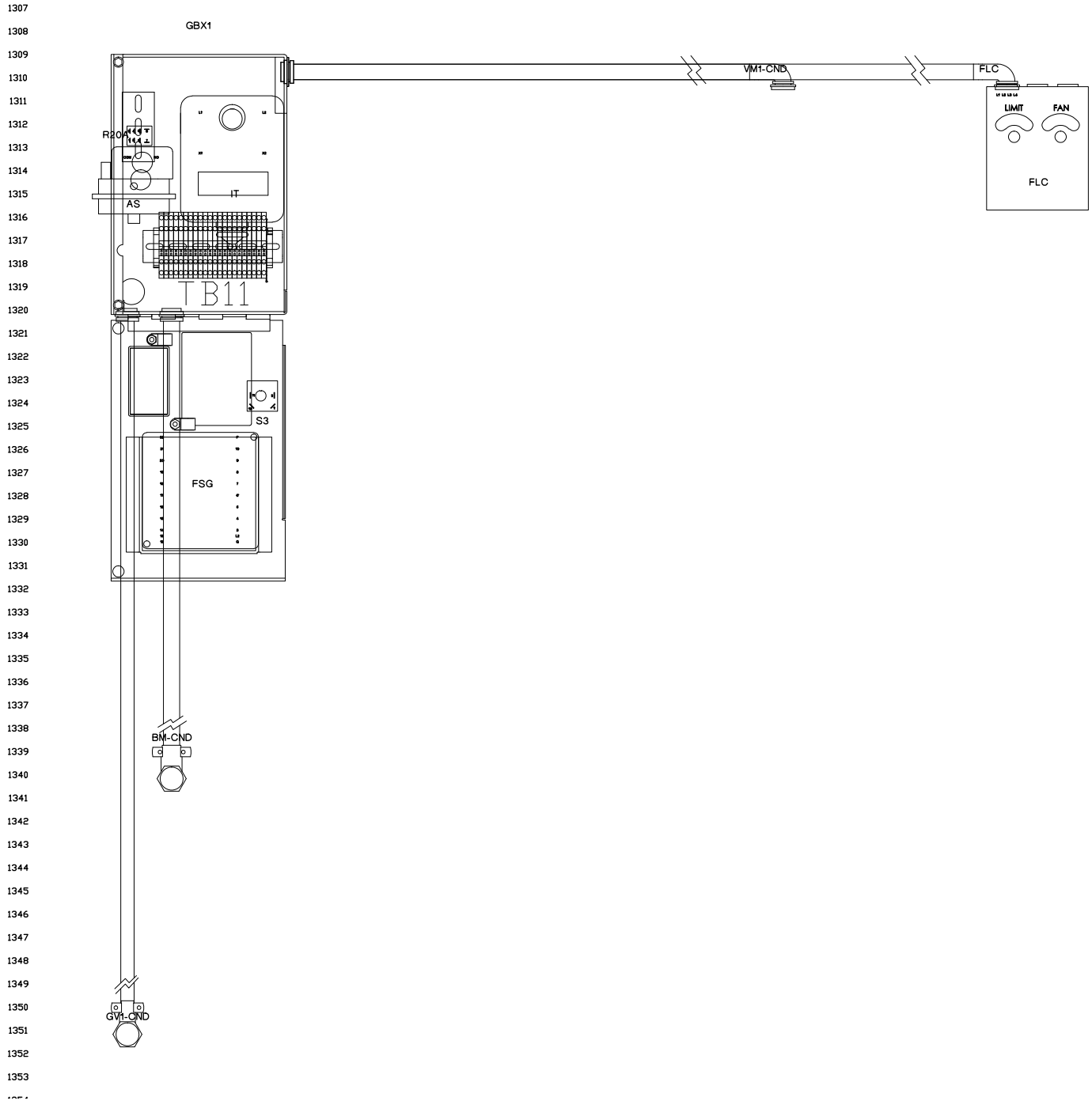
Figure 31 continued: RPS Electrical Panel
