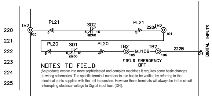
Figure 27: Emergency Shutdown Wiring Diagram
