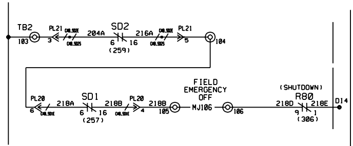
Figure 15: Smoke Detector Wiring Diagram
