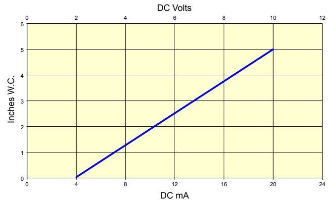
Figure 8: Duct Pressure Sensor Output
