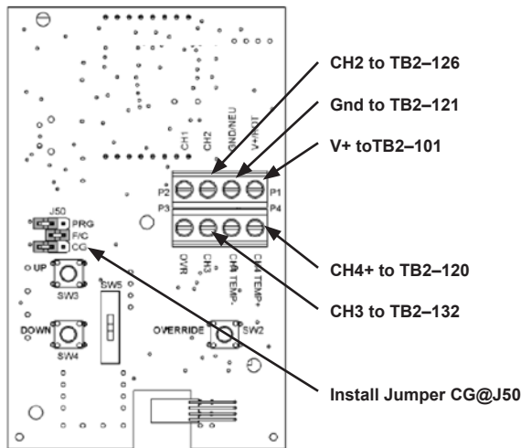
Figure 19: Rebel DPS 3 to 15 Ton MicroTech III Wiring
