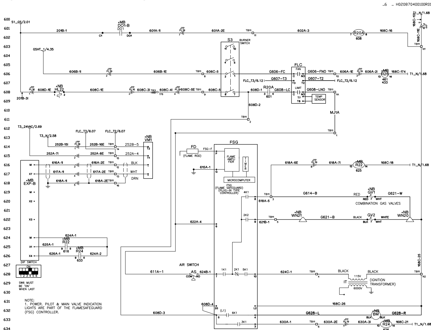
Figure 28 continued: RPS Electrical Diagram
