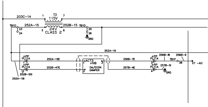
Figure 13: Actuator Wiring Diagram
