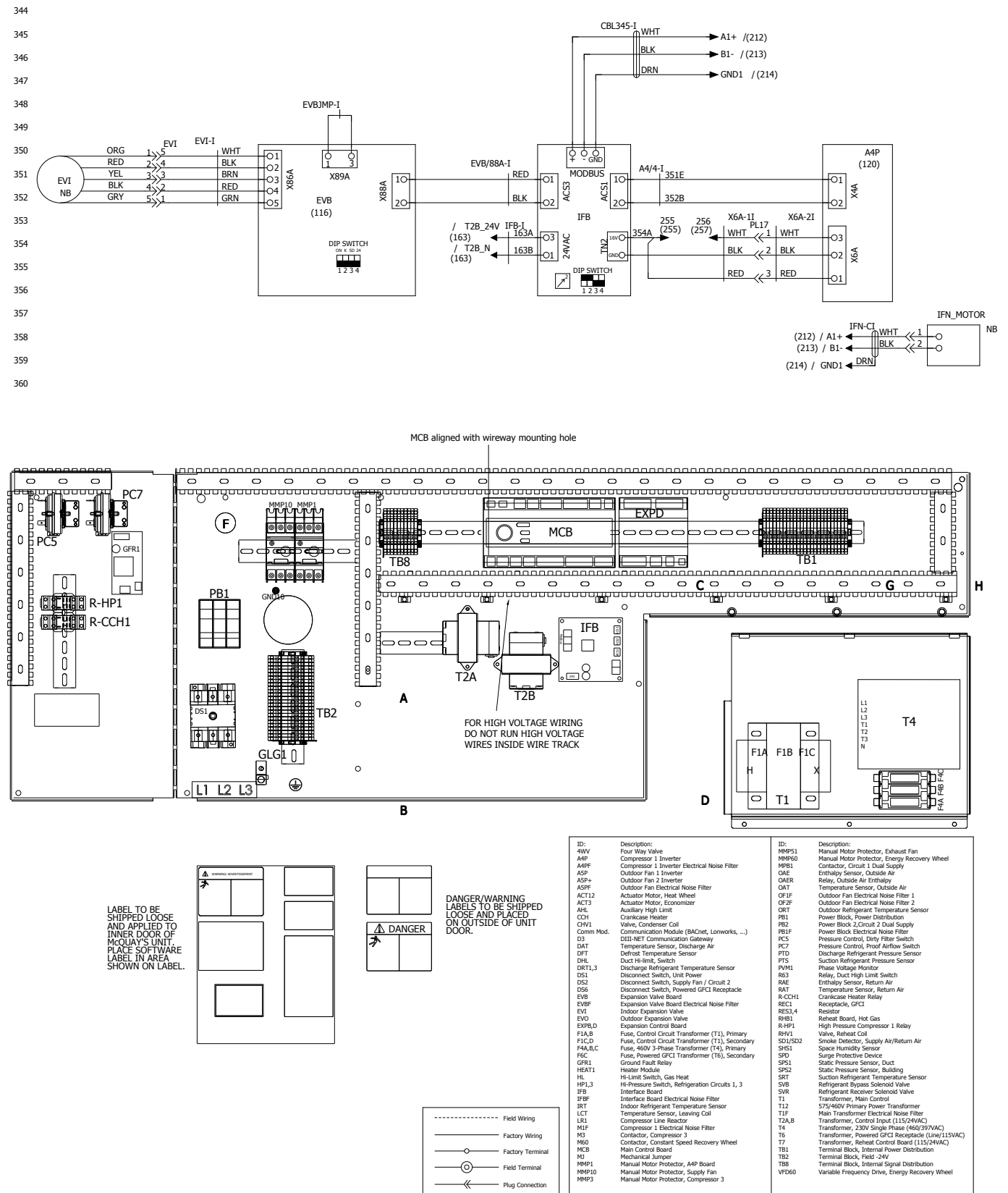
Figure 33 continued: Rebel Electrical Diagram
