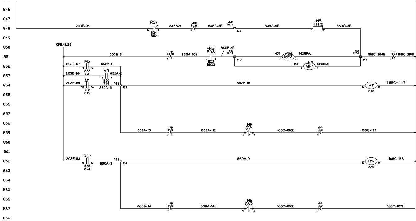
Figure 30 continued: RPS with Variable Speed Inverter Compressors
