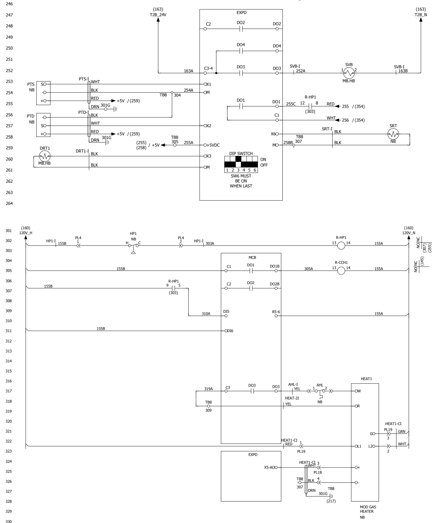
Figure 33 continued: Rebel Electrical Diagram
