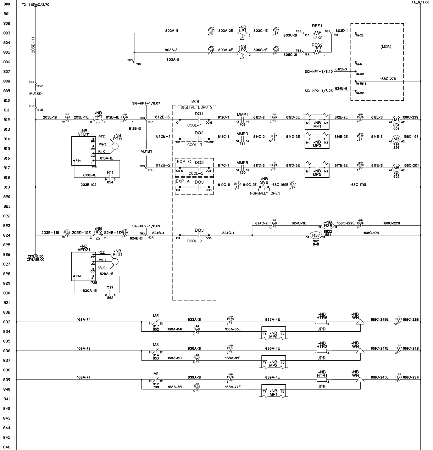
Figure 30: RPS with Variable Speed Inverter Compressors
