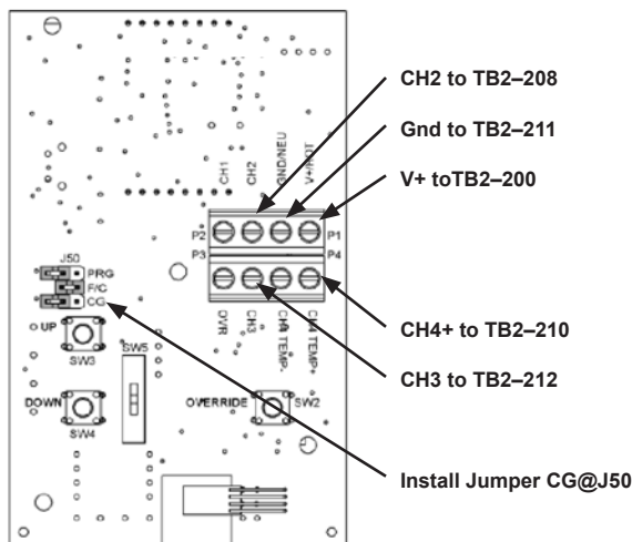
Figure 20: Rebel DPS 16 to 28 Ton MicroTech III Wiring
