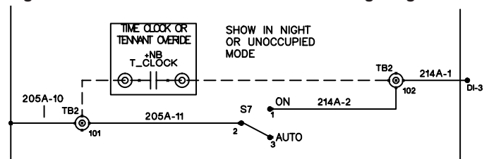
Figure 26: Time Clock/Tenant Override Wiring Diagram
