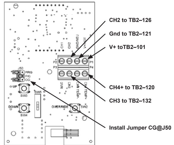
Figure 22: RoofPak RPS MicroTech III Wiring
