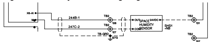
Figure 25: Humidity Sensor Wiring Diagram
