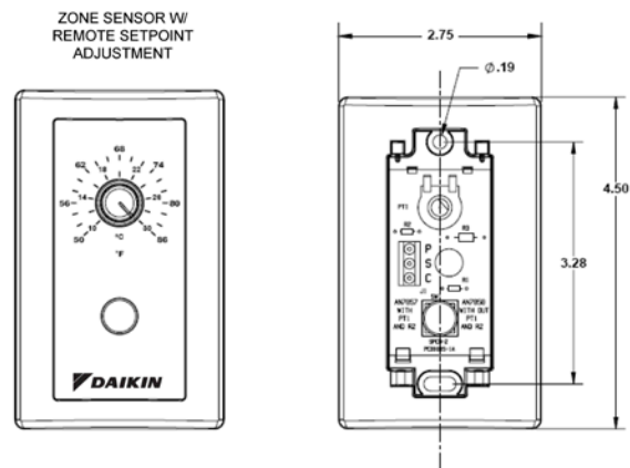
Figure 18: Zone Sensor with Setpoint Adjustment
