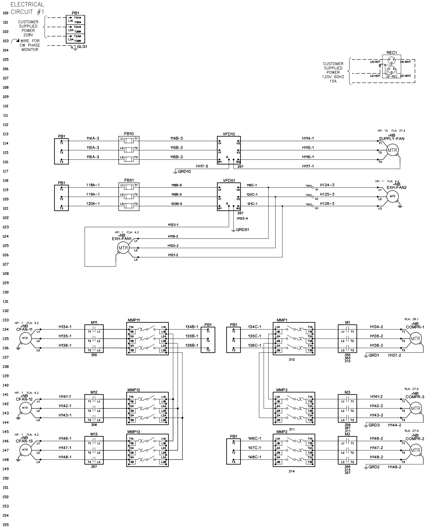
Figure 32: Maverick Electrical Diagram
