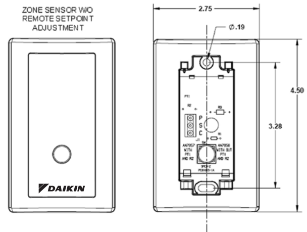
Figure 17: Zone Sensor without Setpoint Adjustment
