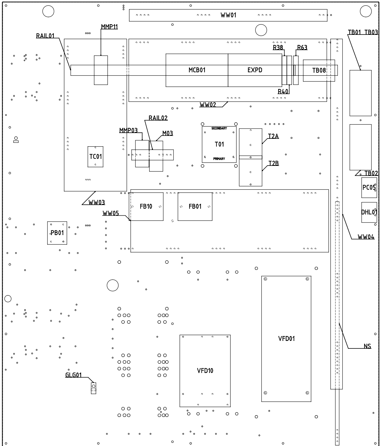
Figure 34 continued: Rebel (New Style) Electrical Diagram
