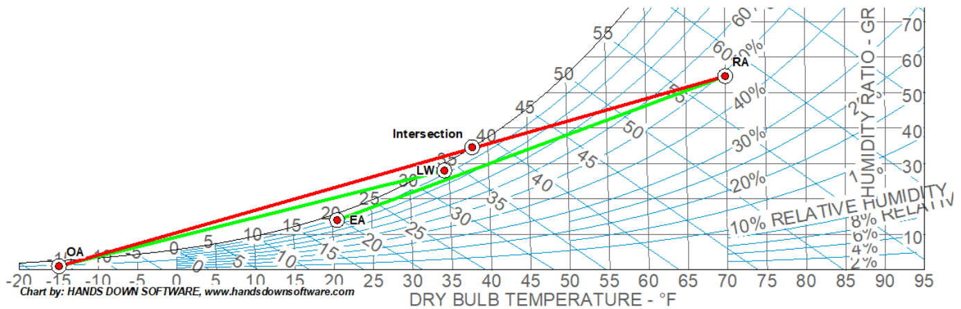
Figure 29: Frost Prevention Curve
