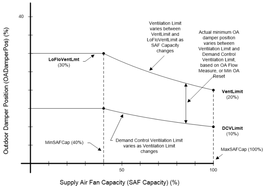
Figure 26: Outdoor Air Damper Reset
