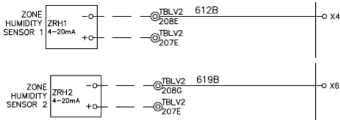
Figure 12: Humidity Sensors Wiring Diagram
