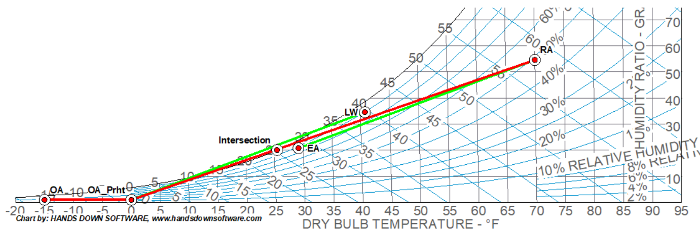
Figure 31: Modulating Wheel Preheat Frost Prevention Curve
