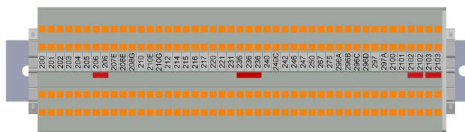
Figure 7: Graphical Representation of TB2
