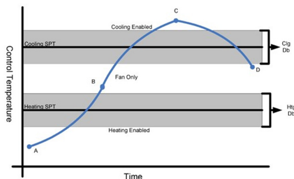
Figure 18: Heating/Cooling Control Temperature
