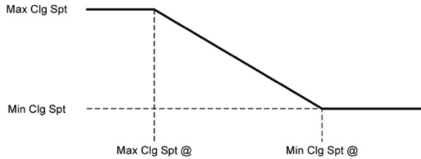
Figure 20: Cooling DAT Setpoints
