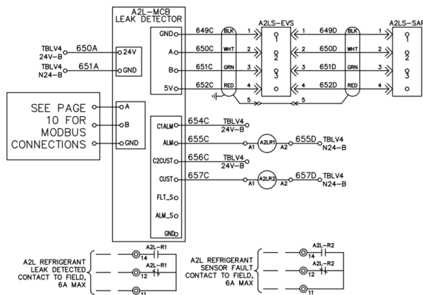
Figure 32: A2L Leak Detector Schematic Sample
