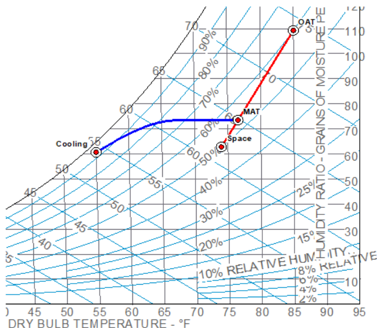
Figure 22: Cooling/Dehumidification Psychrometric Charts
