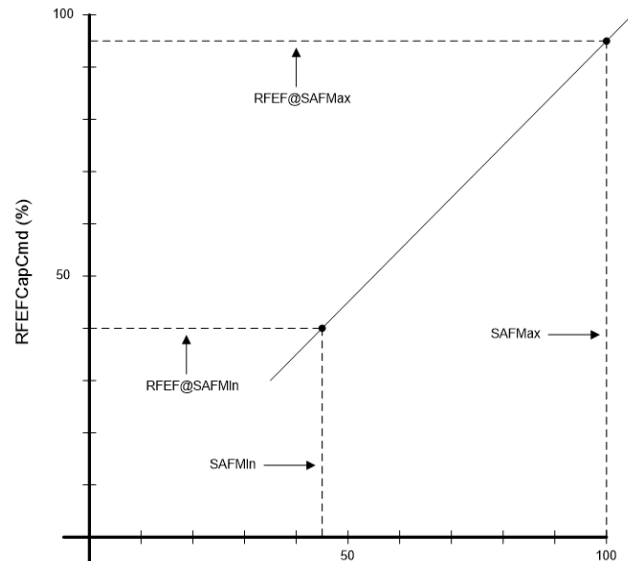
Figure 19: Return/Exhaust Fan Tracking
