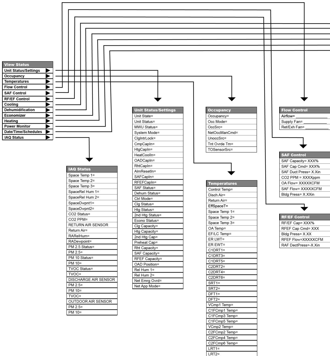
Figure 5: View Status Menu Structure
