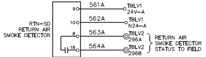
Figure 14: Smoke Detector Wiring Diagram
