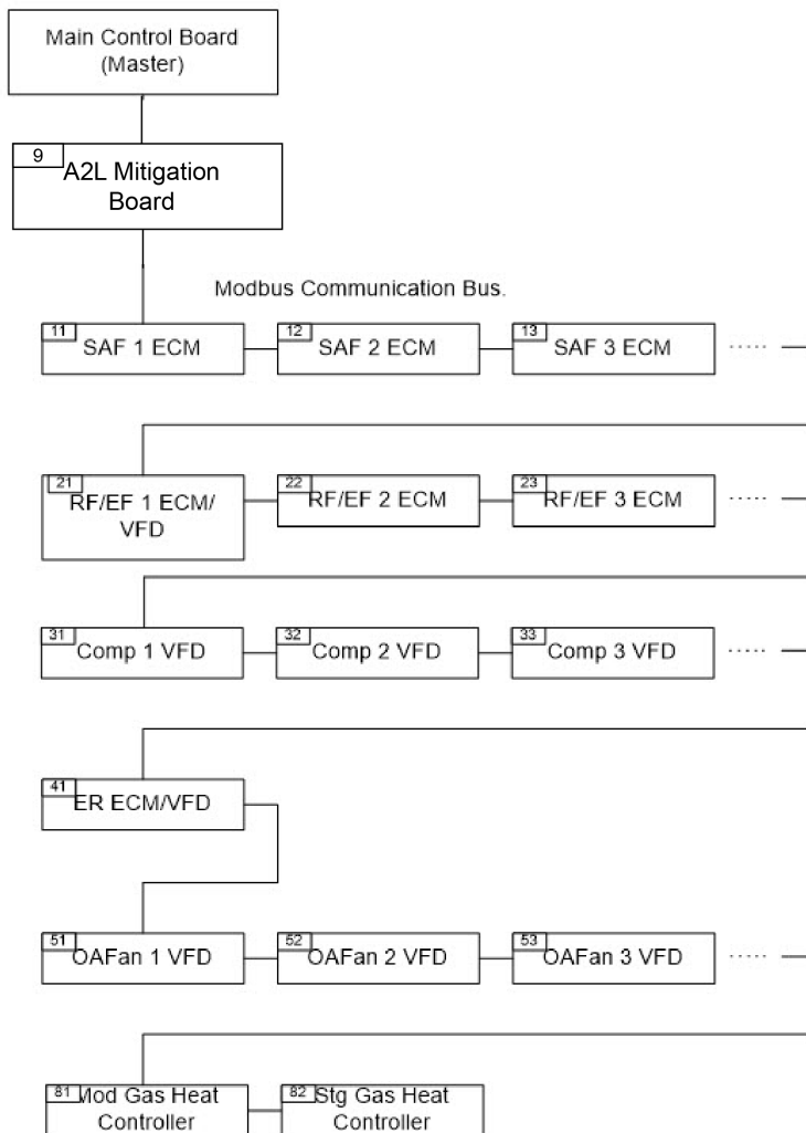
Figure 33: Modbus Network Configuration
