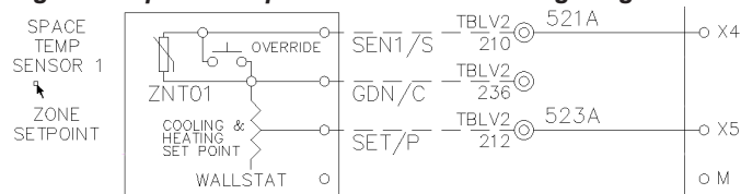
Figure 8: Space Temperature Sensors Wiring Diagram
