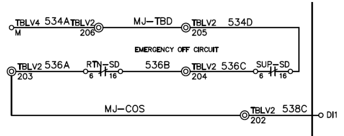
Figure 13: Emergency Off Circuit Wiring Diagram
