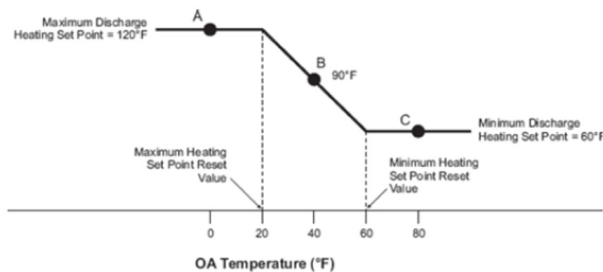
Figure 25: Heating DAT Reset
