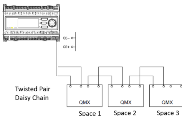
Figure 10: Wired Network Sensor Example
