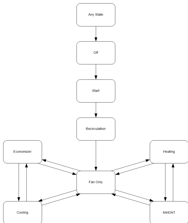
Figure 17: Unit State Diagram
