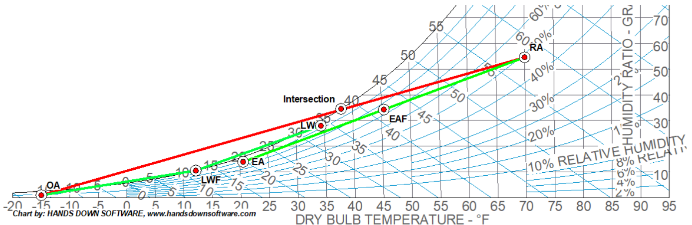
Figure 30: Modulating Wheel Frost Prevention Curve
