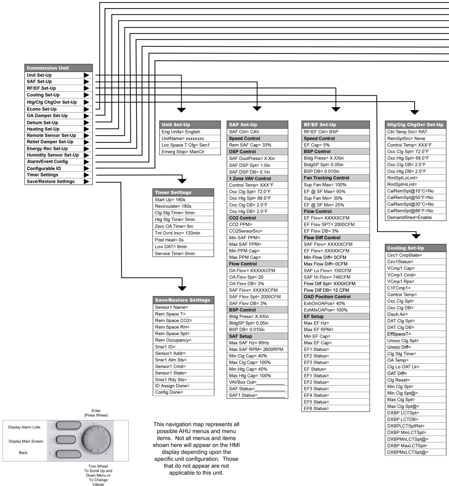
Figure 6: Commission Unit Menu Structure
