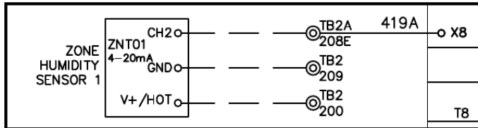
Figure 15: Humidity Sensor 1 Wiring Diagram
