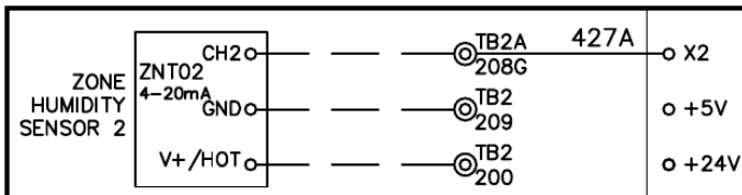
Figure 16: Humidity Sensor 2 Wiring Diagram
