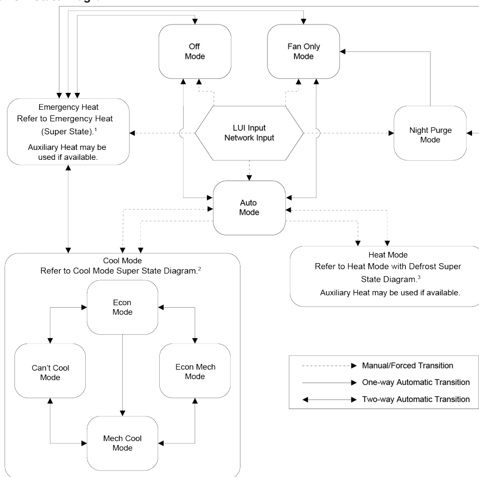
Figure 2: Complete UVC—State Diagram
