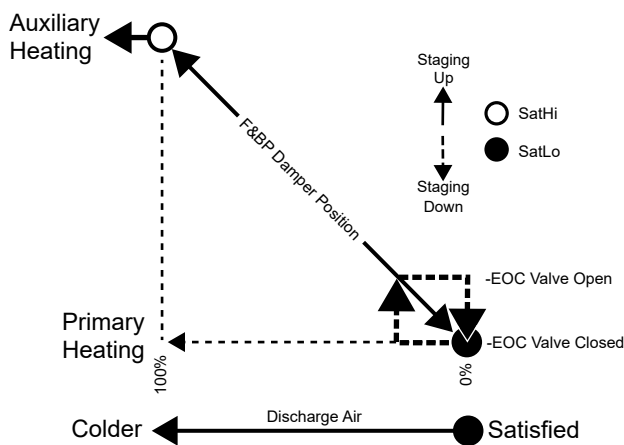
Figure 9: Heat State Operation Face & Bypass Heating
