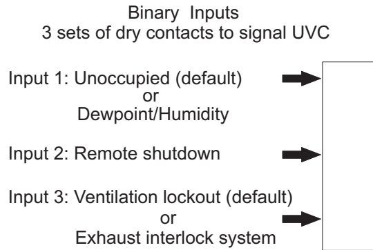
Figure 23: Binary Inputs
