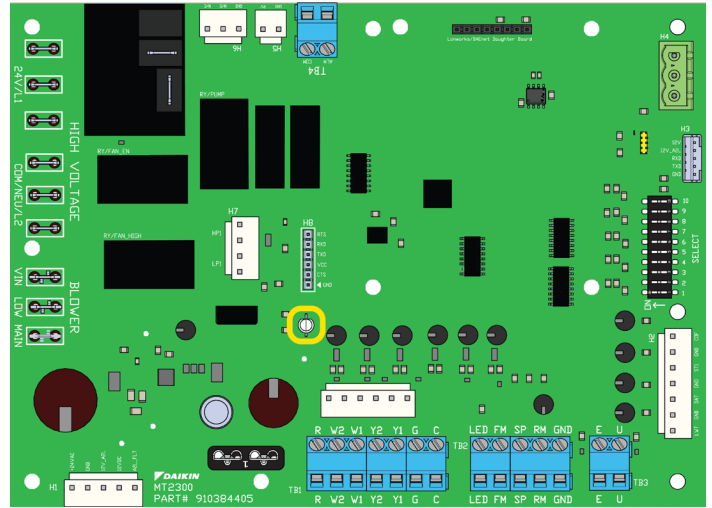
Figure 6: LED Indicator on MT2300 Board
