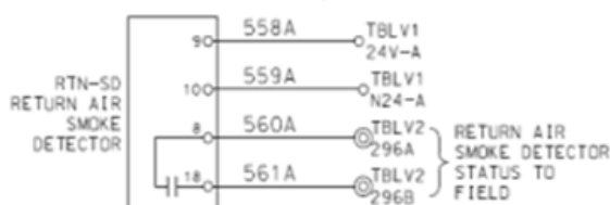
Figure 15: Smoke Detector Output Schematics
