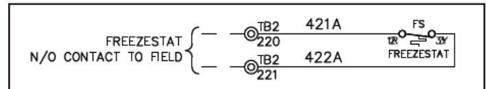
Figure 35: Outdoor Humidity Schematic
