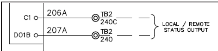
Figure 21: Local Remote Status Schematic
