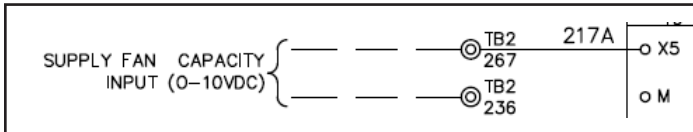
Figure 2: Supply Fan Capacity Input Schematic
