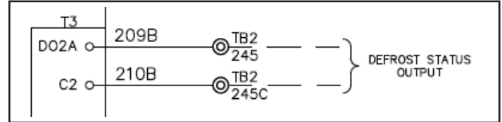
Figure 10: Defrost Status Schematic
