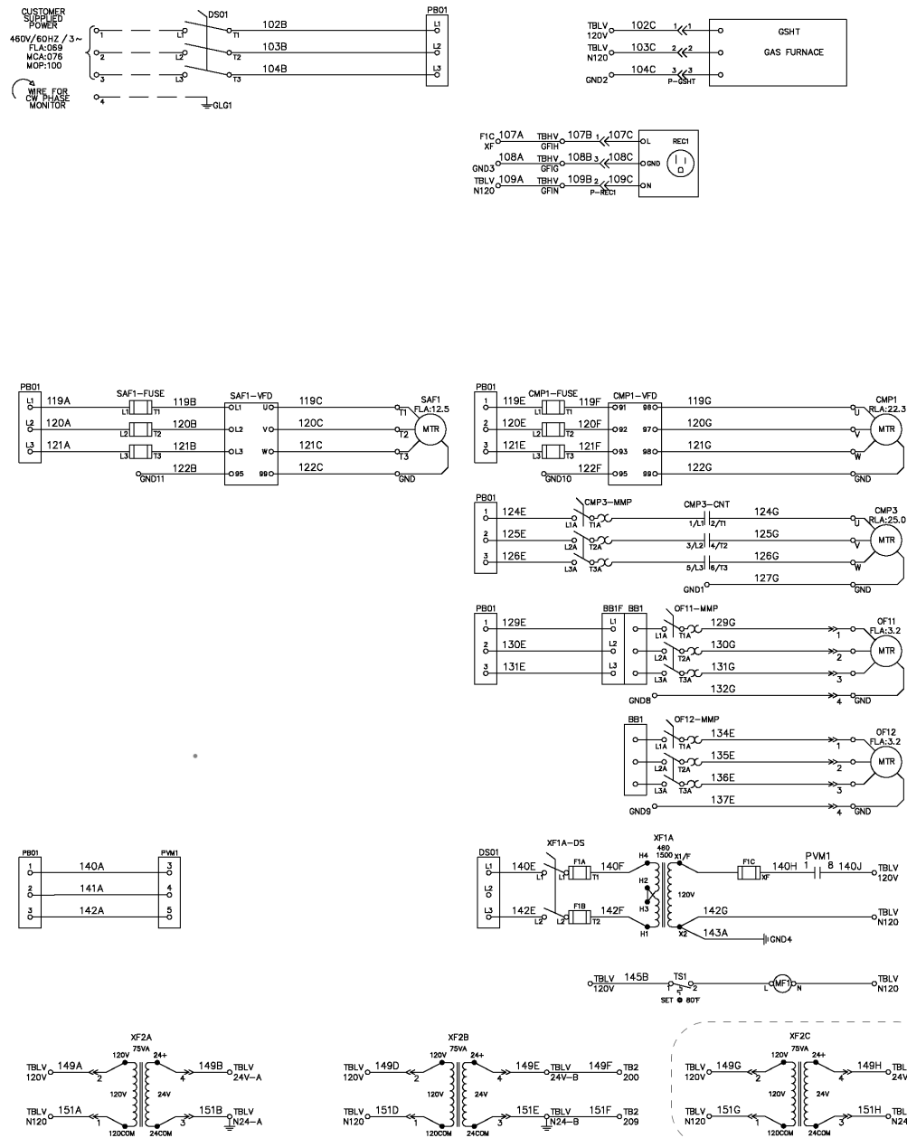
Figure 37: Sample Wiring Diagram (1)
