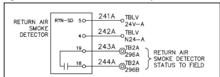
Figure 15: Return Air Smoke Detector Output Schematics
