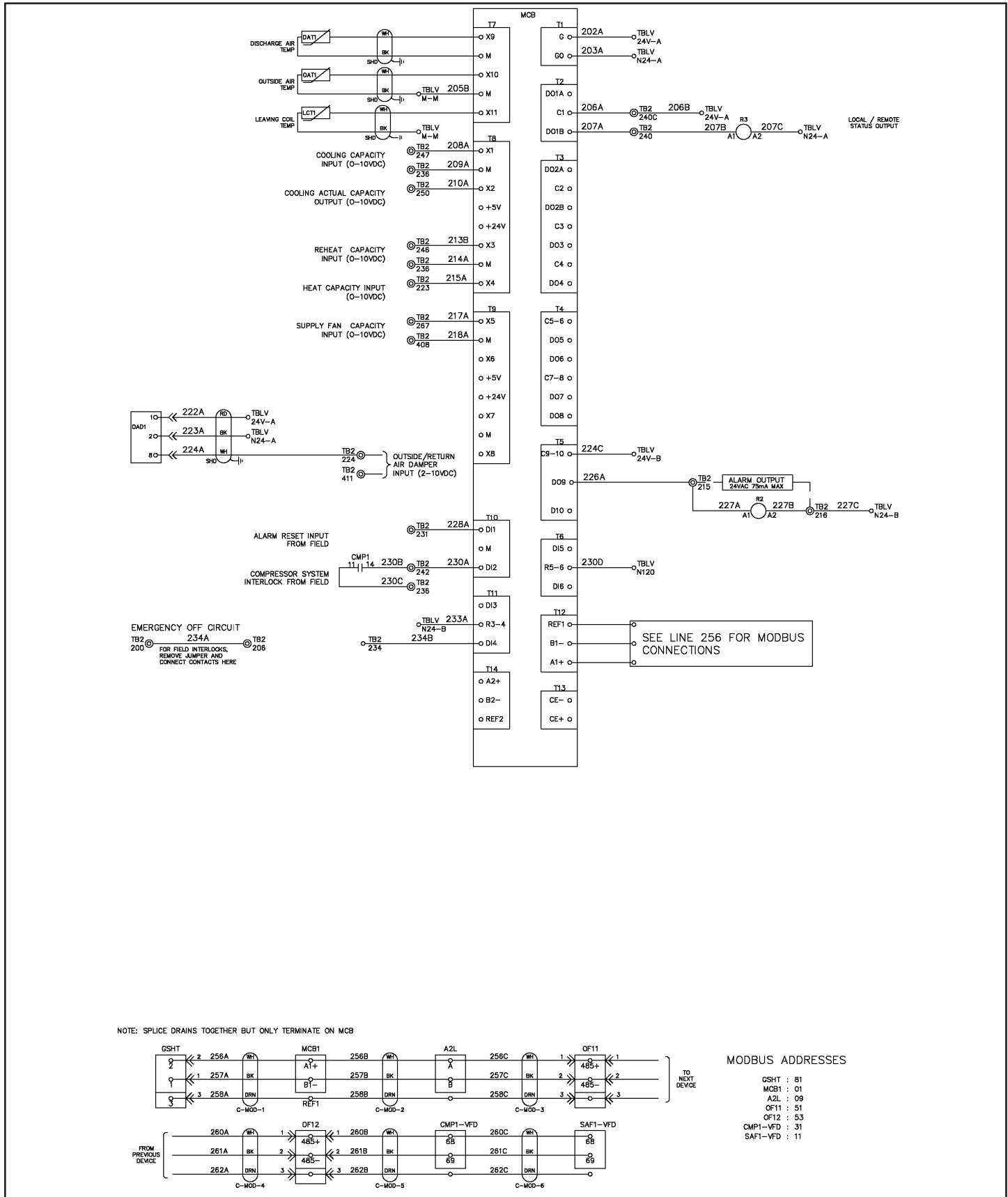
Figure 38: Sample Wiring Diagram (2)
