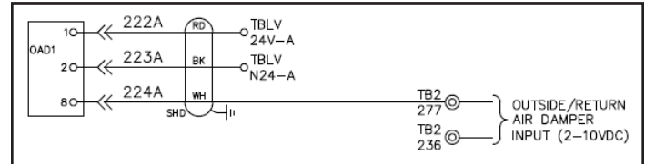
Figure 4: Outside Air Damper Operation Schematic (2)
