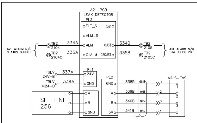
Figure 42: A2L Leak Detector Schematic Sample
