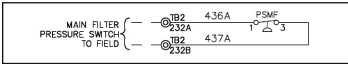
Figure 18: Main Filter Pressure Transducer Schematic
