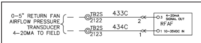
Figure 30: Return Fan Air Flow Schematic
