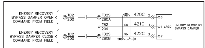
Figure 24: Bypass Damper Schematic
