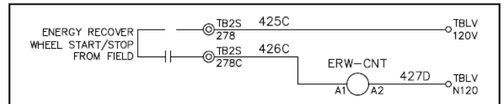
Figure 23: Energy Recovery Wheel Schematic (Start/Stop Contactors)
