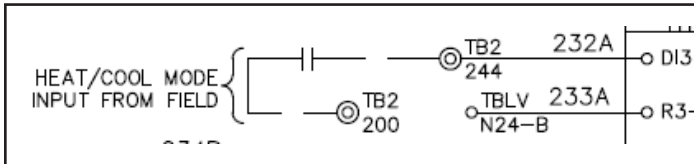
Figure 7: Heat/Cool Mode Input Schematic
