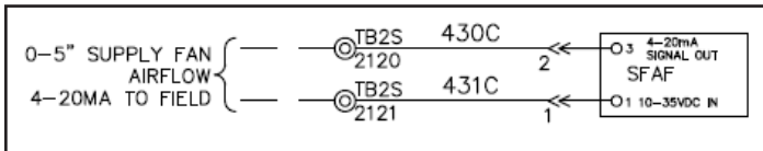
Figure 28: Supply Fan Air Flow Schematic
