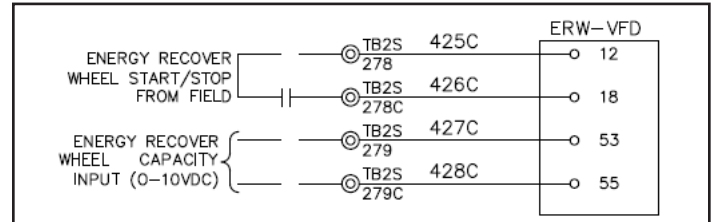
Figure 23: Energy Recovery Wheel Schematic (Start/Stop Contactors)
