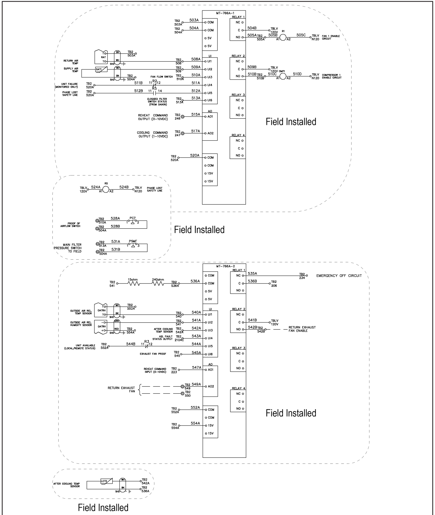
Figure 41: Sample Wiring Diagram (5)
