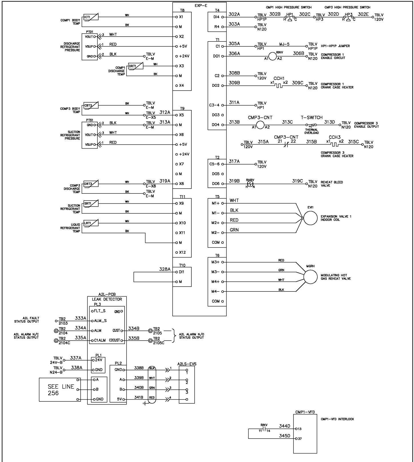
Figure 39: Sample Wiring Diagram (3)
