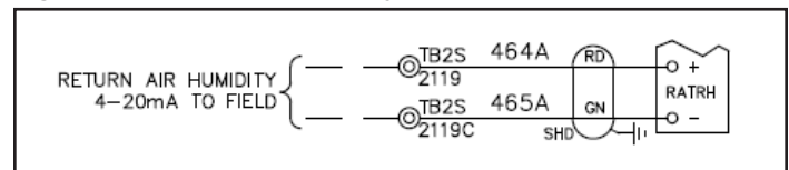
Figure 36: Return Air Humidity Schematic
