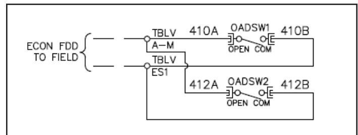
Figure 33: Economizer Fault Detection and Diagnostic Schematic
