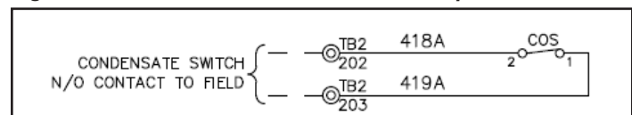
Figure 16: Condensate Overflow Switch Output Schematic
