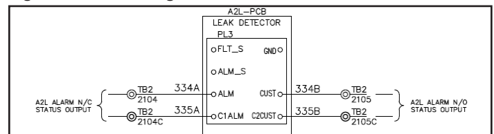
Figure 12: A2L Refrigerant Leak Alarm Schematic
