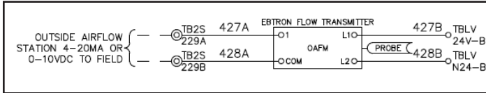
Figure 27: Outside Air Flow Schematic
