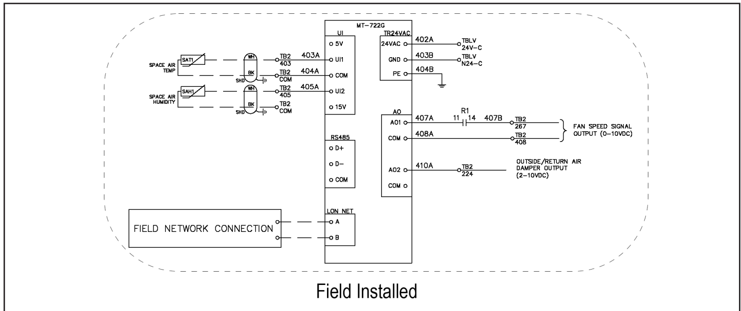
Figure 40: Sample Wiring Diagram (4)
