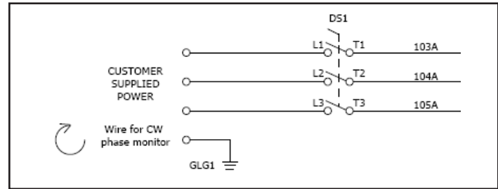
Figure 1: Customer Supplied Power Schematic
