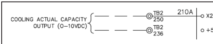
Figure 9: Compressor Actual Capacity Output Schematic
