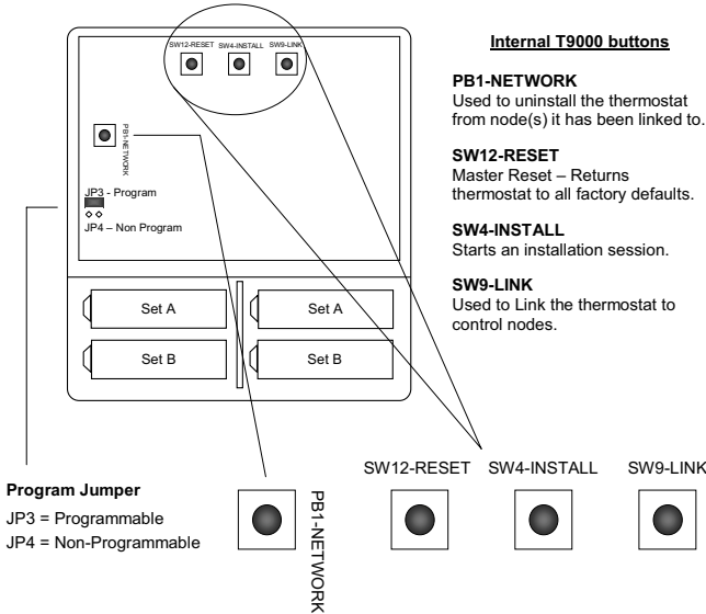
Figure 8: Internal Buttons
