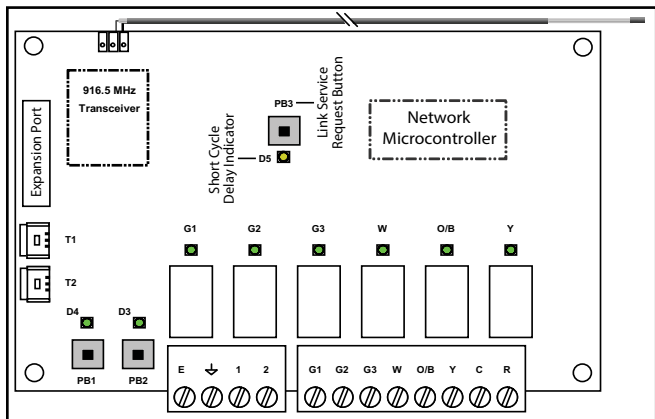
Figure 10: Wireless Control Node
