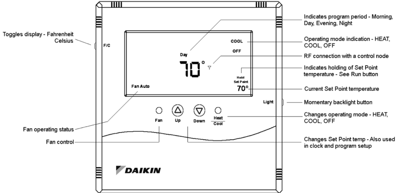
Figure 13: T9000 Non-Programmable Overview - (PN 668898101)
