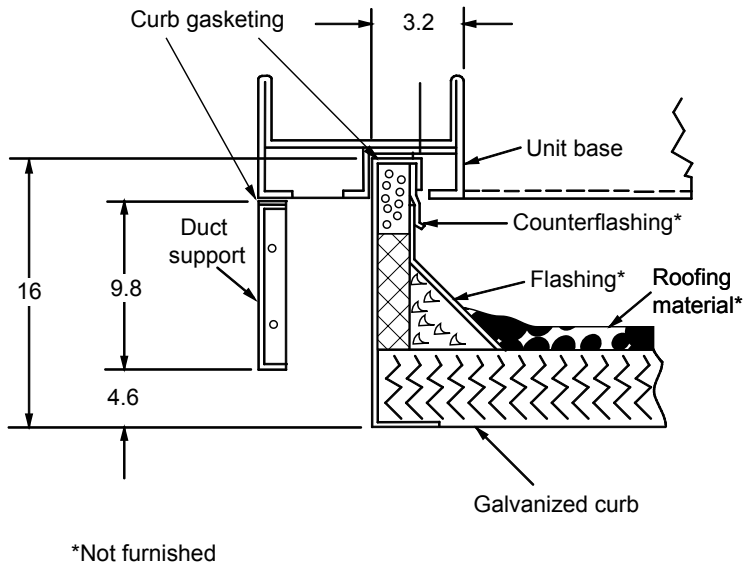
Figure 116: Curb Cross Section
