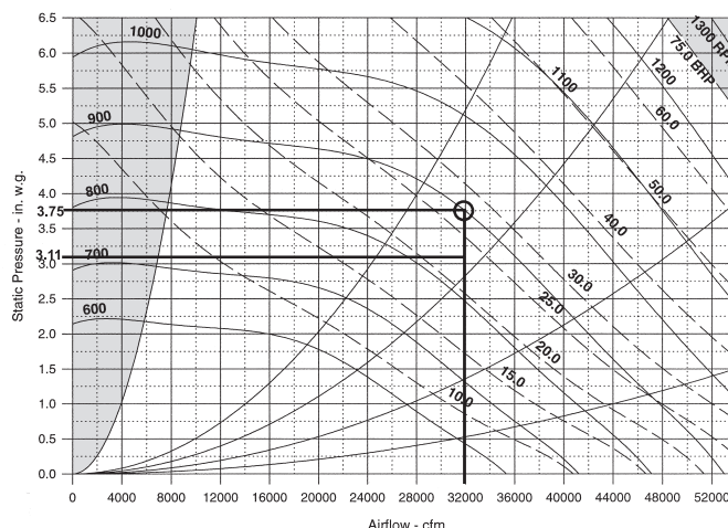
Figure 36: RPS 105C to 135C 40" DWDI Airfoil
