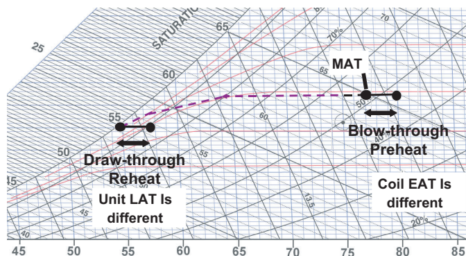
Figure 35: Blow-Through vs. Draw-Through Performance
