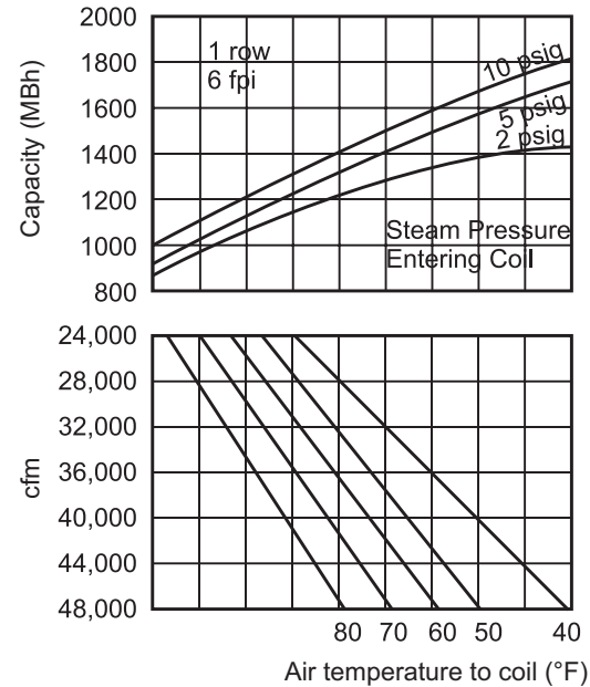
Figure 56: Steam Coil, Low Capacity, 080D to 140D
