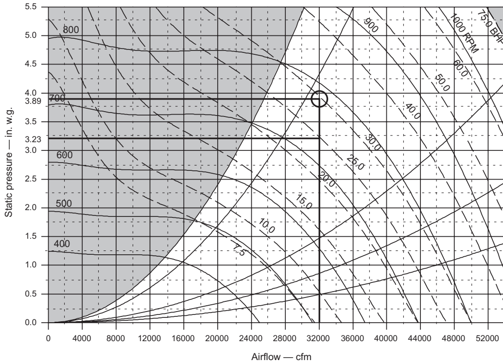
Figure 70: RDT 080D to 140D 49 in. SWSI Airfoil Supply Fan
