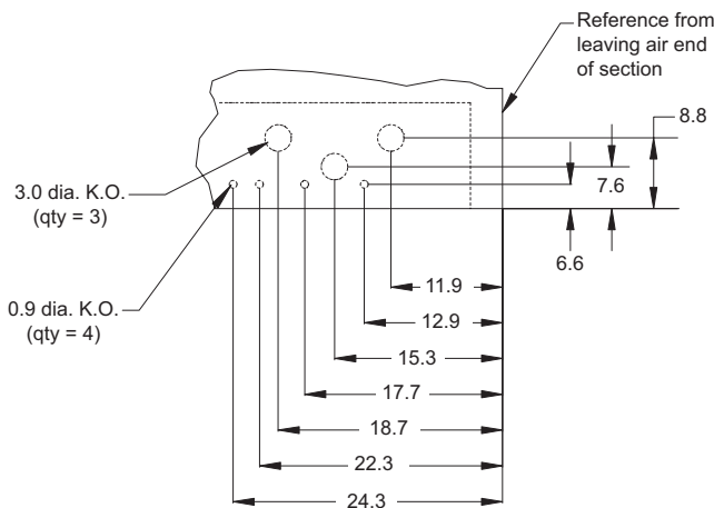
Figure 101: Electric Heat/Heat Section
