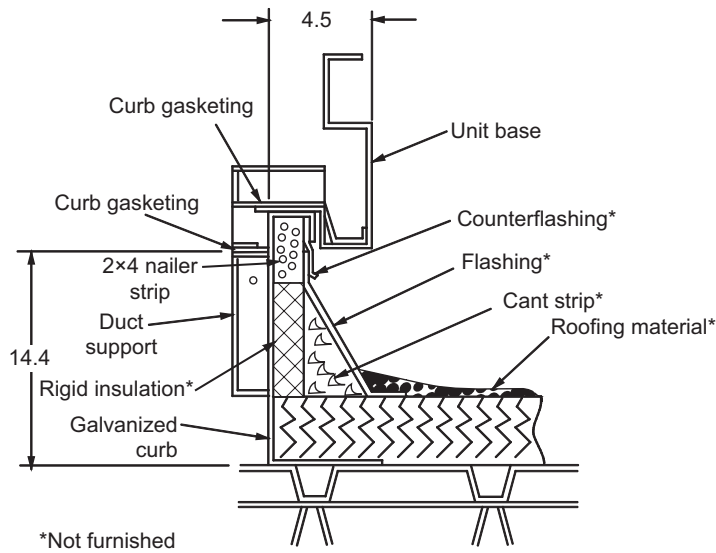
Figure 115: Curb Cross Section
