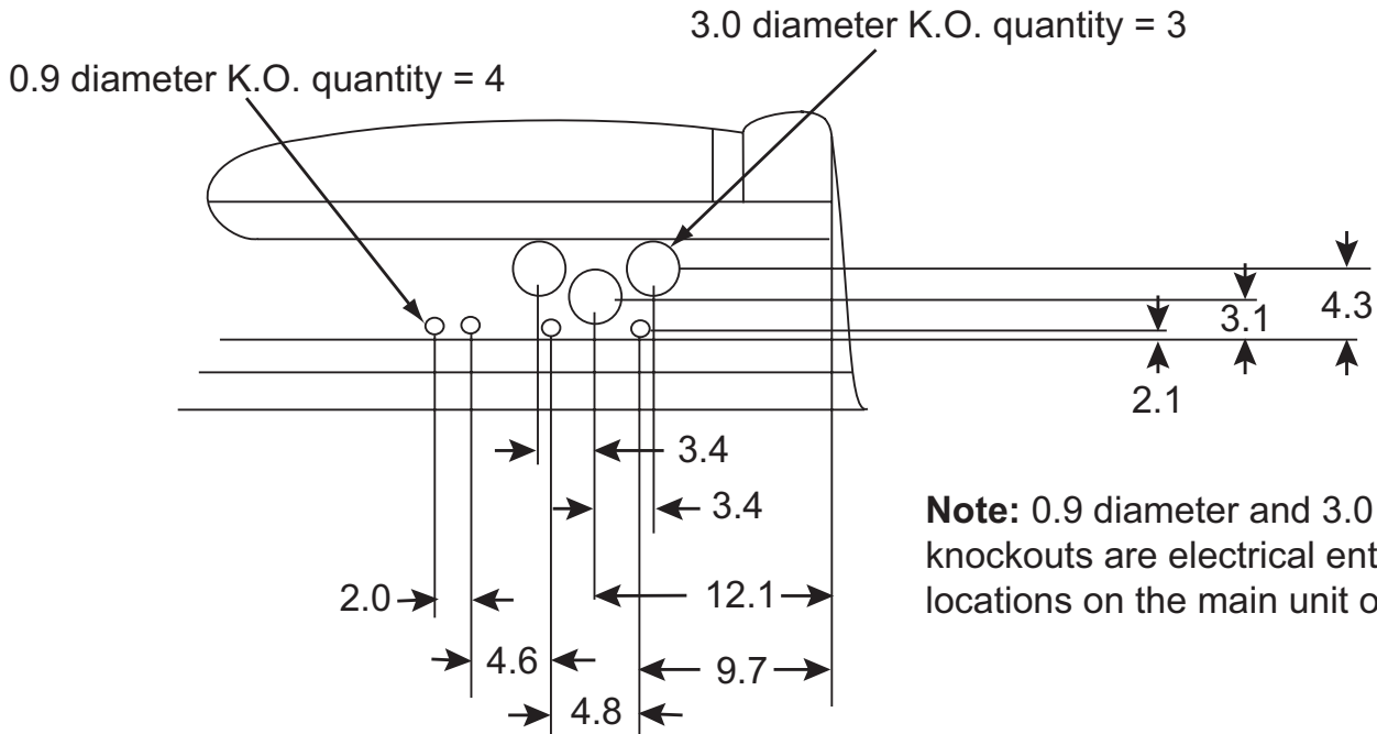
Figure 118: Knockout Detail, 045D to 140D
