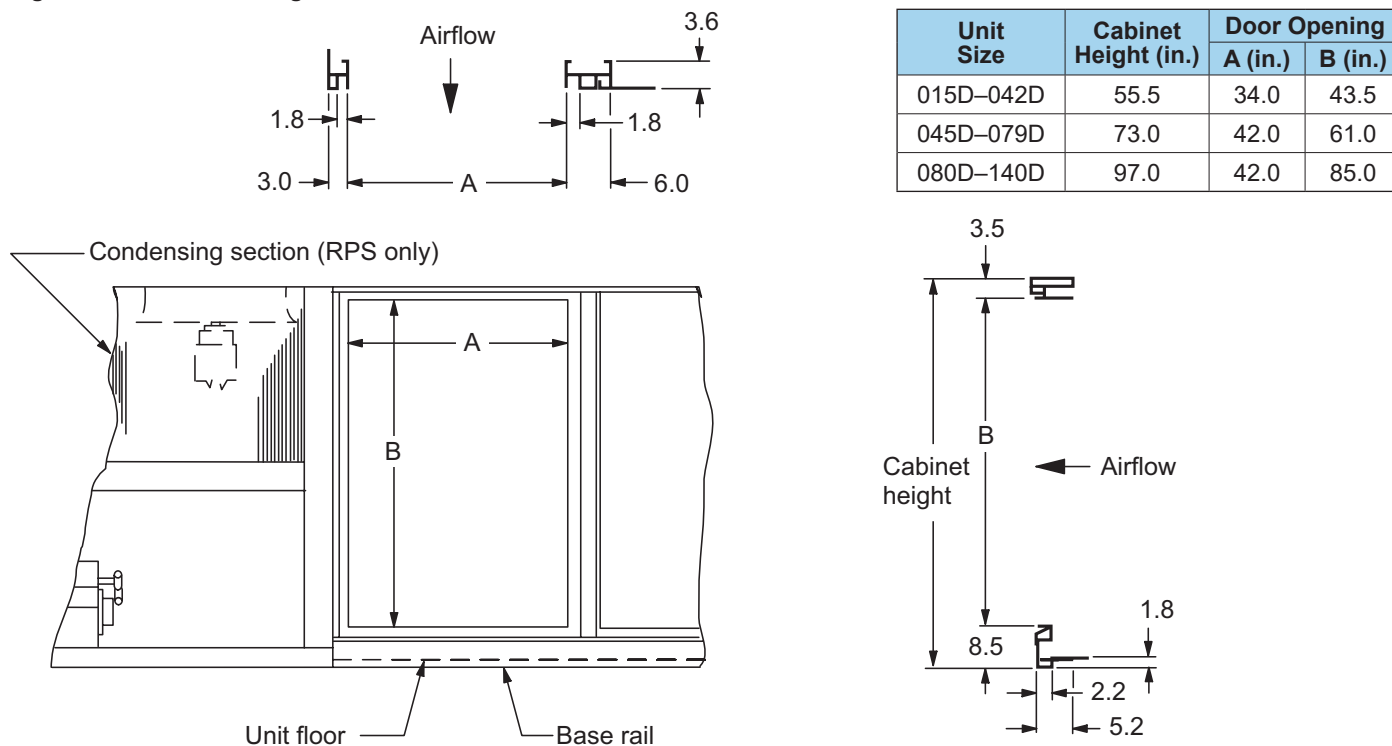
Figure 105: Side Discharge
