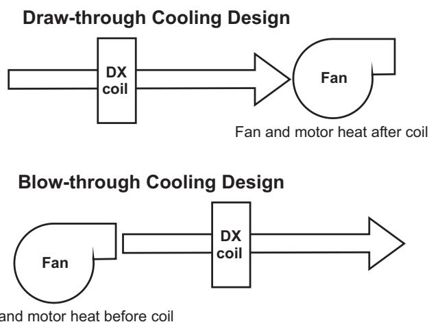
Figure 34: Blow-Through vs. Draw-Through Concept
