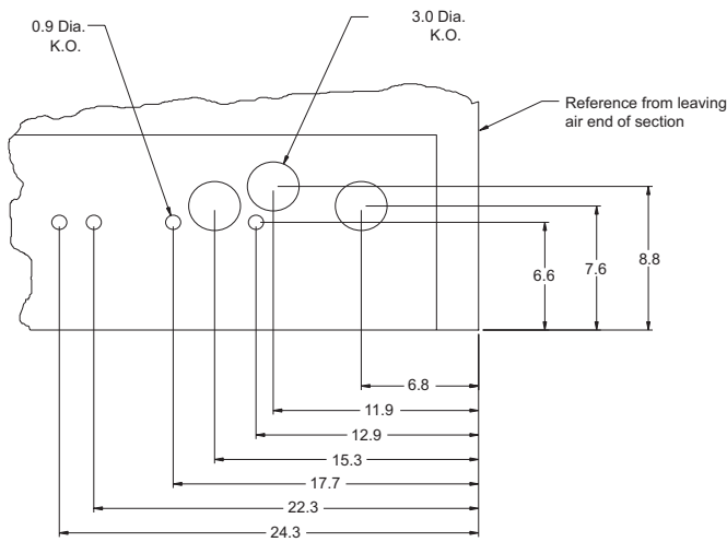
Figure 100: Main Control Panel/Discharge Plenum, RPS/RFS/RDT 045D to 140D
