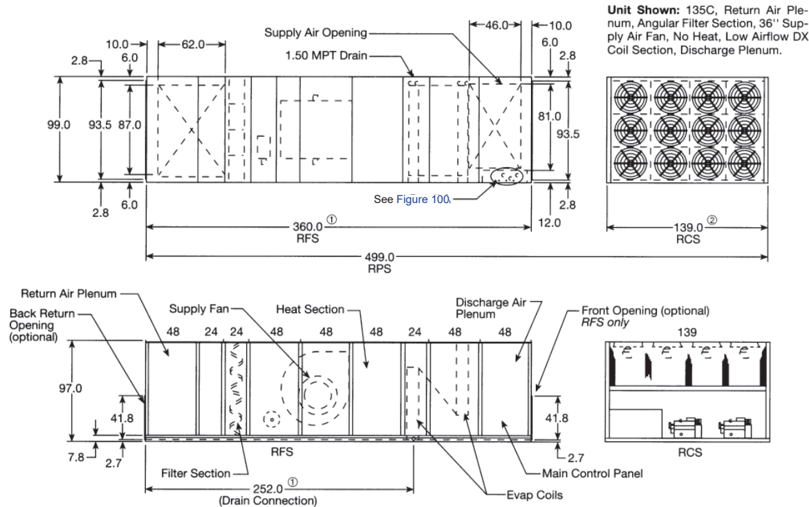
Figure 95: RPS/RFS/RCS 110D to 140D
