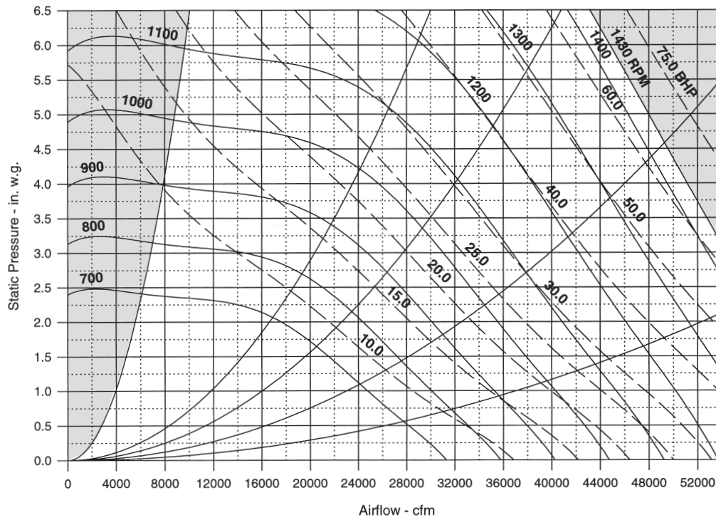
Figure 72: RPS/RFS 080D to 140D 36 in. Airfoil Supply Fan
