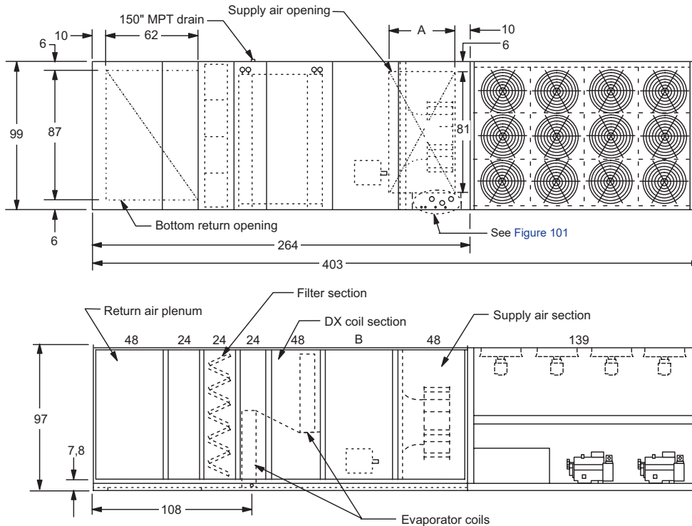
Figure 98: RDT 080D to 140D
