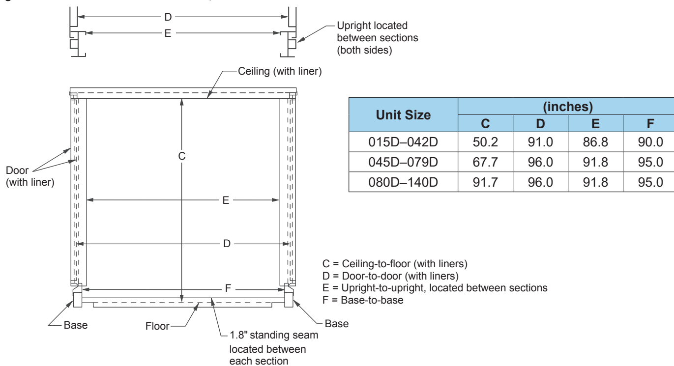
Figure 106: Internal Cabinet Clearance, Air Toward Face
