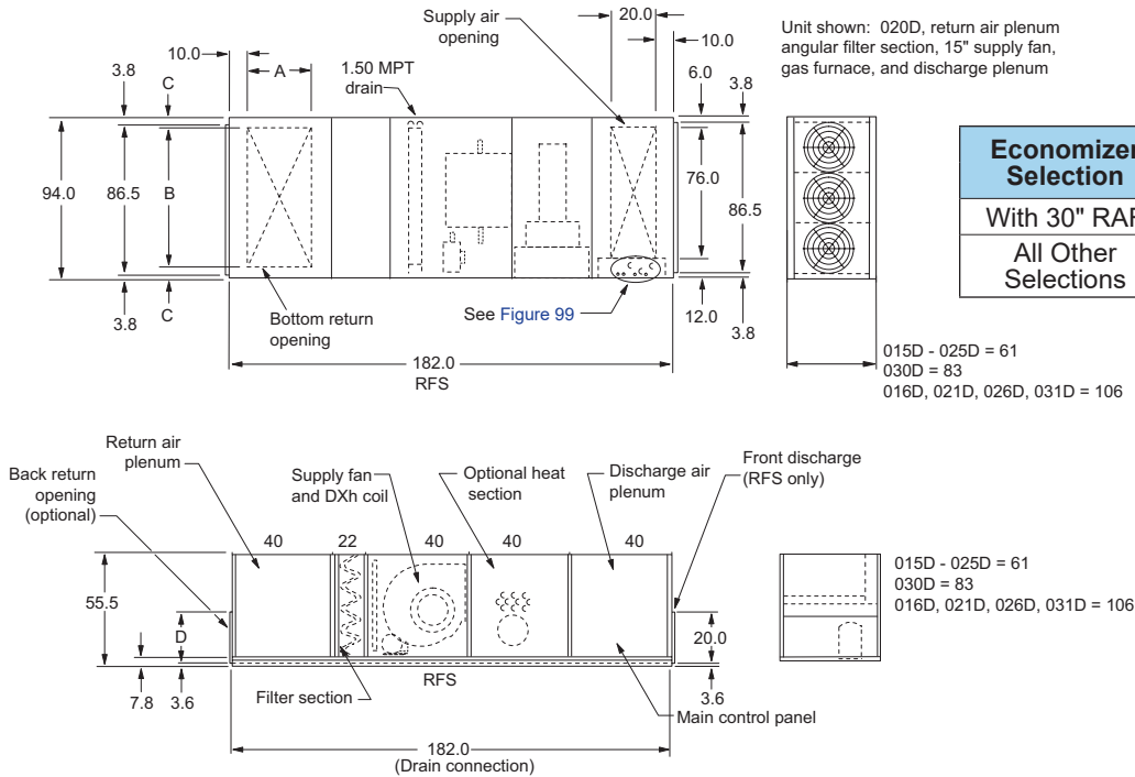
Figure 91: RPS/RFS/RCS 015D to 031D, Basic Configuration
