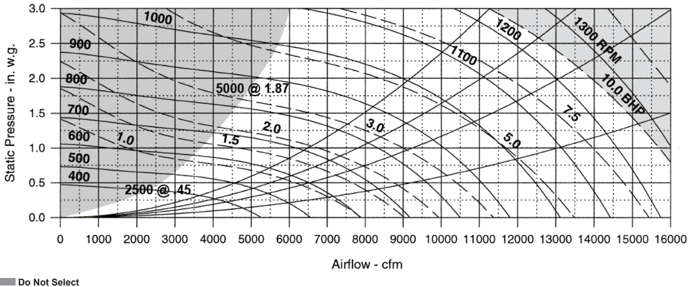
Figure 78: RPS/RFS 015D to 042D, 30 in. SWSI Airfoil Return Fan*
