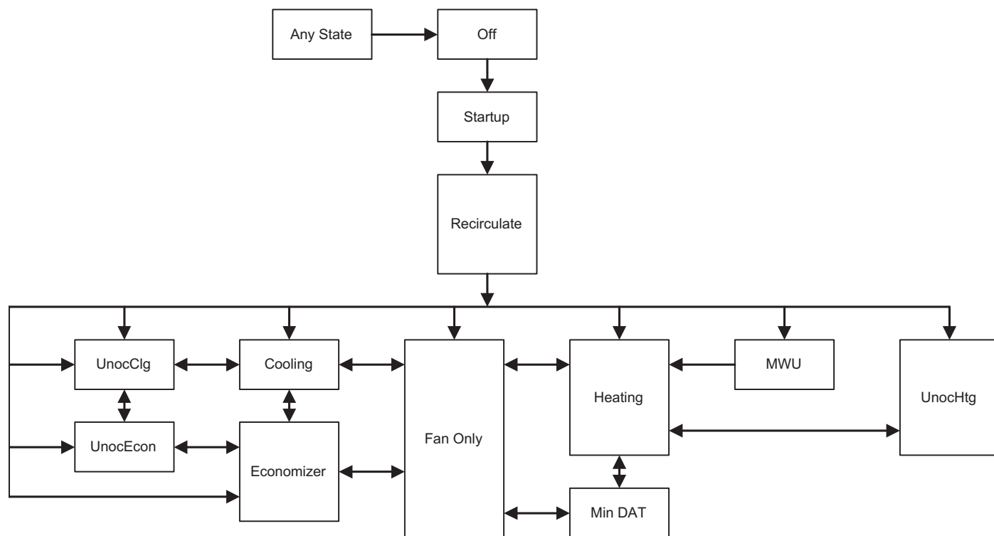
Figure 30: Operating State Sequence Chart
