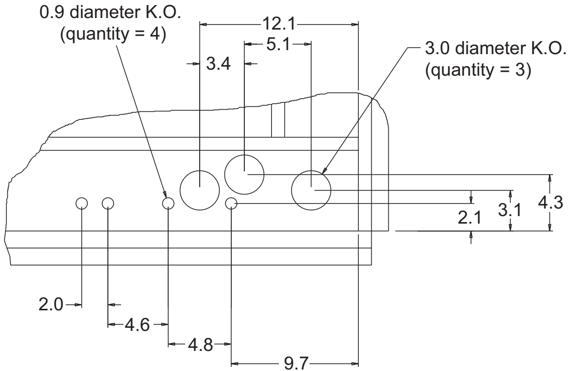
Figure 117: Knockout Detail, 025D to 042D
