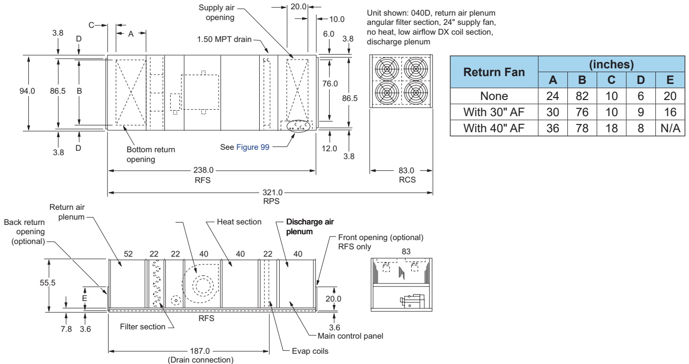
Figure 92: RPS/RFS/RCS 035D to 042D, Basic Configuration
