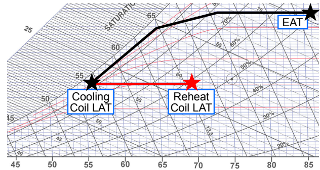
Figure 8: Modulating hot gas reheat is the best way to provide dehumidified 100% outdoor air at 70°F/60% RH
