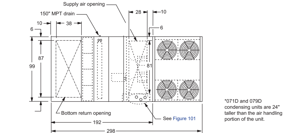
Figure 97: RDT 070D to 079D
