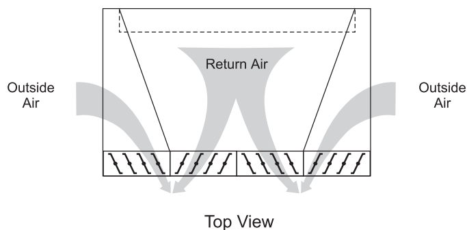
Figure 14: Economizer Airflow
