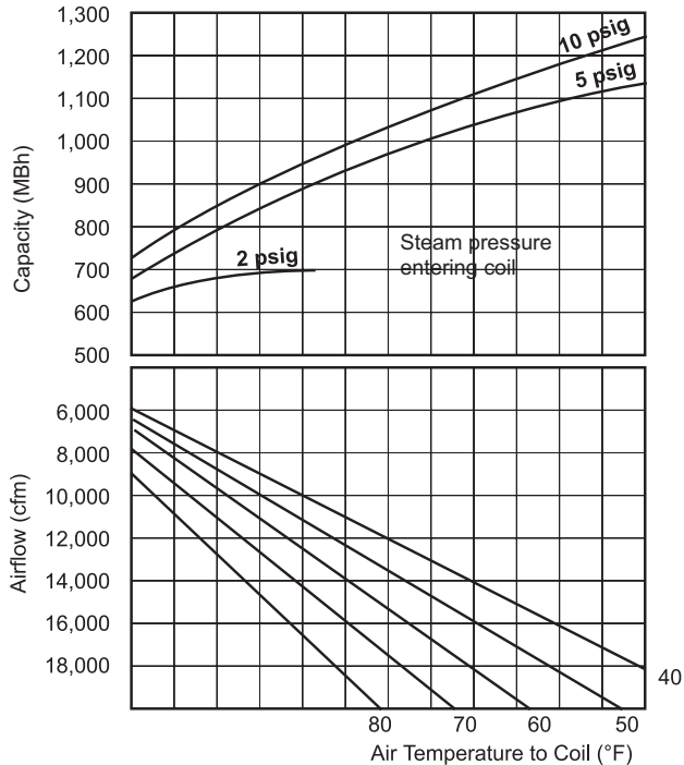
Figure 51: Steam Coil, High Capacity, 015D to 042D
