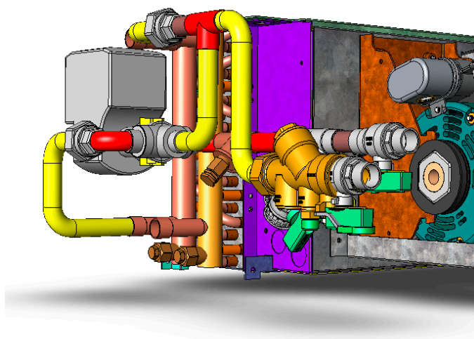
Figure 4: Deluxe Valve and Piping Package
