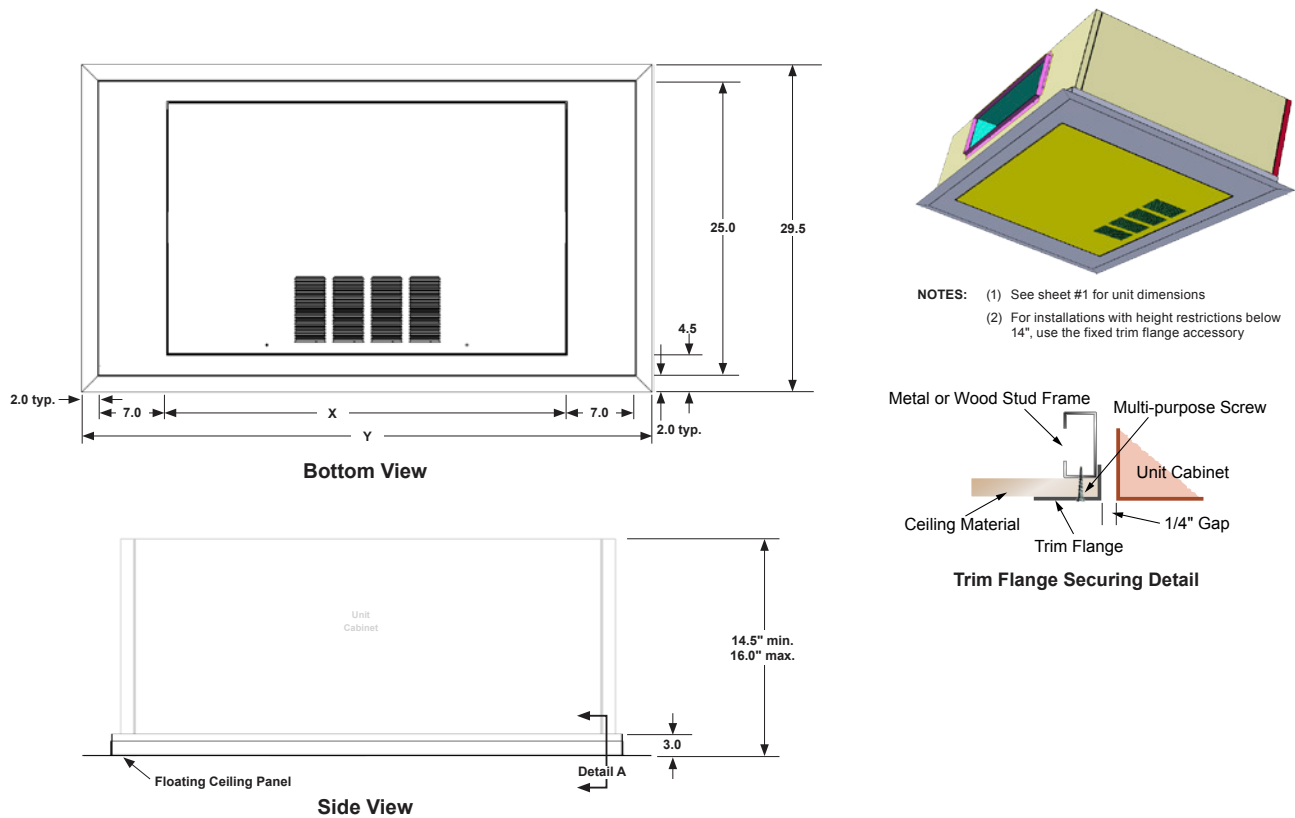
Figure 21: Dimensions – Trim Flange Mount
