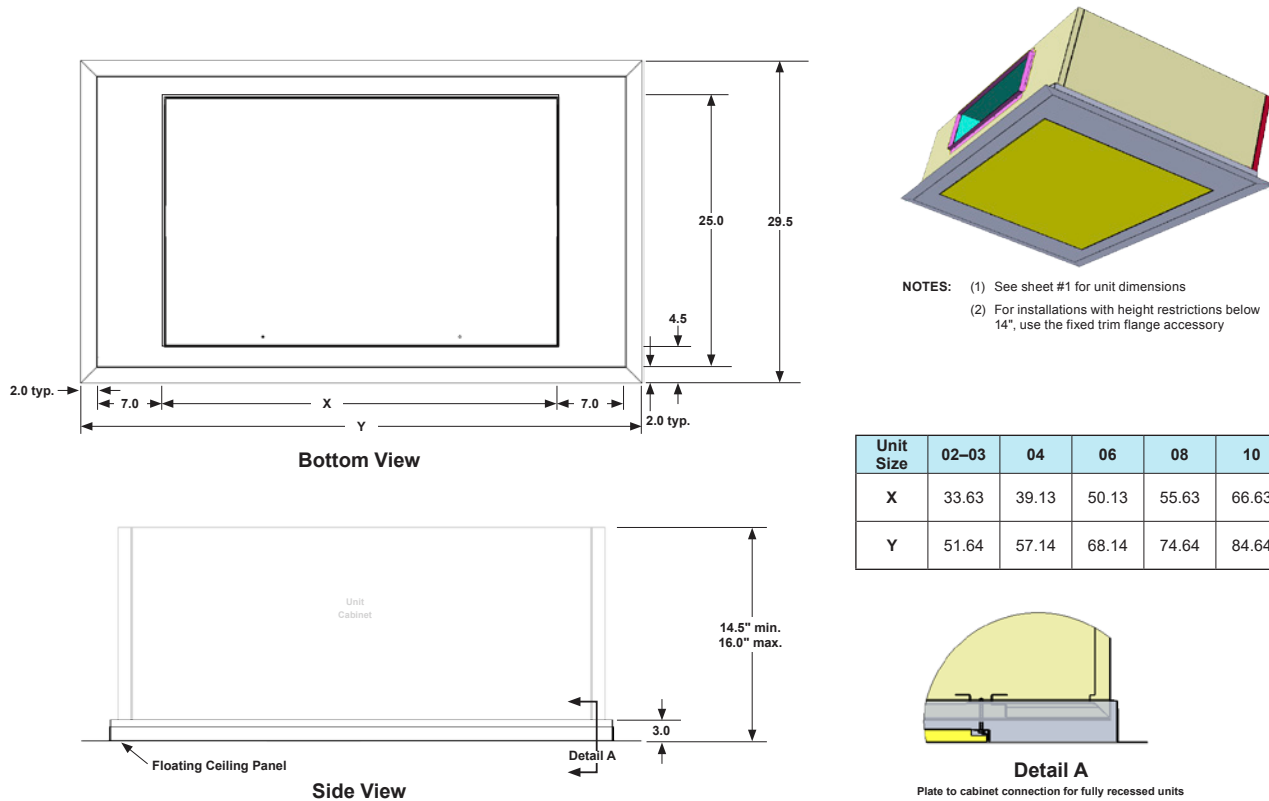
Figure 21: Dimensions – Trim Flange Mount
